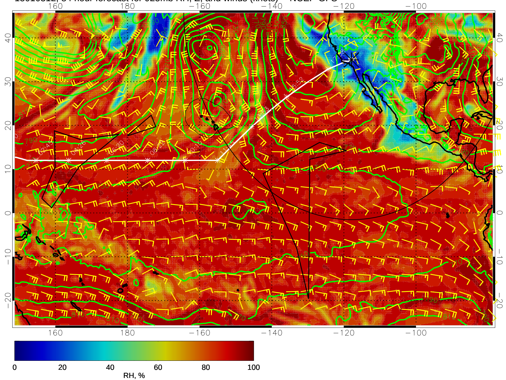
15010312, 84 hour forecast for 925mb RH, Z, and winds (knots) -- NCEP GFS
