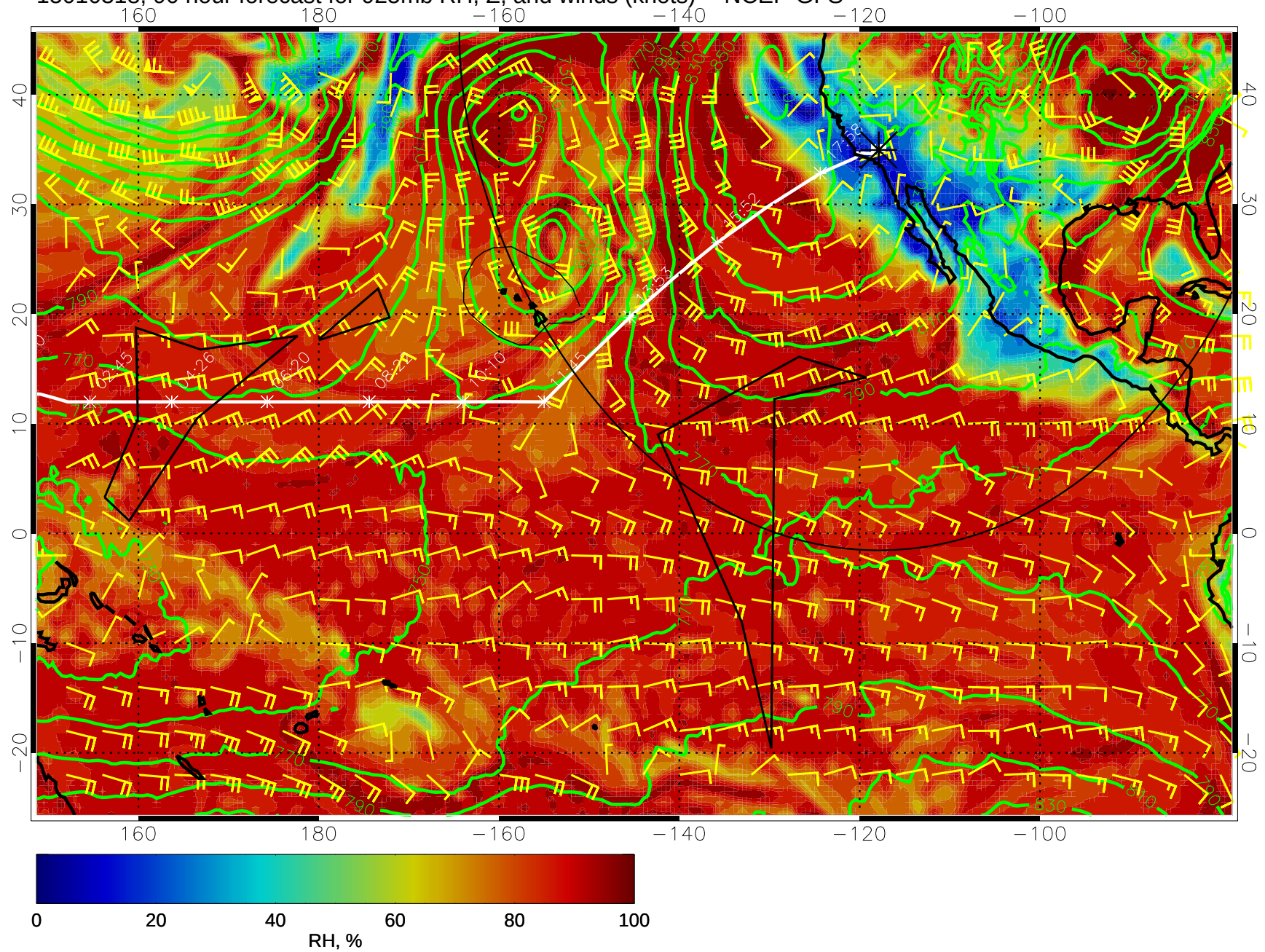
15010318, 90 hour forecast for 925mb RH, Z, and winds (knots) -- NCEP GFS
