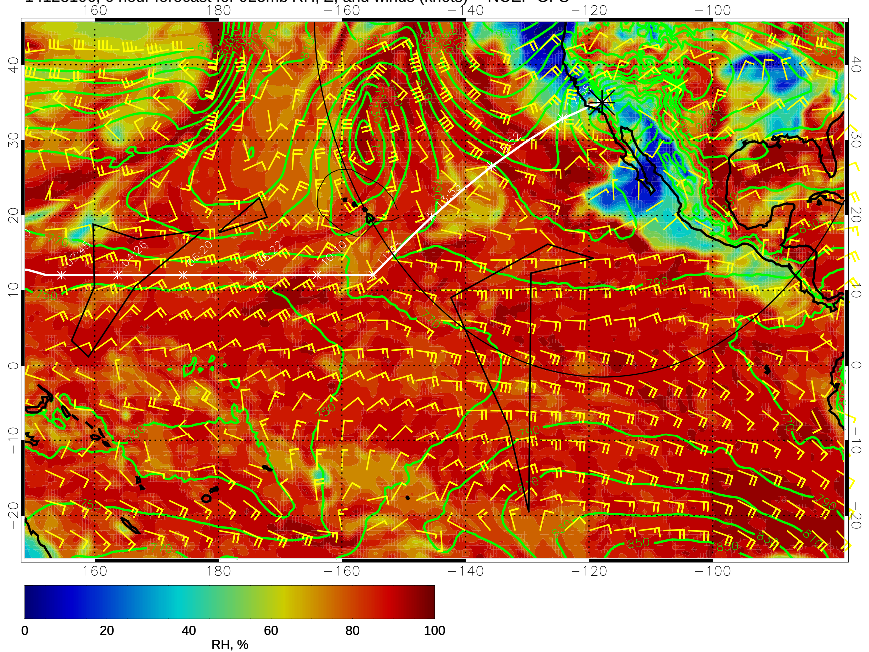
14123106, 6 hour forecast for 925mb RH, Z, and winds (knots) -- NCEP GFS
