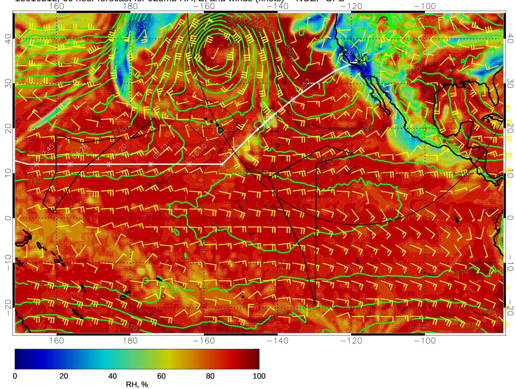
15010212, 60 hour forecast for 925mb RH, Z, and winds (knots) -- NCEP GFS
