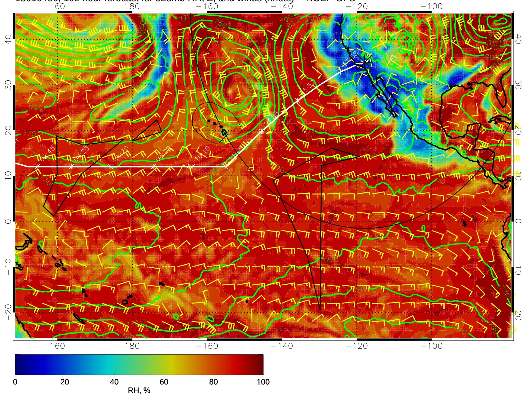
15010406, 102 hour forecast for 925mb RH, Z, and winds (knots) -- NCEP GFS
