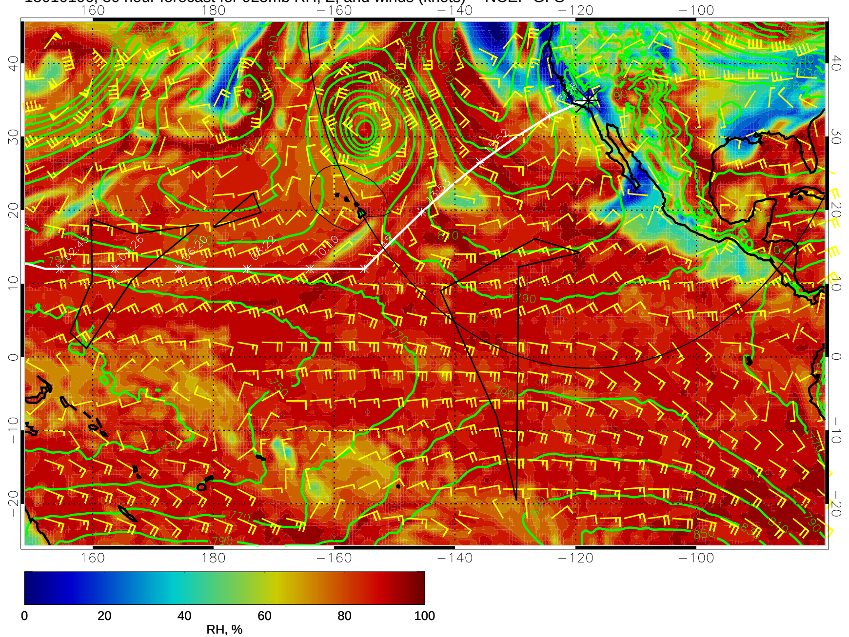
15010106, 30 hour forecast for 925mb RH, Z, and winds (knots) -- NCEP GFS
