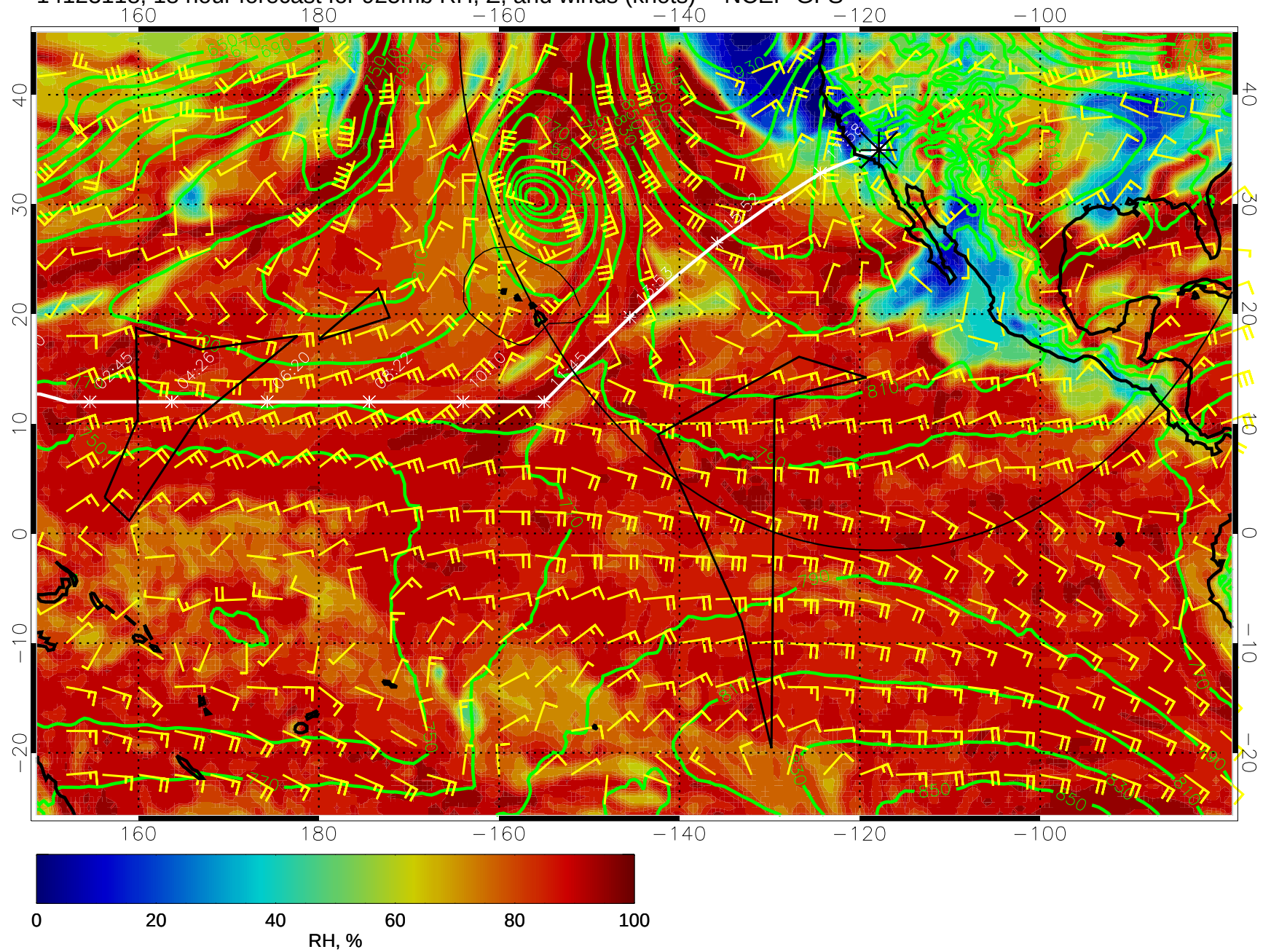
14123118, 18 hour forecast for 925mb RH, Z, and winds (knots) -- NCEP GFS
