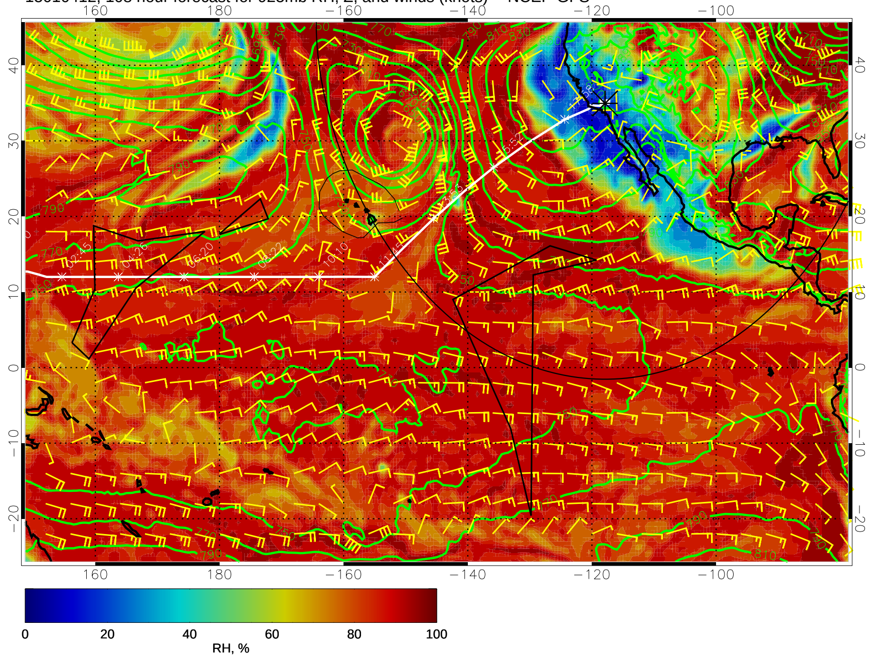
15010412, 108 hour forecast for 925mb RH, Z, and winds (knots) -- NCEP GFS
