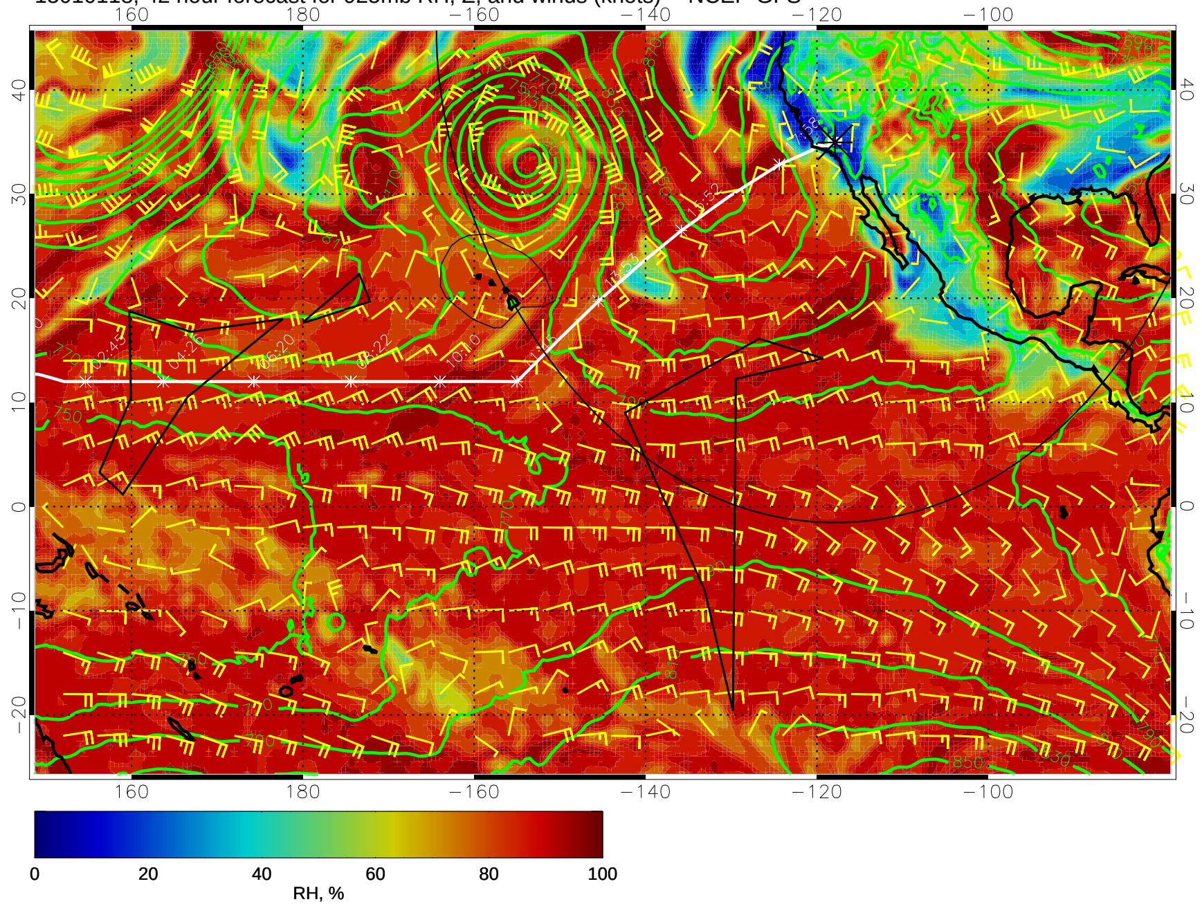
15010118, 42 hour forecast for 925mb RH, Z, and winds (knots) -- NCEP GFS
