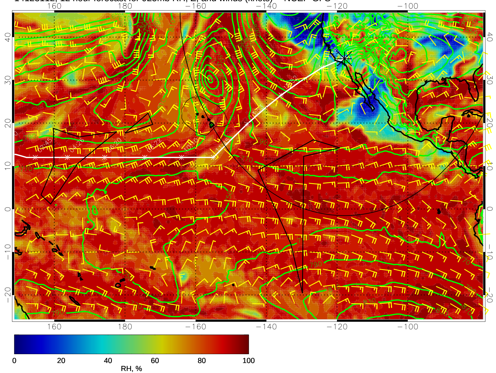
14123112, 12 hour forecast for 925mb RH, Z, and winds (knots) -- NCEP GFS
