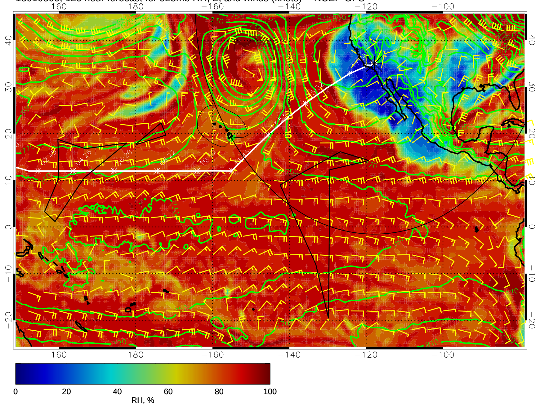
15010500, 120 hour forecast for 925mb RH, Z, and winds (knots) -- NCEP GFS
