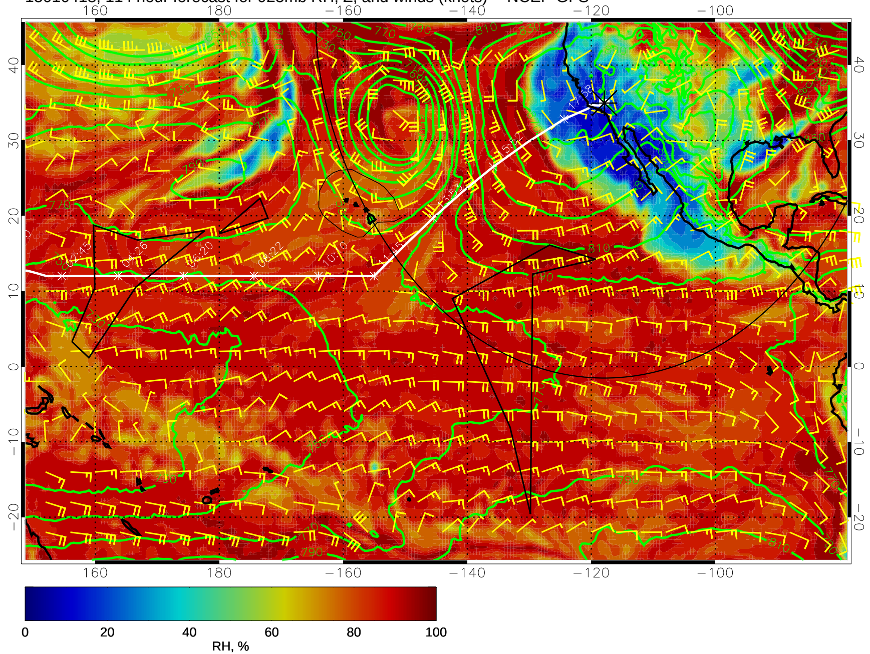
15010418, 114 hour forecast for 925mb RH, Z, and winds (knots) -- NCEP GFS
