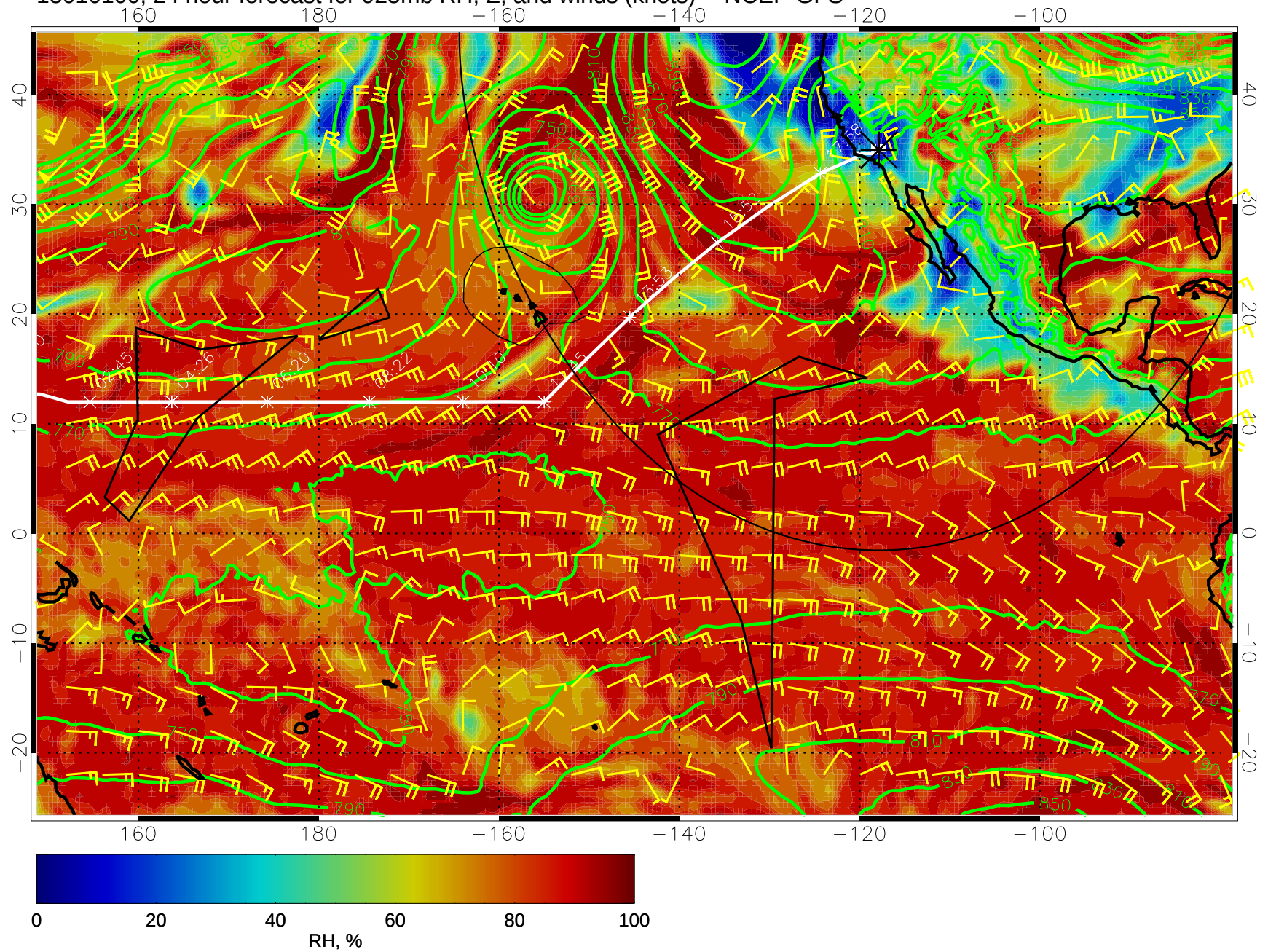
15010100, 24 hour forecast for 925mb RH, Z, and winds (knots) -- NCEP GFS
