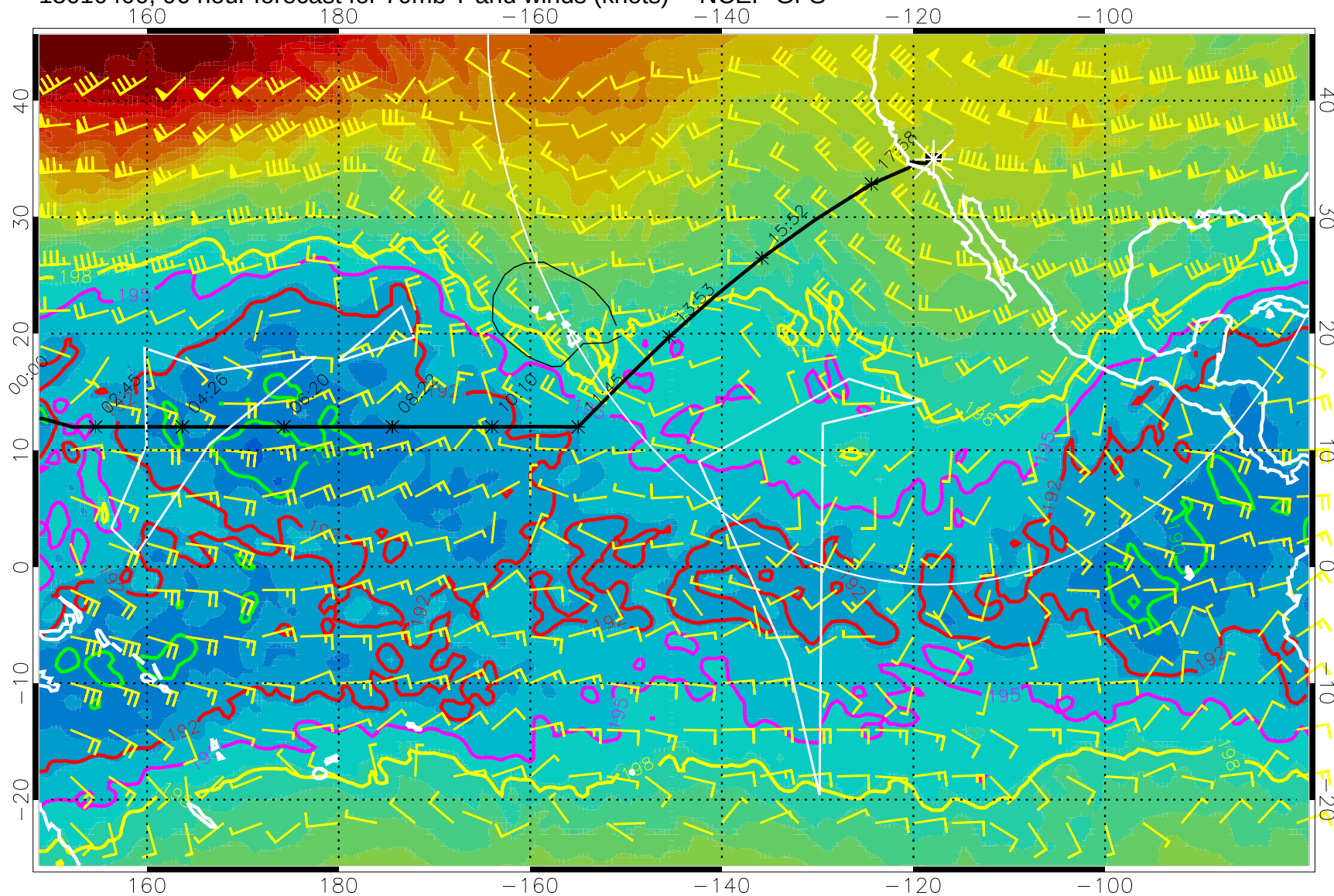
15010400, 96 hour forecast for 70mb T and winds (knots) -- NCEP GFS
