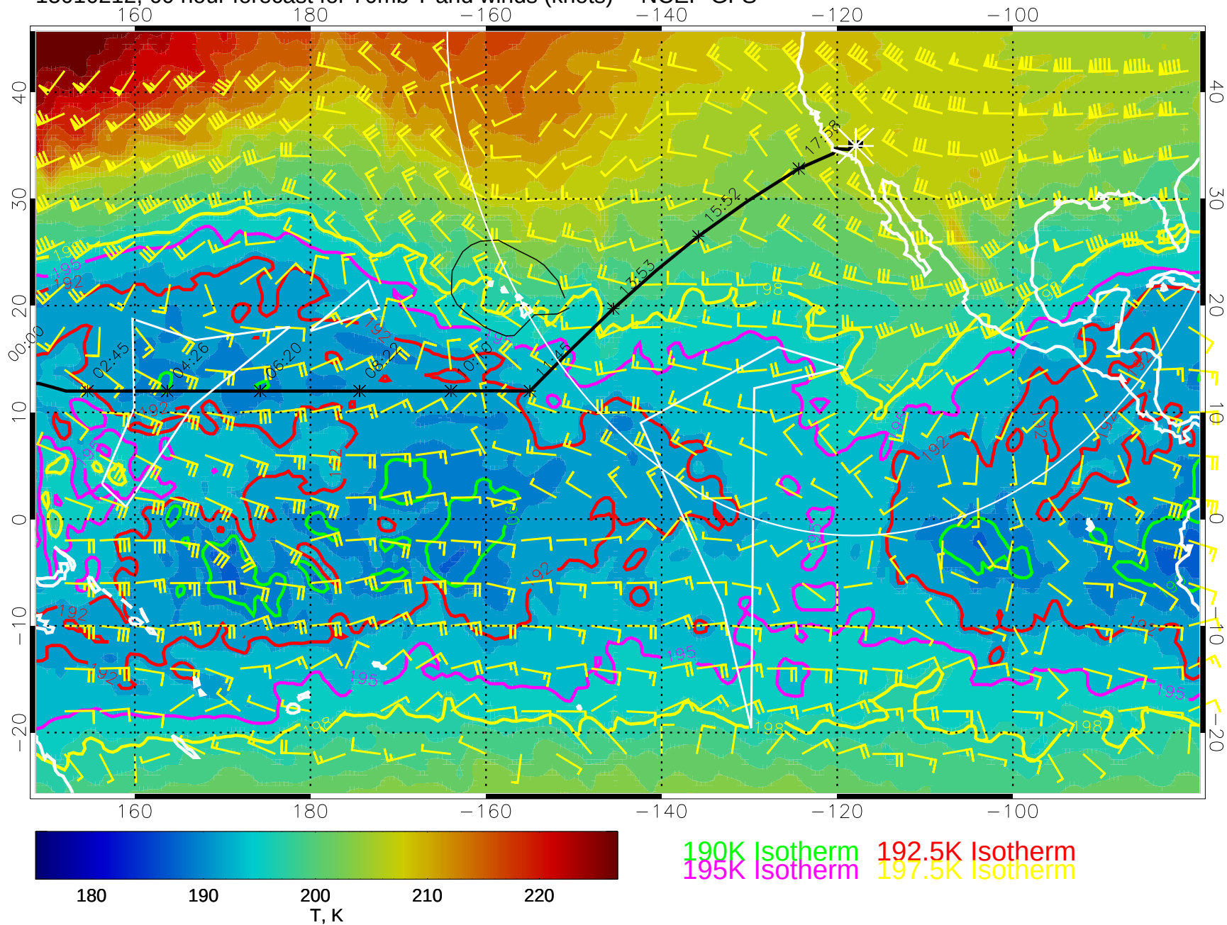
15010212, 60 hour forecast for 70mb T and winds (knots) -- NCEP GFS
