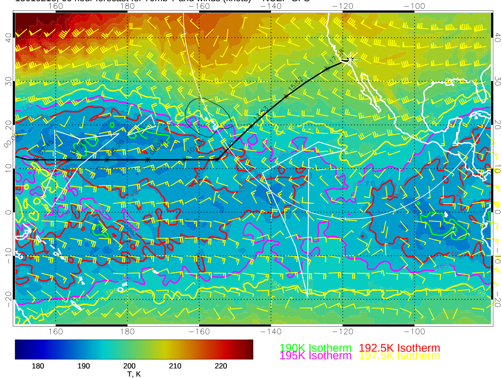
15010218, 66 hour forecast for 70mb T and winds (knots) -- NCEP GFS
