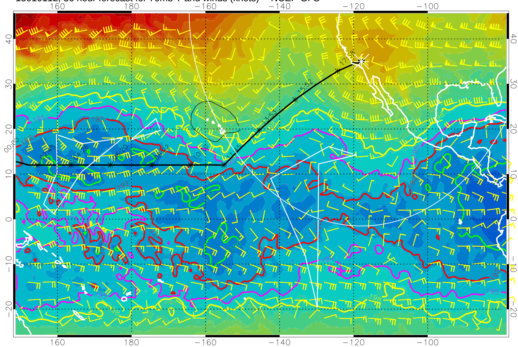
15010112, 36 hour forecast for 70mb T and winds (knots) -- NCEP GFS
