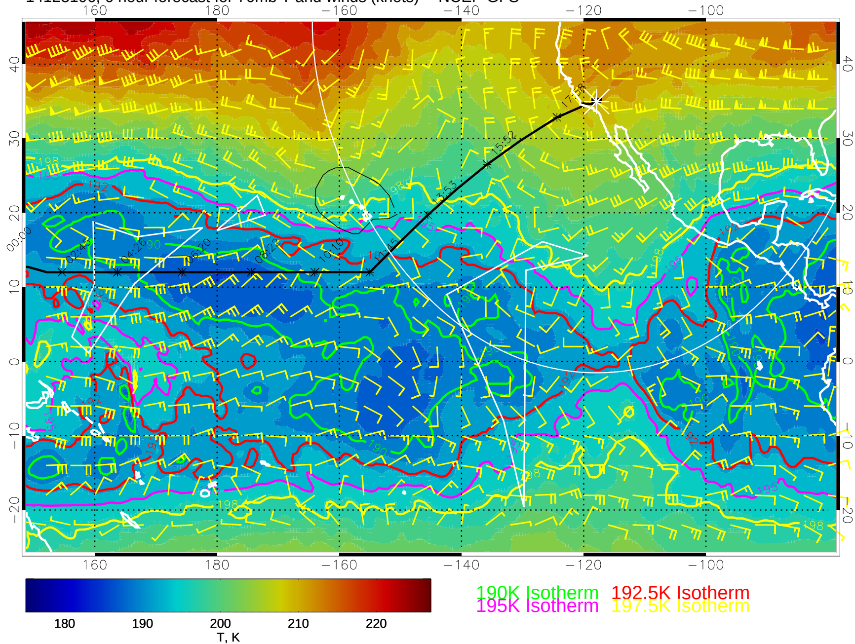
14123106, 6 hour forecast for 70mb T and winds (knots) -- NCEP GFS
