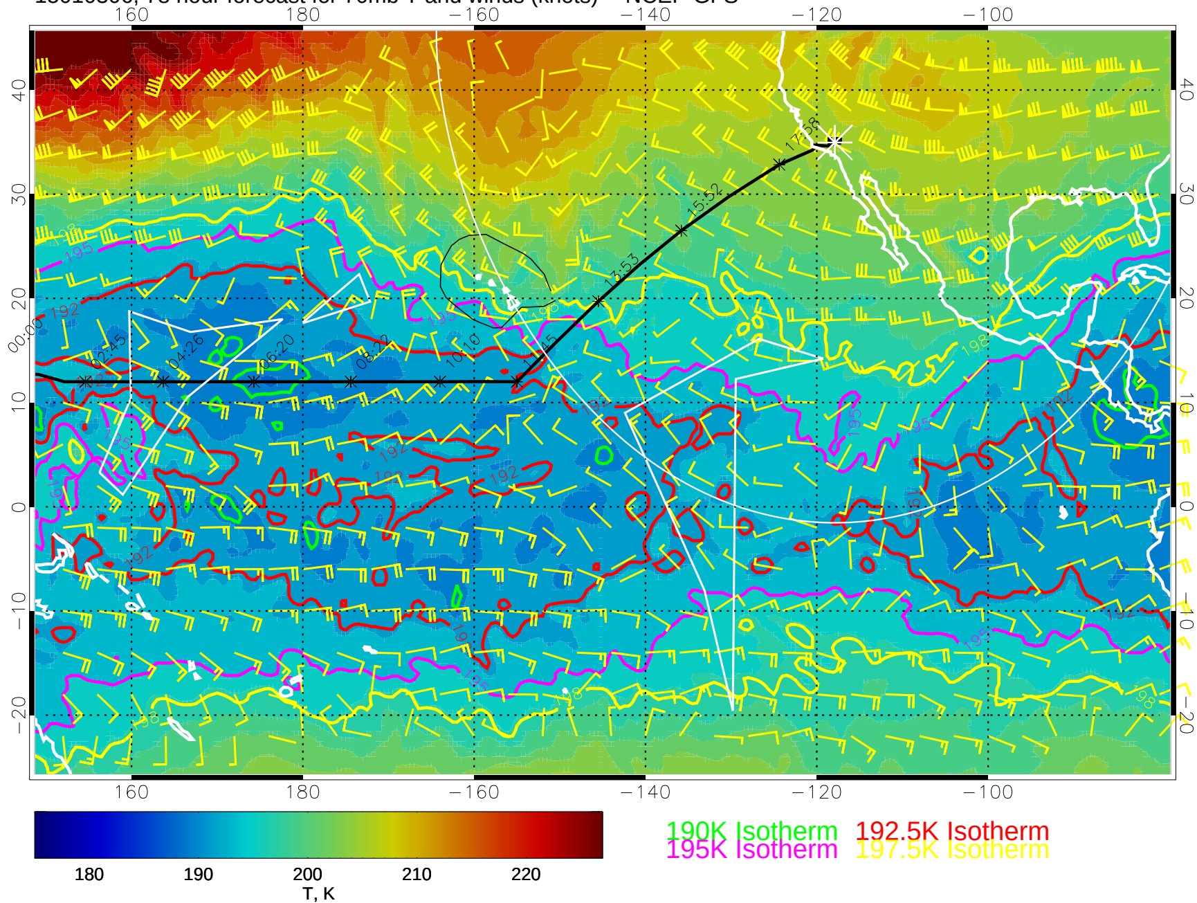
15010306, 78 hour forecast for 70mb T and winds (knots) -- NCEP GFS
