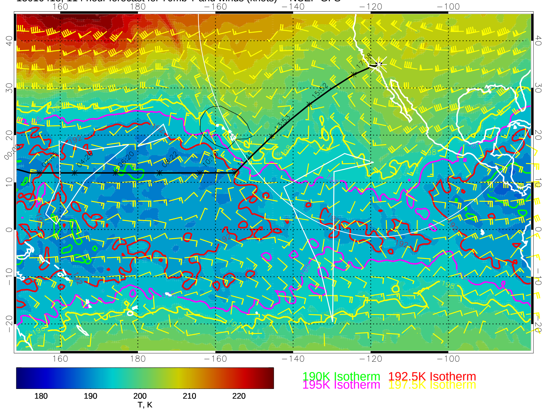
15010418, 114 hour forecast for 70mb T and winds (knots) -- NCEP GFS
