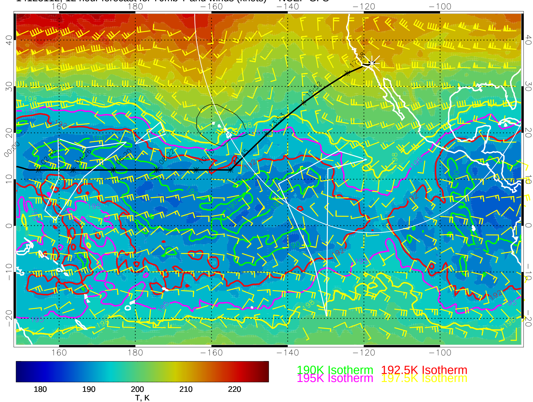
14123112, 12 hour forecast for 70mb T and winds (knots) -- NCEP GFS
