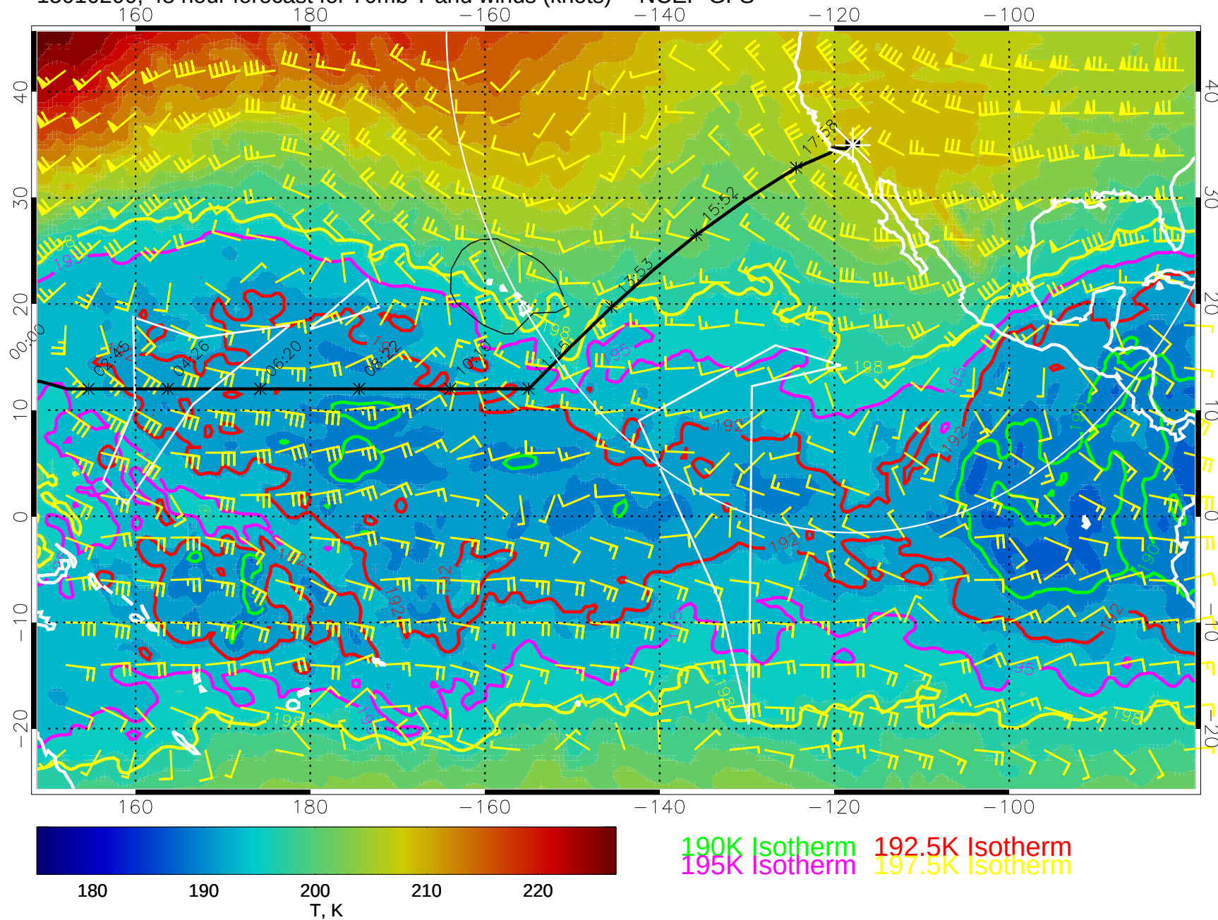
15010200, 48 hour forecast for 70mb T and winds (knots) -- NCEP GFS
