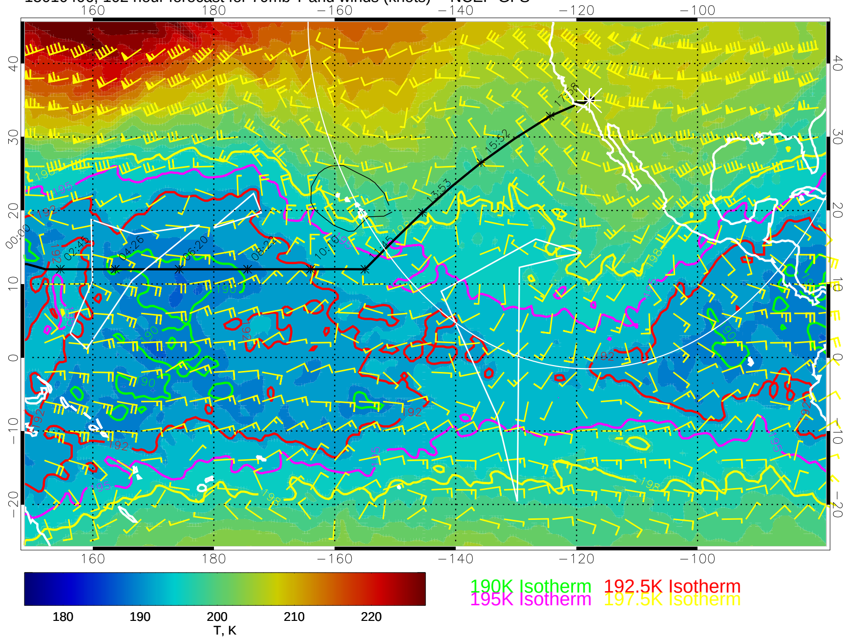
15010406, 102 hour forecast for 70mb T and winds (knots) -- NCEP GFS
