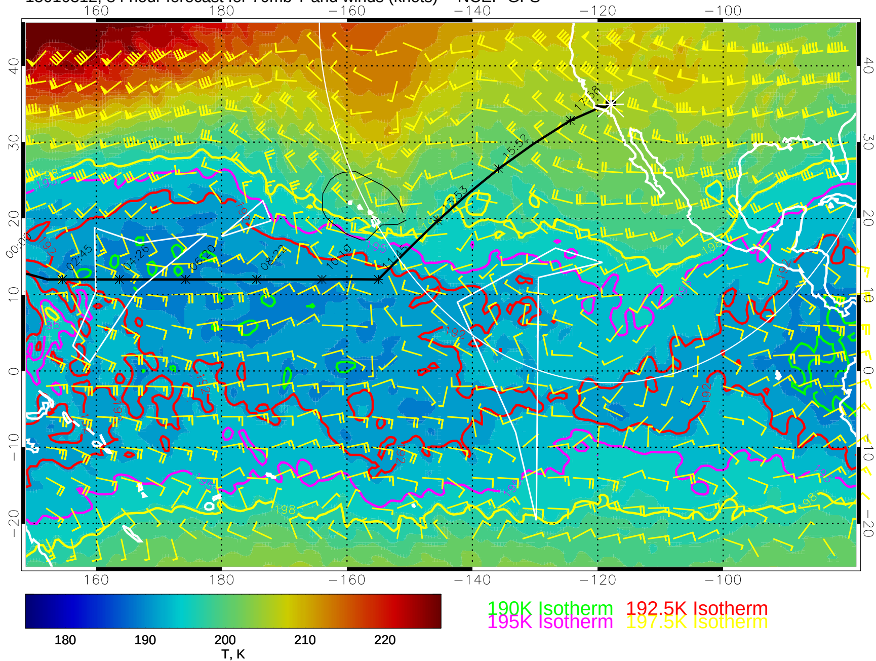
15010312, 84 hour forecast for 70mb T and winds (knots) -- NCEP GFS
