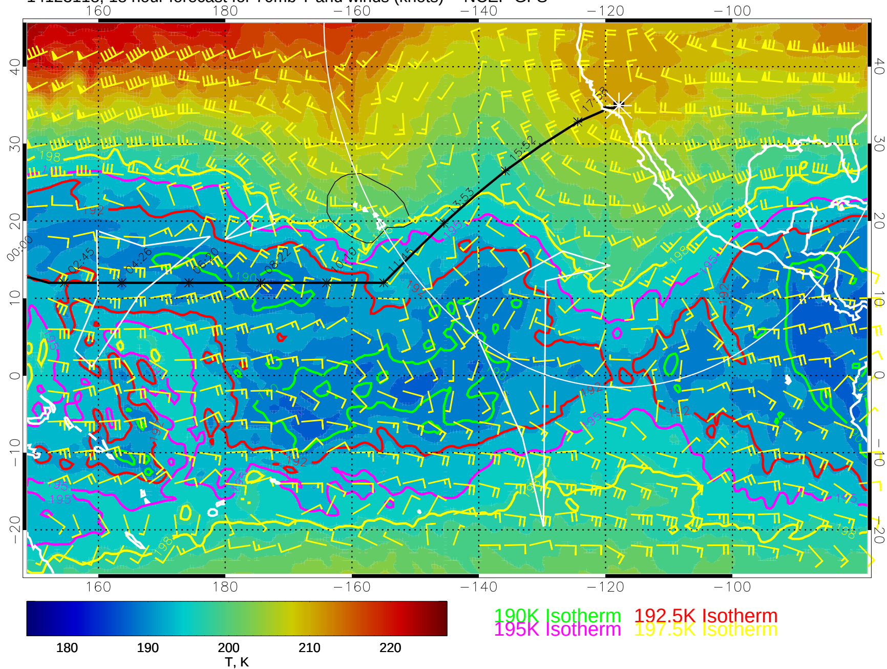
14123118, 18 hour forecast for 70mb T and winds (knots) -- NCEP GFS
