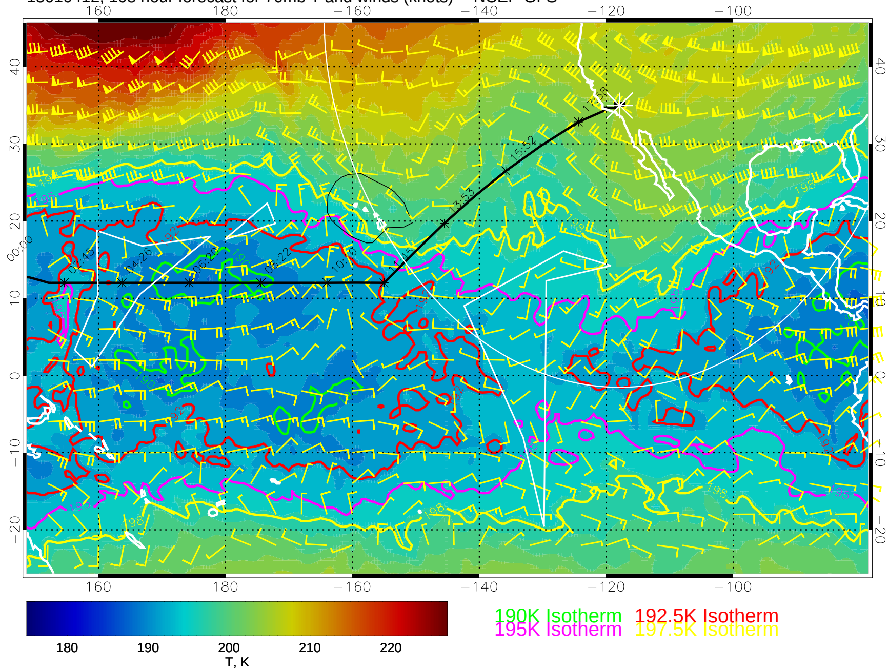
15010412, 108 hour forecast for 70mb T and winds (knots) -- NCEP GFS
