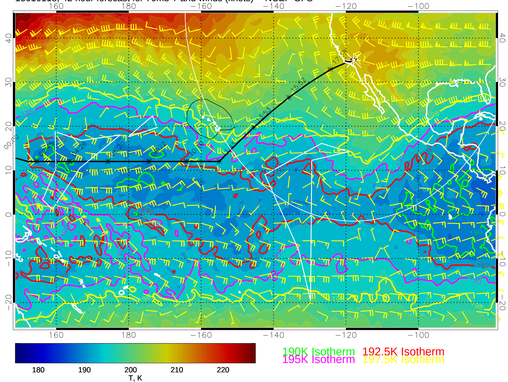
15010118, 42 hour forecast for 70mb T and winds (knots) -- NCEP GFS
