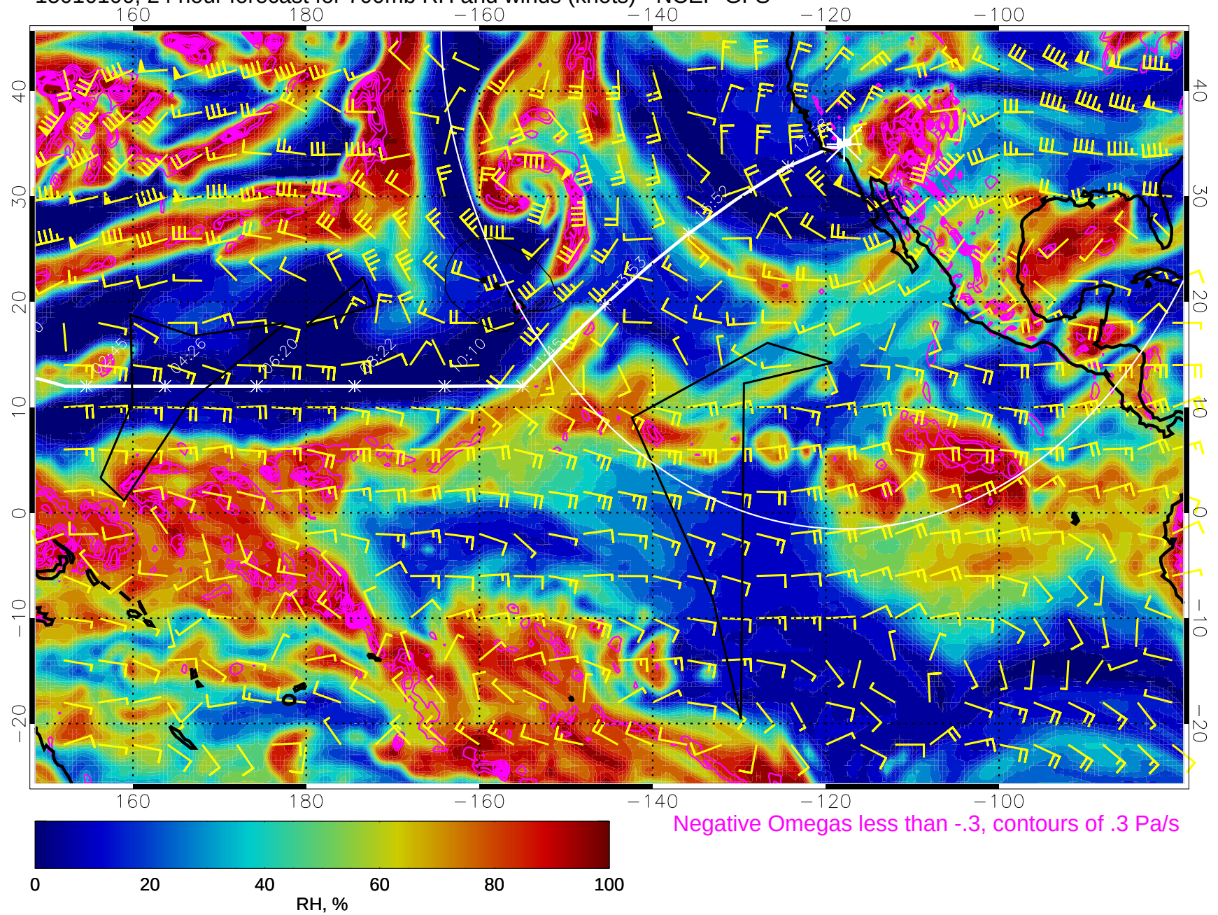
15010100, 24 hour forecast for 700mb RH and winds (knots) - NCEP GFS
