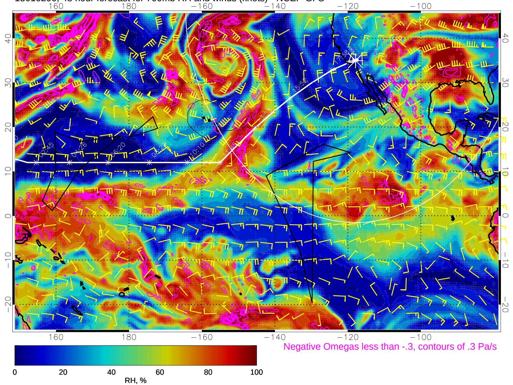
15010200, 48 hour forecast for 700mb RH and winds (knots) - NCEP GFS
