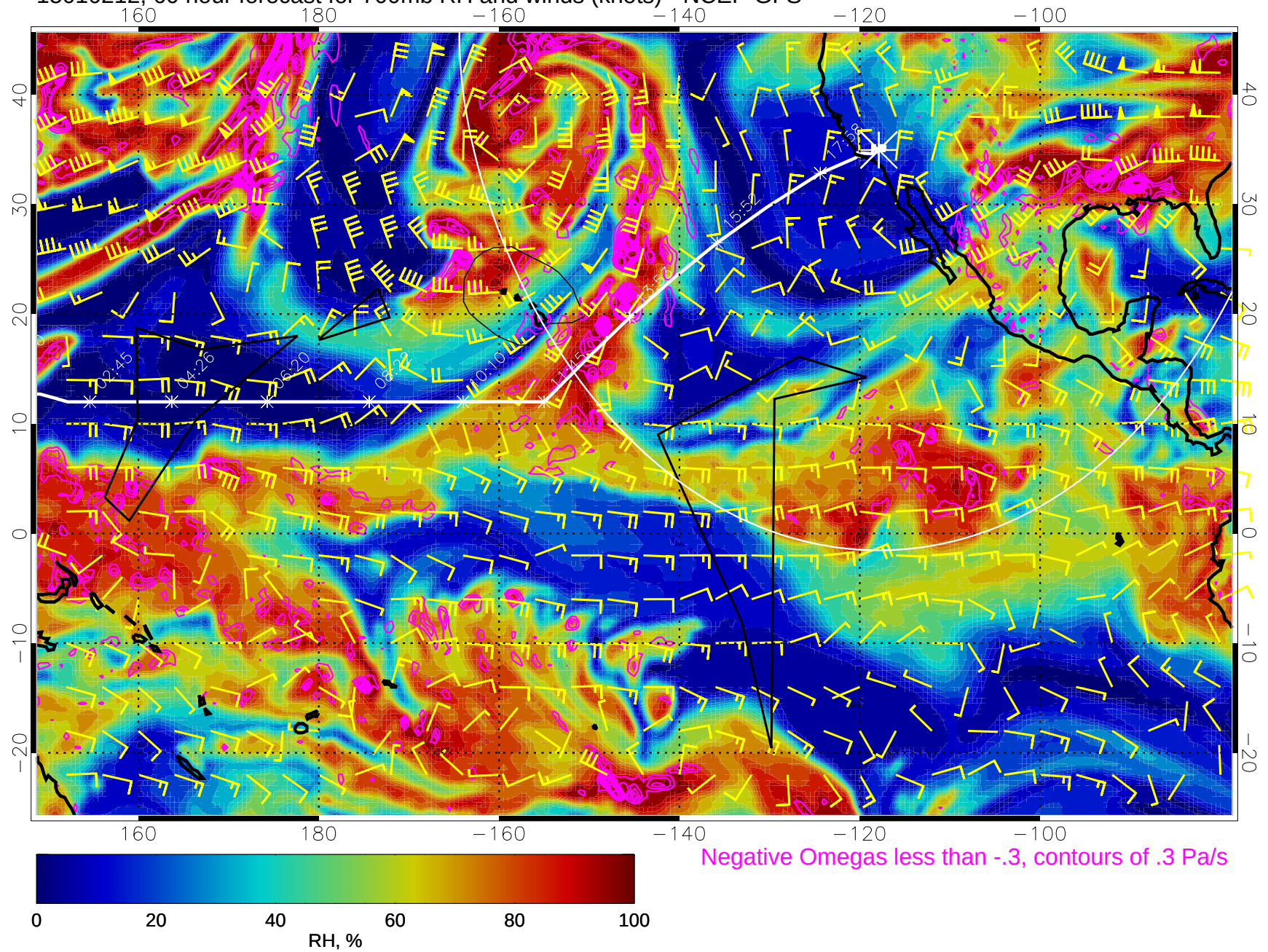
15010212, 60 hour forecast for 700mb RH and winds (knots) - NCEP GFS
