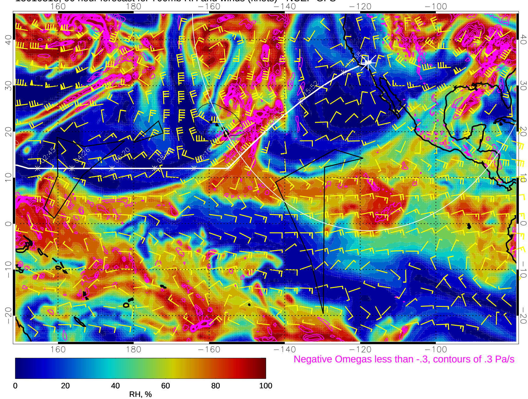
15010318, 90 hour forecast for 700mb RH and winds (knots) - NCEP GFS
