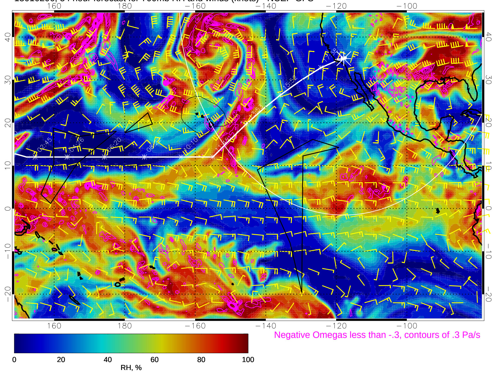
15010206, 54 hour forecast for 700mb RH and winds (knots) - NCEP GFS
