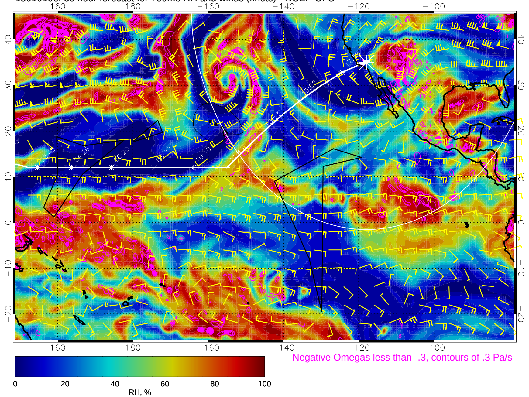
15010106, 30 hour forecast for 700mb RH and winds (knots) - NCEP GFS
