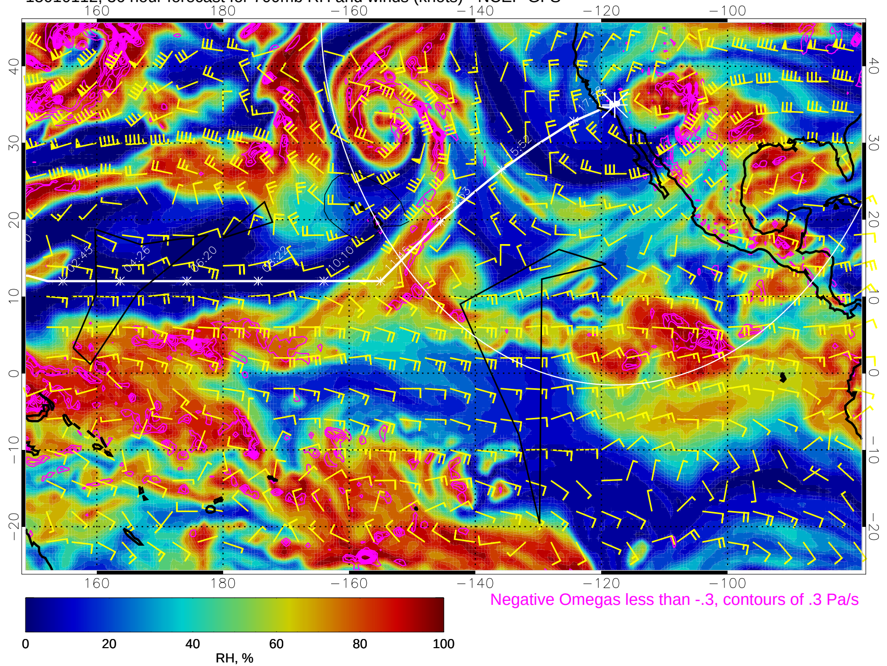
15010112, 36 hour forecast for 700mb RH and winds (knots) - NCEP GFS
