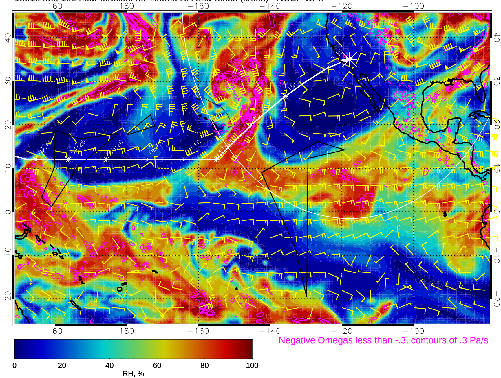
15010406, 102 hour forecast for 700mb RH and winds (knots) - NCEP GFS
