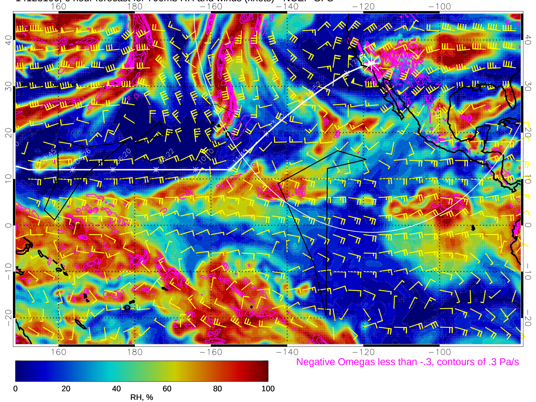
14123106, 6 hour forecast for 700mb RH and winds (knots) - NCEP GFS
