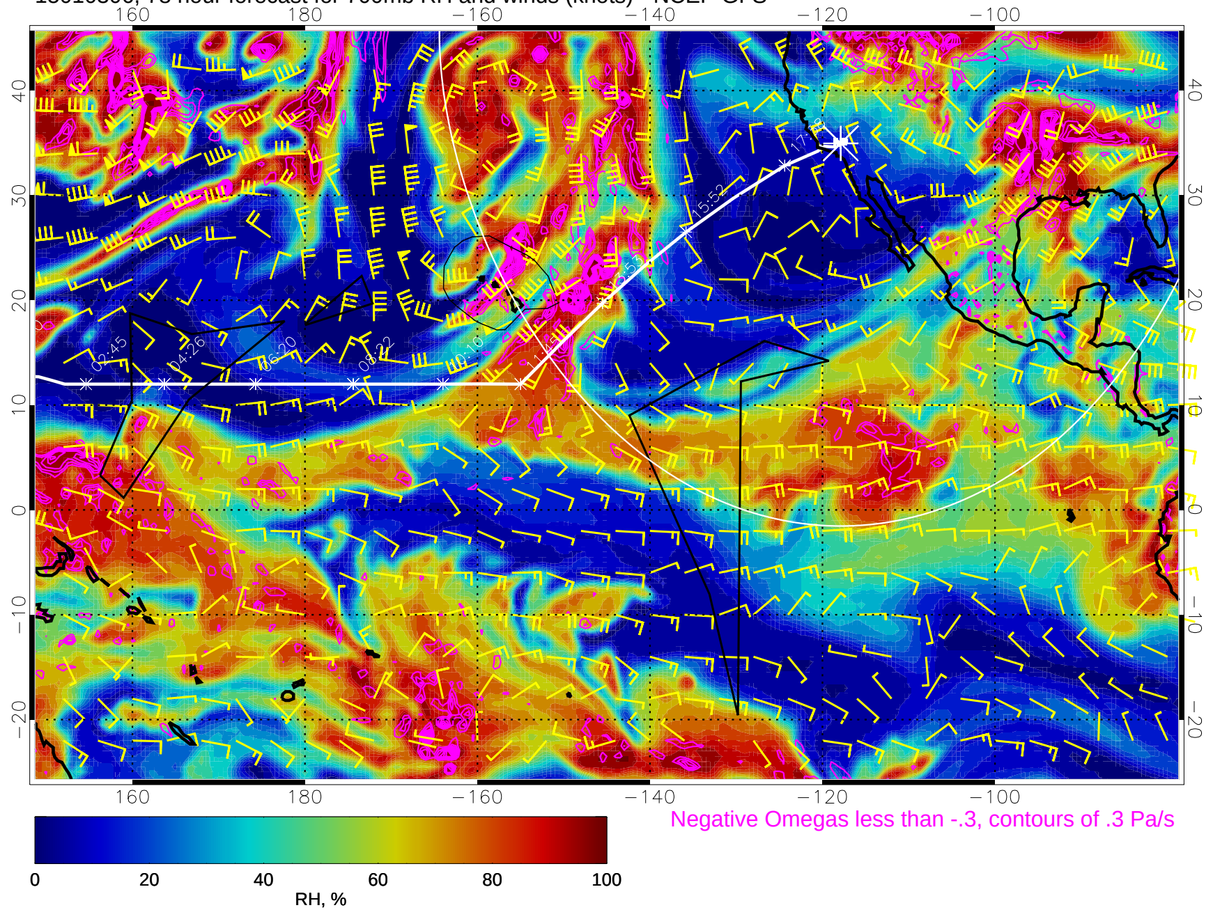
15010306, 78 hour forecast for 700mb RH and winds (knots) - NCEP GFS
