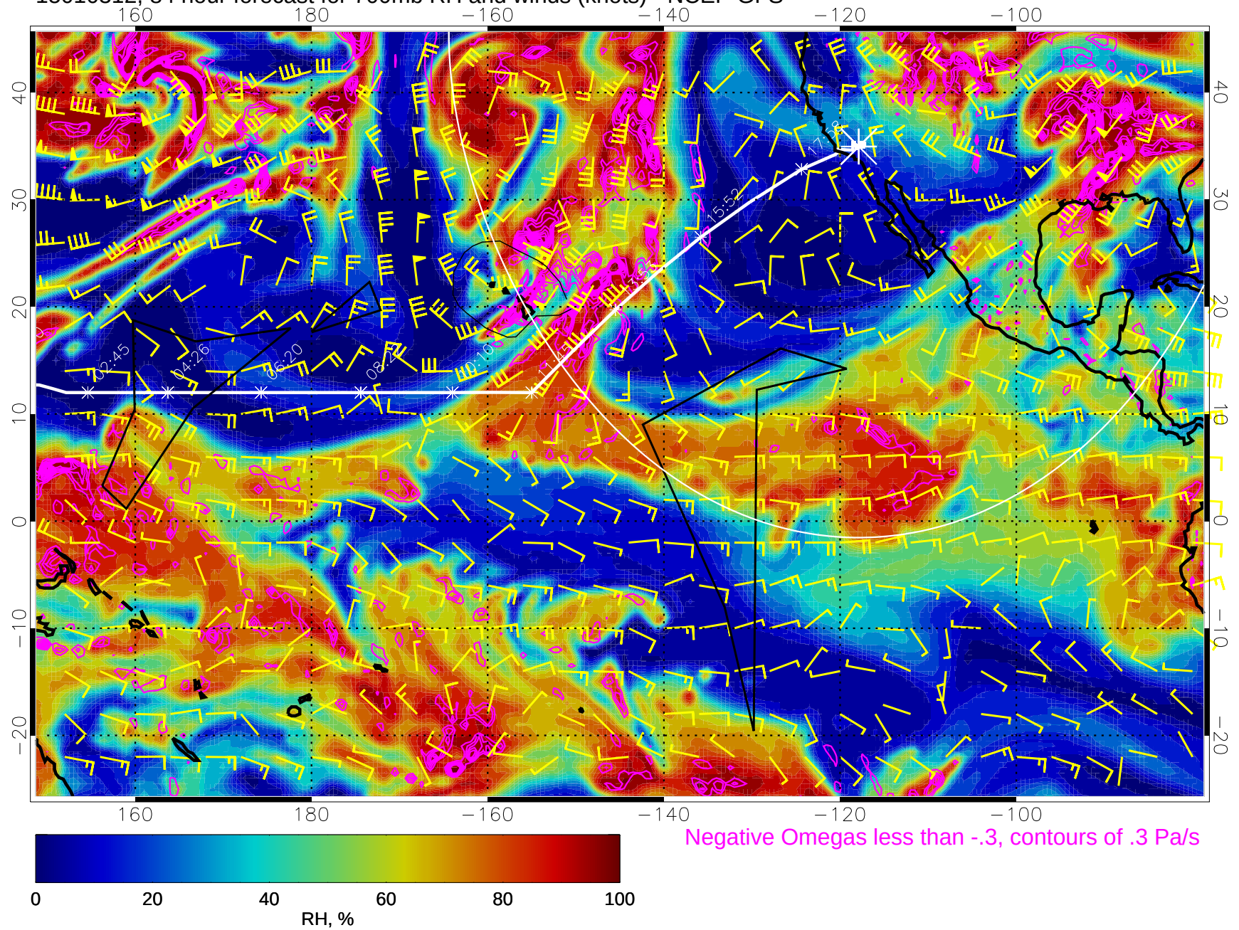
15010312, 84 hour forecast for 700mb RH and winds (knots) - NCEP GFS
