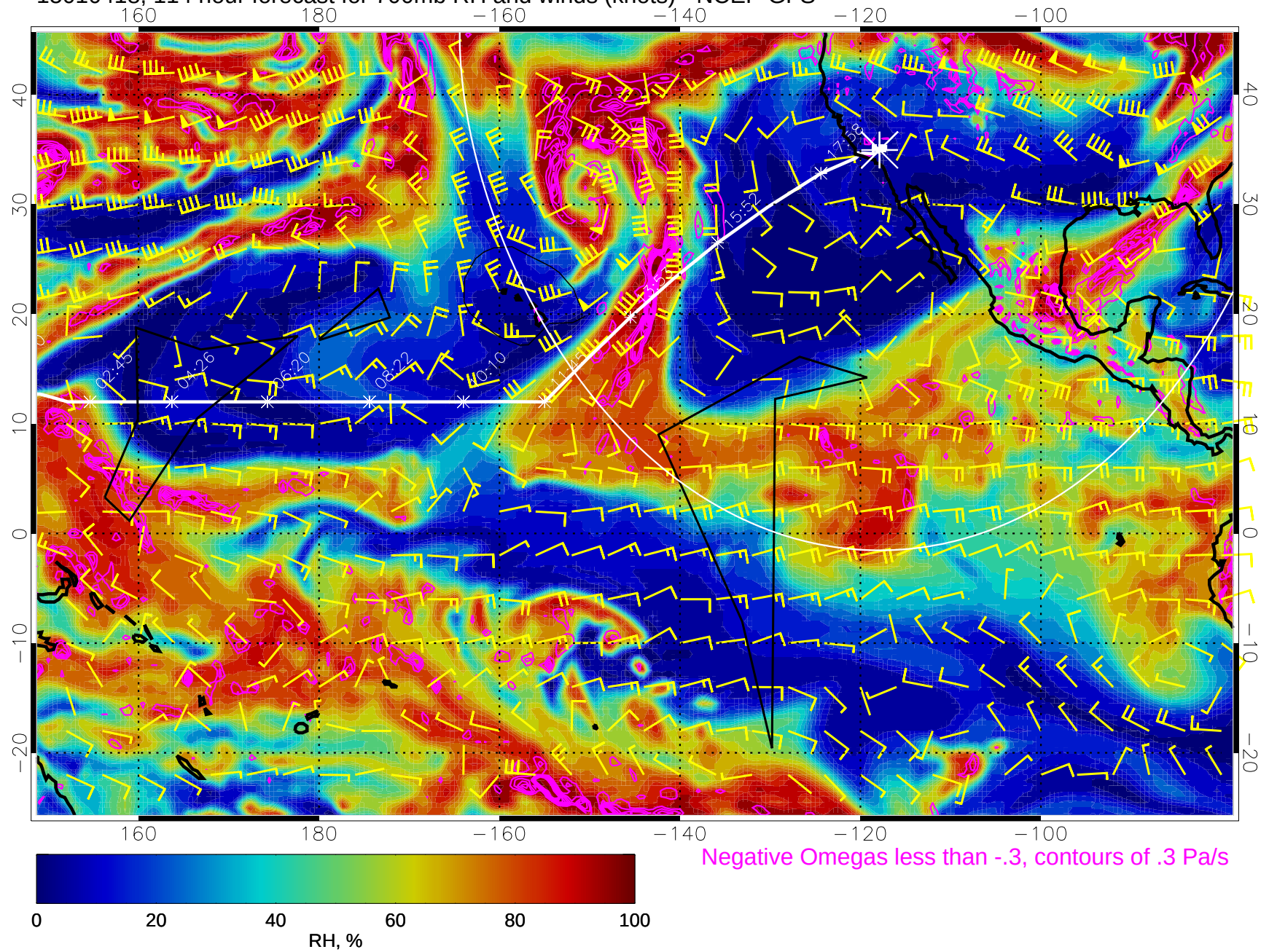
15010418, 114 hour forecast for 700mb RH and winds (knots) - NCEP GFS
