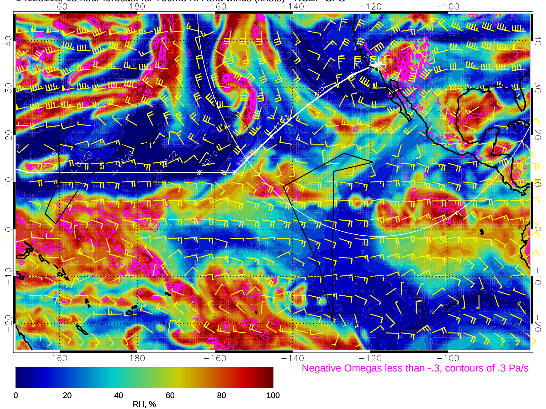
14123118, 18 hour forecast for 700mb RH and winds (knots) - NCEP GFS
