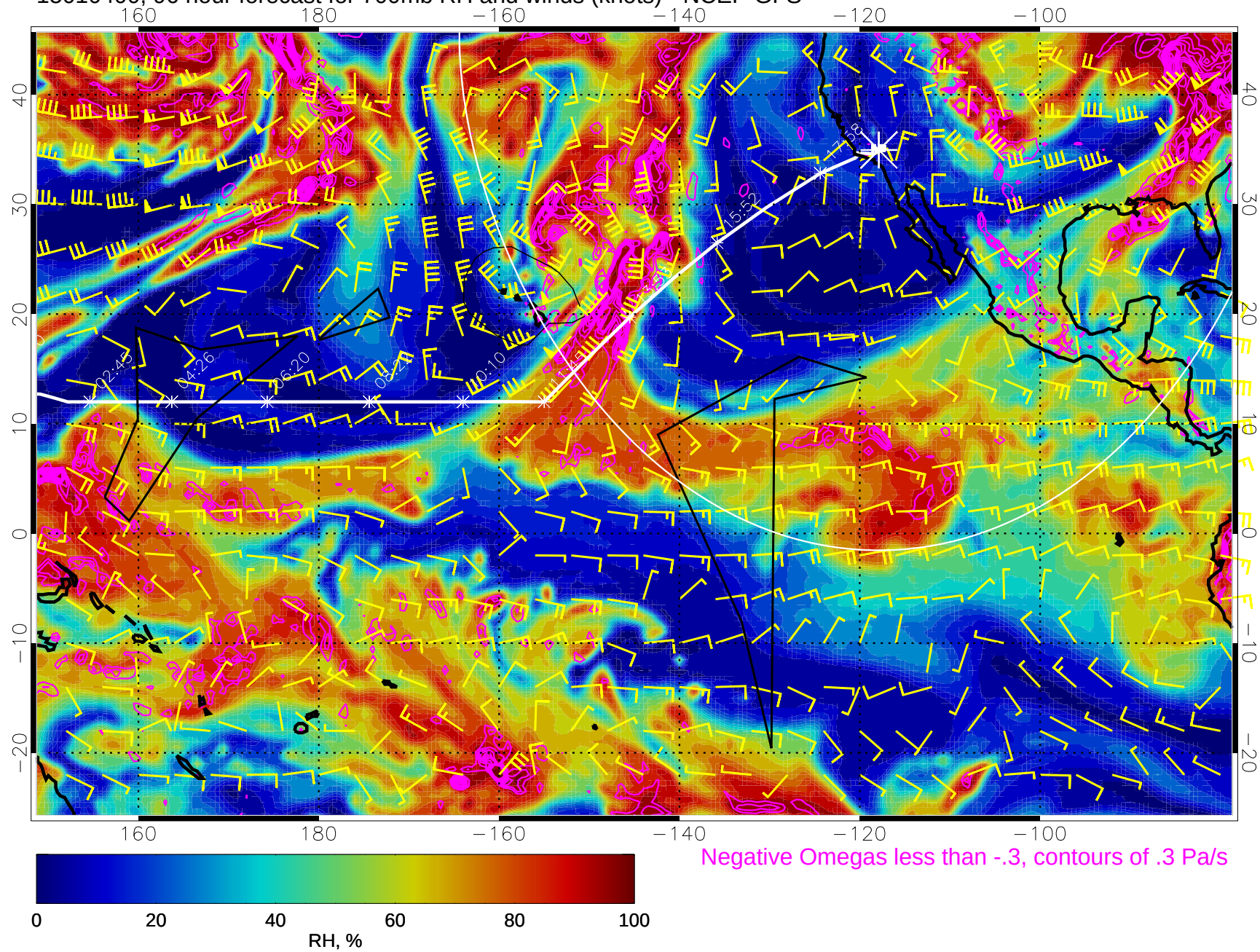
15010400, 96 hour forecast for 700mb RH and winds (knots) - NCEP GFS
