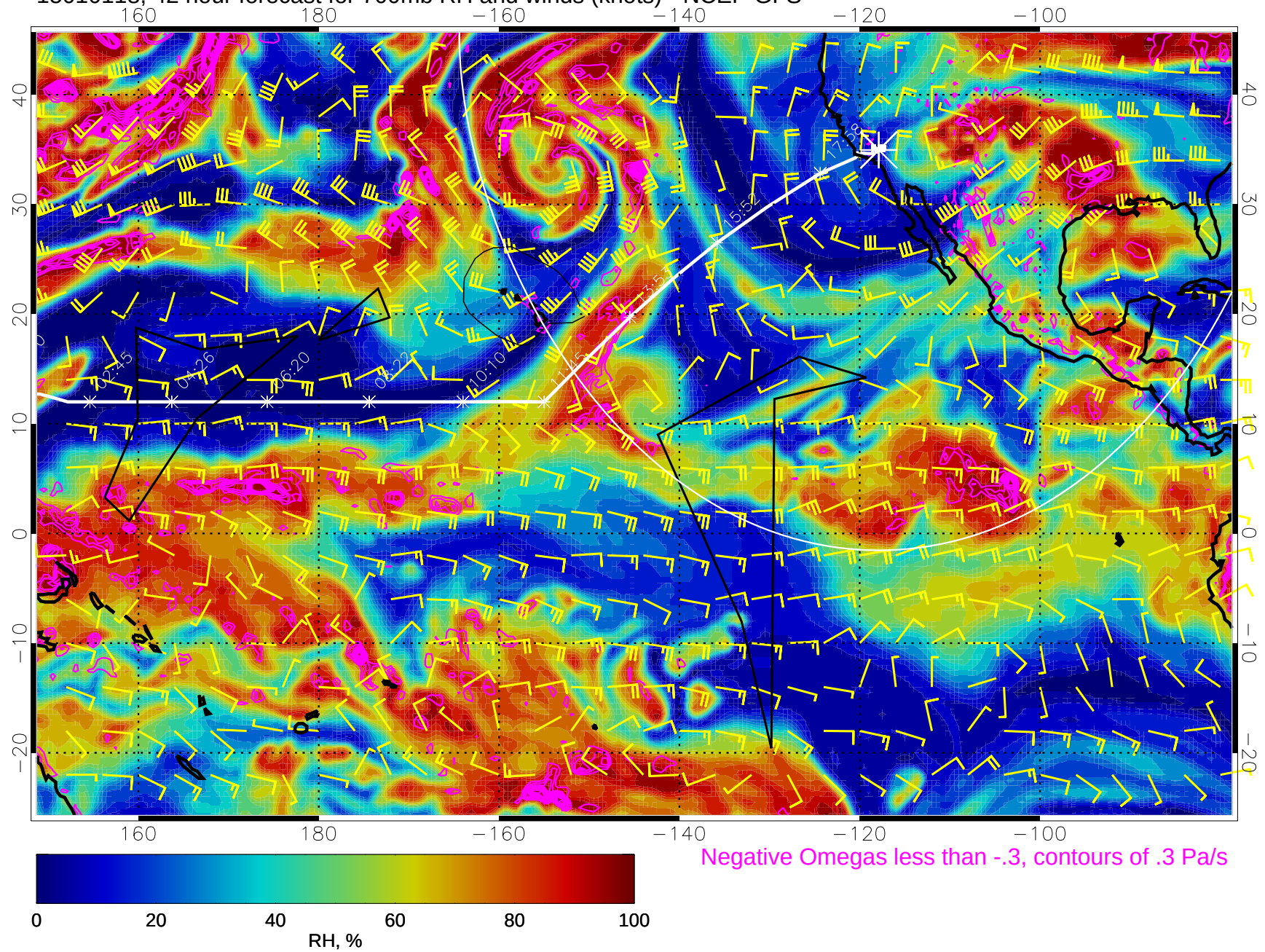
15010118, 42 hour forecast for 700mb RH and winds (knots) - NCEP GFS
