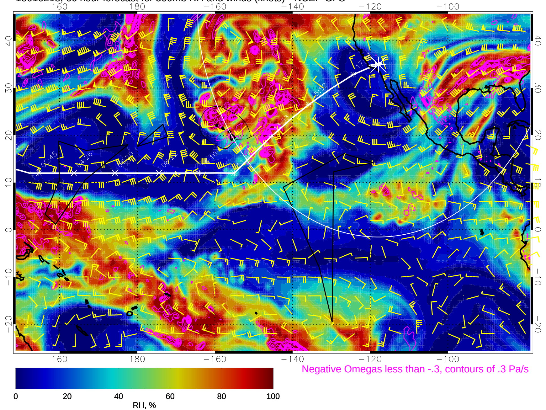
15010218, 66 hour forecast for 500mb RH and winds (knots) - NCEP GFS
