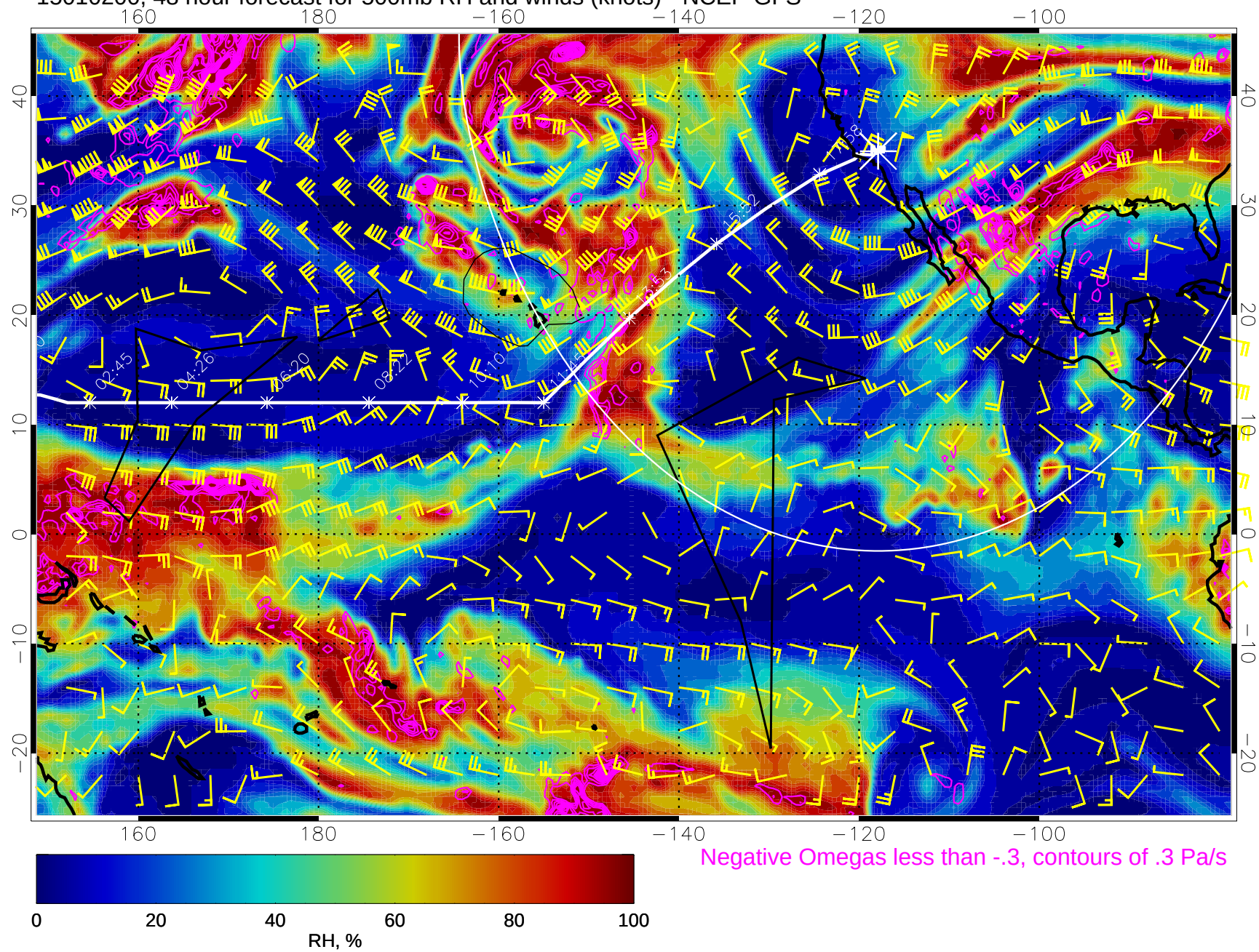
15010200, 48 hour forecast for 500mb RH and winds (knots) - NCEP GFS
