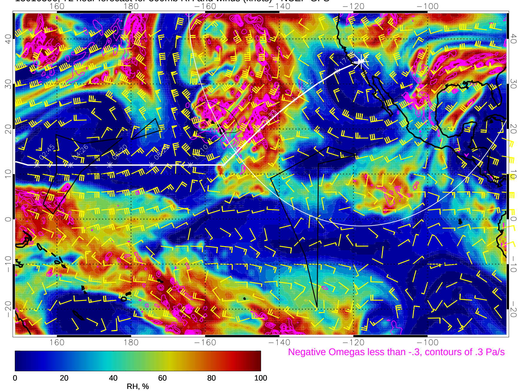
15010300, 72 hour forecast for 500mb RH and winds (knots) - NCEP GFS
