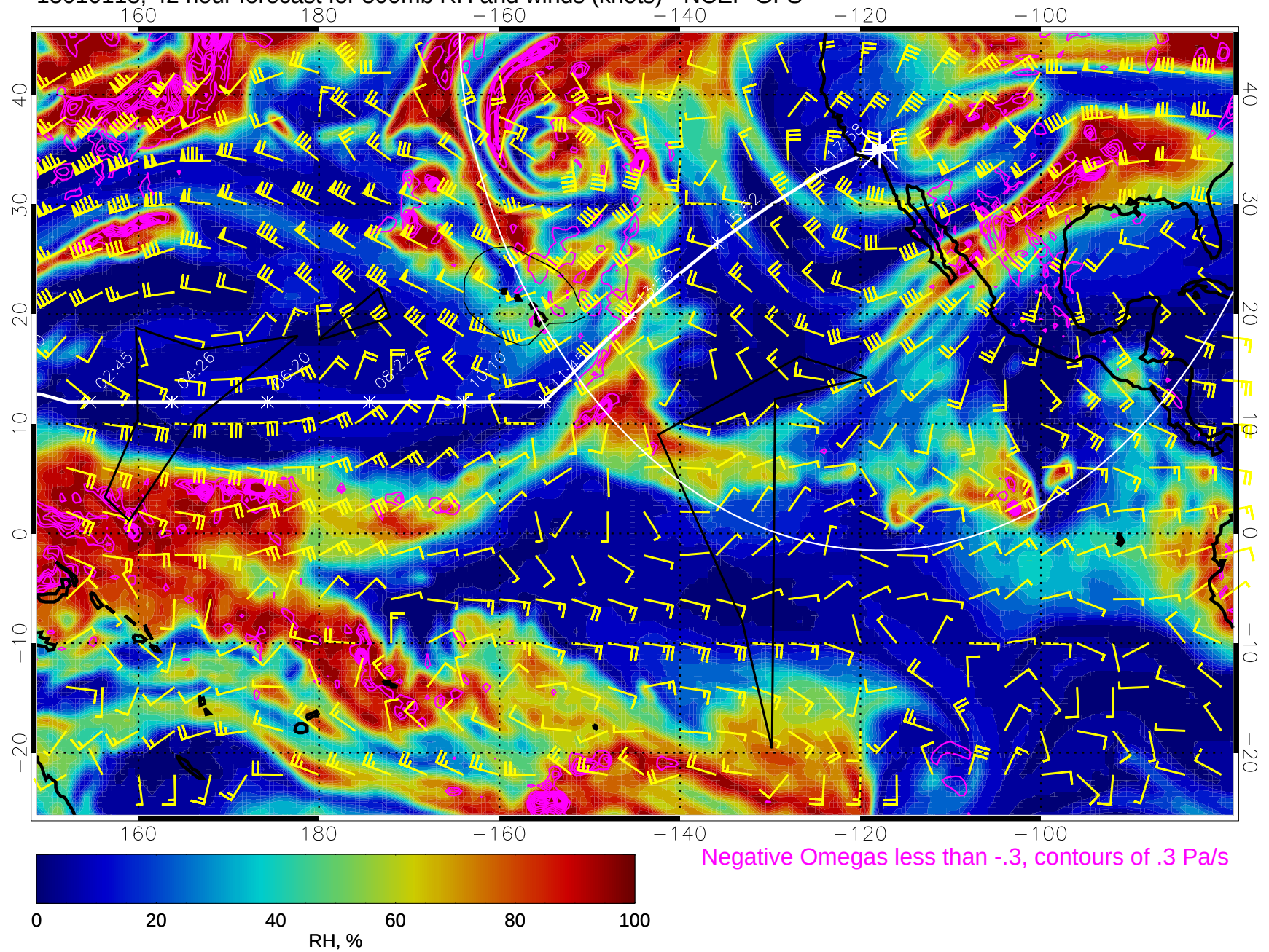
15010118, 42 hour forecast for 500mb RH and winds (knots) - NCEP GFS
