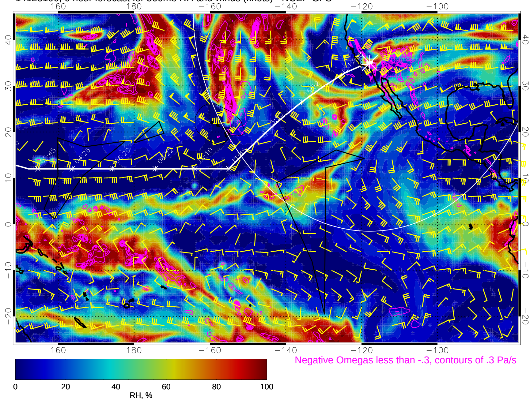
14123106, 6 hour forecast for 500mb RH and winds (knots) - NCEP GFS
