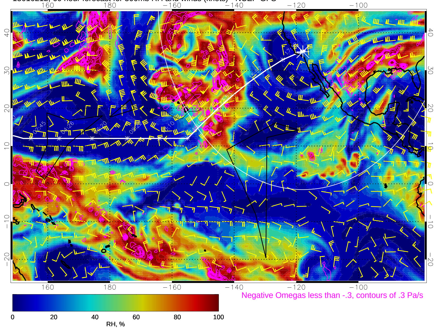
15010212, 60 hour forecast for 500mb RH and winds (knots) - NCEP GFS
