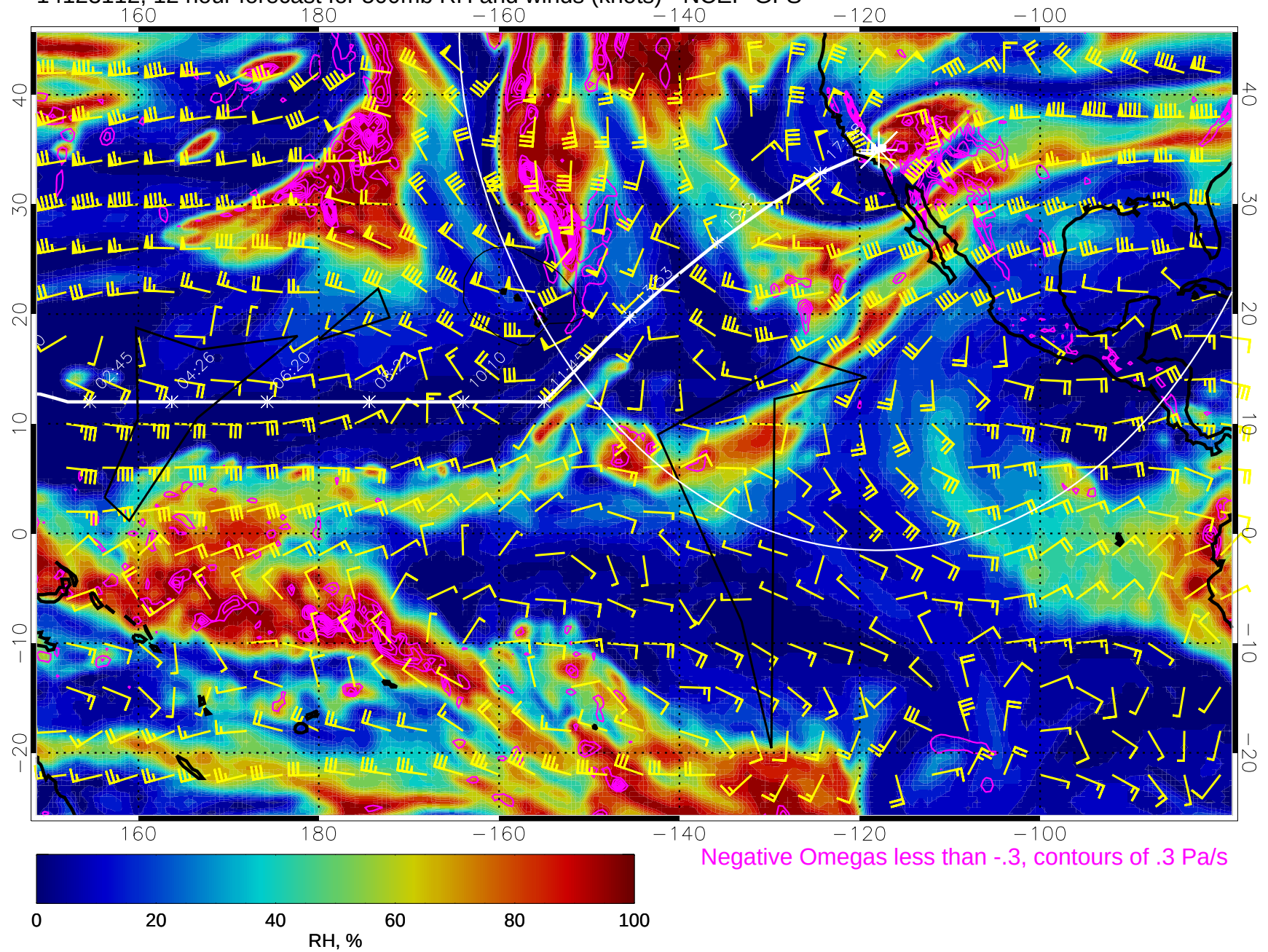
14123112, 12 hour forecast for 500mb RH and winds (knots) - NCEP GFS
