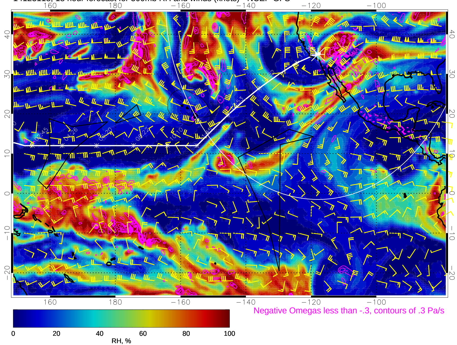
14123118, 18 hour forecast for 500mb RH and winds (knots) - NCEP GFS
