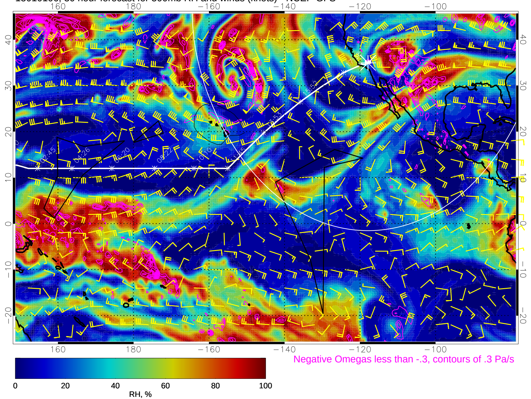
15010106, 30 hour forecast for 500mb RH and winds (knots) - NCEP GFS
