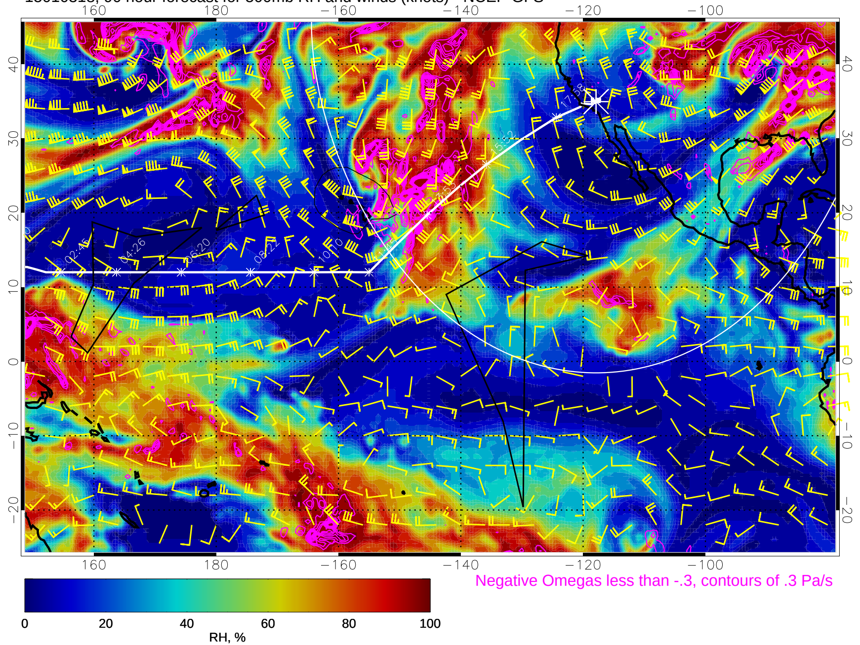
15010318, 90 hour forecast for 500mb RH and winds (knots) - NCEP GFS
