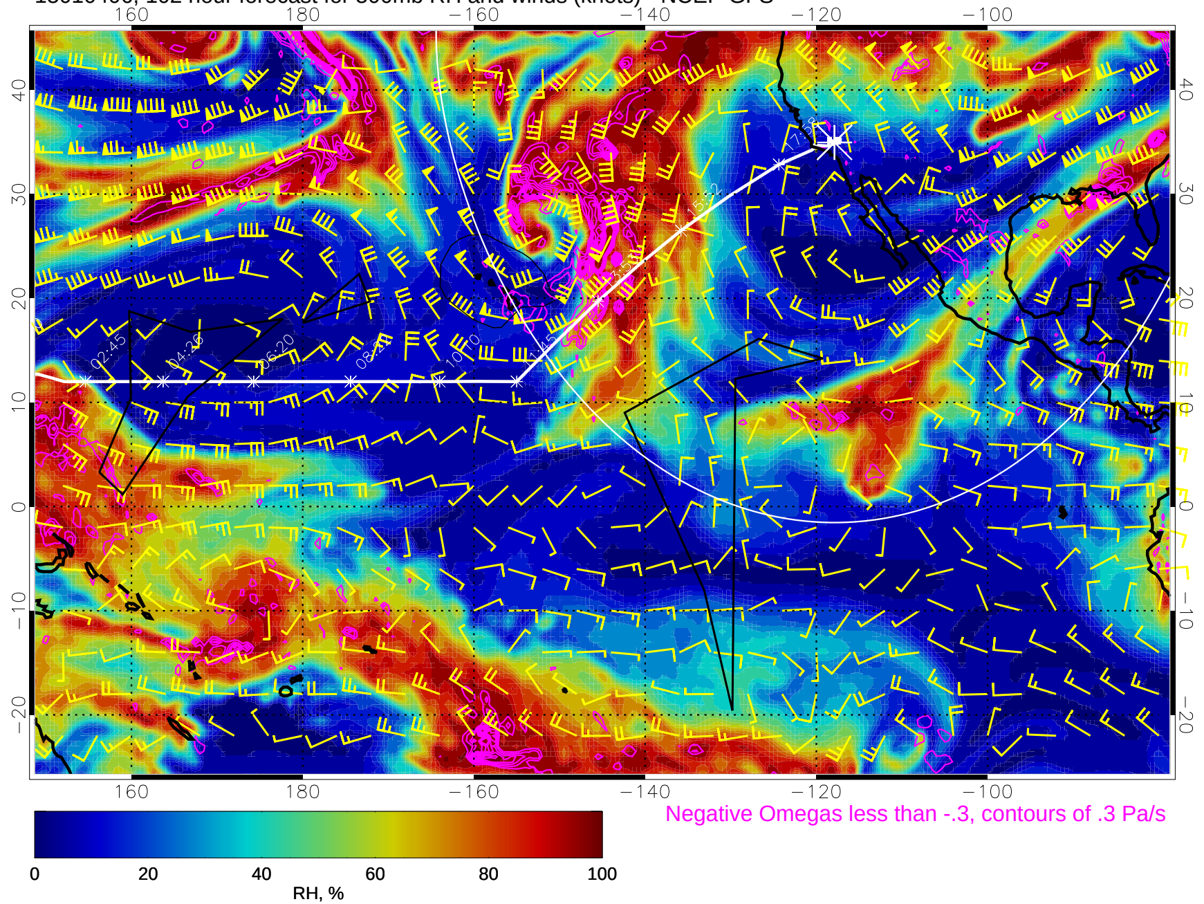
15010406, 102 hour forecast for 500mb RH and winds (knots) - NCEP GFS
