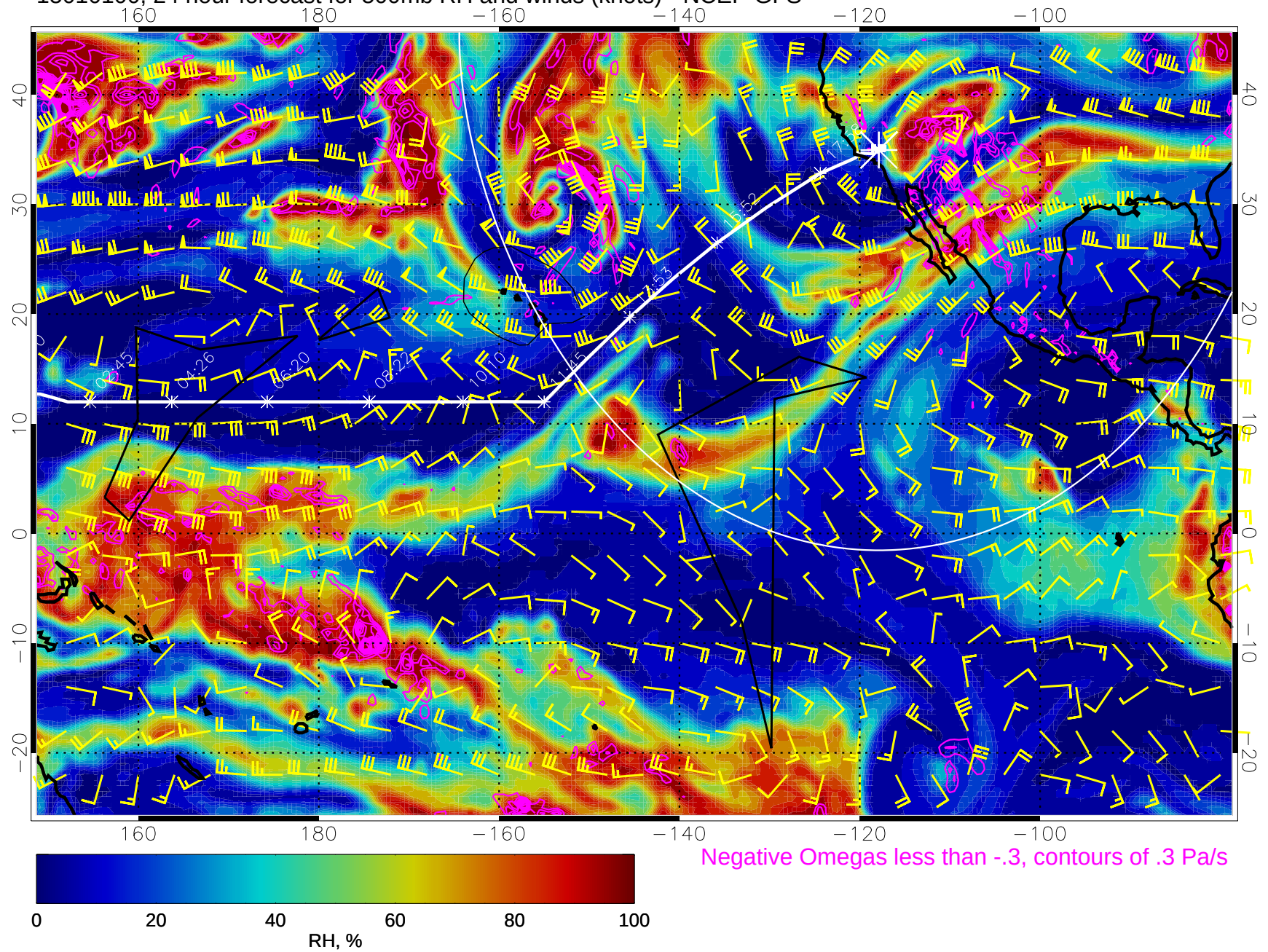
15010100, 24 hour forecast for 500mb RH and winds (knots) - NCEP GFS
