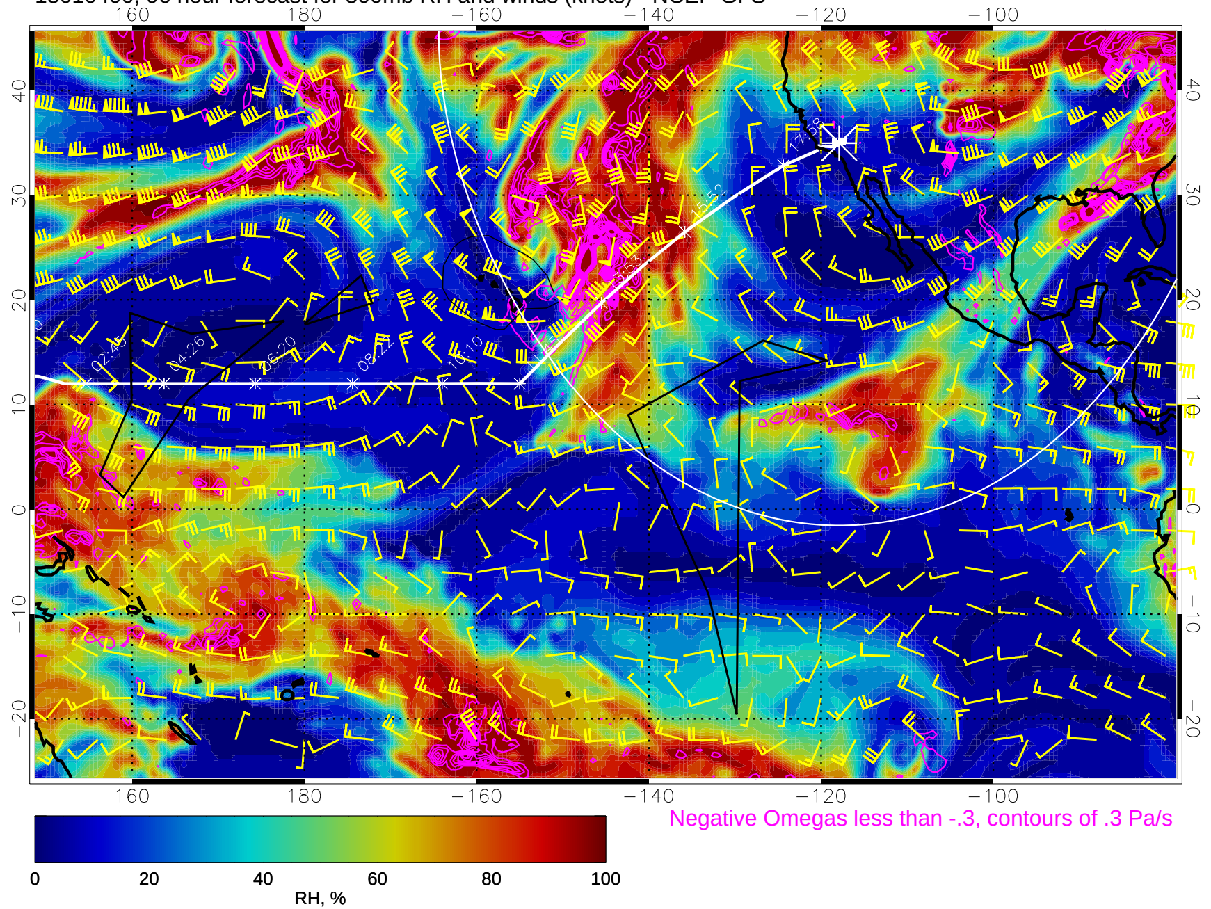
15010400, 96 hour forecast for 500mb RH and winds (knots) - NCEP GFS
