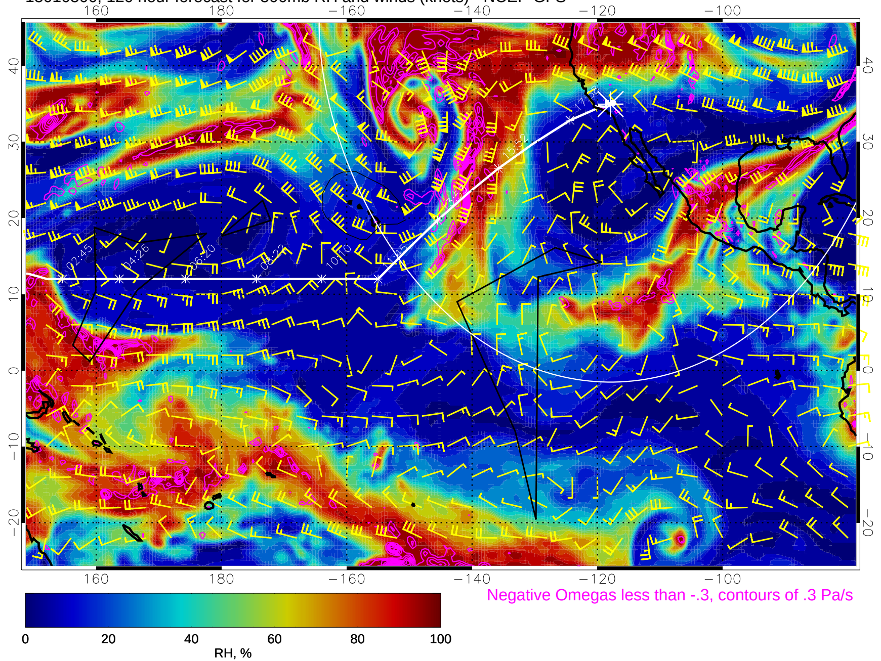
15010500, 120 hour forecast for 500mb RH and winds (knots) - NCEP GFS
