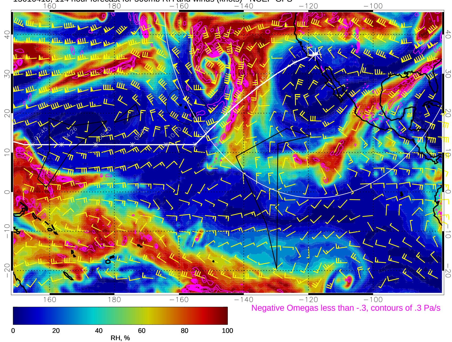
15010418, 114 hour forecast for 500mb RH and winds (knots) - NCEP GFS
