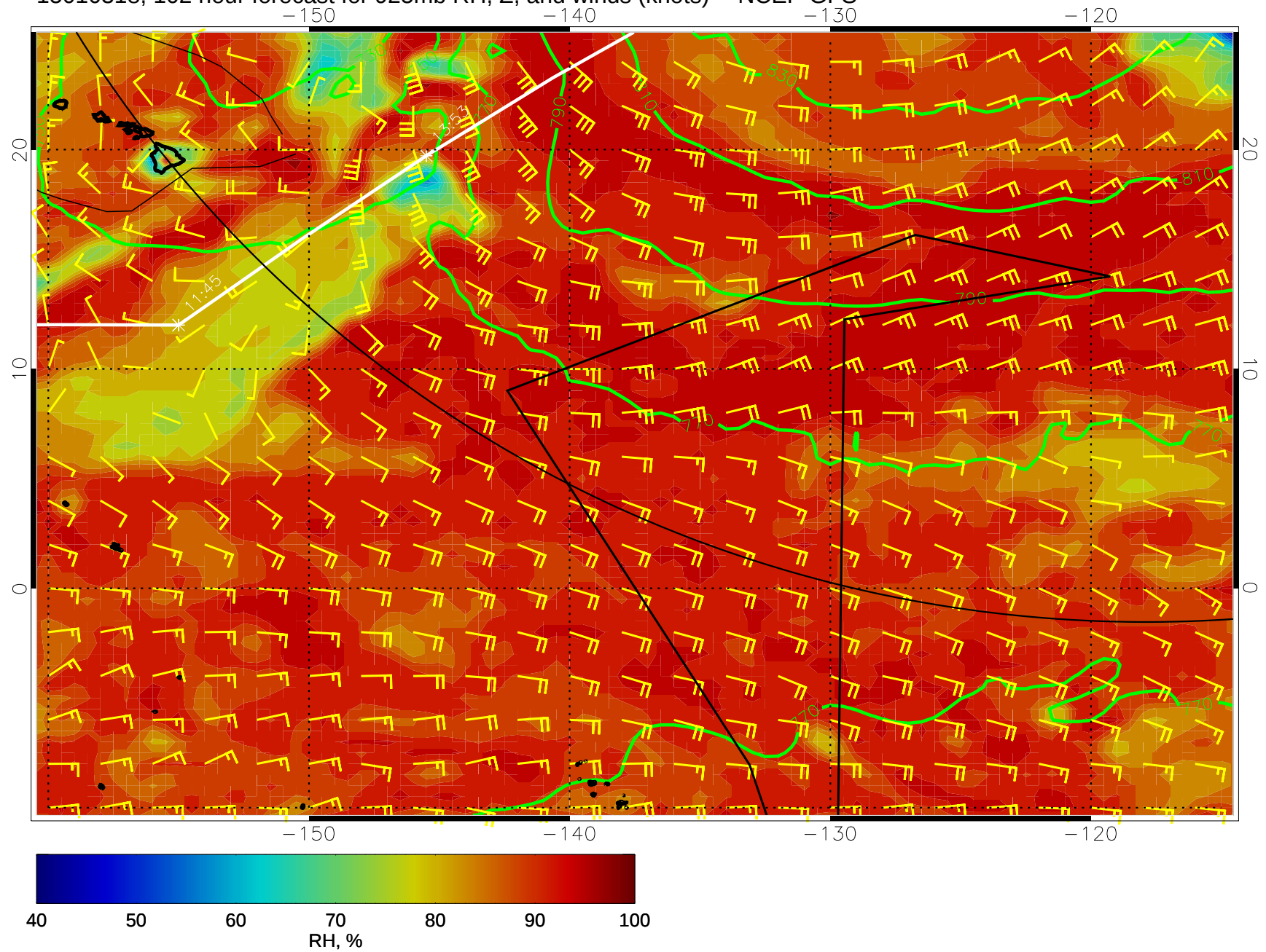
15010318, 102 hour forecast for 925mb RH, Z, and winds (knots) -- NCEP GFS
