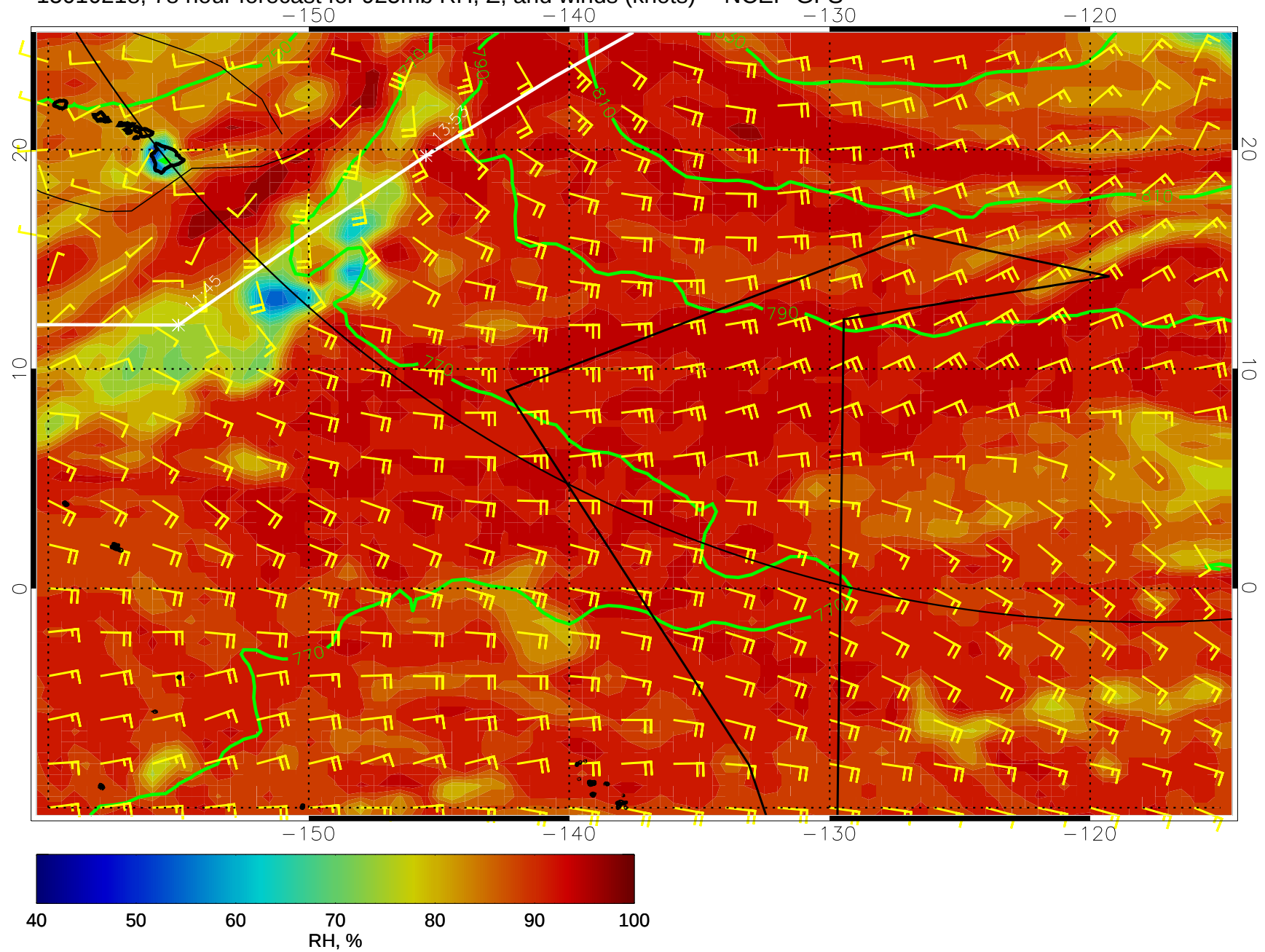
15010218, 78 hour forecast for 925mb RH, Z, and winds (knots) -- NCEP GFS
