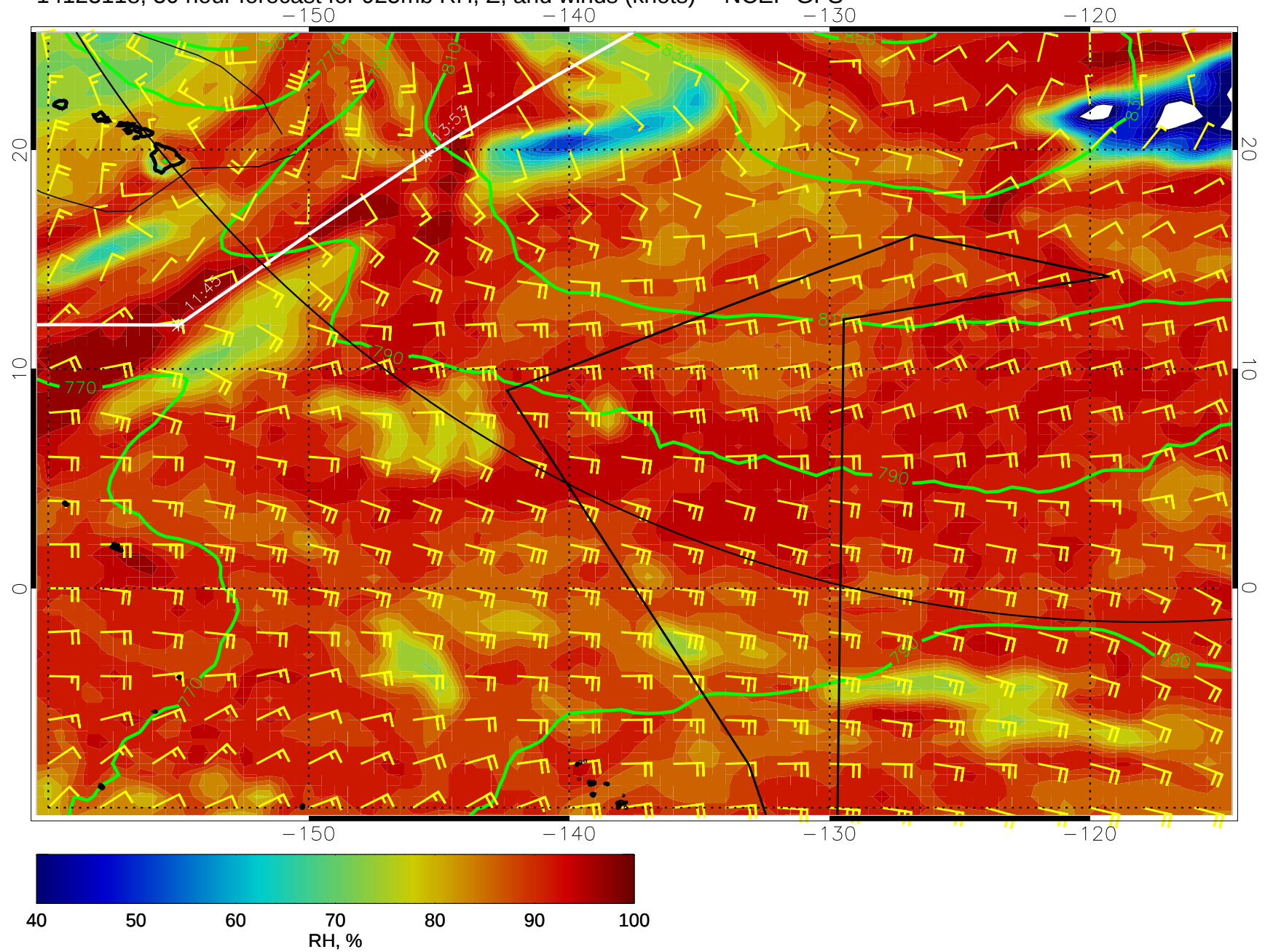
14123118, 30 hour forecast for 925mb RH, Z, and winds (knots) -- NCEP GFS
