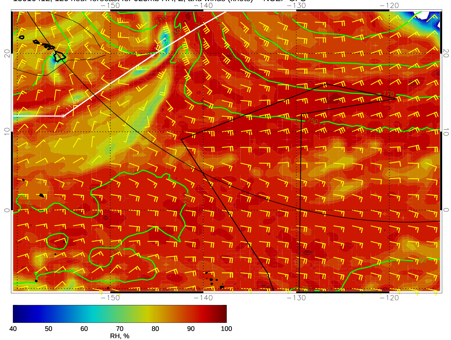
15010412, 120 hour forecast for 925mb RH, Z, and winds (knots) -- NCEP GFS
