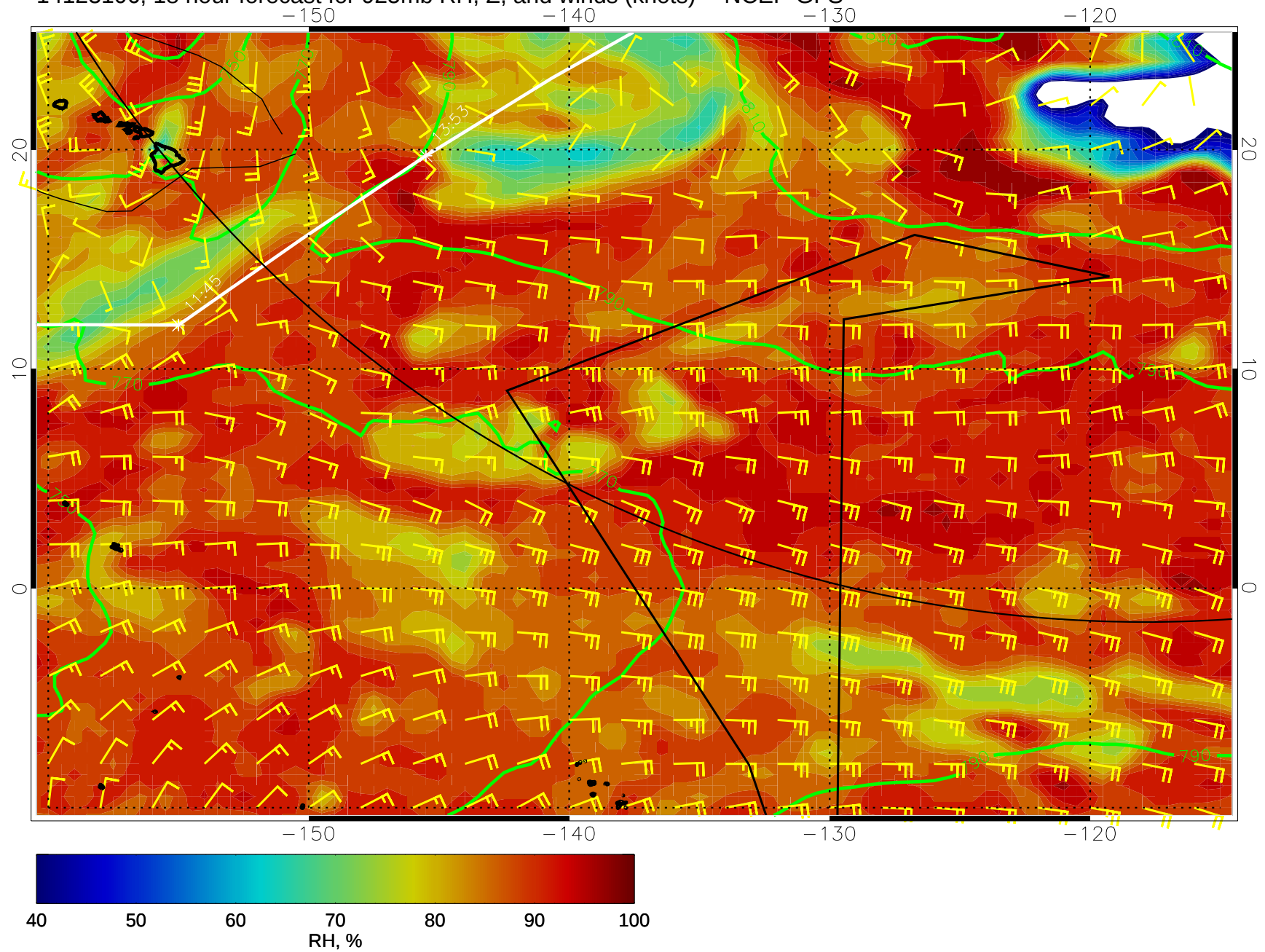
14123106, 18 hour forecast for 925mb RH, Z, and winds (knots) -- NCEP GFS
