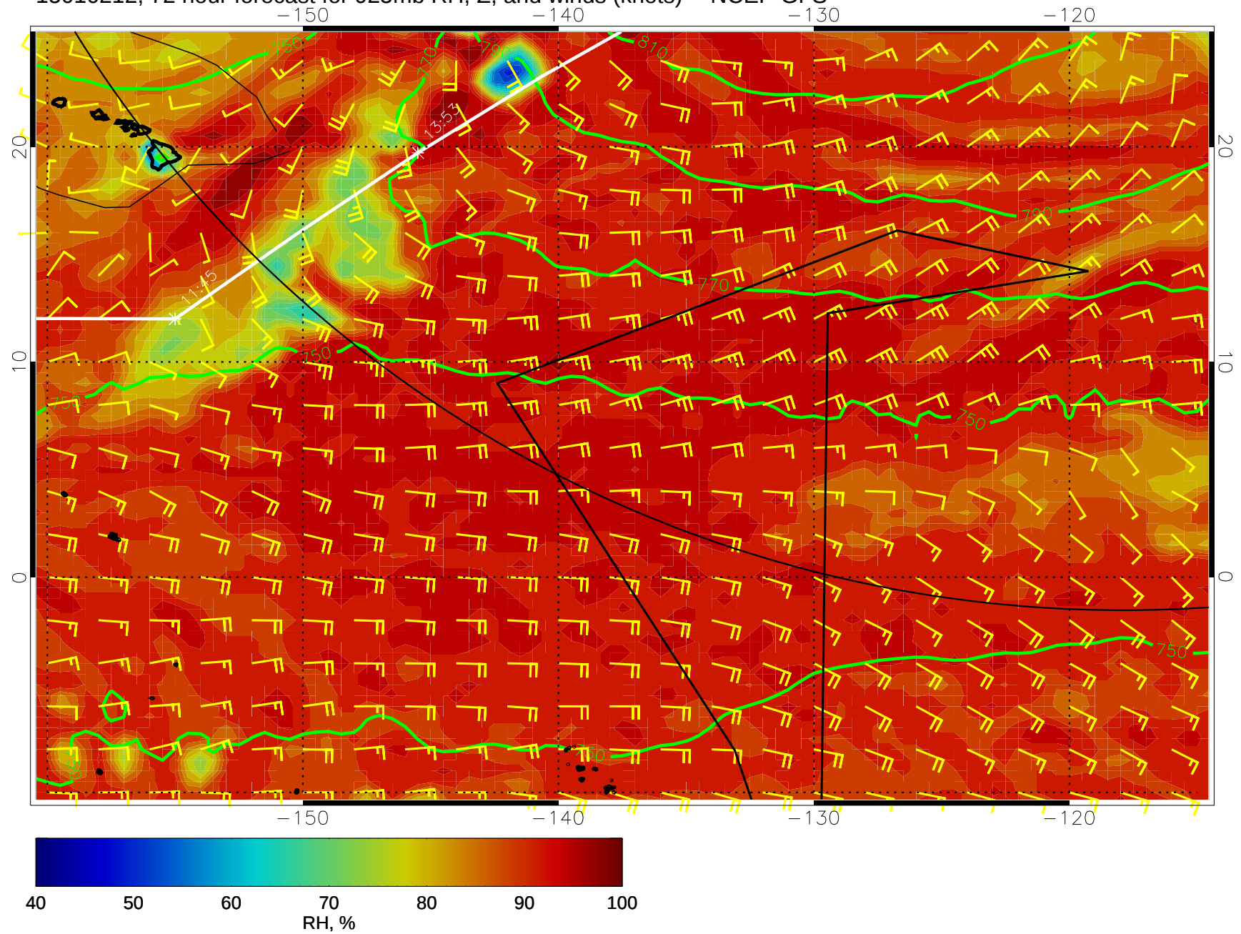
15010212, 72 hour forecast for 925mb RH, Z, and winds (knots) -- NCEP GFS
