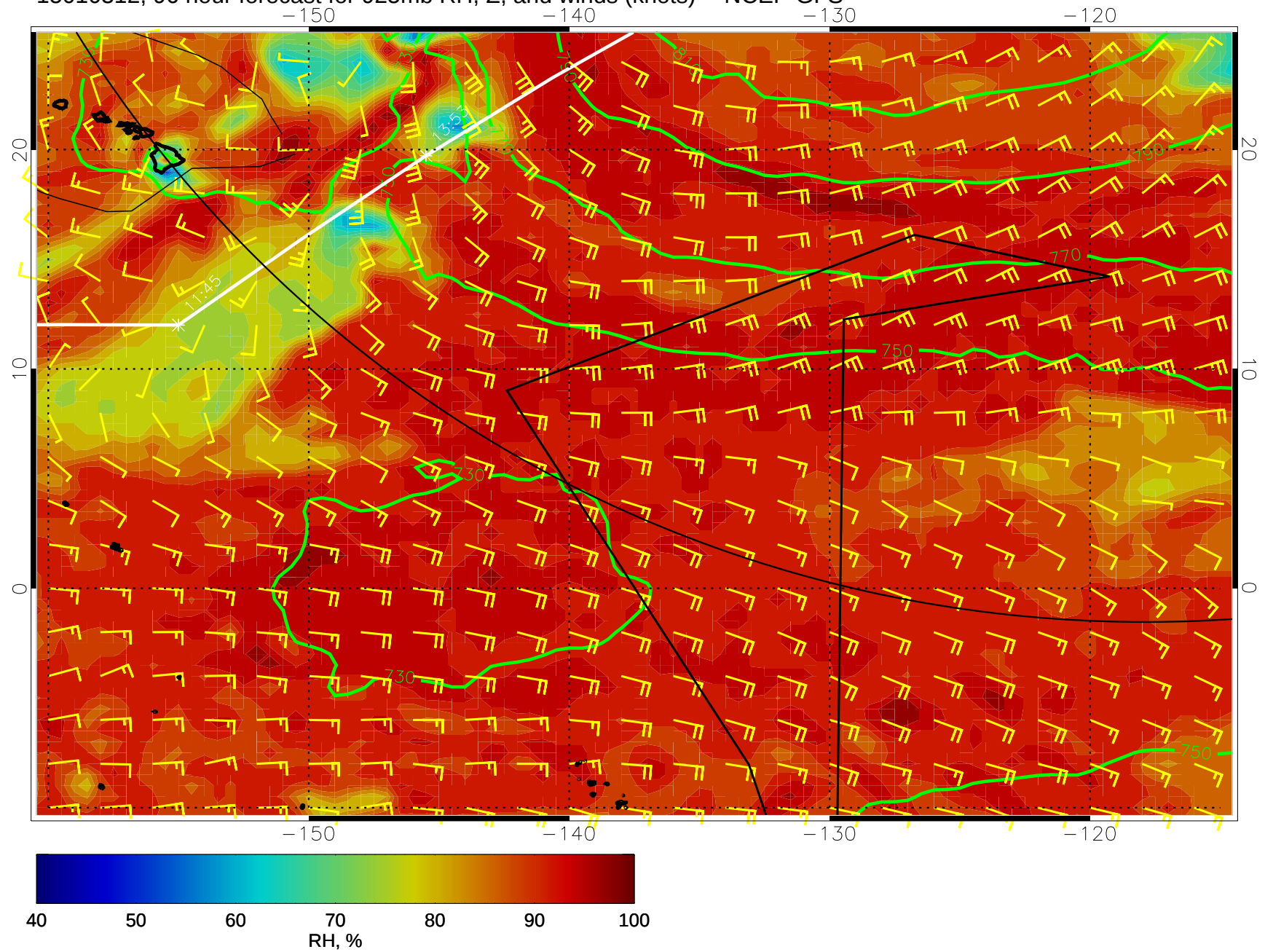
15010312, 96 hour forecast for 925mb RH, Z, and winds (knots) -- NCEP GFS
