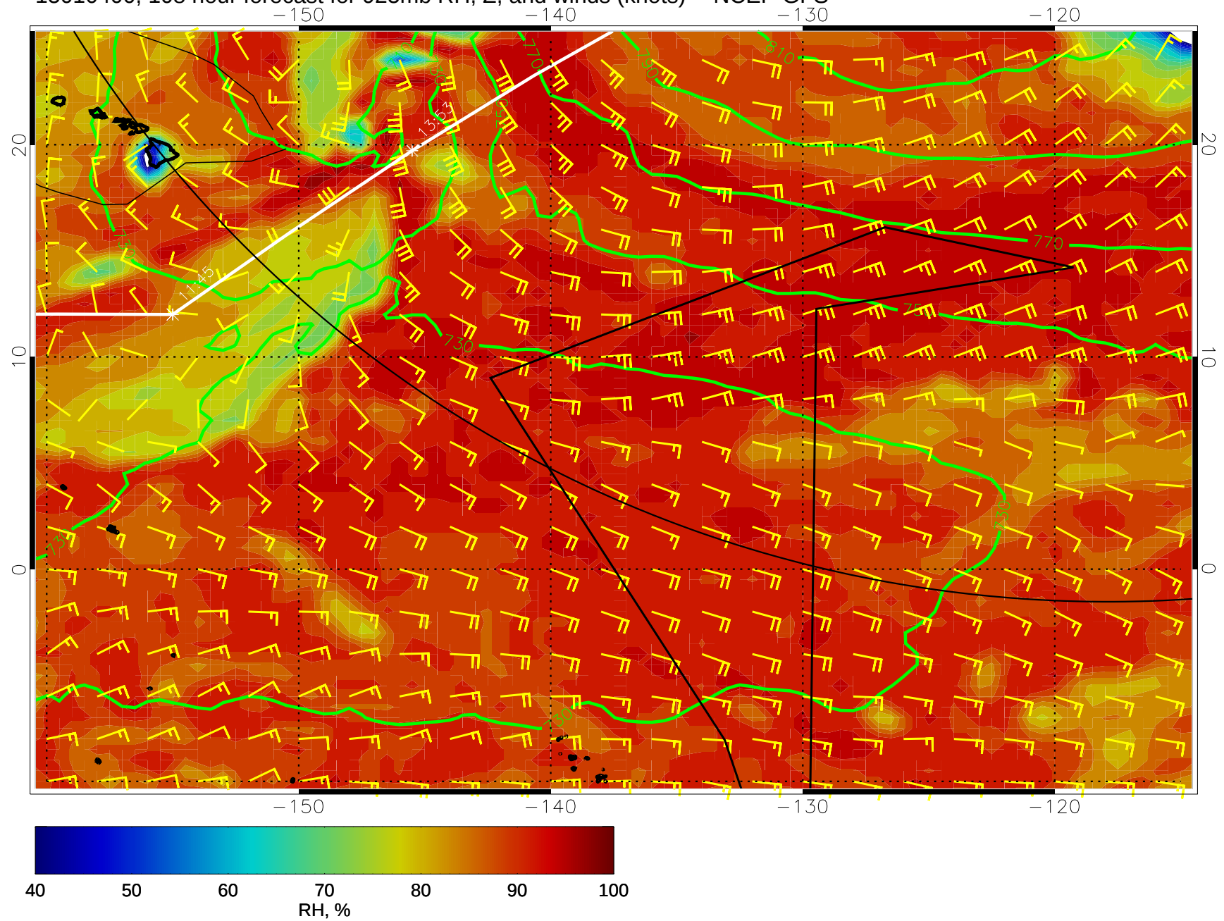
15010400, 108 hour forecast for 925mb RH, Z, and winds (knots) -- NCEP GFS
