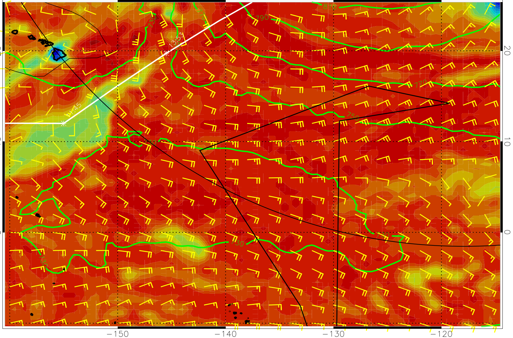
20020000, 5 yr. lead, forecast for: storms (in), \pm , and winds (knots) 2002 2003 2004 2005 -150 -140 -130 -120
