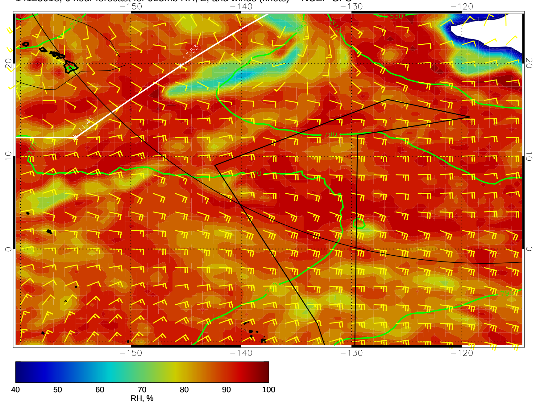
14123018, 6 hour forecast for 925mb RH, Z, and winds (knots) -- NCEP GFS
