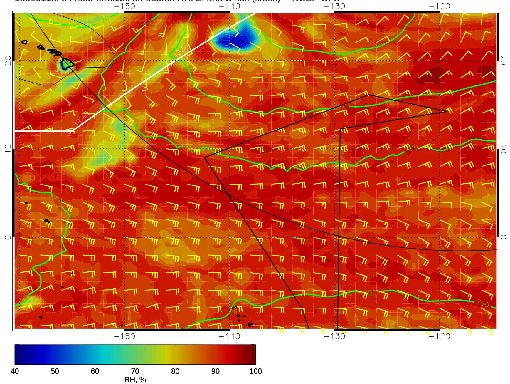
15010118, 54 hour forecast for 925mb RH, Z, and winds (knots) -- NCEP GFS
