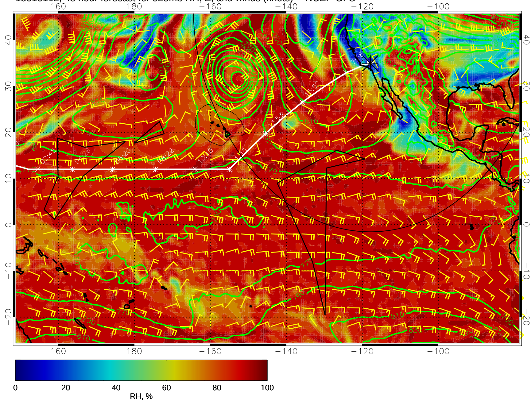
15010112, 48 hour forecast for 925mb RH, Z, and winds (knots) -- NCEP GFS
