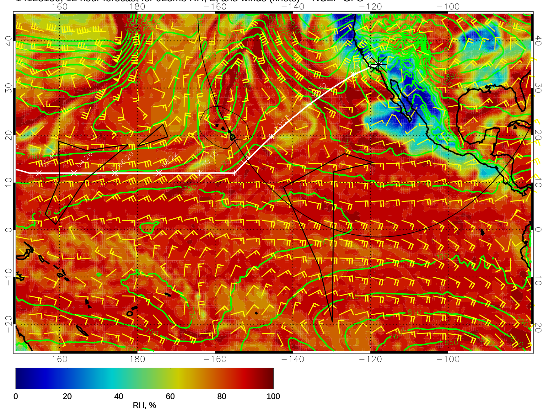
14123100, 12 hour forecast for 925mb RH, Z, and winds (knots) -- NCEP GFS
