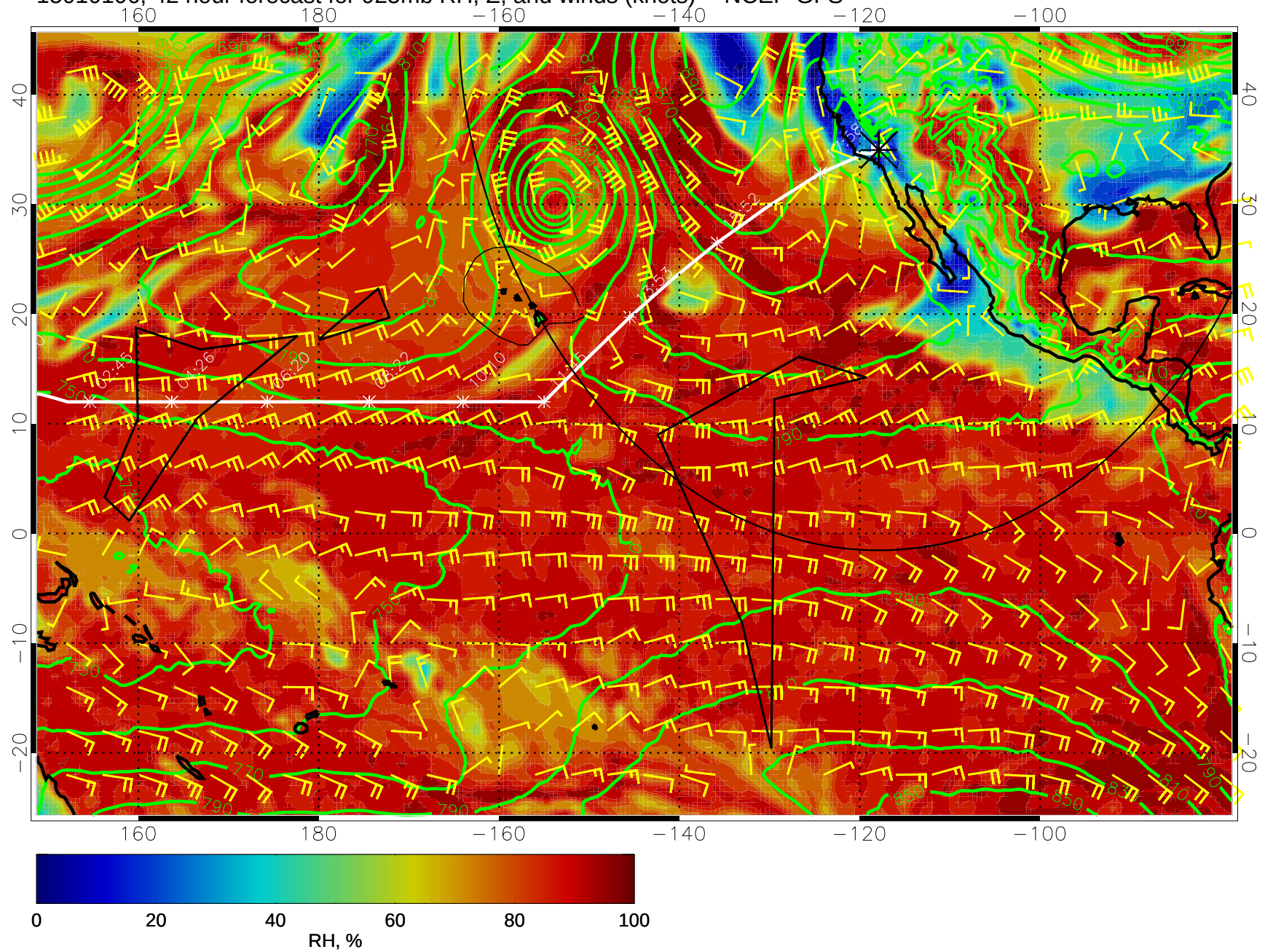
15010106, 42 hour forecast for 925mb RH, Z, and winds (knots) -- NCEP GFS
