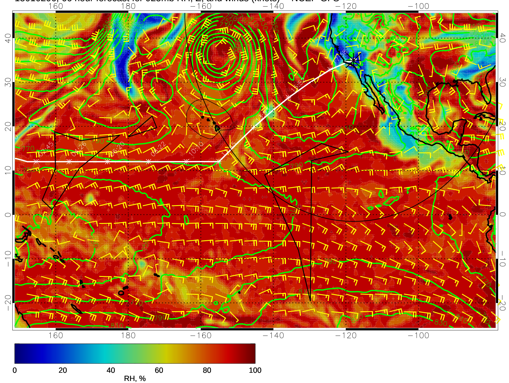
15010206, 66 hour forecast for 925mb RH, Z, and winds (knots) -- NCEP GFS
