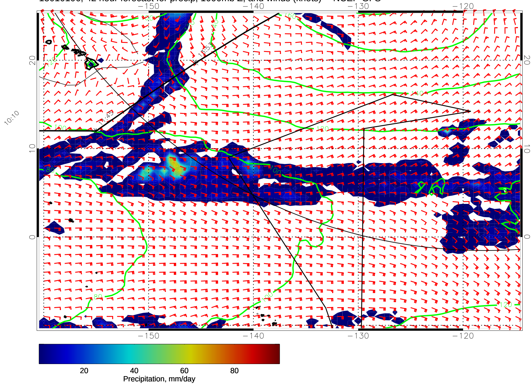
15010106, 42 hour forecast for precip, 1000mb Z, and winds (knots) -- NCEP GFS
