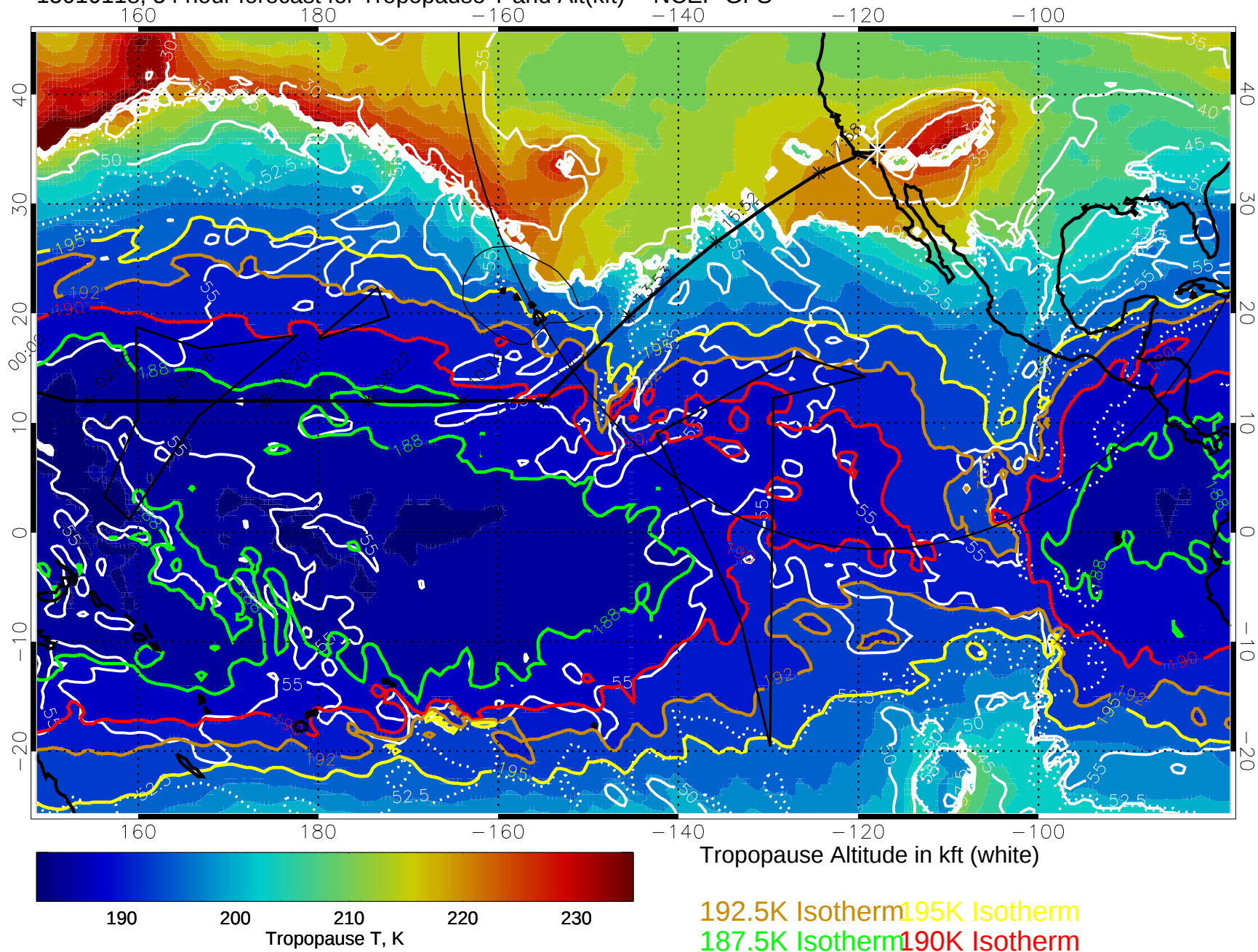
15010118, 54 hour forecast for Tropopause T and Alt(kft) -- NCEP GFS
