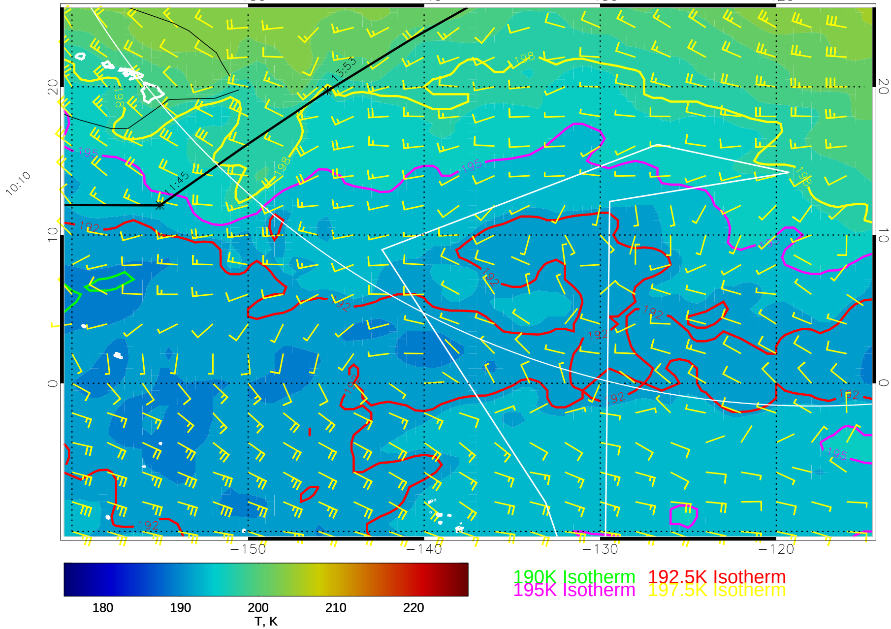
15010118, 54 hour forecast for 70mb T and winds (knots) -- NCEP GFS
