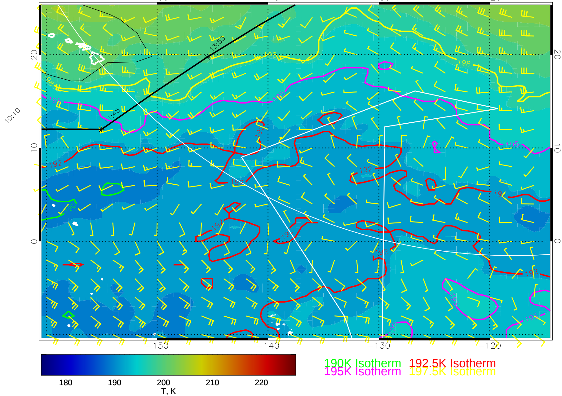
15010112, 48 hour forecast for 70mb T and winds (knots) -- NCEP GFS
