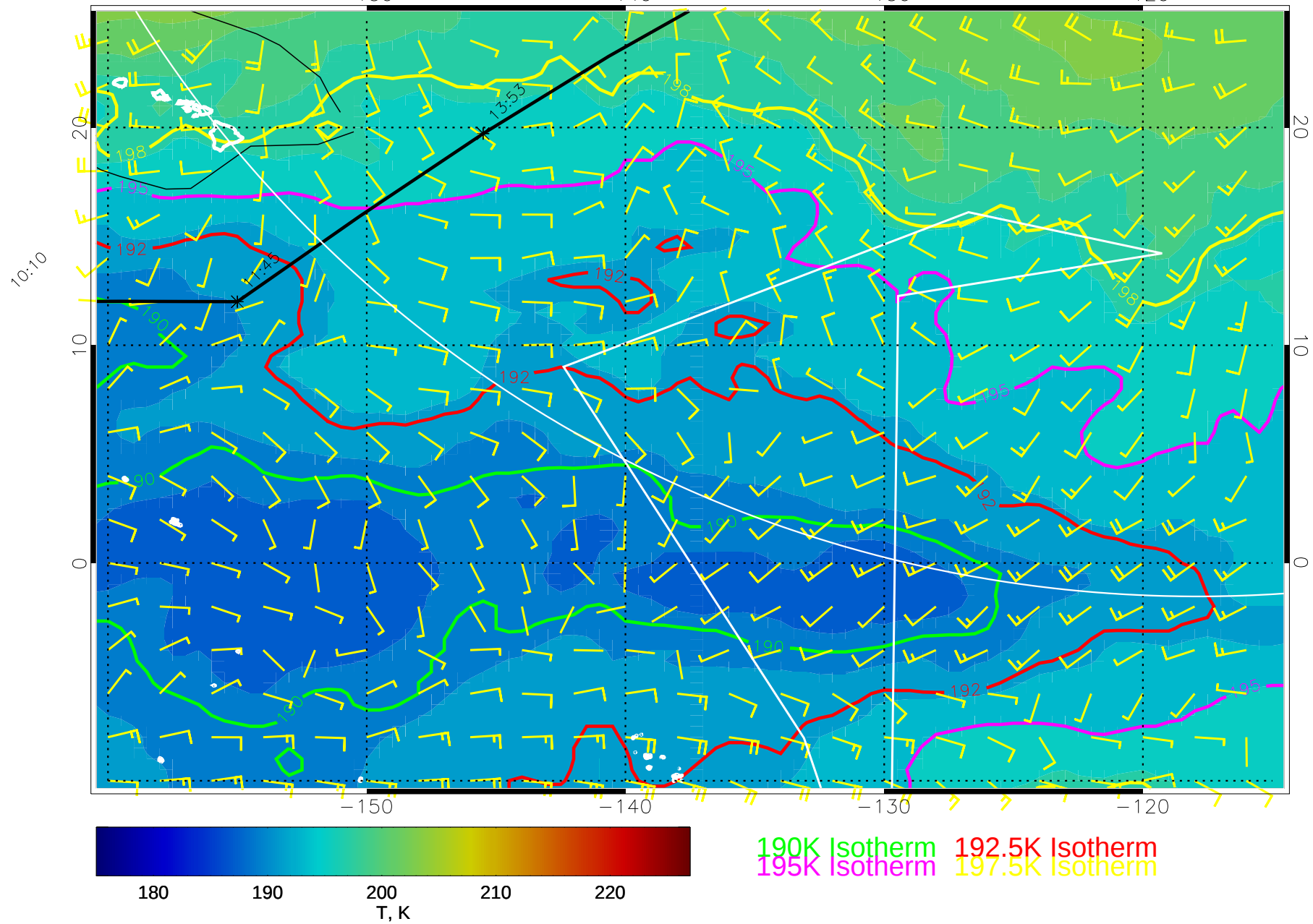
14123100, 12 hour forecast for 70mb T and winds (knots) -- NCEP GFS
