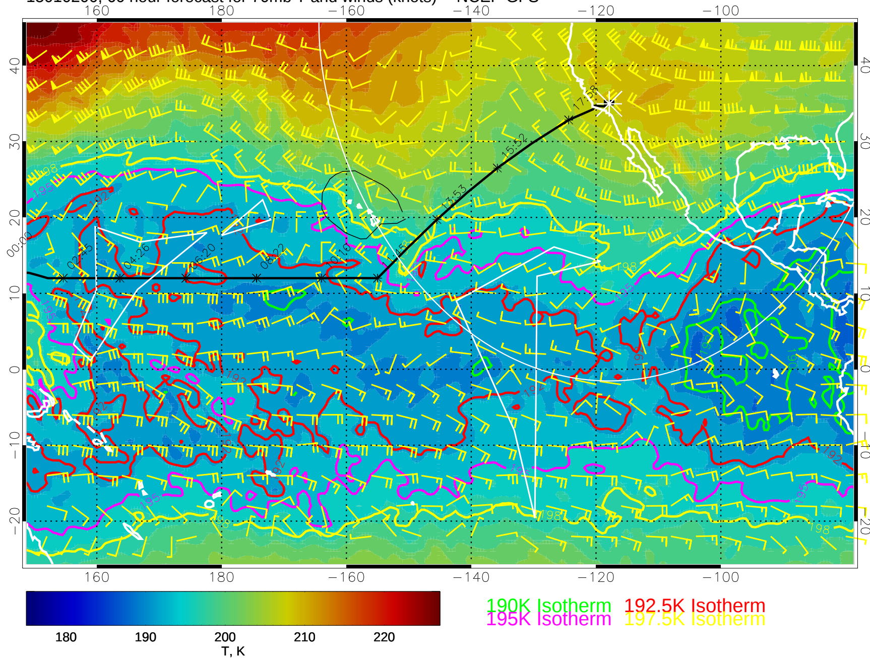
15010200, 60 hour forecast for 70mb T and winds (knots) -- NCEP GFS
