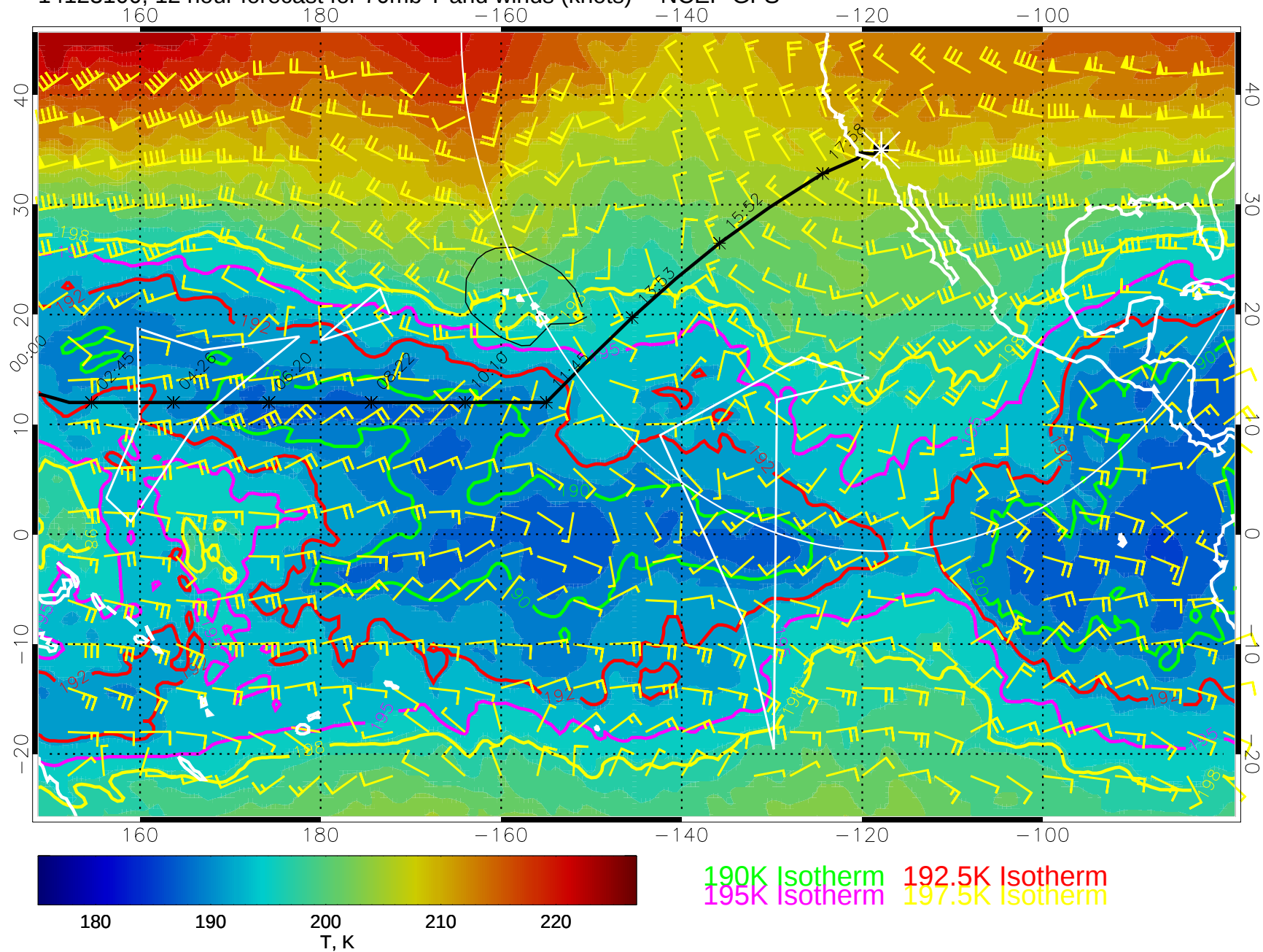
14123100, 12 hour forecast for 70mb T and winds (knots) -- NCEP GFS
