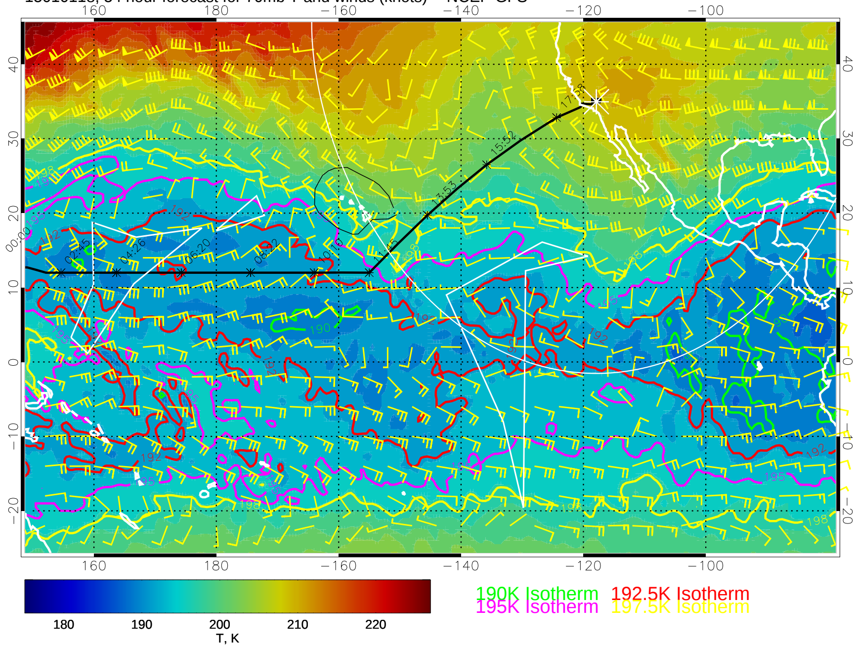
15010118, 54 hour forecast for 70mb T and winds (knots) -- NCEP GFS
