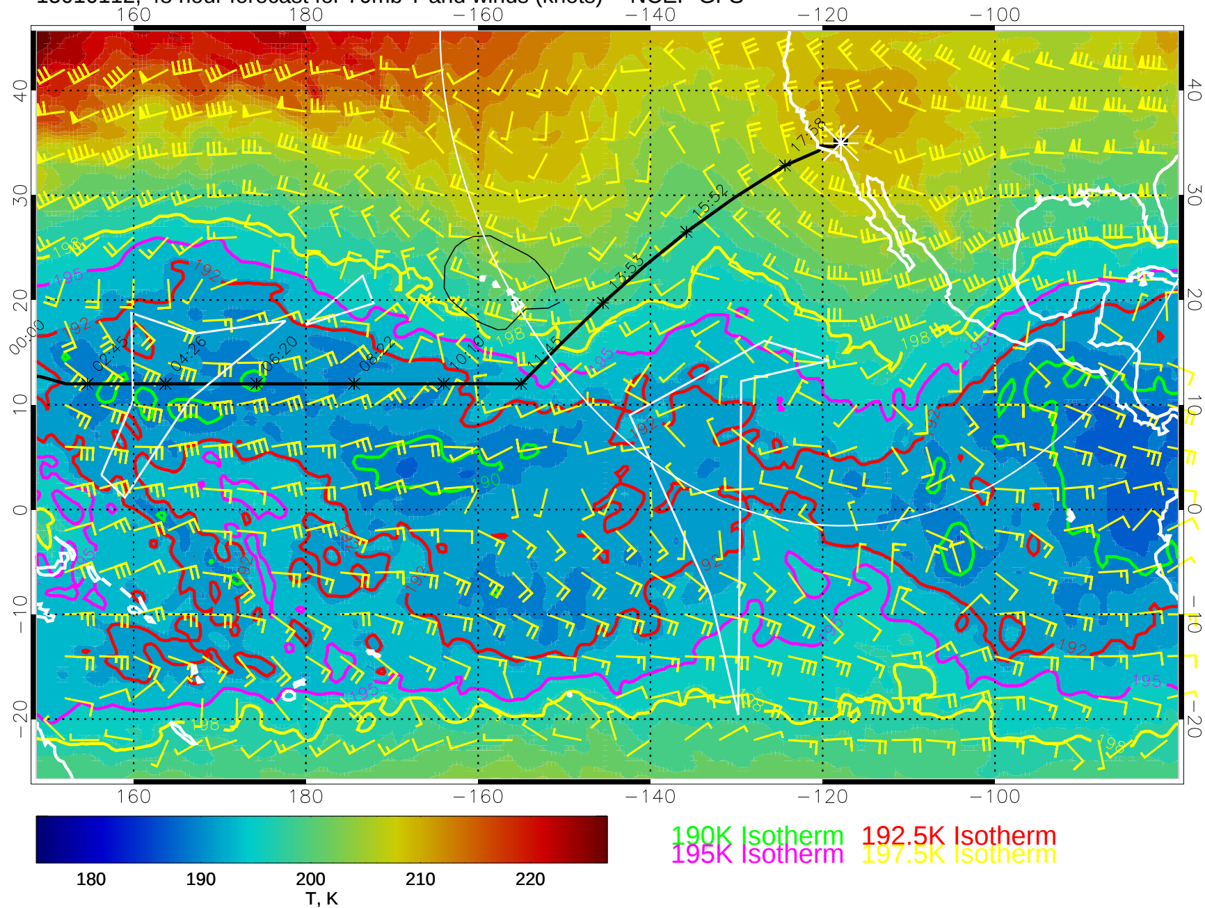
15010112, 48 hour forecast for 70mb T and winds (knots) -- NCEP GFS
