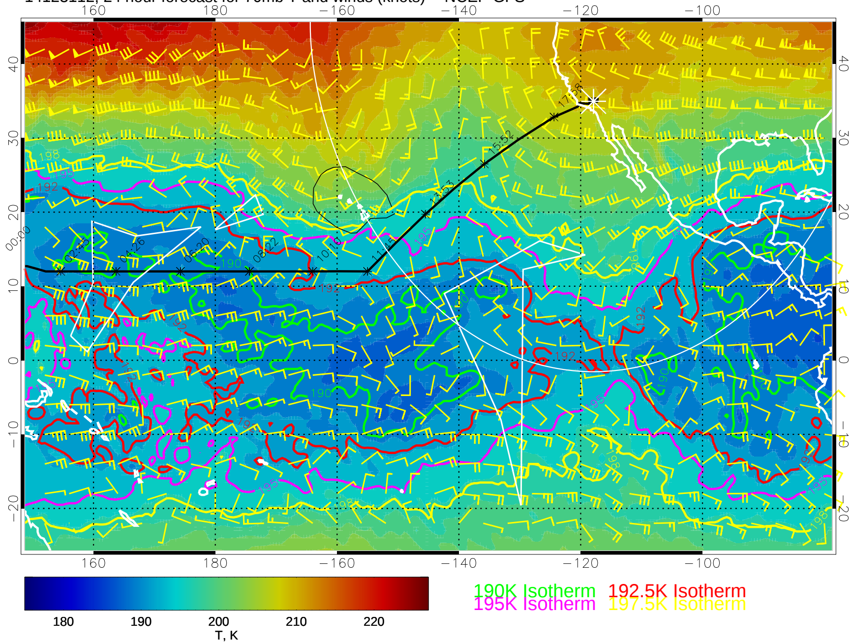
14123112, 24 hour forecast for 70mb T and winds (knots) -- NCEP GFS
