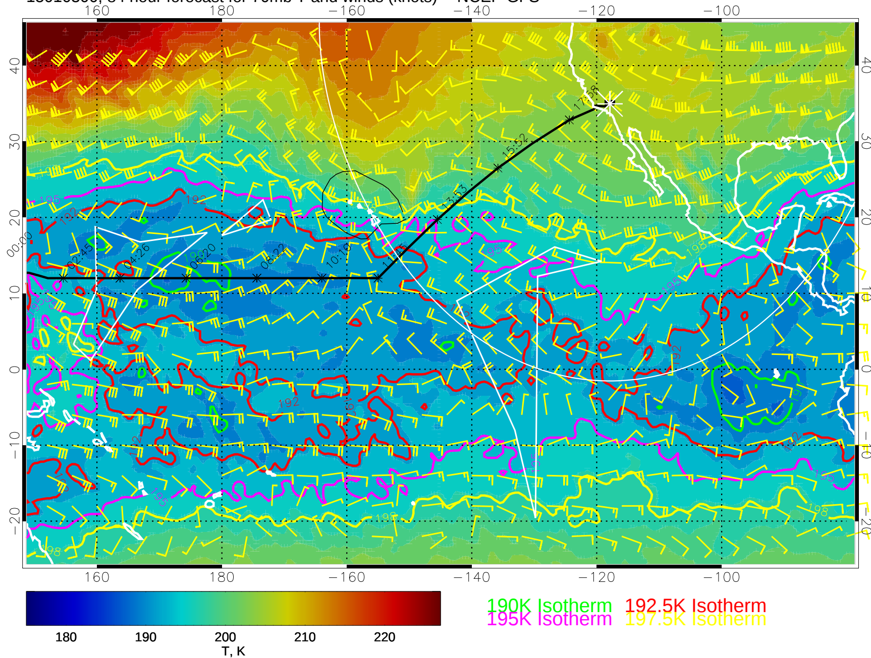
15010300, 84 hour forecast for 70mb T and winds (knots) -- NCEP GFS
