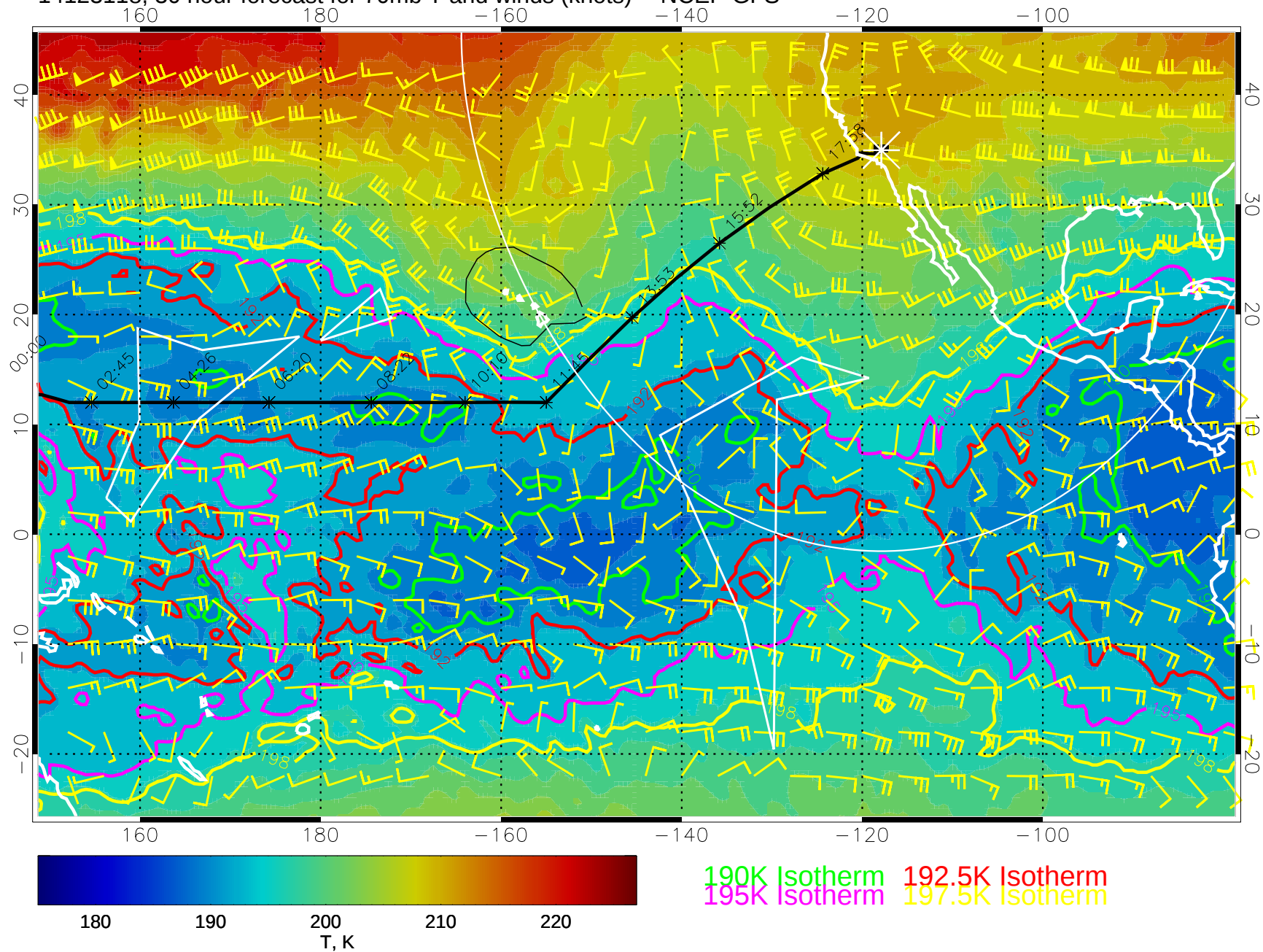
14123118, 30 hour forecast for 70mb T and winds (knots) -- NCEP GFS
