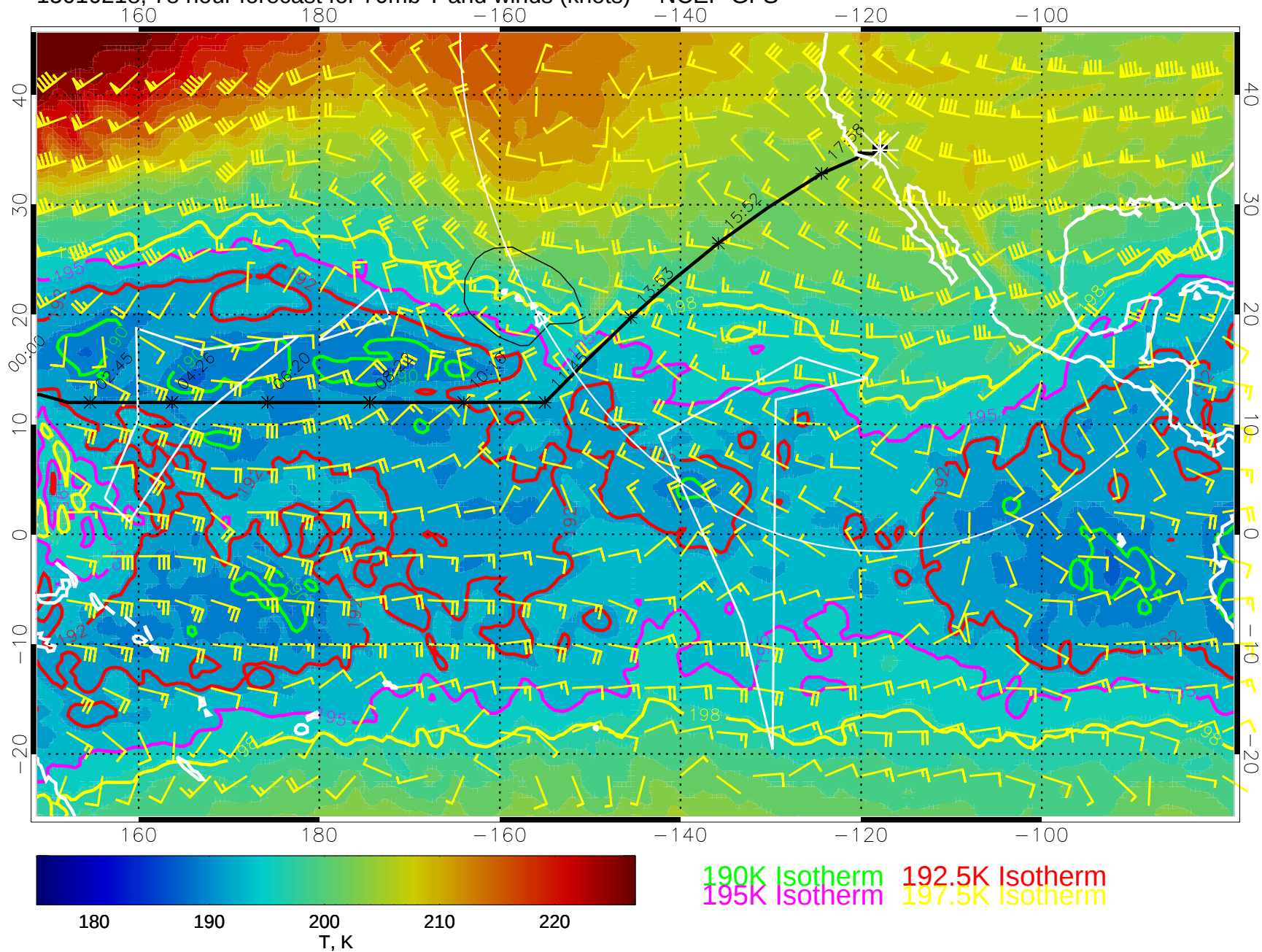
15010218, 78 hour forecast for 70mb T and winds (knots) -- NCEP GFS
