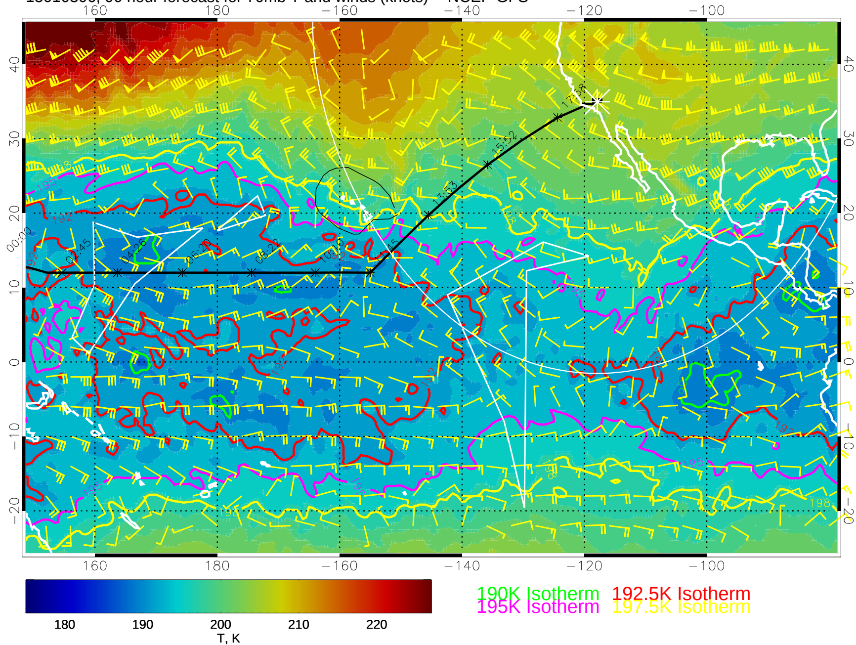
15010306, 90 hour forecast for 70mb T and winds (knots) -- NCEP GFS
