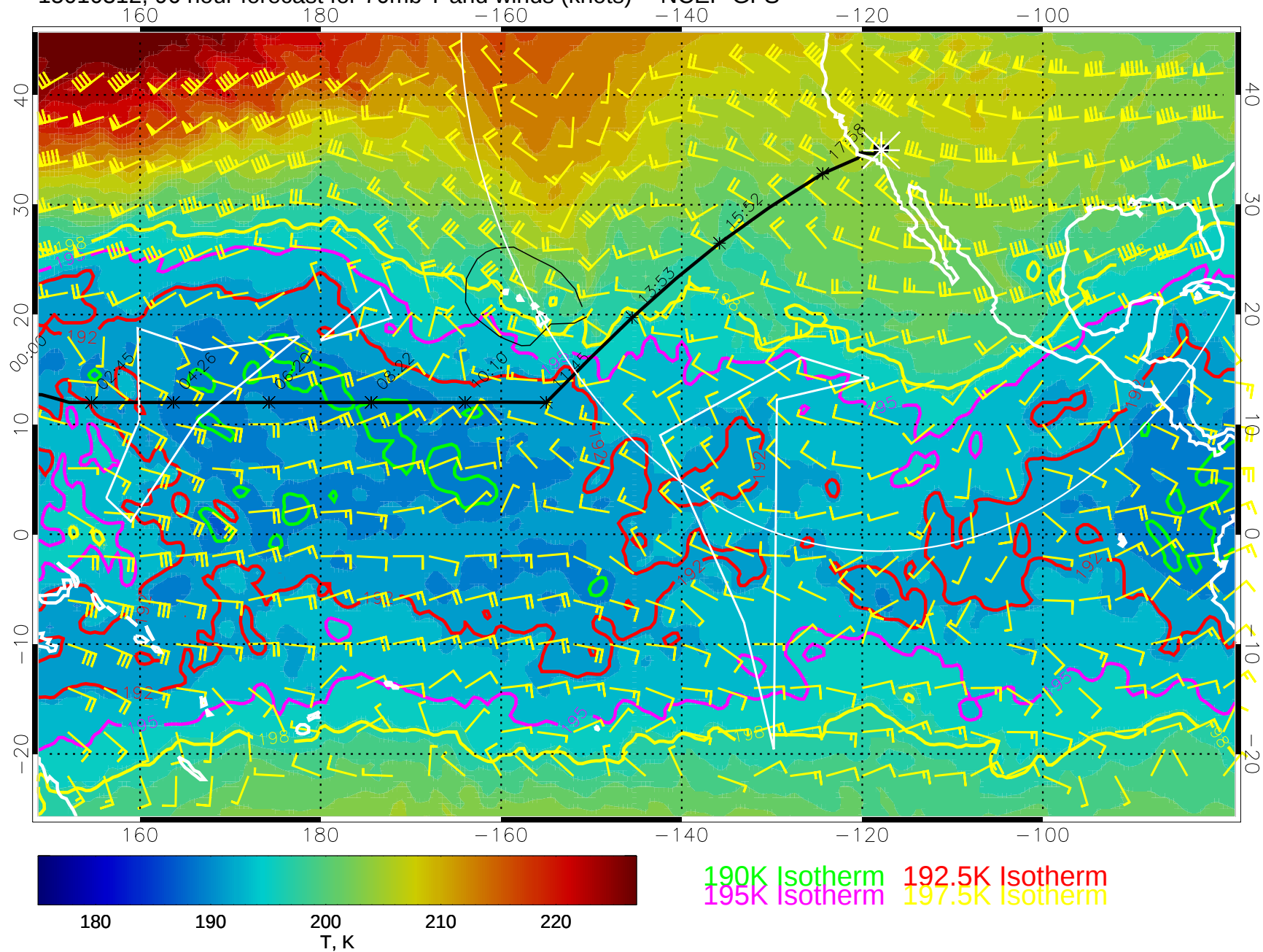
15010312, 96 hour forecast for 70mb T and winds (knots) -- NCEP GFS
