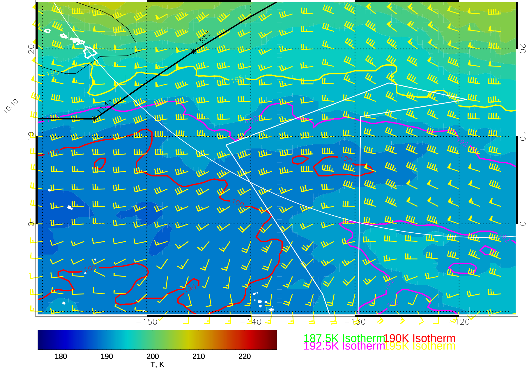
15010100, 36 hour forecast for 100mb T and winds (knots) -- NCEP GFS
