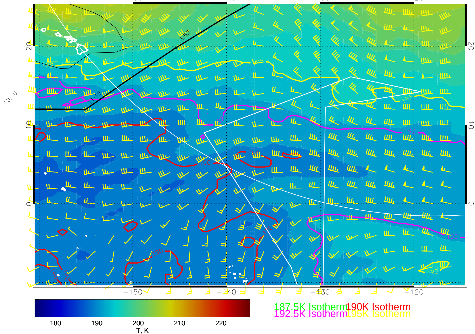
14123118, 30 hour forecast for 100mb T and winds (knots) -- NCEP GFS
