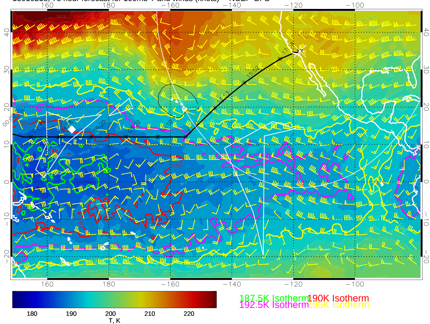
15010218, 78 hour forecast for 100mb T and winds (knots) -- NCEP GFS
