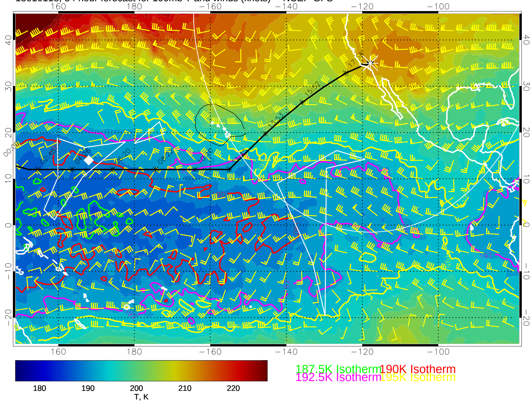
15010118, 54 hour forecast for 100mb T and winds (knots) -- NCEP GFS
