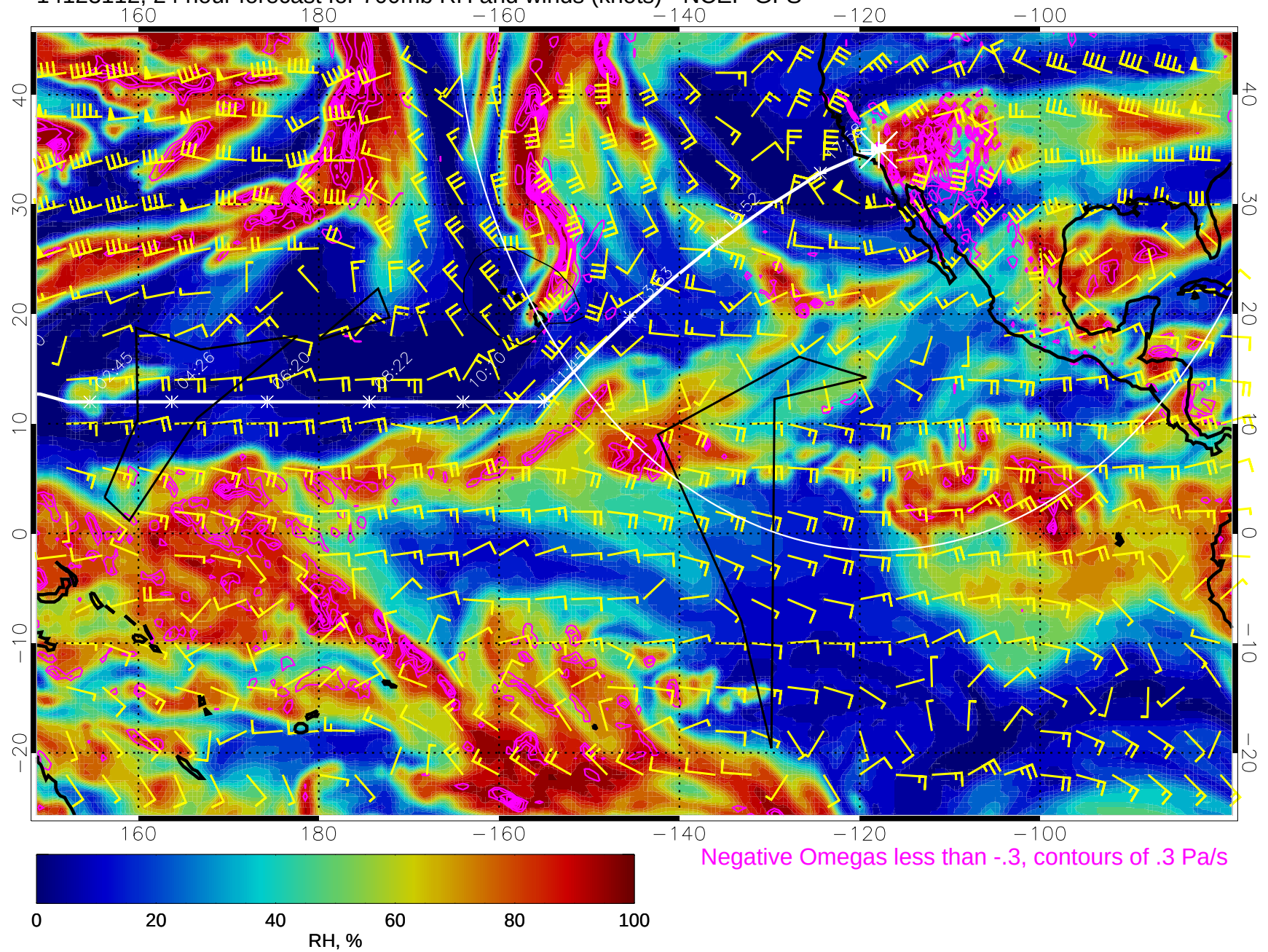
14123112, 24 hour forecast for 700mb RH and winds (knots) - NCEP GFS
