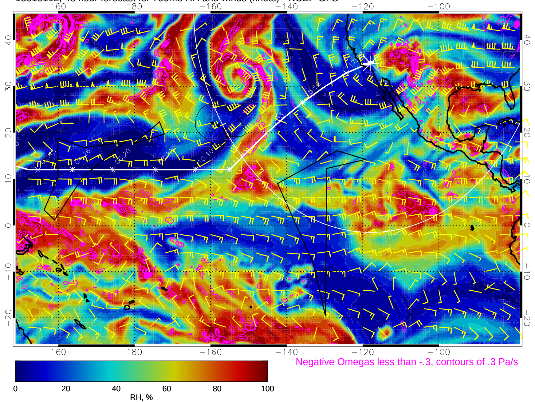
15010112, 48 hour forecast for 700mb RH and winds (knots) - NCEP GFS
