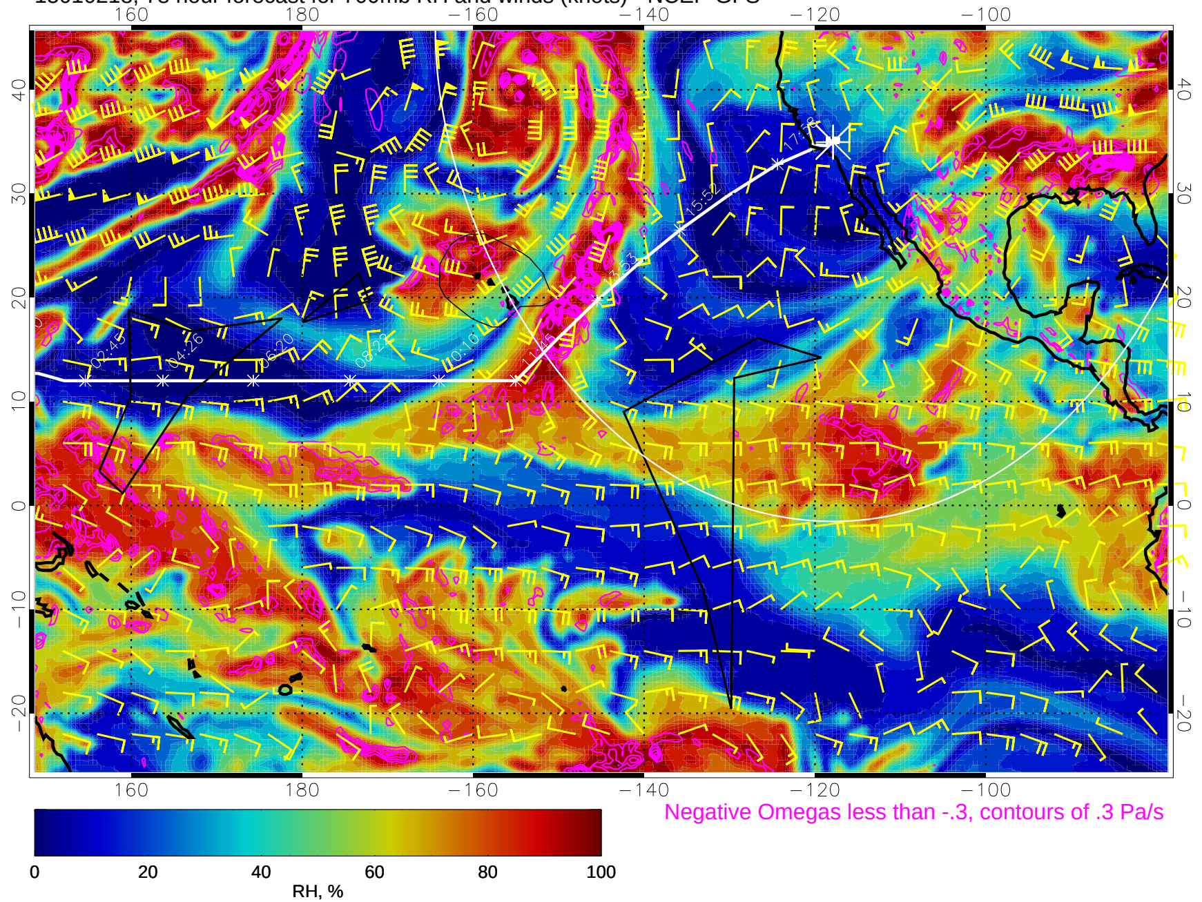
15010218, 78 hour forecast for 700mb RH and winds (knots) - NCEP GFS
