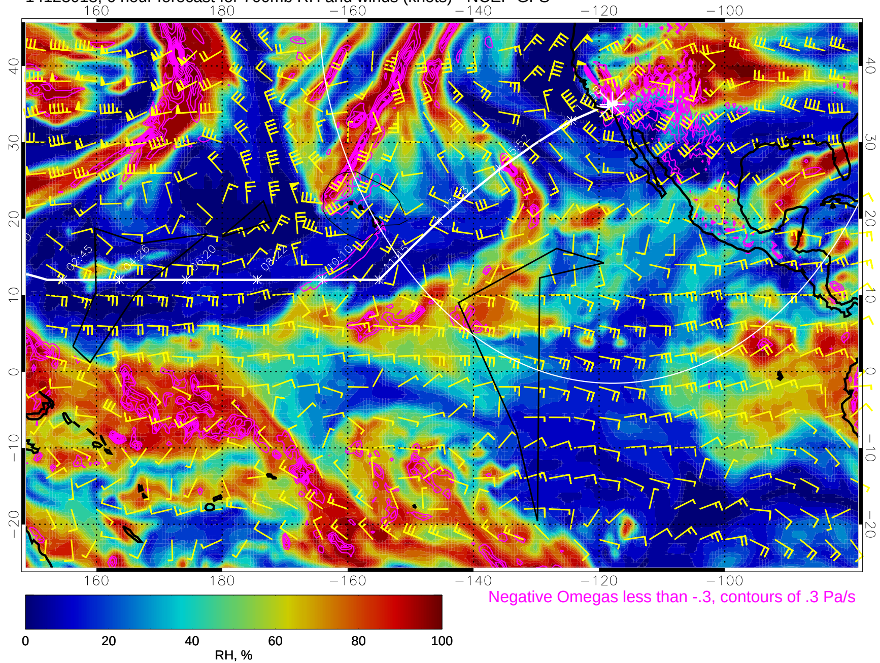
14123018, 6 hour forecast for 700mb RH and winds (knots) - NCEP GFS
