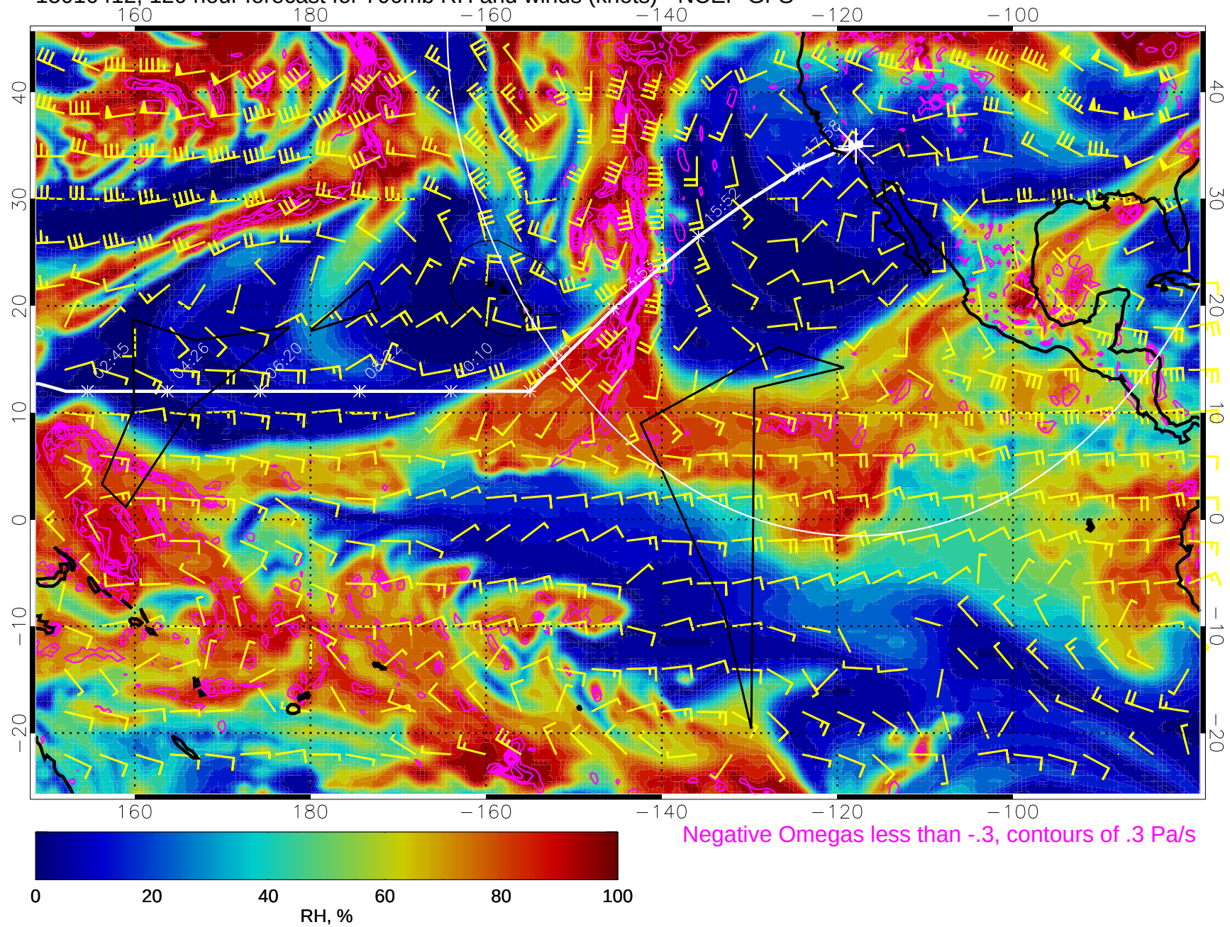
15010412, 120 hour forecast for 700mb RH and winds (knots) - NCEP GFS
