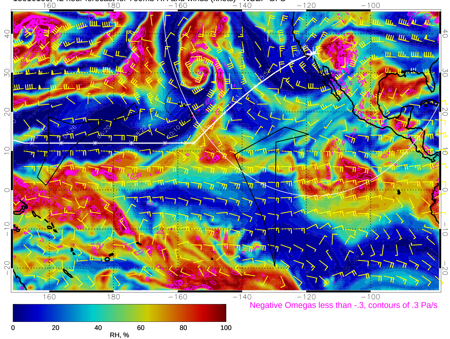
15010106, 42 hour forecast for 700mb RH and winds (knots) - NCEP GFS
