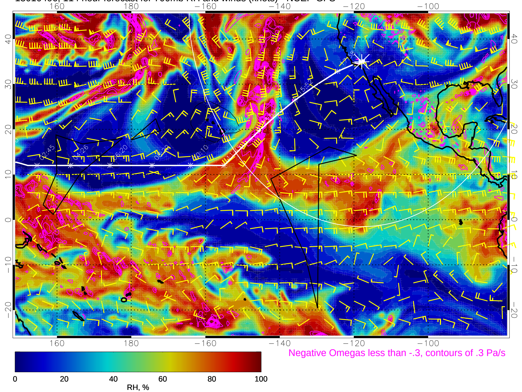
15010406, 114 hour forecast for 700mb RH and winds (knots) - NCEP GFS
