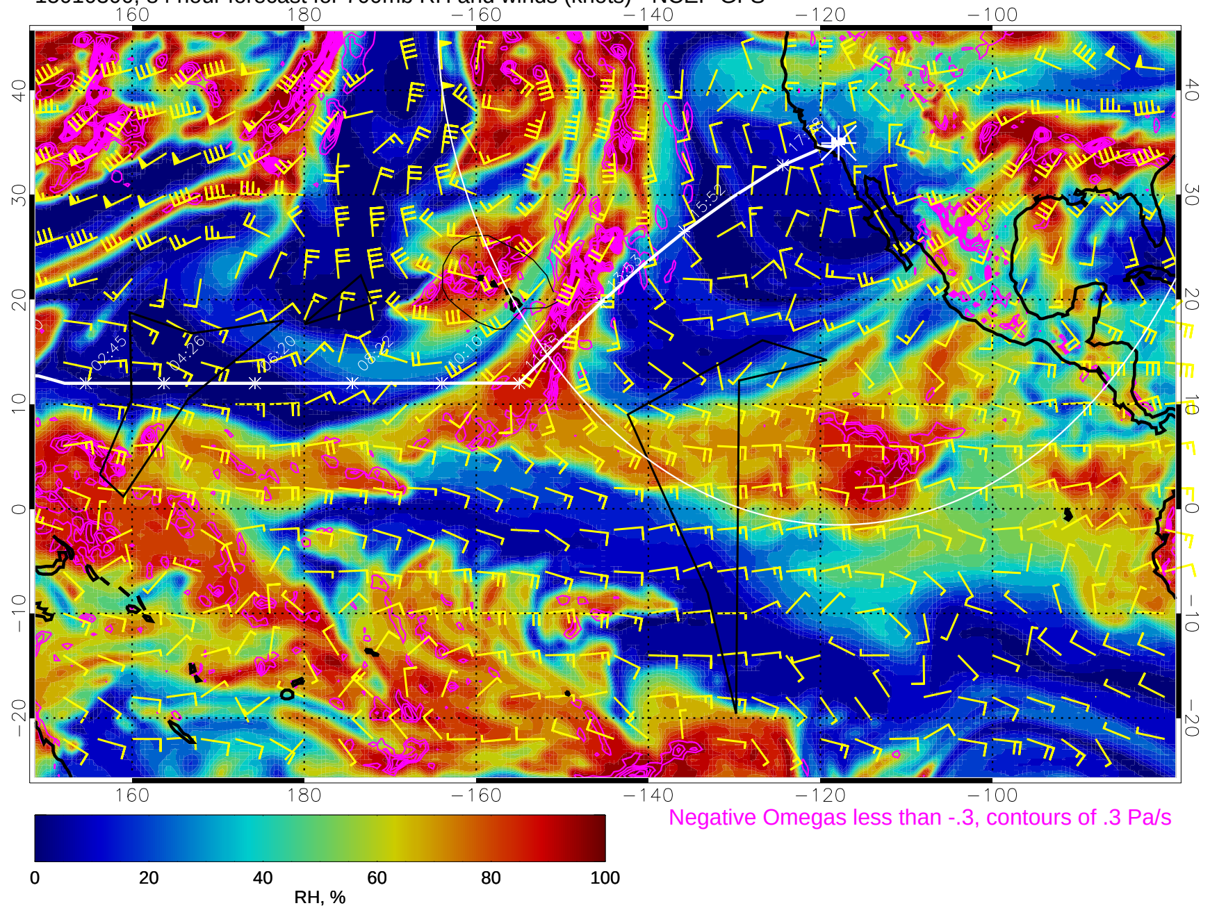
15010300, 84 hour forecast for 700mb RH and winds (knots) - NCEP GFS
