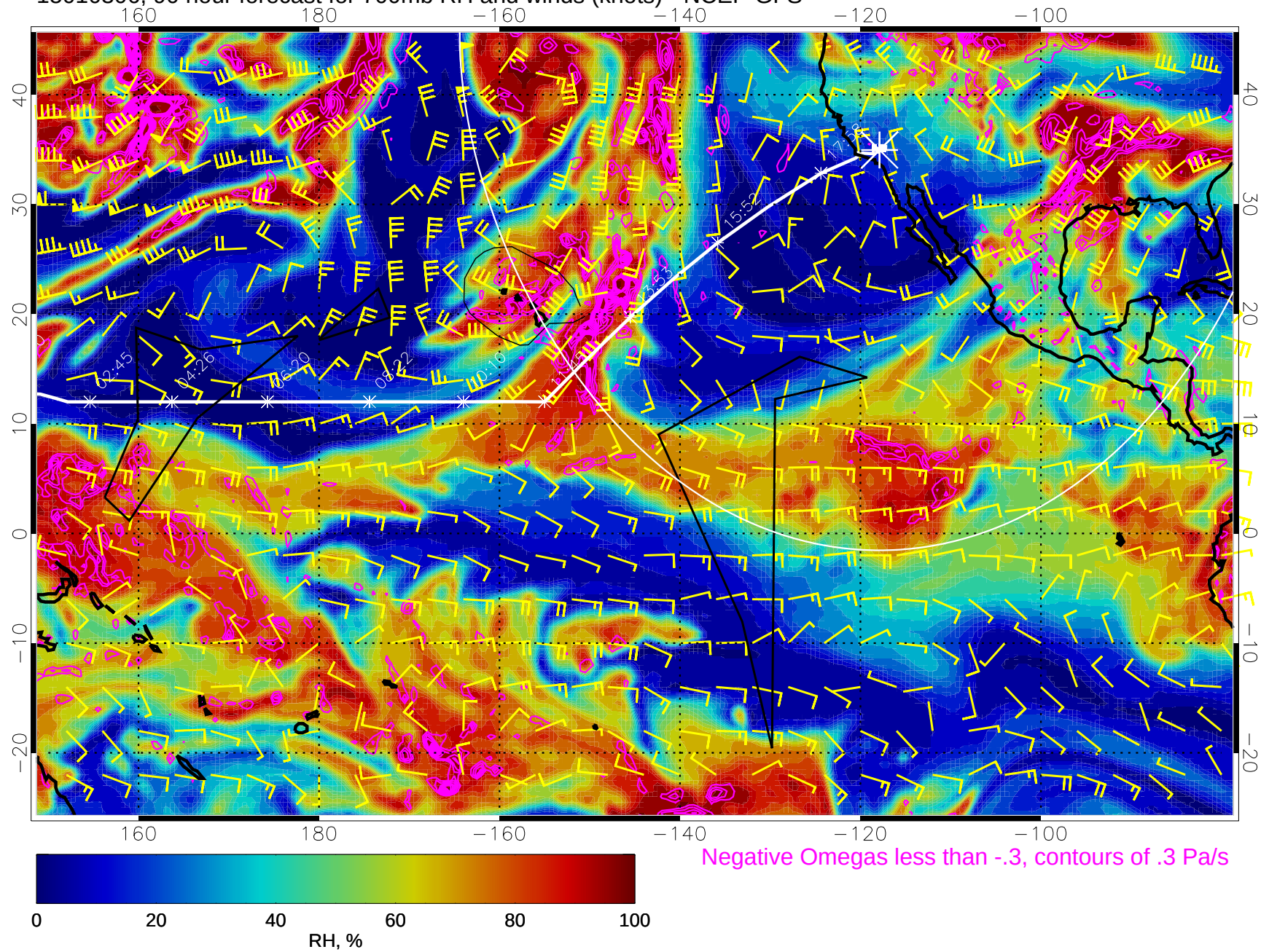
15010306, 90 hour forecast for 700mb RH and winds (knots) - NCEP GFS
