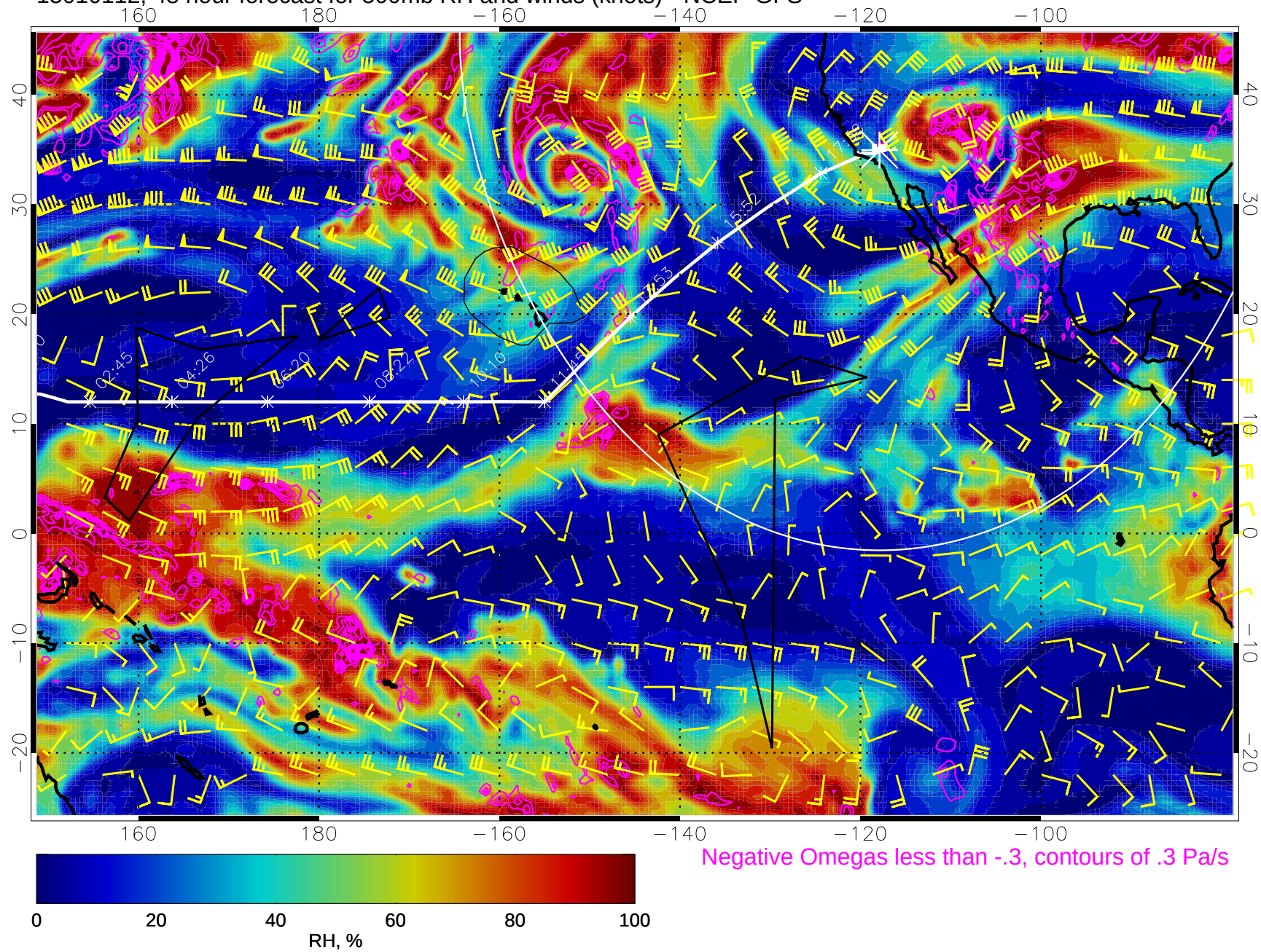
15010112, 48 hour forecast for 500mb RH and winds (knots) - NCEP GFS
