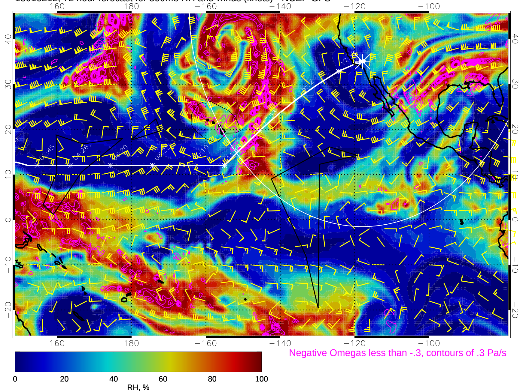
15010212, 72 hour forecast for 500mb RH and winds (knots) - NCEP GFS
