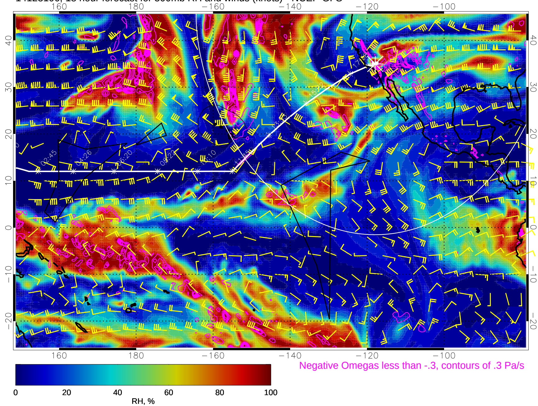
14123106, 18 hour forecast for 500mb RH and winds (knots) - NCEP GFS
