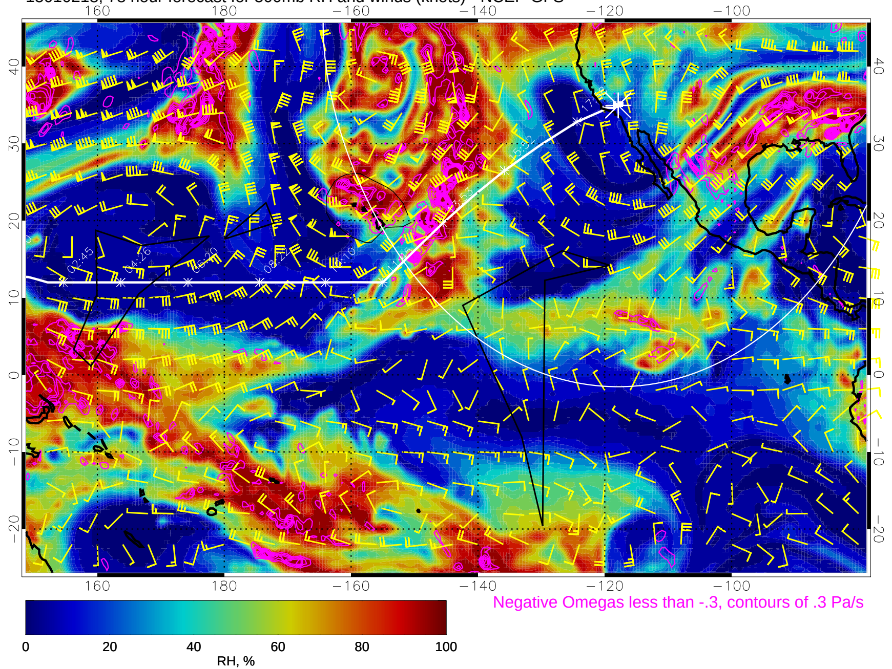
15010218, 78 hour forecast for 500mb RH and winds (knots) - NCEP GFS
