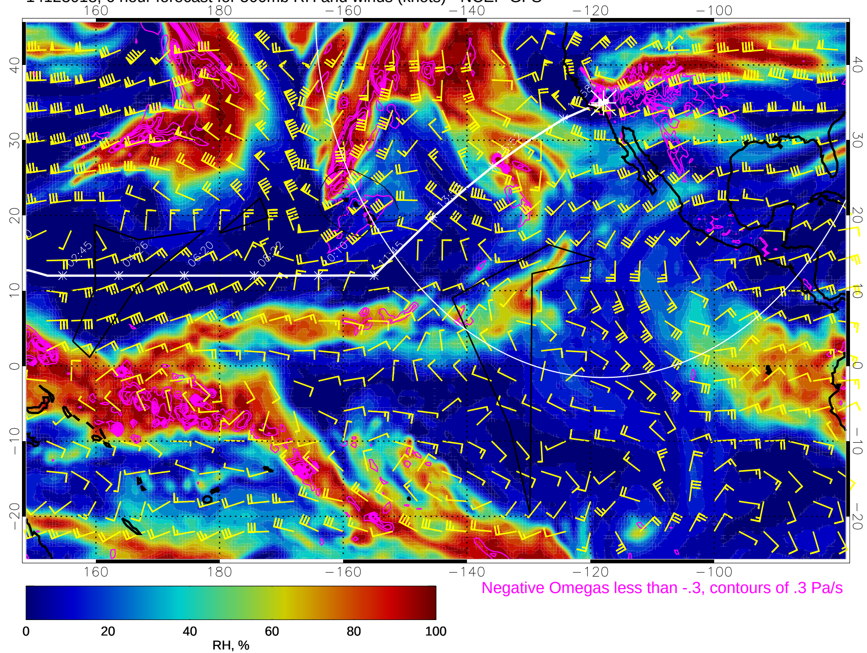
14123018, 6 hour forecast for 500mb RH and winds (knots) - NCEP GFS
