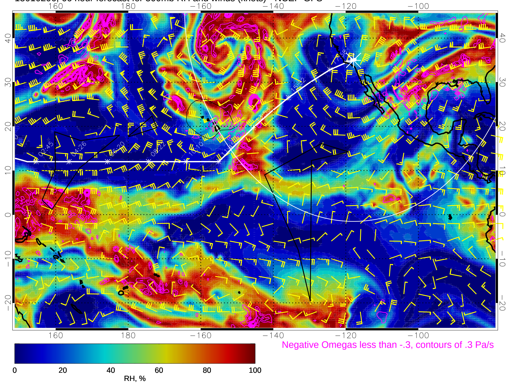
15010206, 66 hour forecast for 500mb RH and winds (knots) - NCEP GFS
