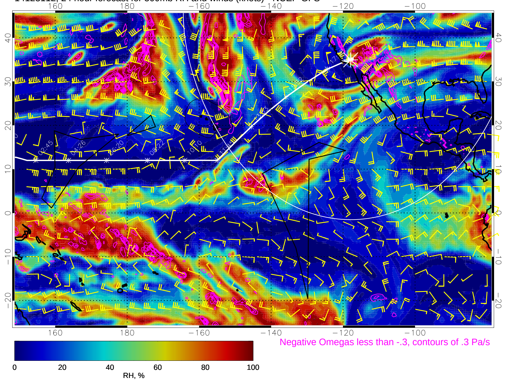
14123112, 24 hour forecast for 500mb RH and winds (knots) - NCEP GFS
