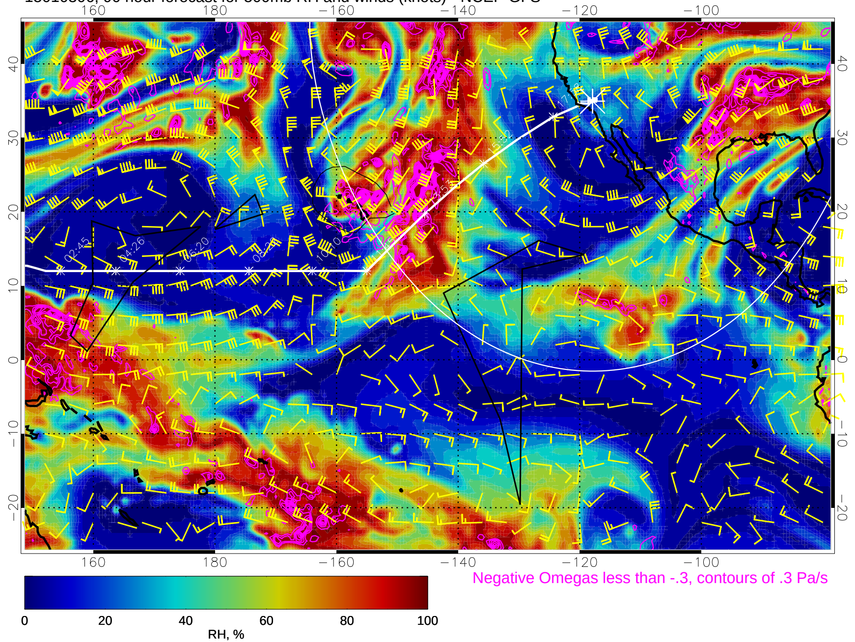
15010306, 90 hour forecast for 500mb RH and winds (knots) - NCEP GFS
