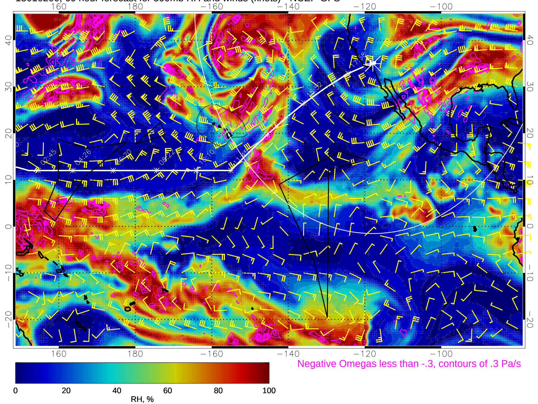
15010200, 60 hour forecast for 500mb RH and winds (knots) - NCEP GFS
