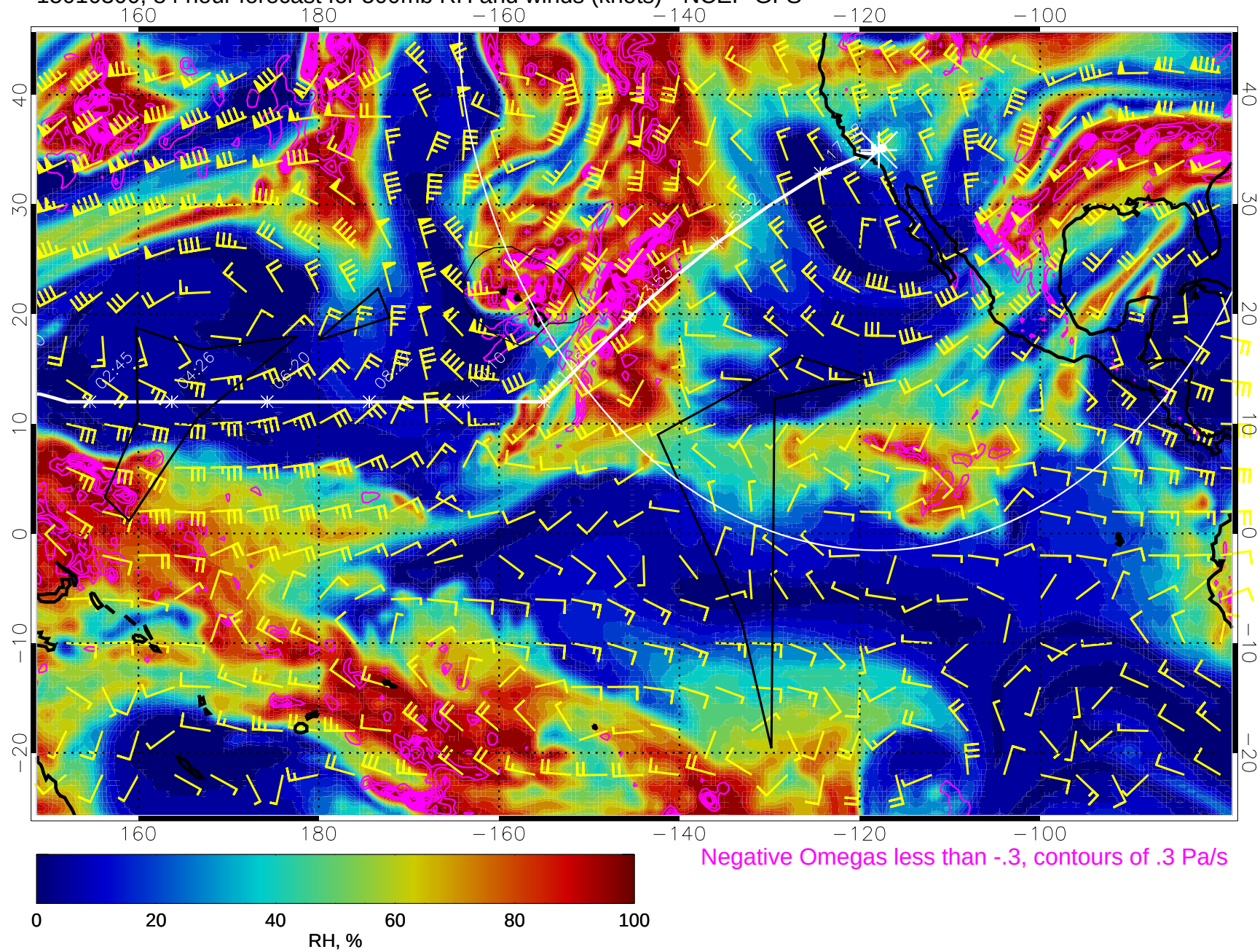
15010300, 84 hour forecast for 500mb RH and winds (knots) - NCEP GFS
