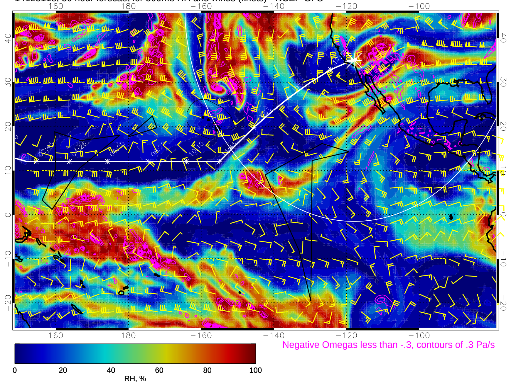
14123118, 30 hour forecast for 500mb RH and winds (knots) - NCEP GFS
