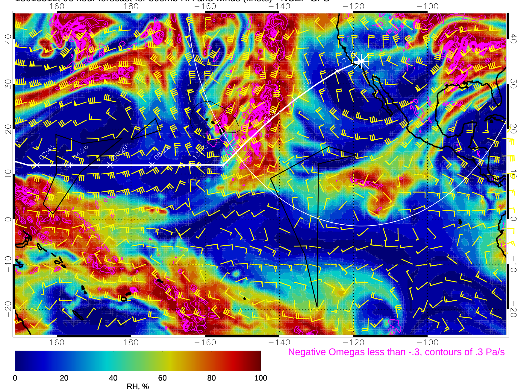
15010312, 96 hour forecast for 500mb RH and winds (knots) - NCEP GFS
