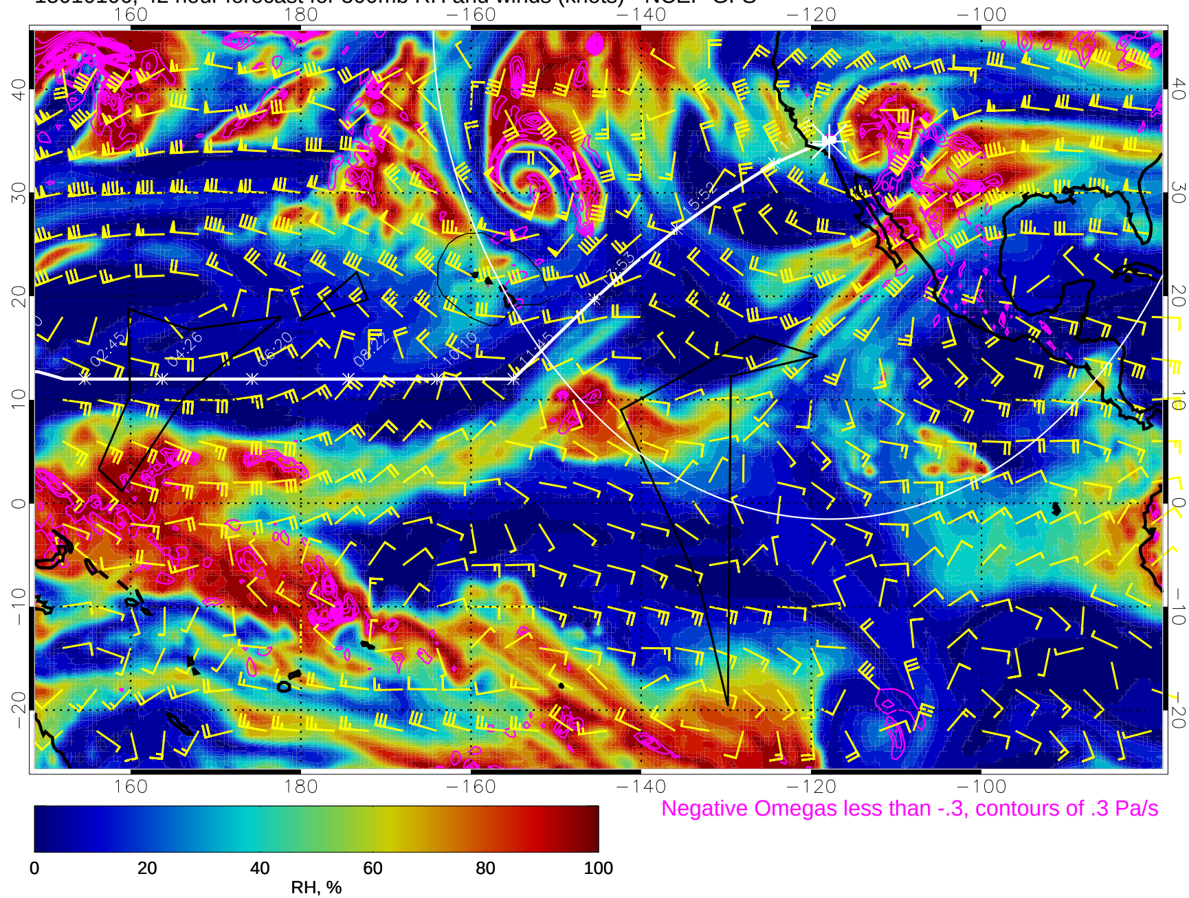
15010106, 42 hour forecast for 500mb RH and winds (knots) - NCEP GFS
