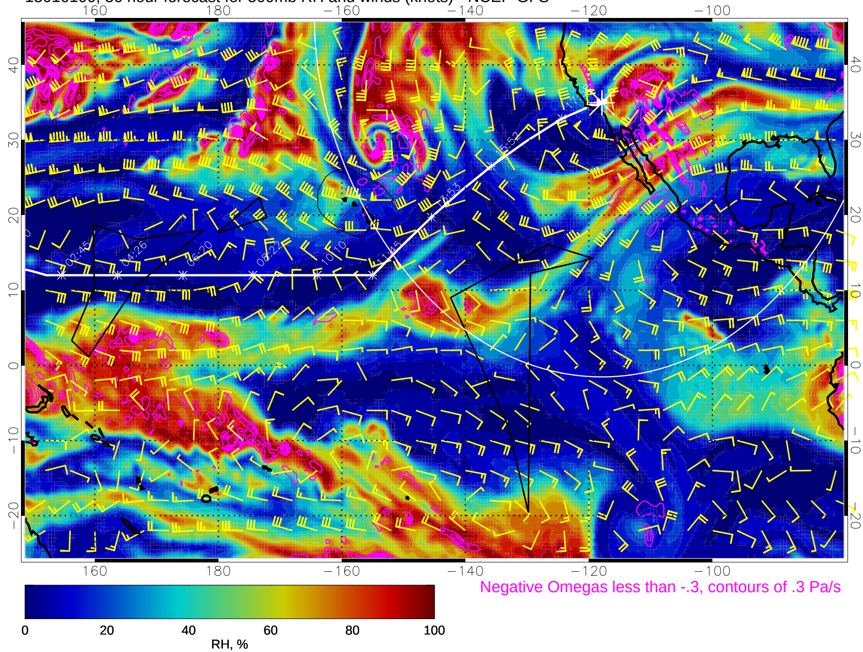
15010100, 36 hour forecast for 500mb RH and winds (knots) - NCEP GFS
