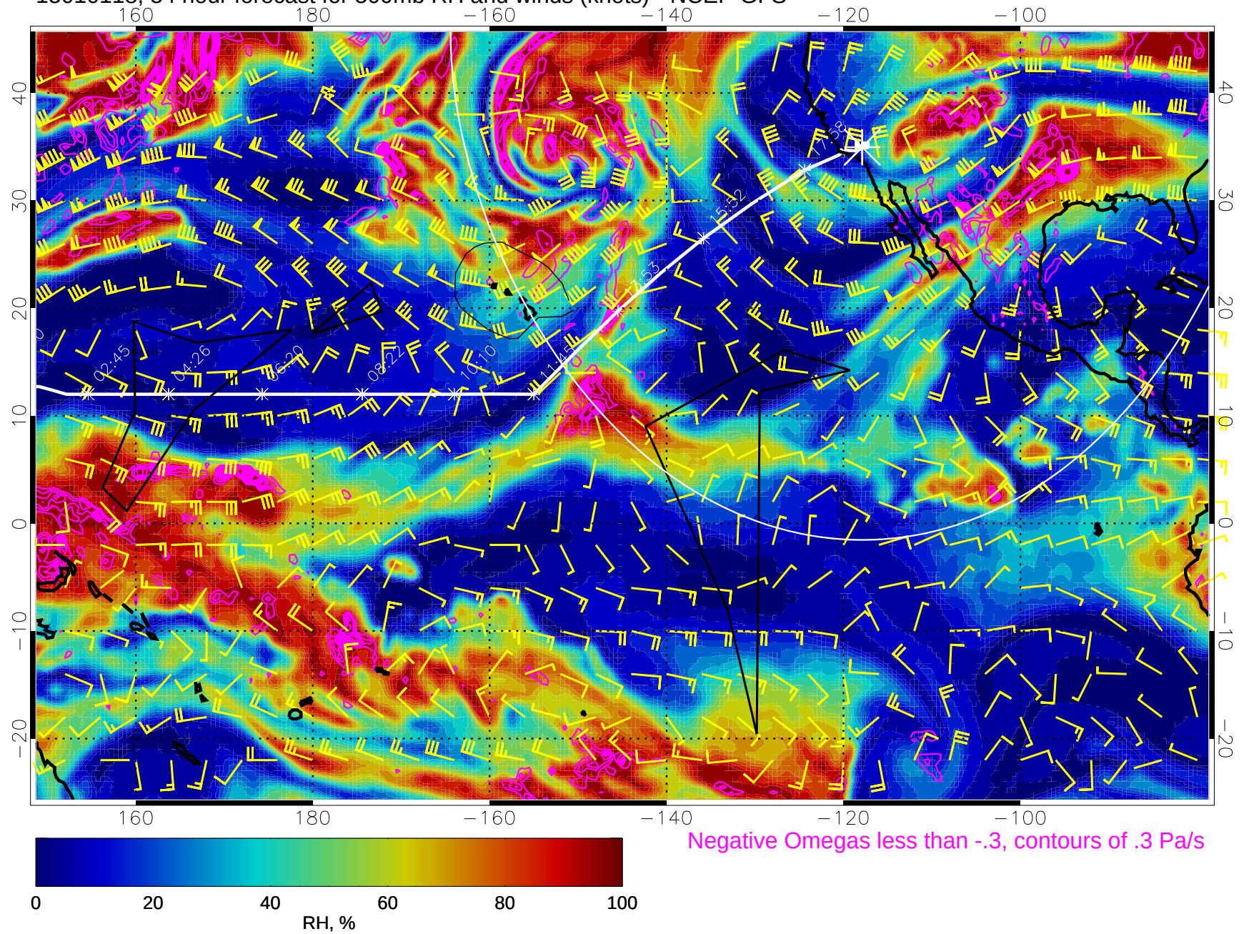
15010118, 54 hour forecast for 500mb RH and winds (knots) - NCEP GFS
