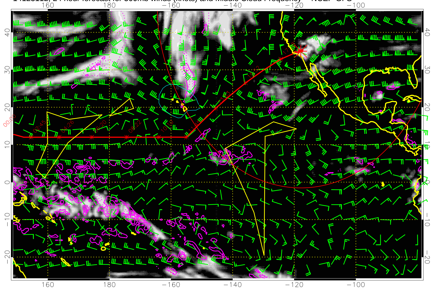
14123112, 24 hour forecast for 500mb winds (knots) and Middle Cloud Frequency -- NCEP GFS
