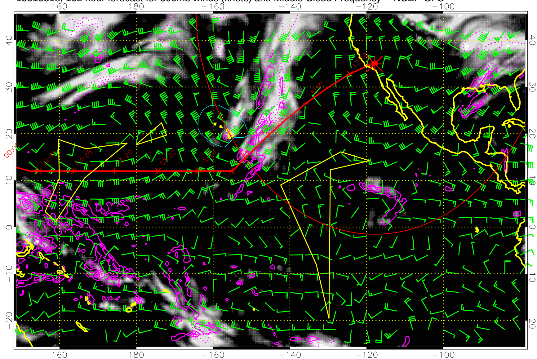
15010318, 102 hour forecast for 500mb winds (knots) and Middle Cloud Frequency -- NCEP GFS
