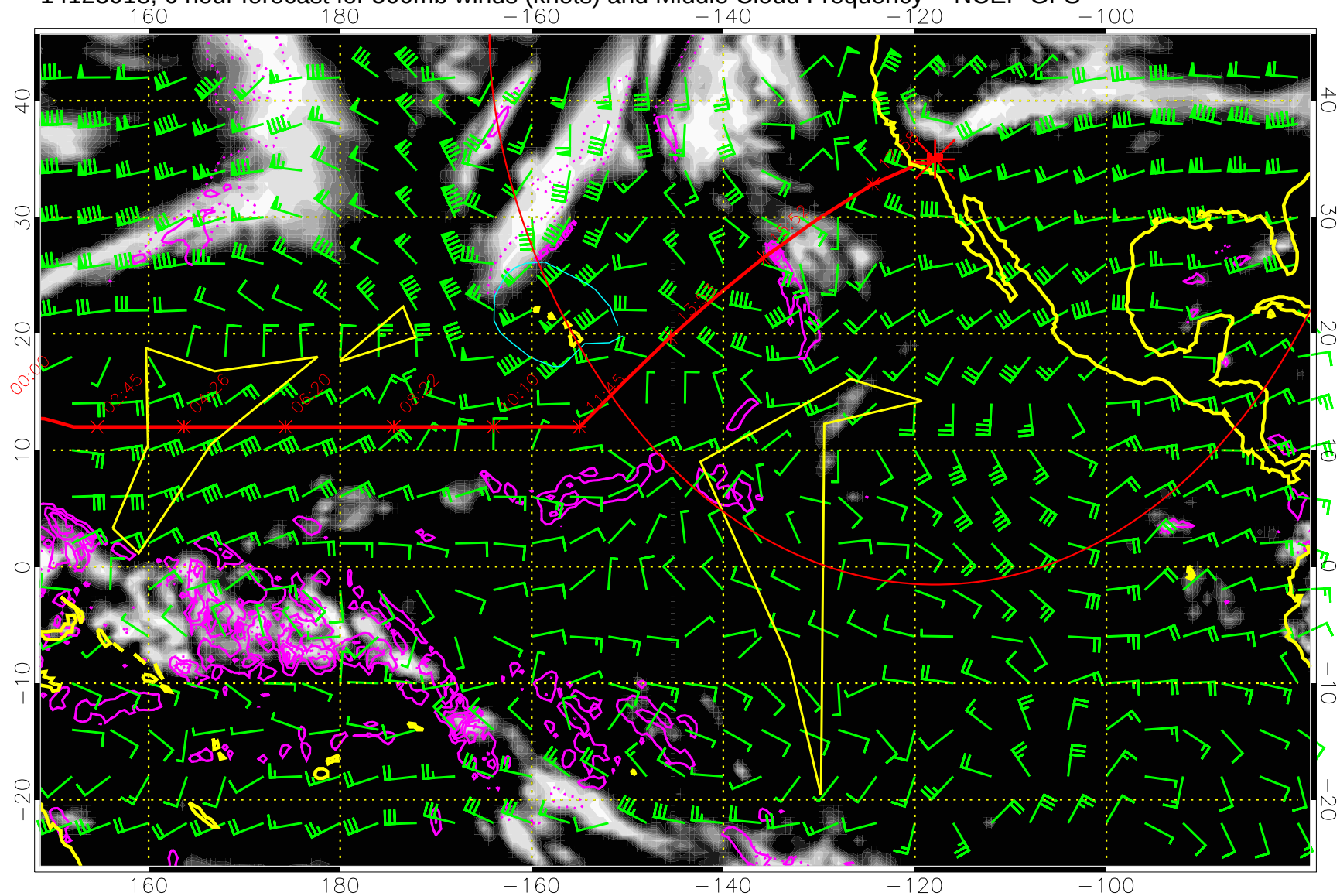
14123018, 6 hour forecast for 500mb winds (knots) and Middle Cloud Frequency -- NCEP GFS
