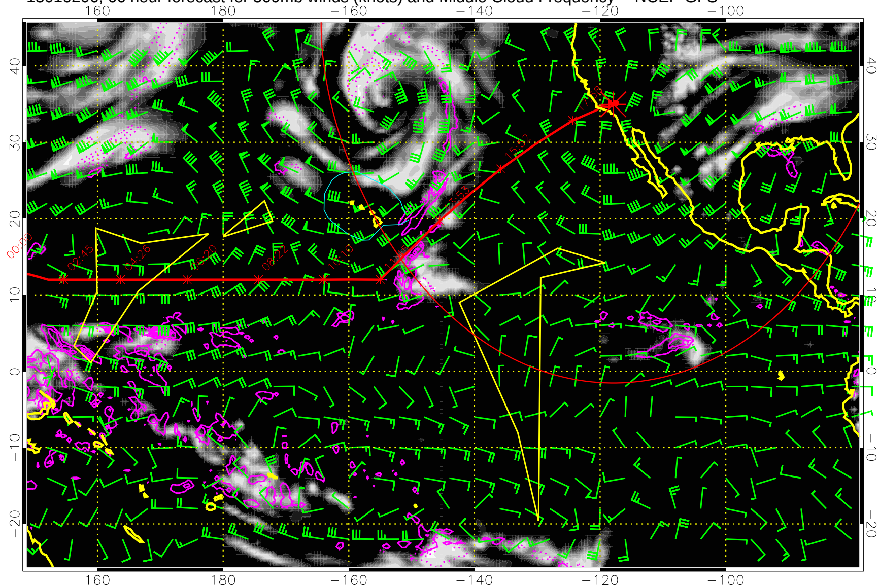
15010206, 66 hour forecast for 500mb winds (knots) and Middle Cloud Frequency -- NCEP GFS
