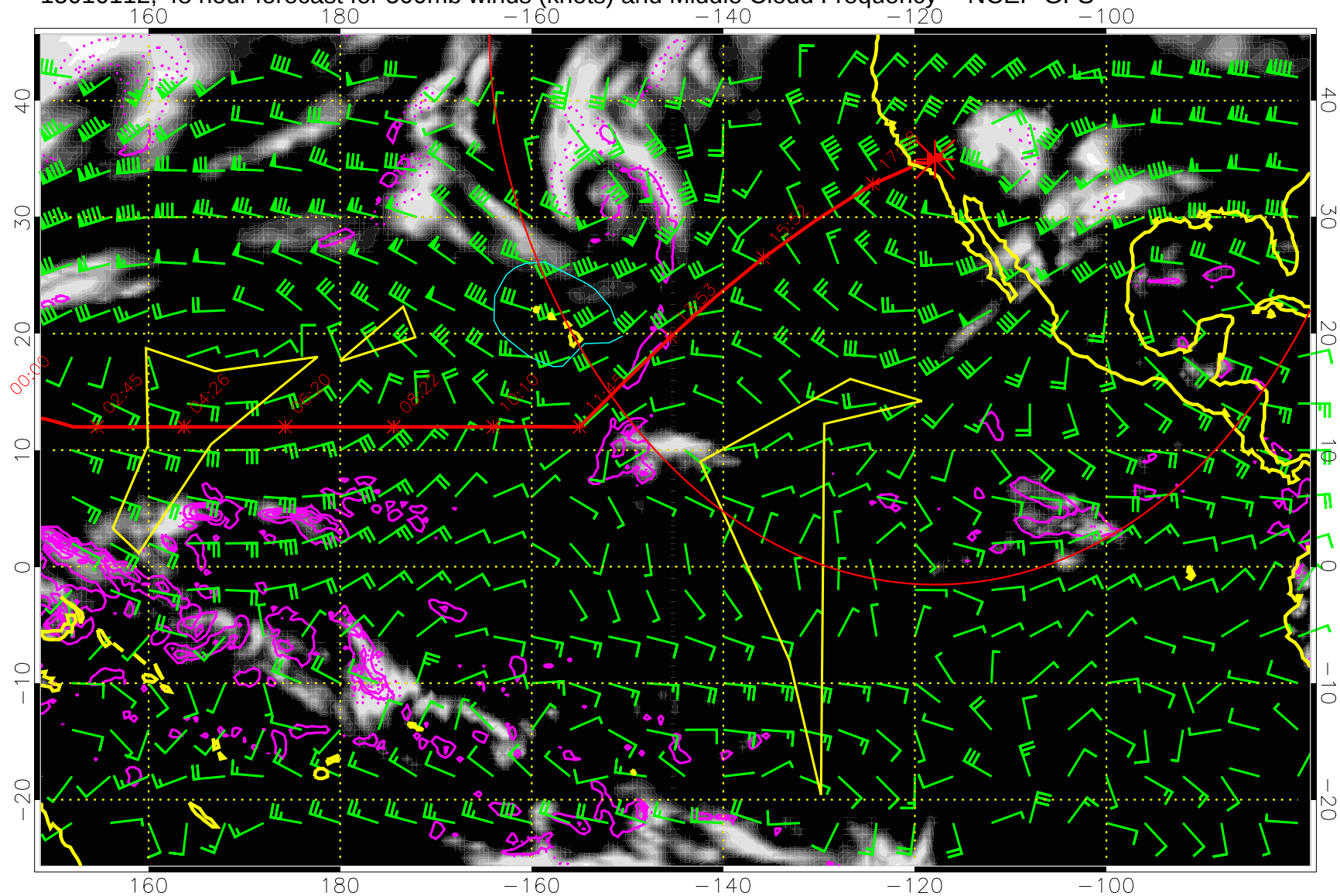
15010112, 48 hour forecast for 500mb winds (knots) and Middle Cloud Frequency -- NCEP GFS
