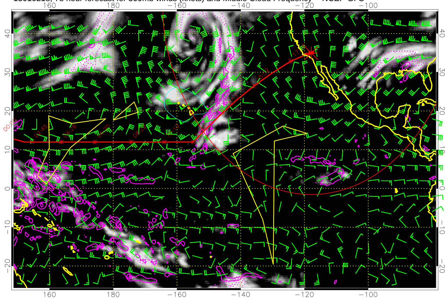
15010218, 78 hour forecast for 500mb winds (knots) and Middle Cloud Frequency -- NCEP GFS
