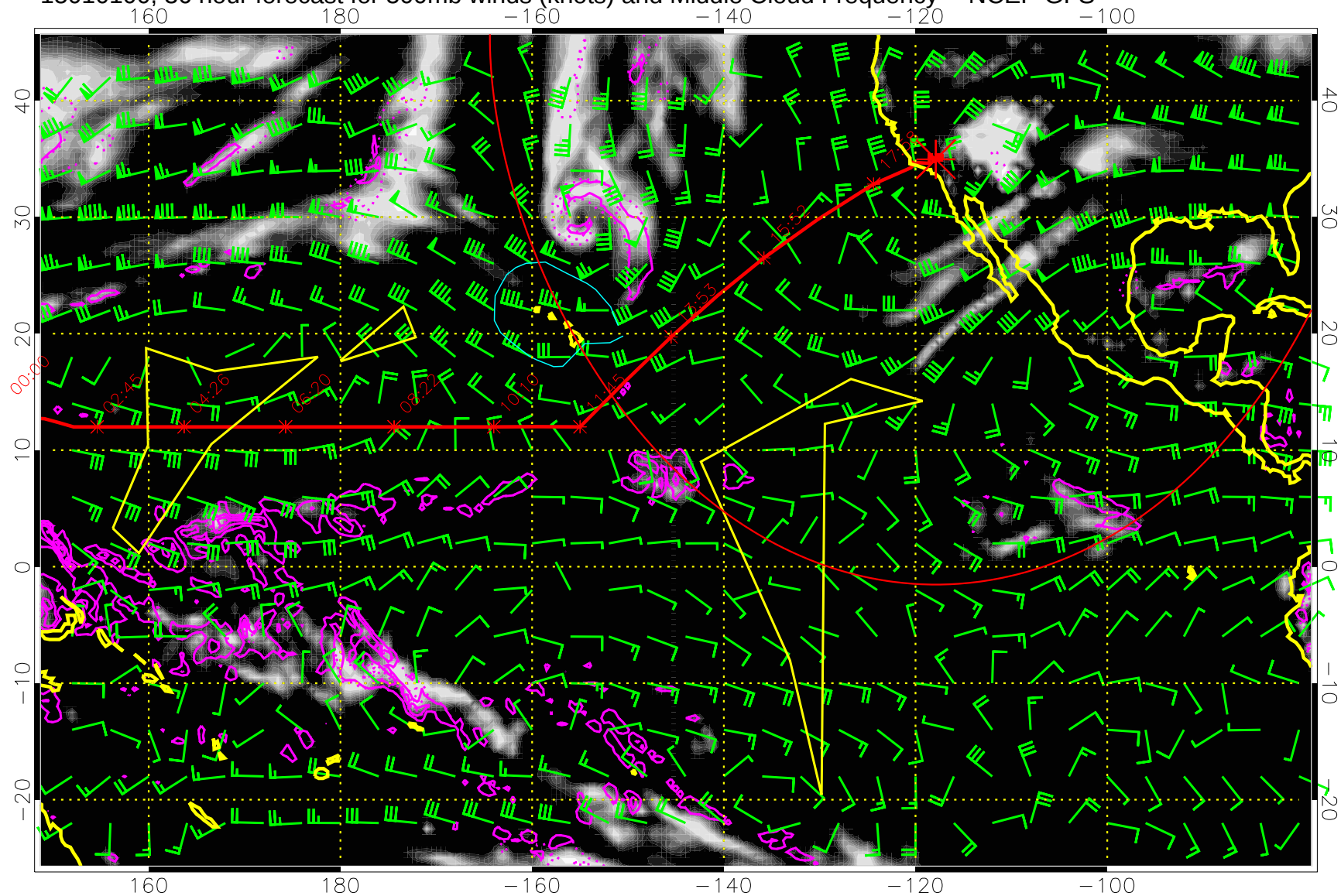
15010100, 36 hour forecast for 500mb winds (knots) and Middle Cloud Frequency -- NCEP GFS
