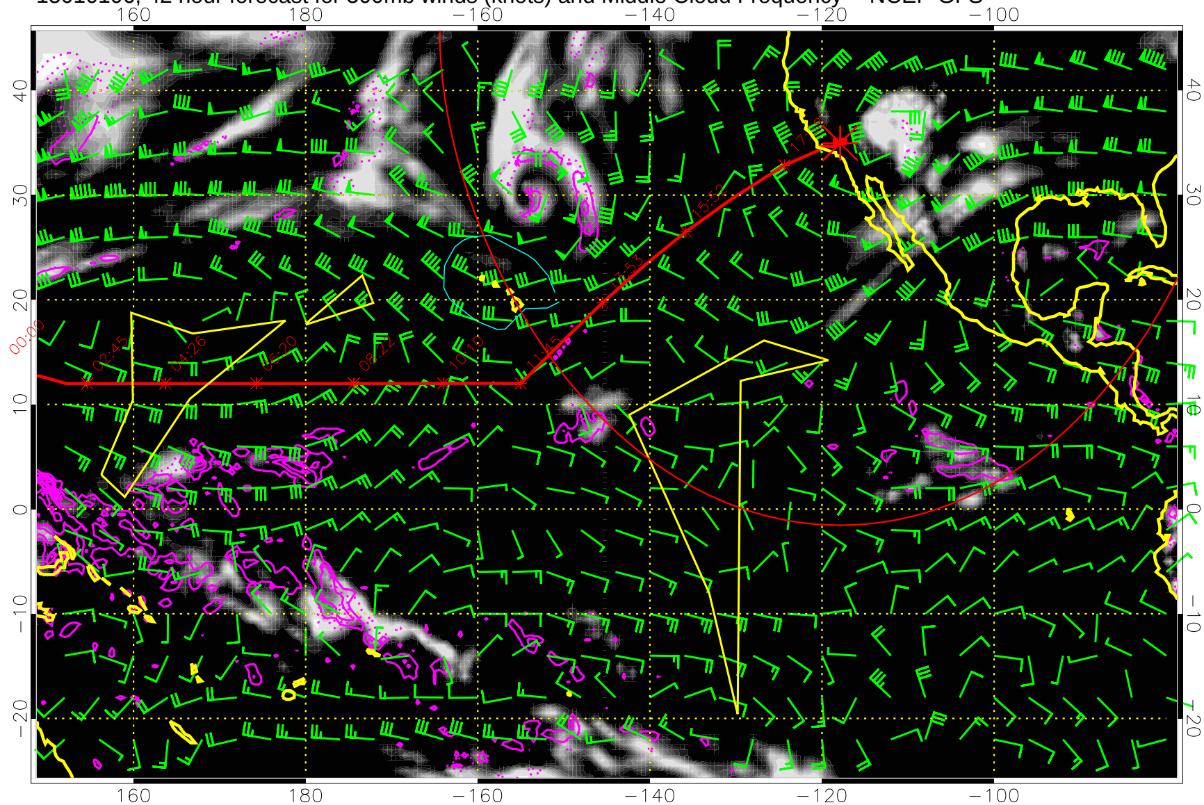
15010106, 42 hour forecast for 500mb winds (knots) and Middle Cloud Frequency -- NCEP GFS
