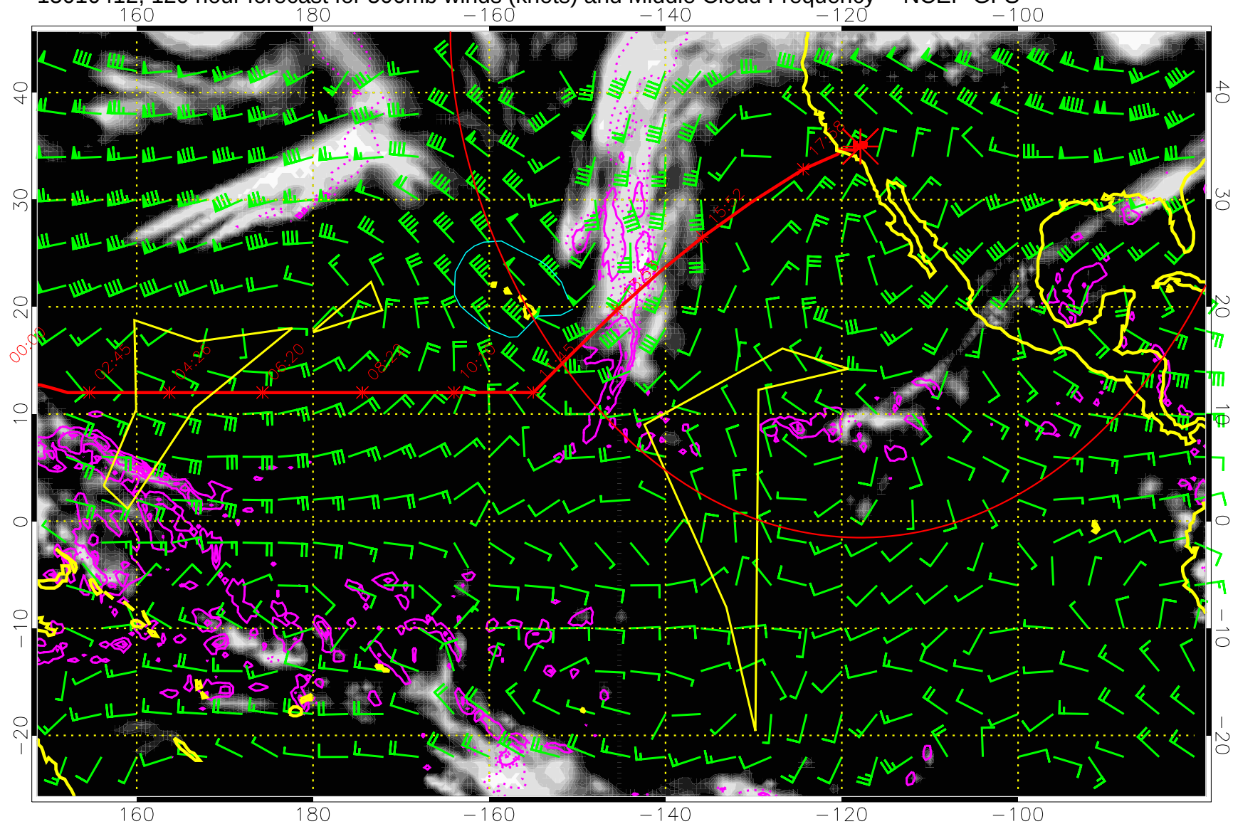
15010412, 120 hour forecast for 500mb winds (knots) and Middle Cloud Frequency -- NCEP GFS
