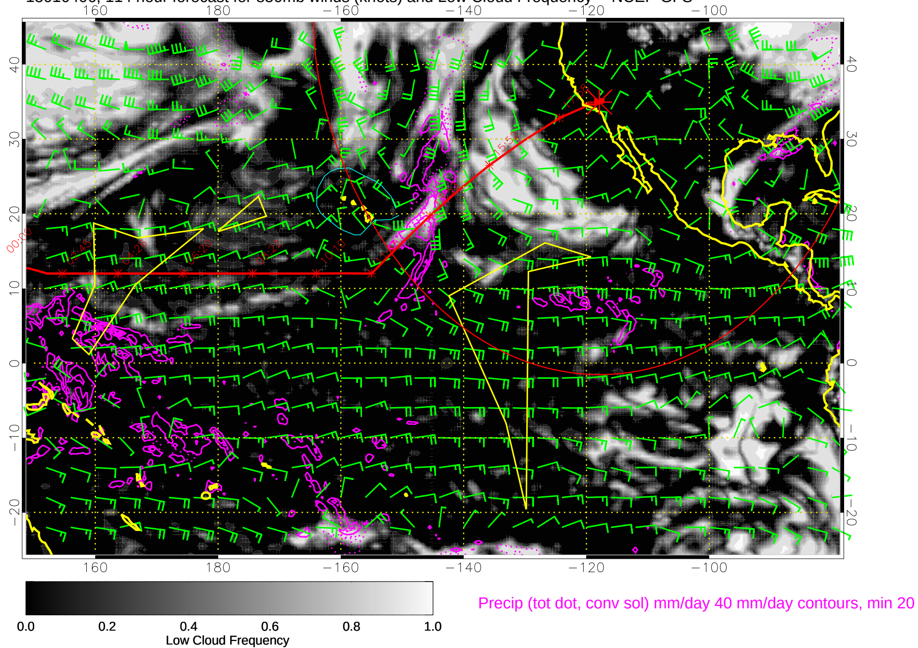
15010406, 114 hour forecast for 850mb winds (knots) and Low Cloud Frequency -- NCEP GFS
