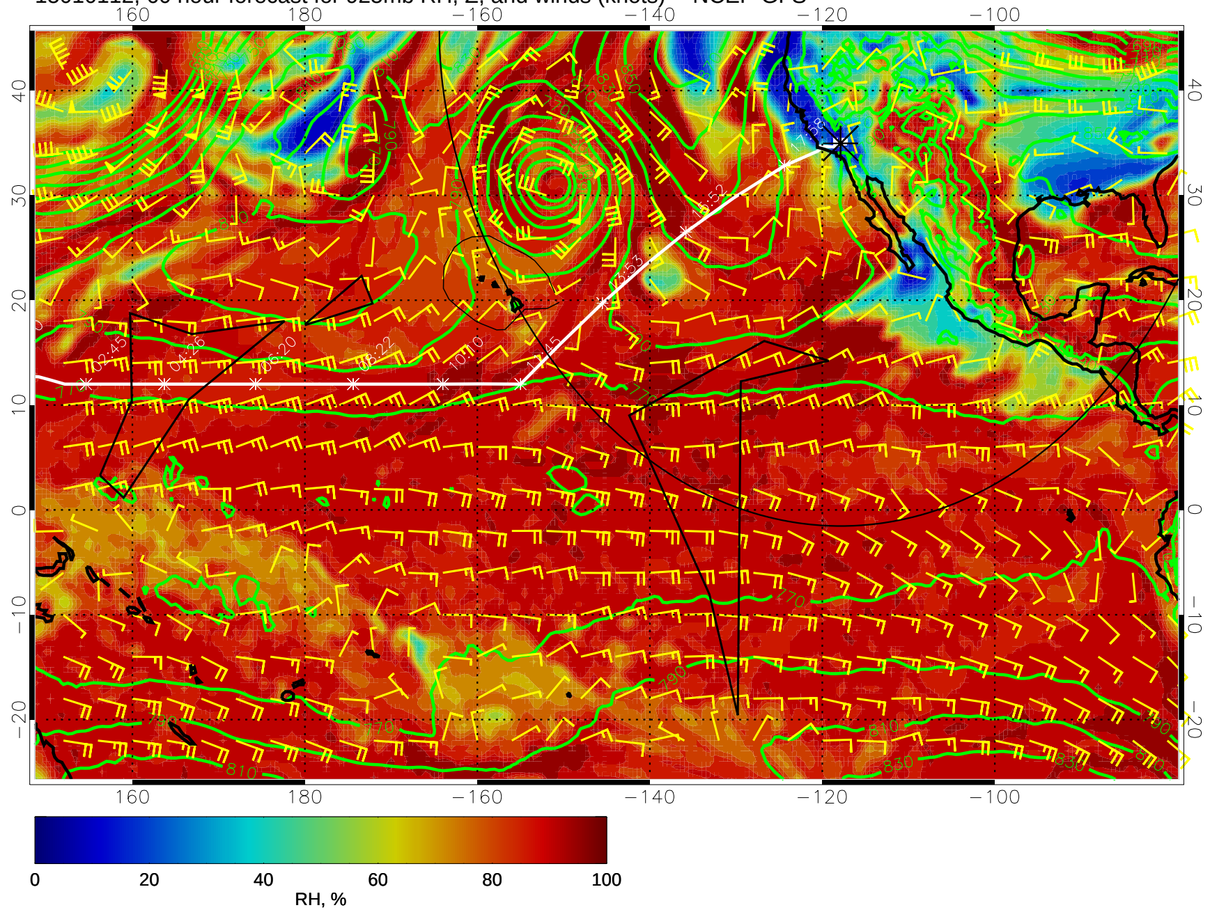
15010112, 60 hour forecast for 925mb RH, Z, and winds (knots) -- NCEP GFS
