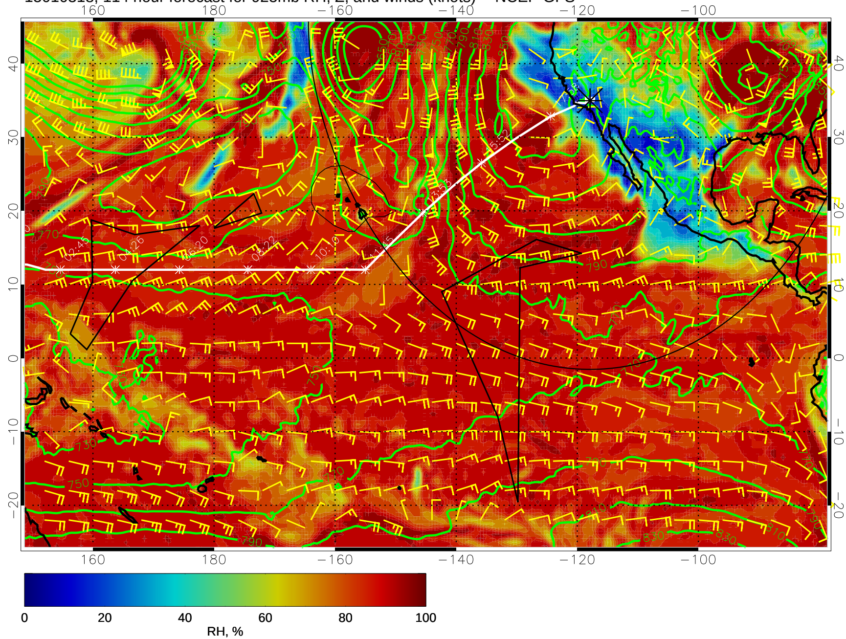
15010318, 114 hour forecast for 925mb RH, Z, and winds (knots) -- NCEP GFS
