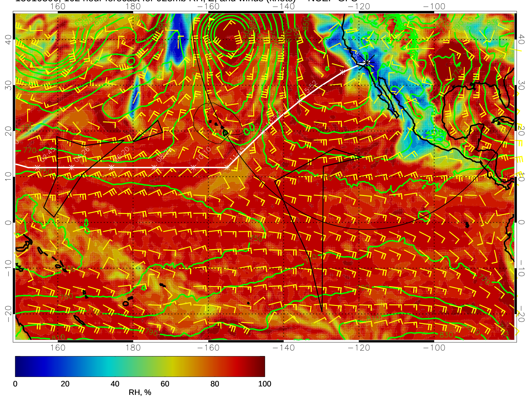
15010306, 102 hour forecast for 925mb RH, Z, and winds (knots) -- NCEP GFS
