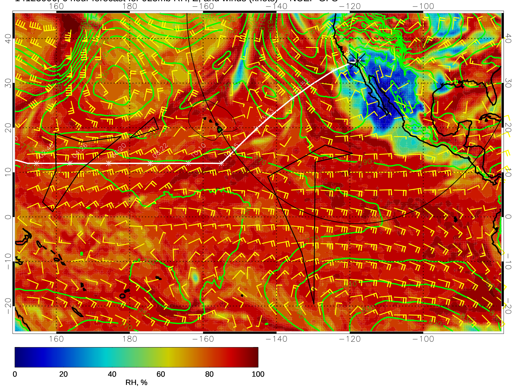
14123006, 6 hour forecast for 925mb RH, Z, and winds (knots) -- NCEP GFS
