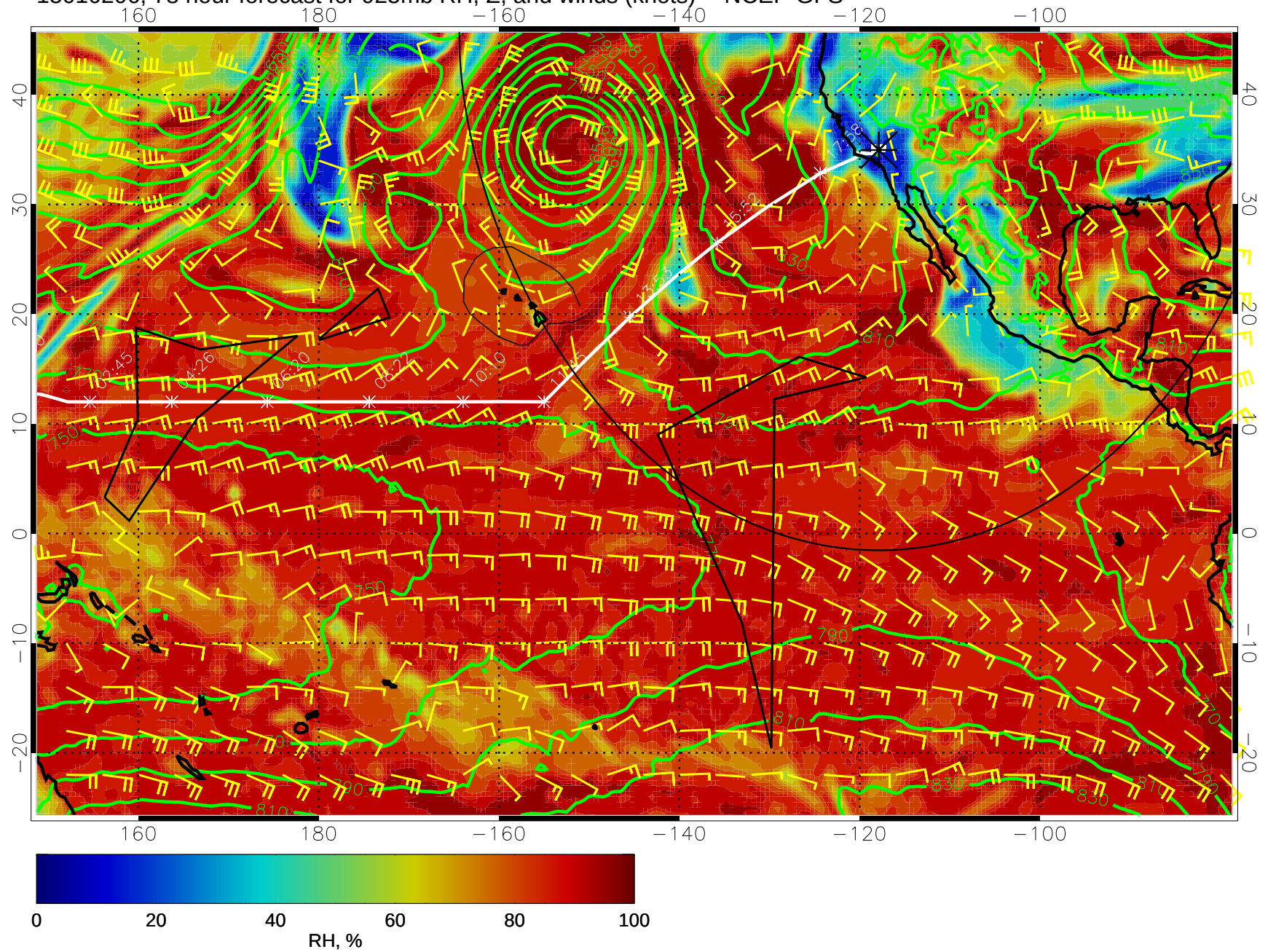
15010206, 78 hour forecast for 925mb RH, Z, and winds (knots) -- NCEP GFS
