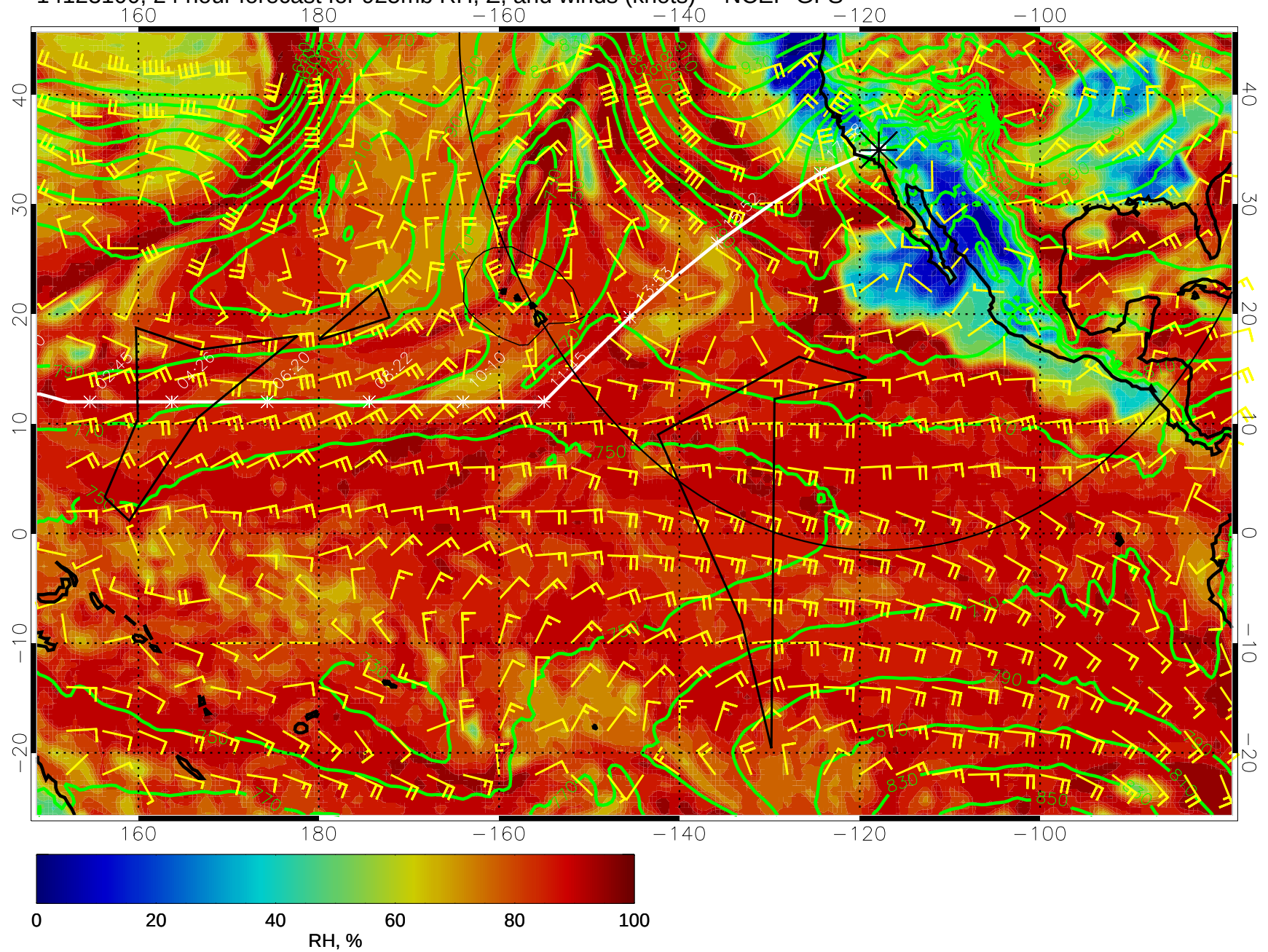
14123100, 24 hour forecast for 925mb RH, Z, and winds (knots) -- NCEP GFS
