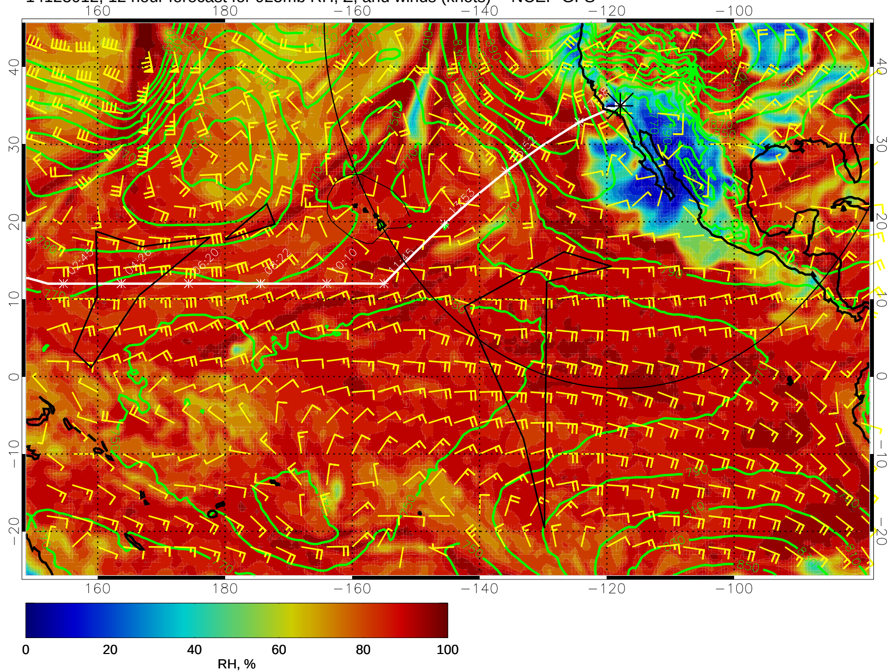
14123012, 12 hour forecast for 925mb RH, Z, and winds (knots) -- NCEP GFS
