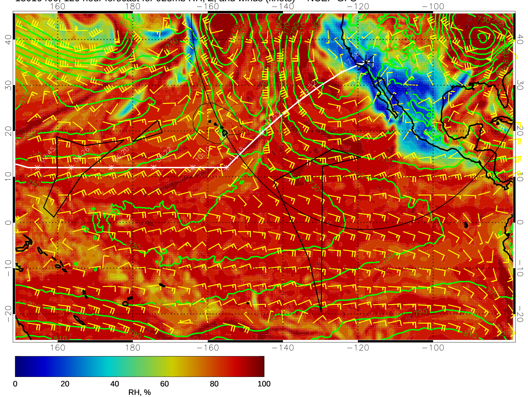
15010400, 120 hour forecast for 925mb RH, Z, and winds (knots) -- NCEP GFS
