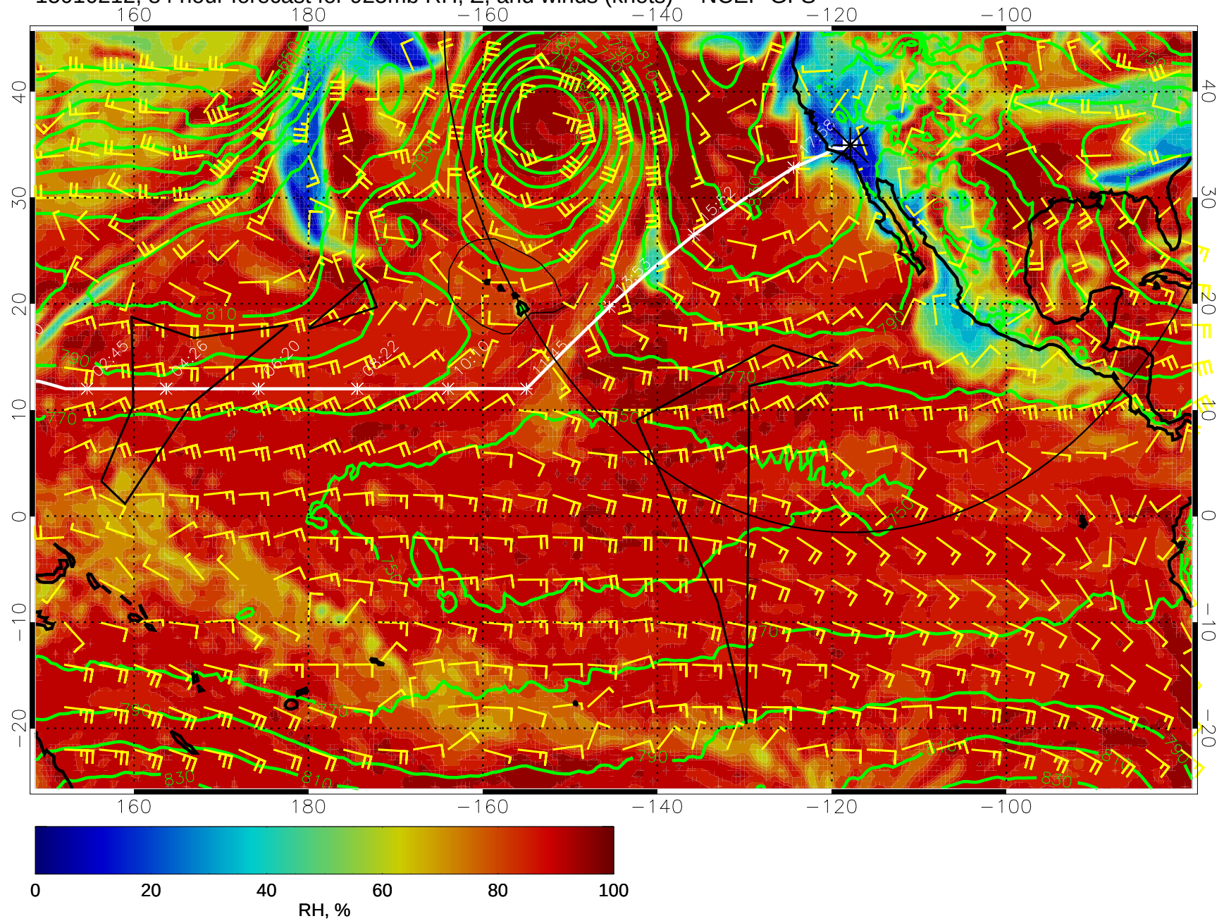
15010212, 84 hour forecast for 925mb RH, Z, and winds (knots) -- NCEP GFS
