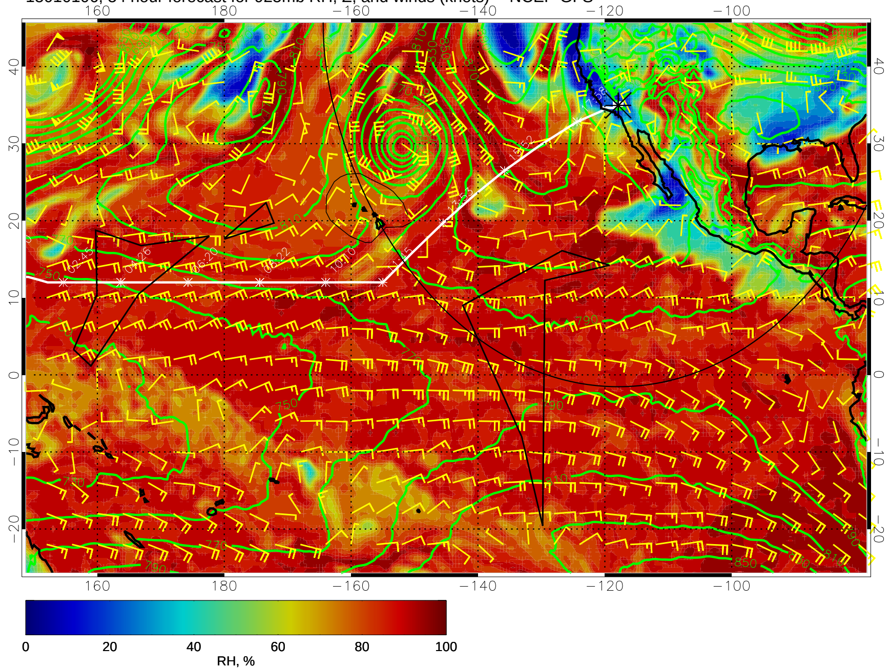
15010106, 54 hour forecast for 925mb RH, Z, and winds (knots) -- NCEP GFS
