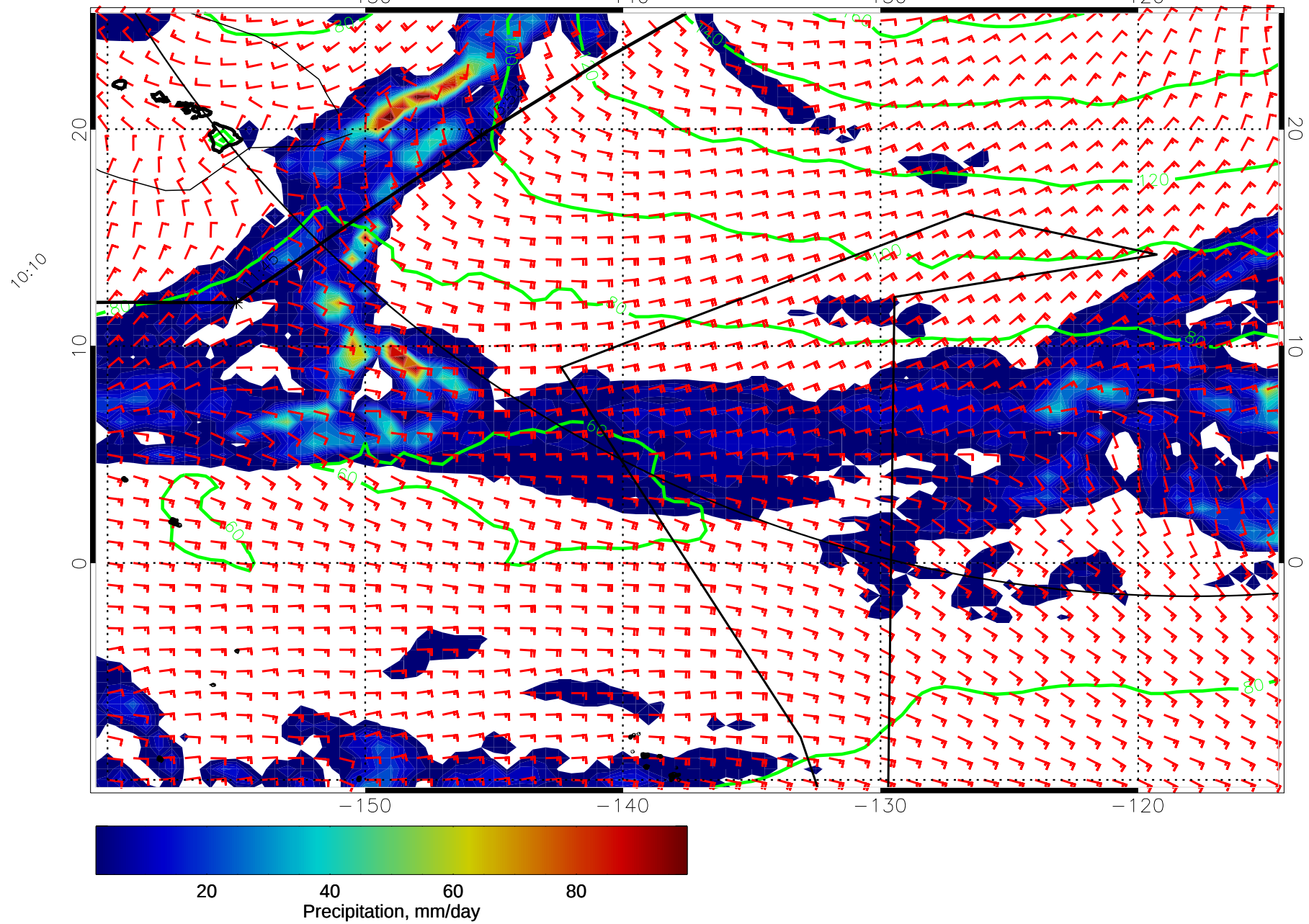
15010212, 84 hour forecast for precip, 1000mb Z, and winds (knots) -- NCEP GFS
