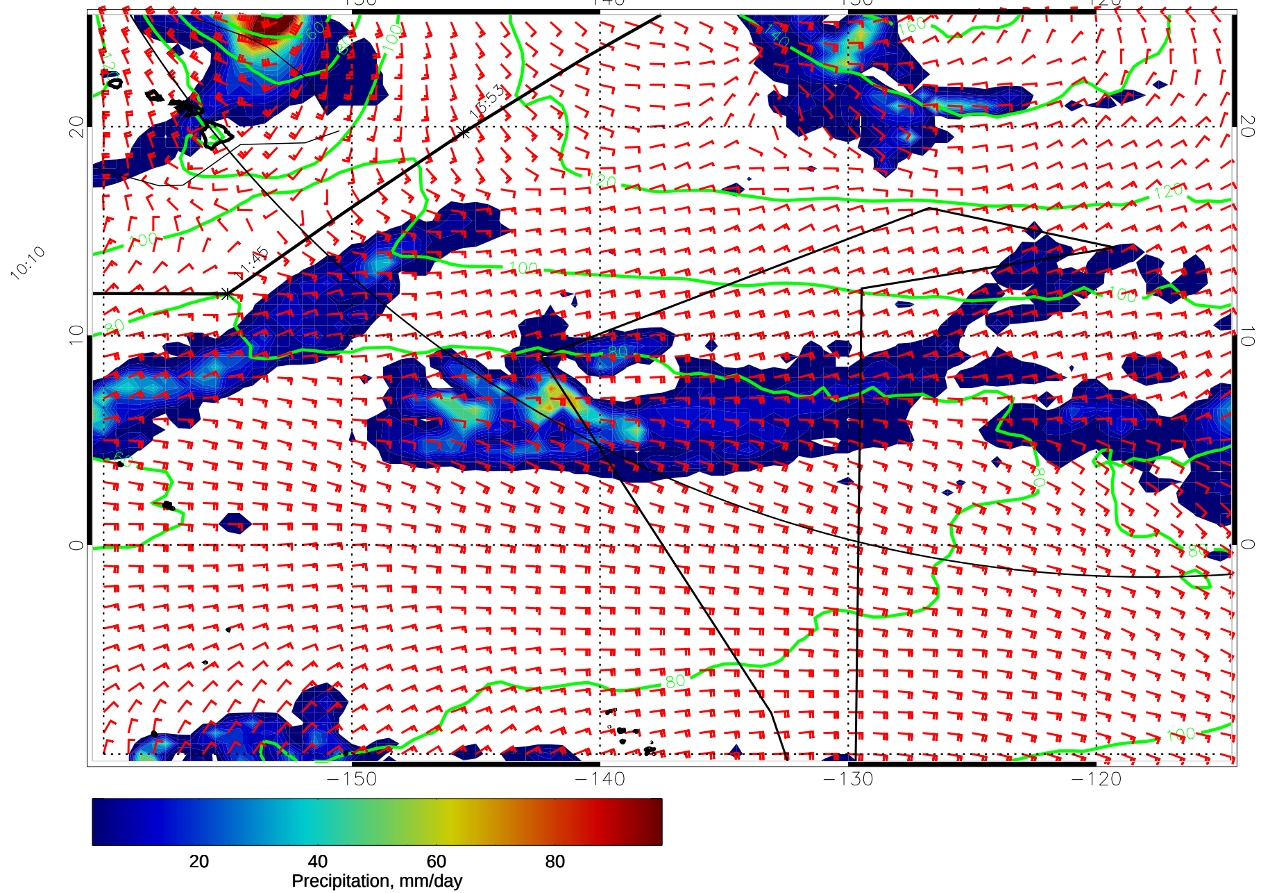
14123112, 36 hour forecast for precip, 1000mb Z, and winds (knots) -- NCEP GFS
