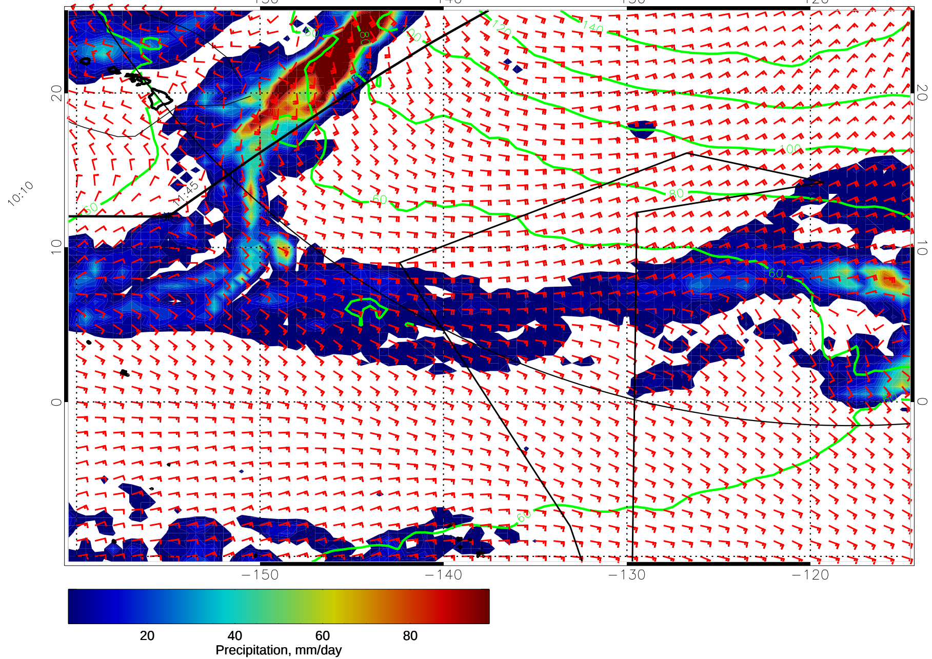
15010300, 96 hour forecast for precip, 1000mb Z, and winds (knots) -- NCEP GFS
