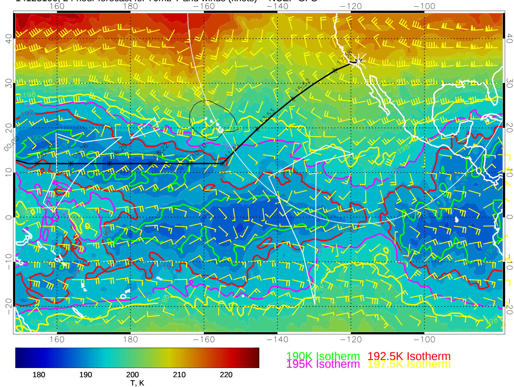
14123100, 24 hour forecast for 70mb T and winds (knots) -- NCEP GFS
