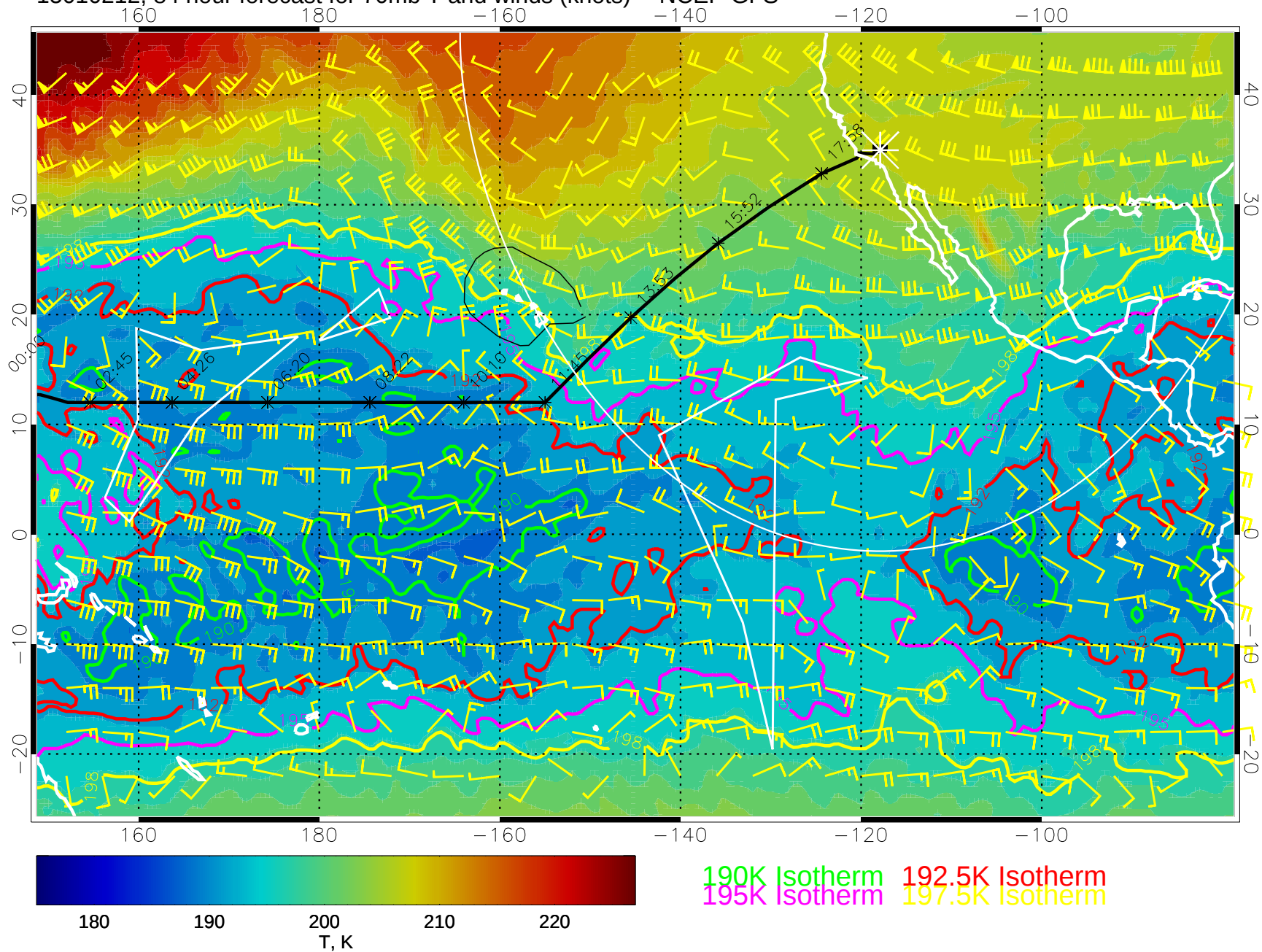
15010212, 84 hour forecast for 70mb T and winds (knots) -- NCEP GFS
