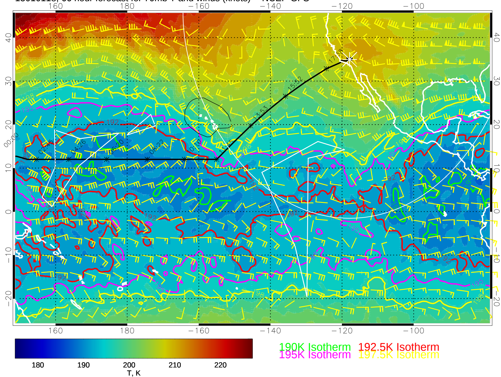
15010118, 66 hour forecast for 70mb T and winds (knots) -- NCEP GFS
