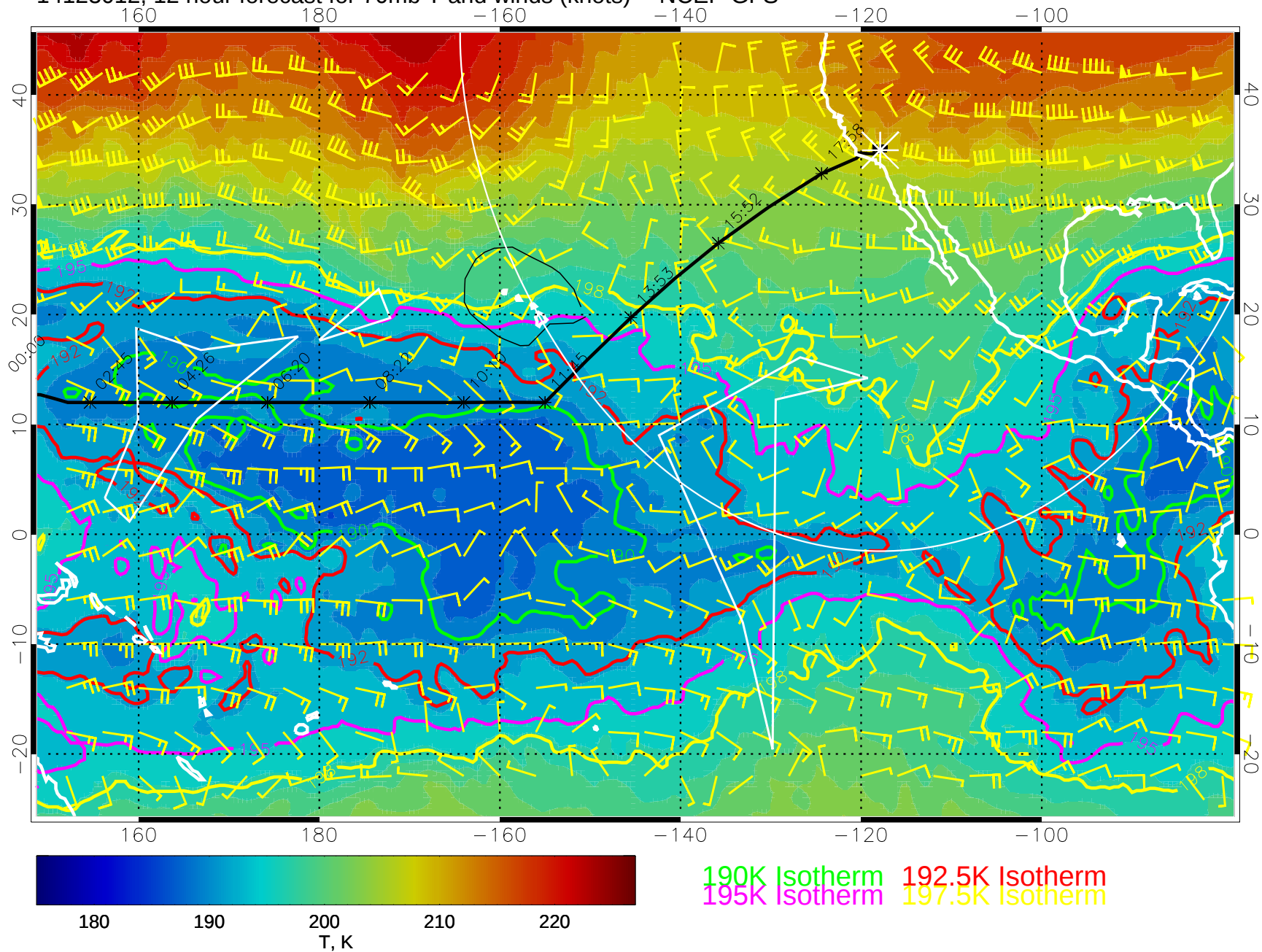
14123012, 12 hour forecast for 70mb T and winds (knots) -- NCEP GFS
