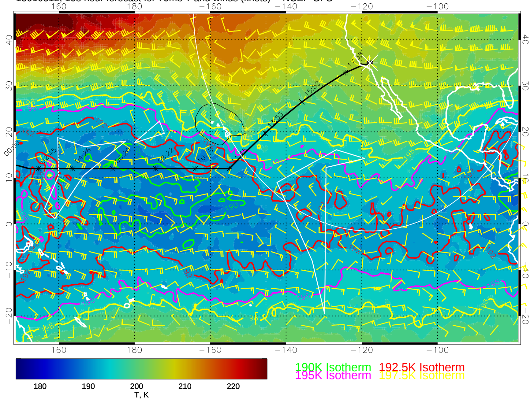
15010312, 108 hour forecast for 70mb T and winds (knots) -- NCEP GFS
