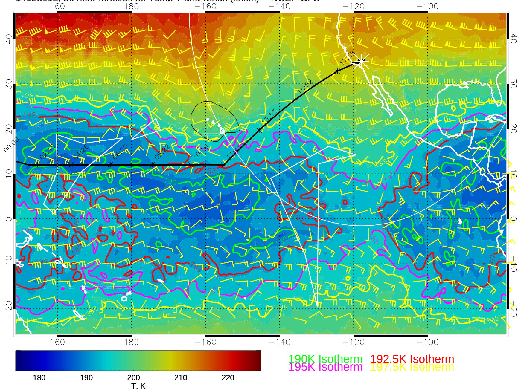
14123112, 36 hour forecast for 70mb T and winds (knots) -- NCEP GFS
