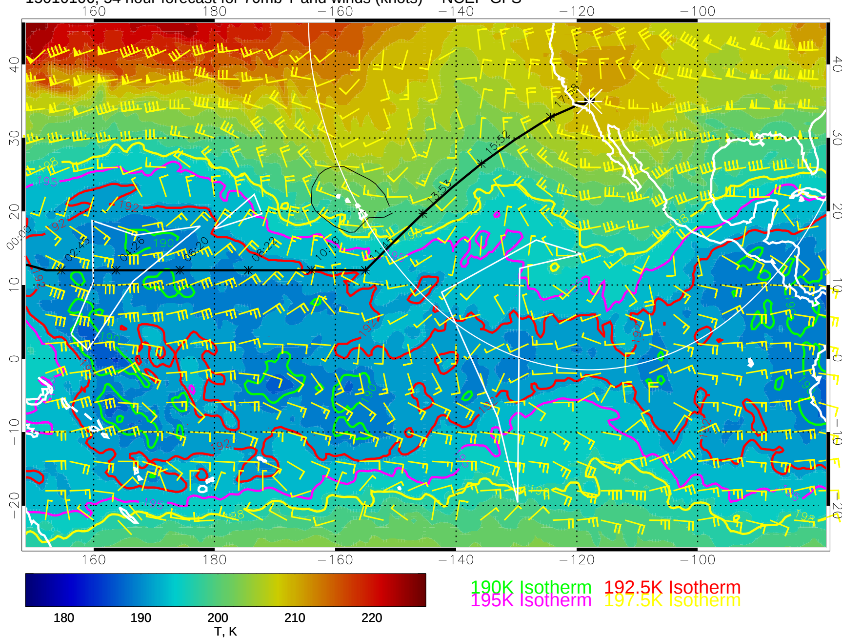
15010106, 54 hour forecast for 70mb T and winds (knots) -- NCEP GFS
