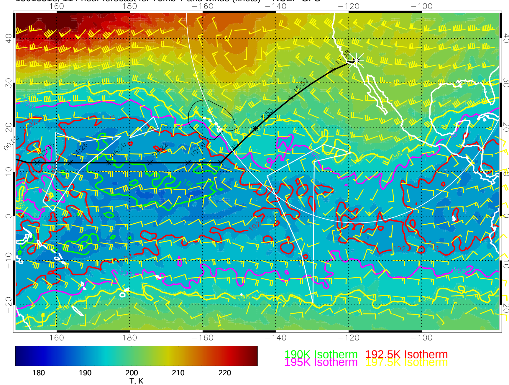
15010318, 114 hour forecast for 70mb T and winds (knots) -- NCEP GFS
