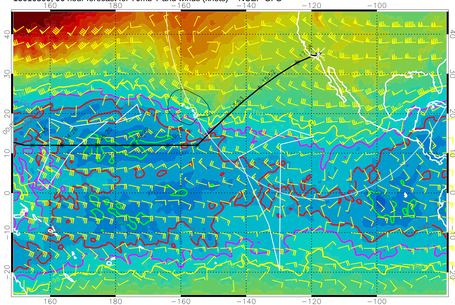
15010300, 96 hour forecast for 70mb T and winds (knots) -- NCEP GFS
