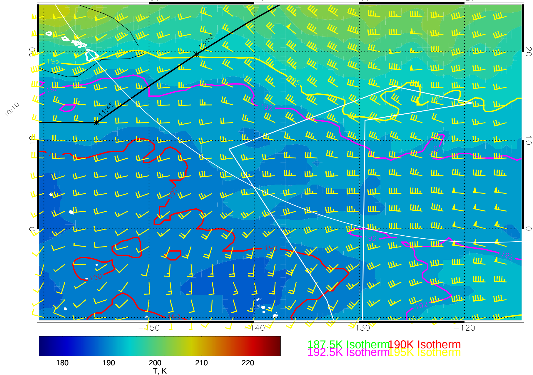
14123100, 24 hour forecast for 100mb T and winds (knots) -- NCEP GFS
