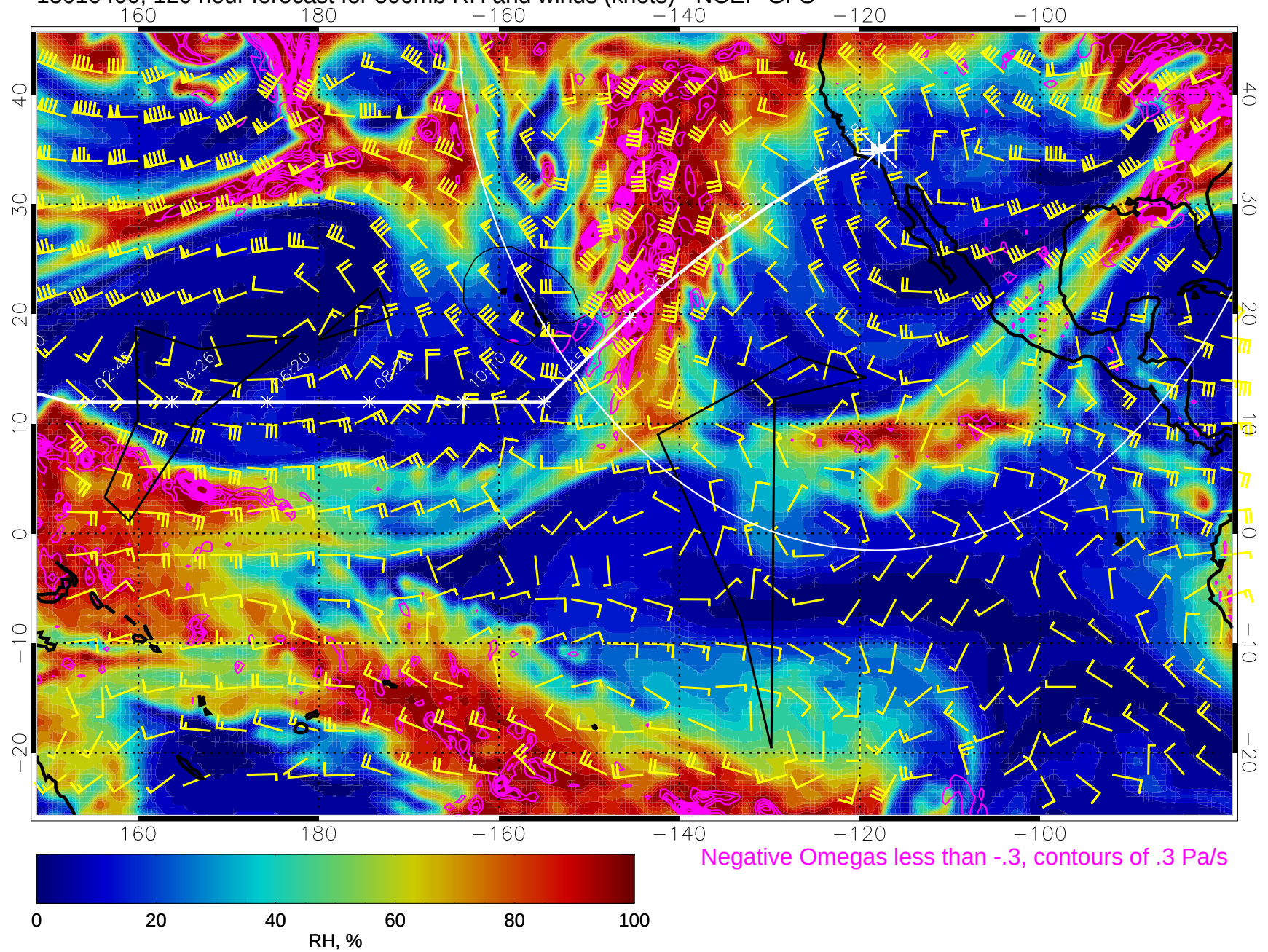
15010400, 120 hour forecast for 500mb RH and winds (knots) - NCEP GFS
