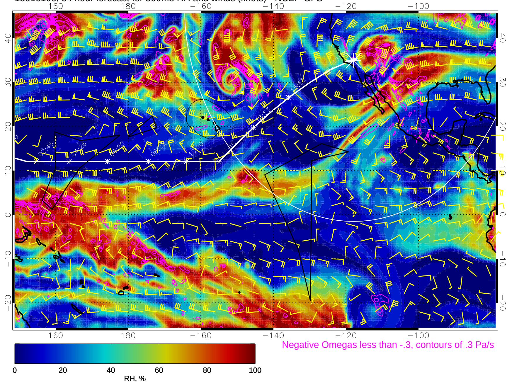
15010106, 54 hour forecast for 500mb RH and winds (knots) - NCEP GFS
