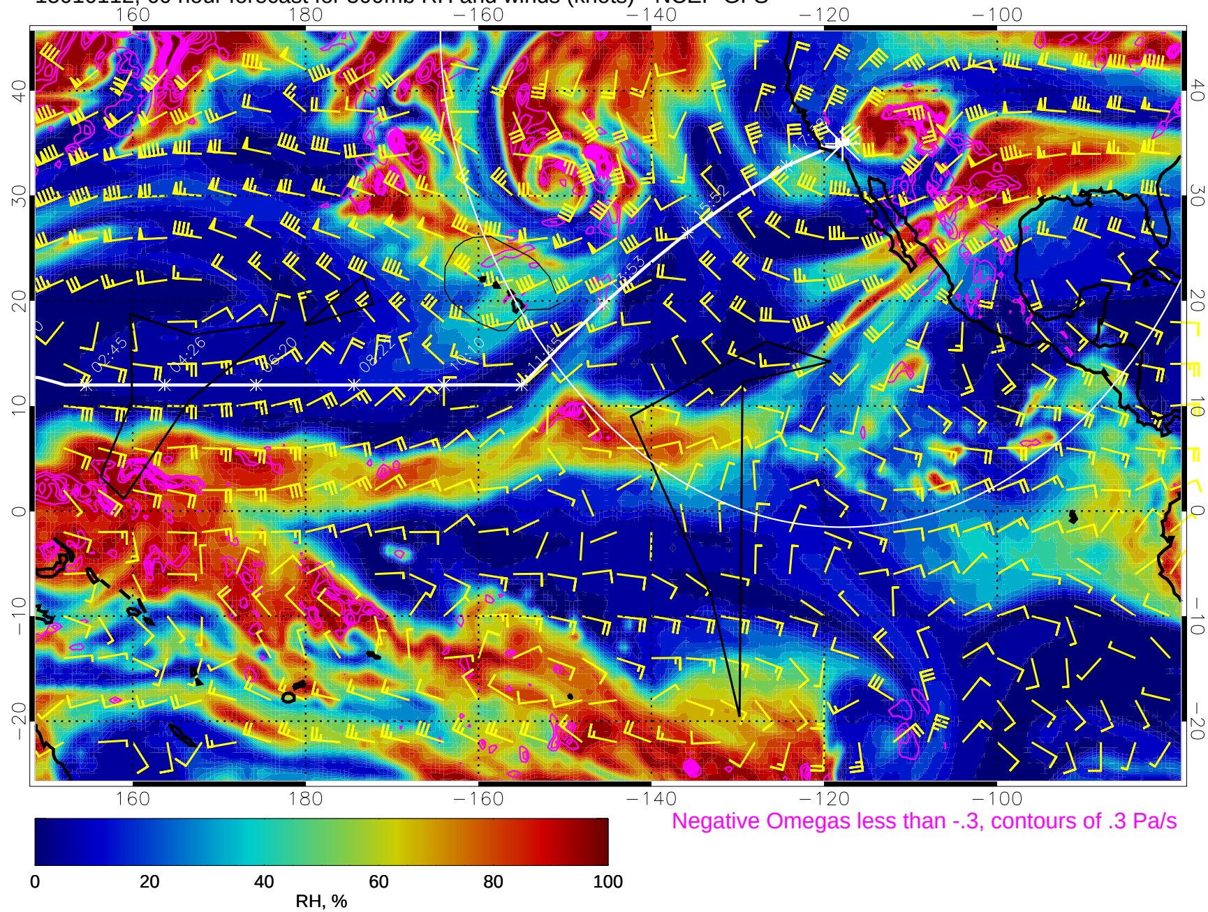
15010112, 60 hour forecast for 500mb RH and winds (knots) - NCEP GFS
