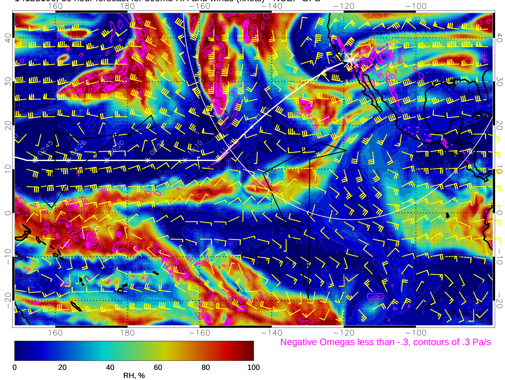
14123106, 30 hour forecast for 500mb RH and winds (knots) - NCEP GFS
