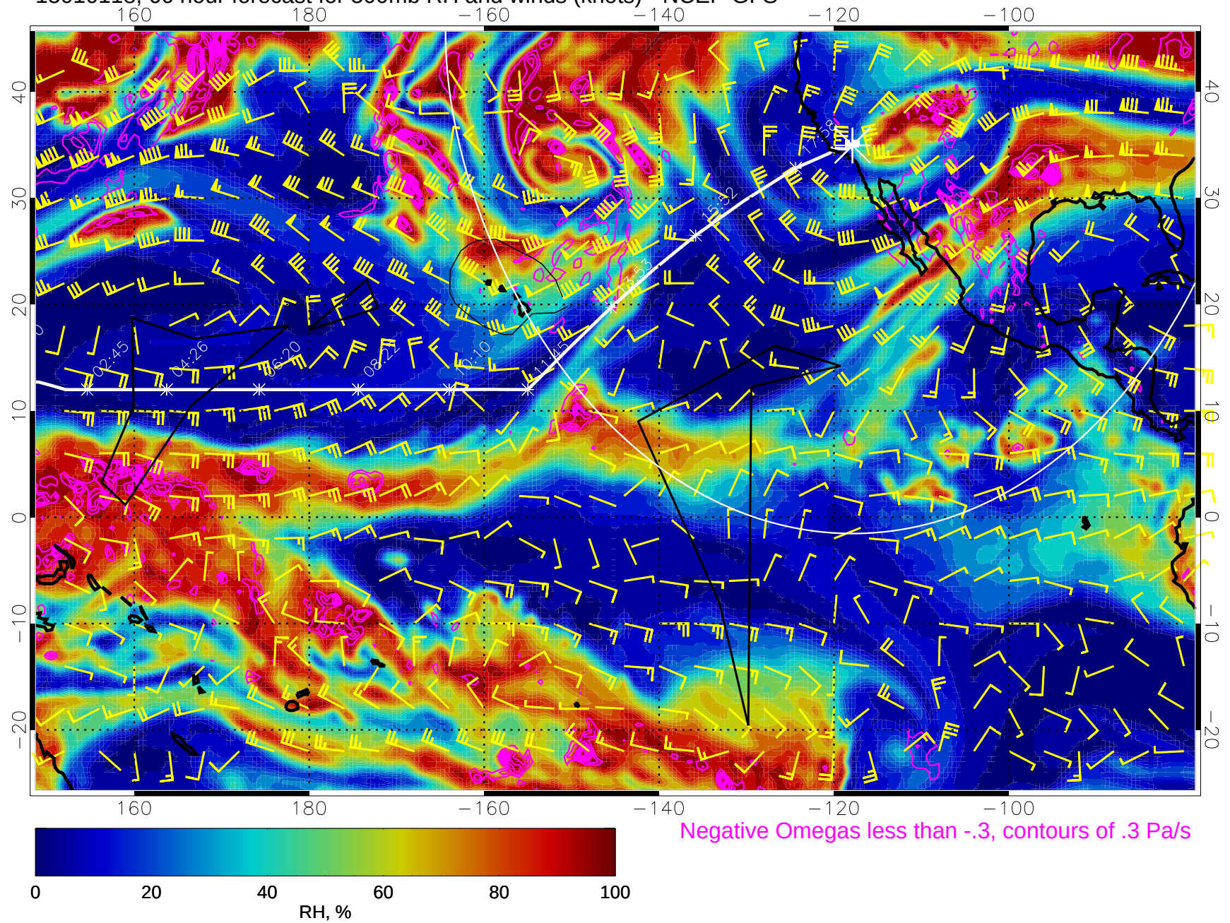
15010118, 66 hour forecast for 500mb RH and winds (knots) - NCEP GFS
