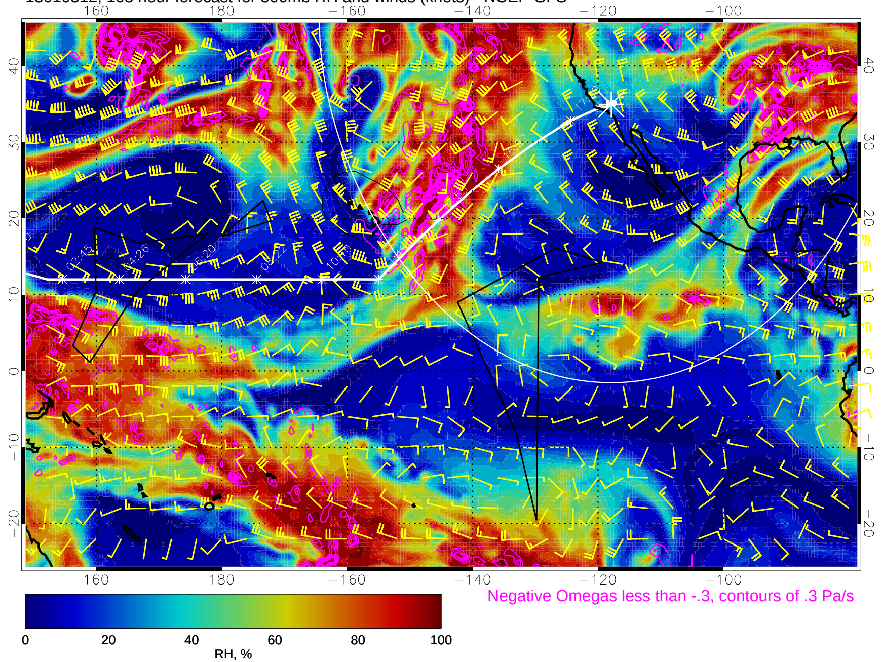
15010312, 108 hour forecast for 500mb RH and winds (knots) - NCEP GFS
