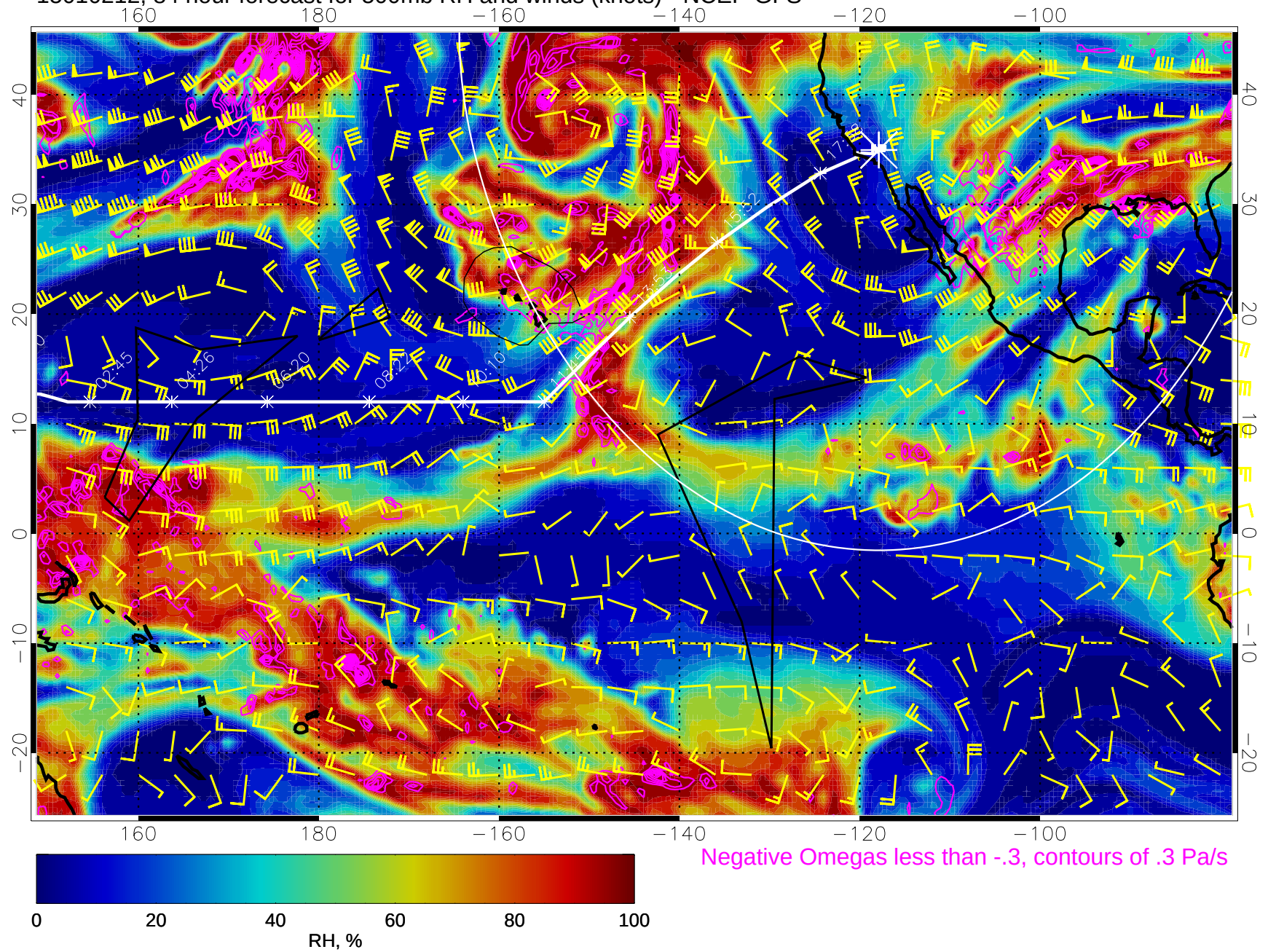
15010212, 84 hour forecast for 500mb RH and winds (knots) - NCEP GFS
