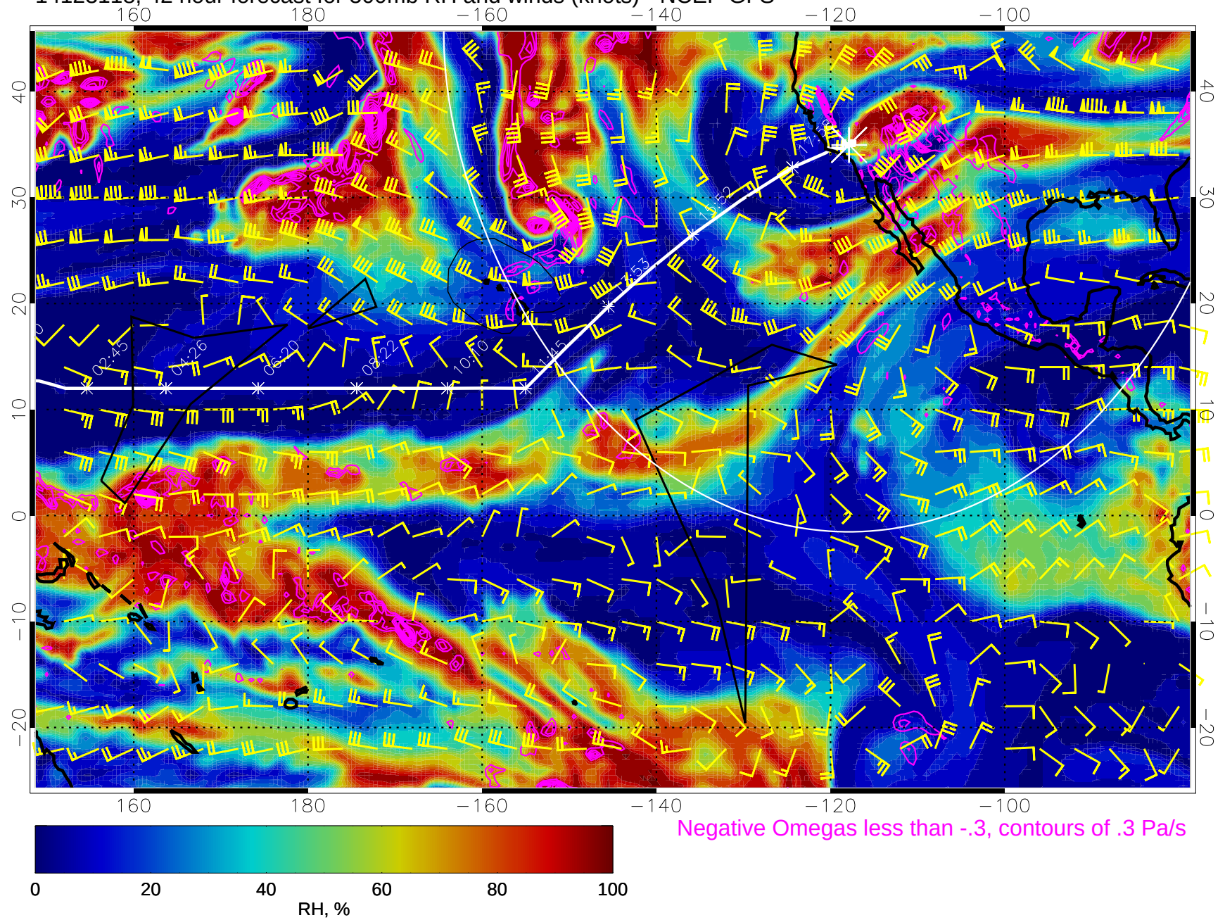
14123118, 42 hour forecast for 500mb RH and winds (knots) - NCEP GFS
