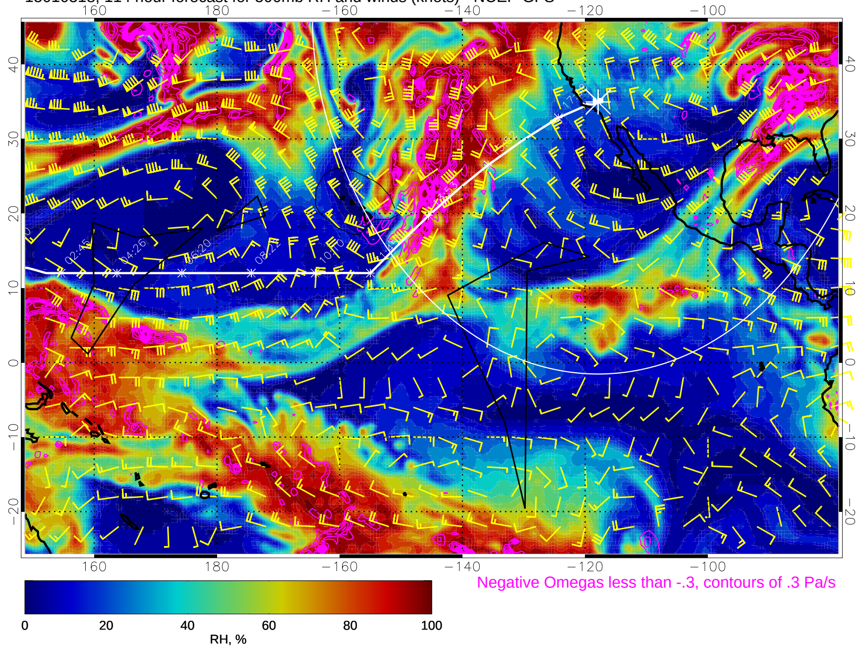
15010318, 114 hour forecast for 500mb RH and winds (knots) - NCEP GFS
