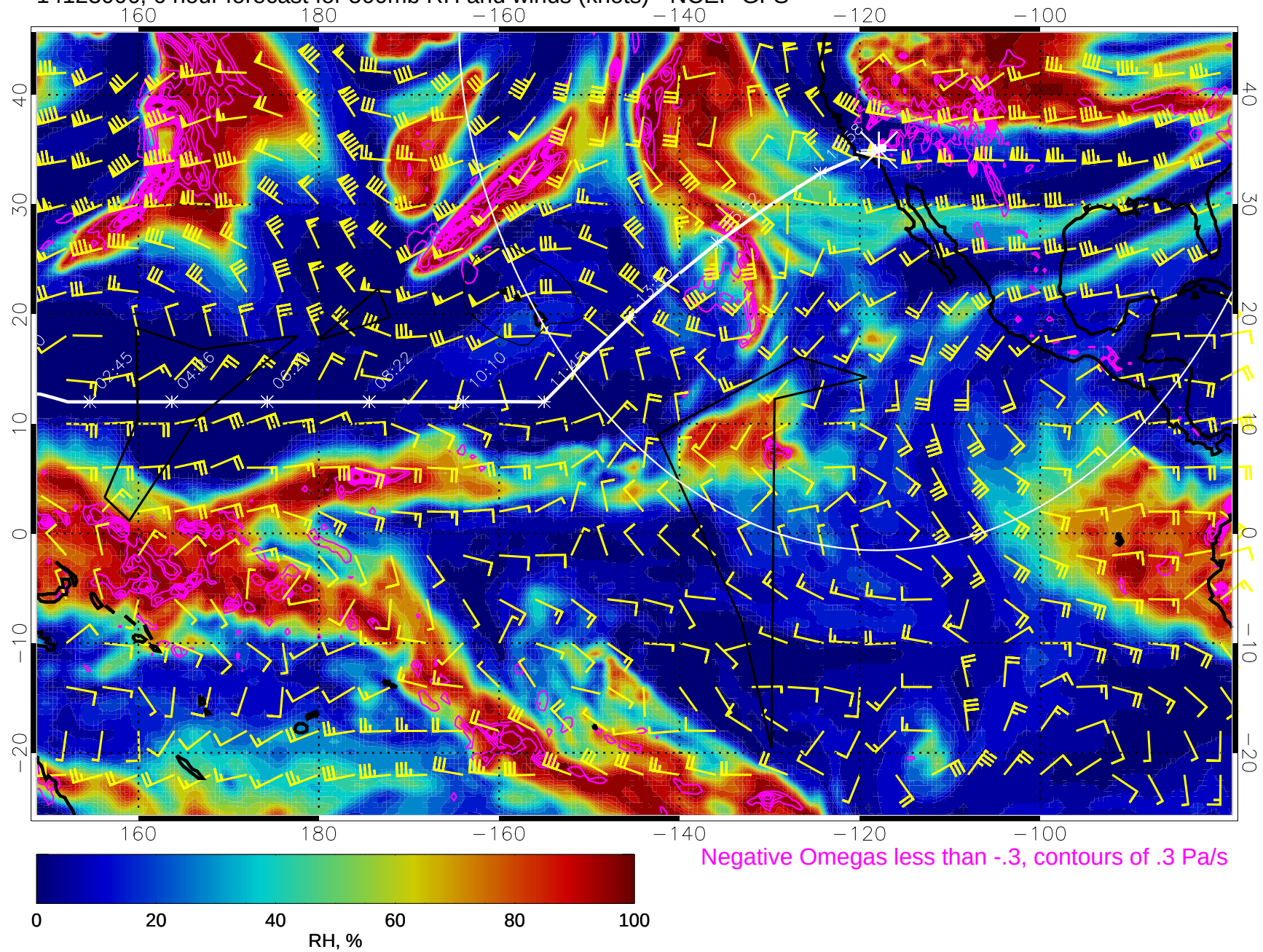
14123006, 6 hour forecast for 500mb RH and winds (knots) - NCEP GFS
