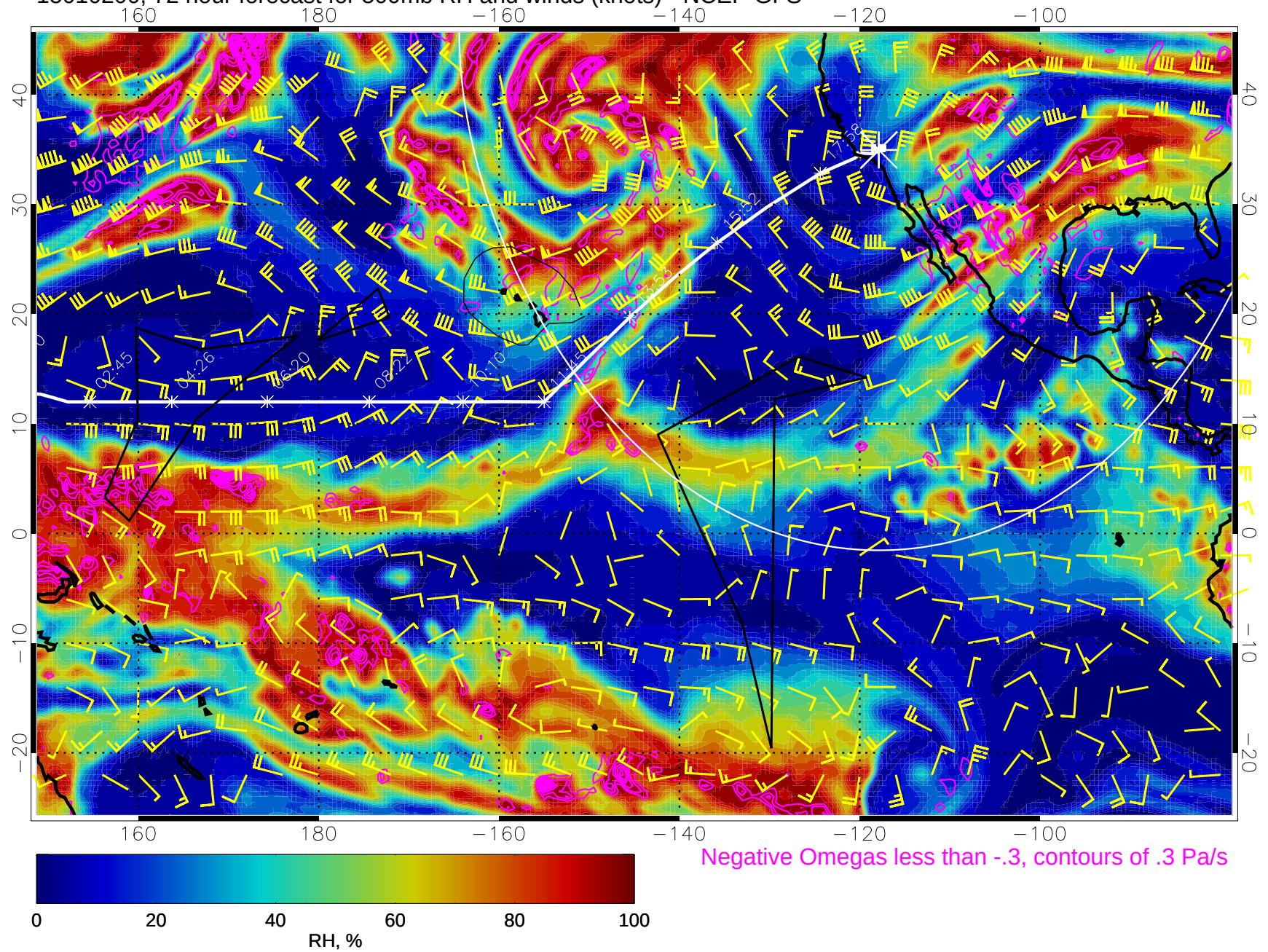
15010200, 72 hour forecast for 500mb RH and winds (knots) - NCEP GFS
