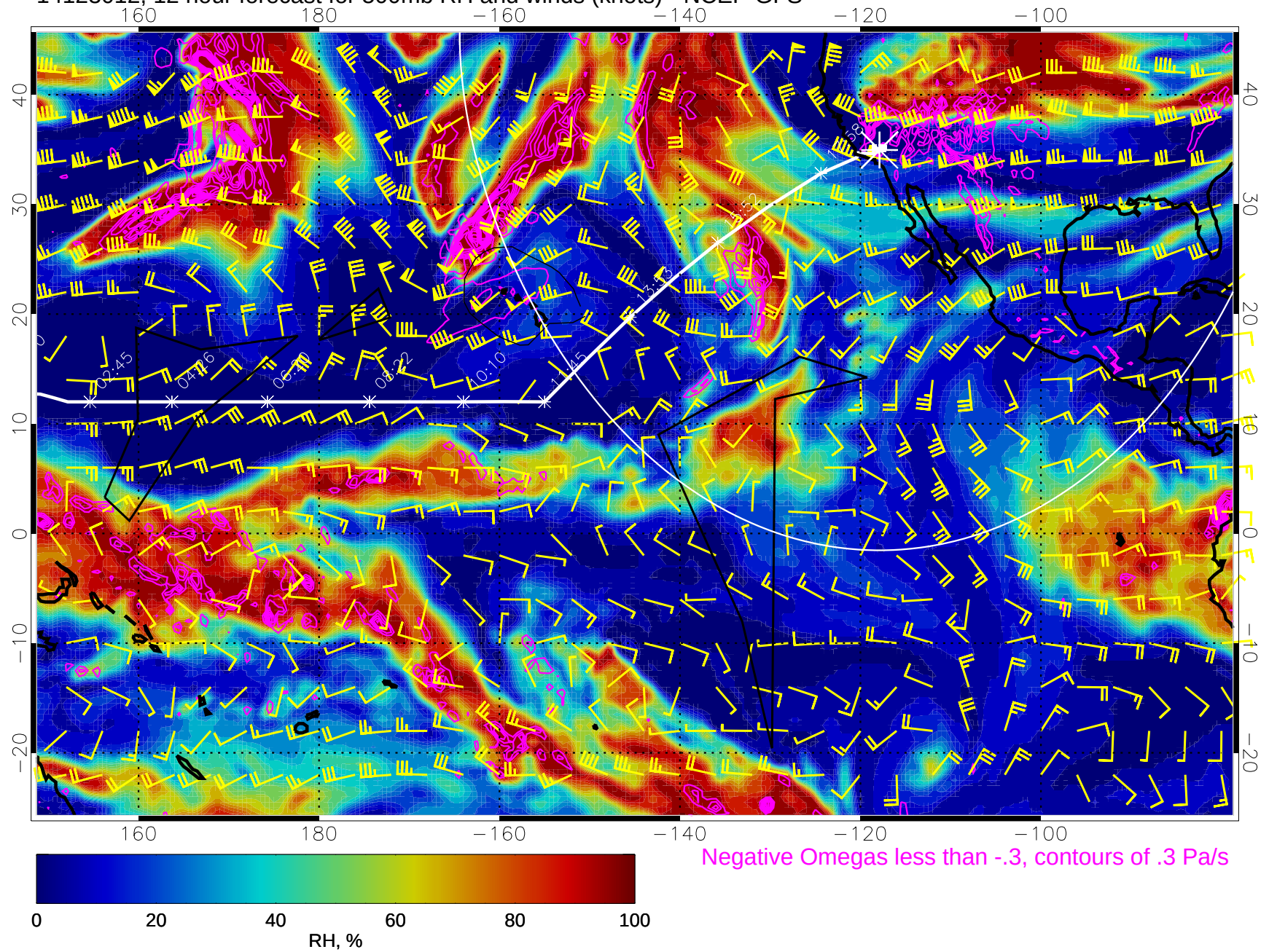
14123012, 12 hour forecast for 500mb RH and winds (knots) - NCEP GFS
