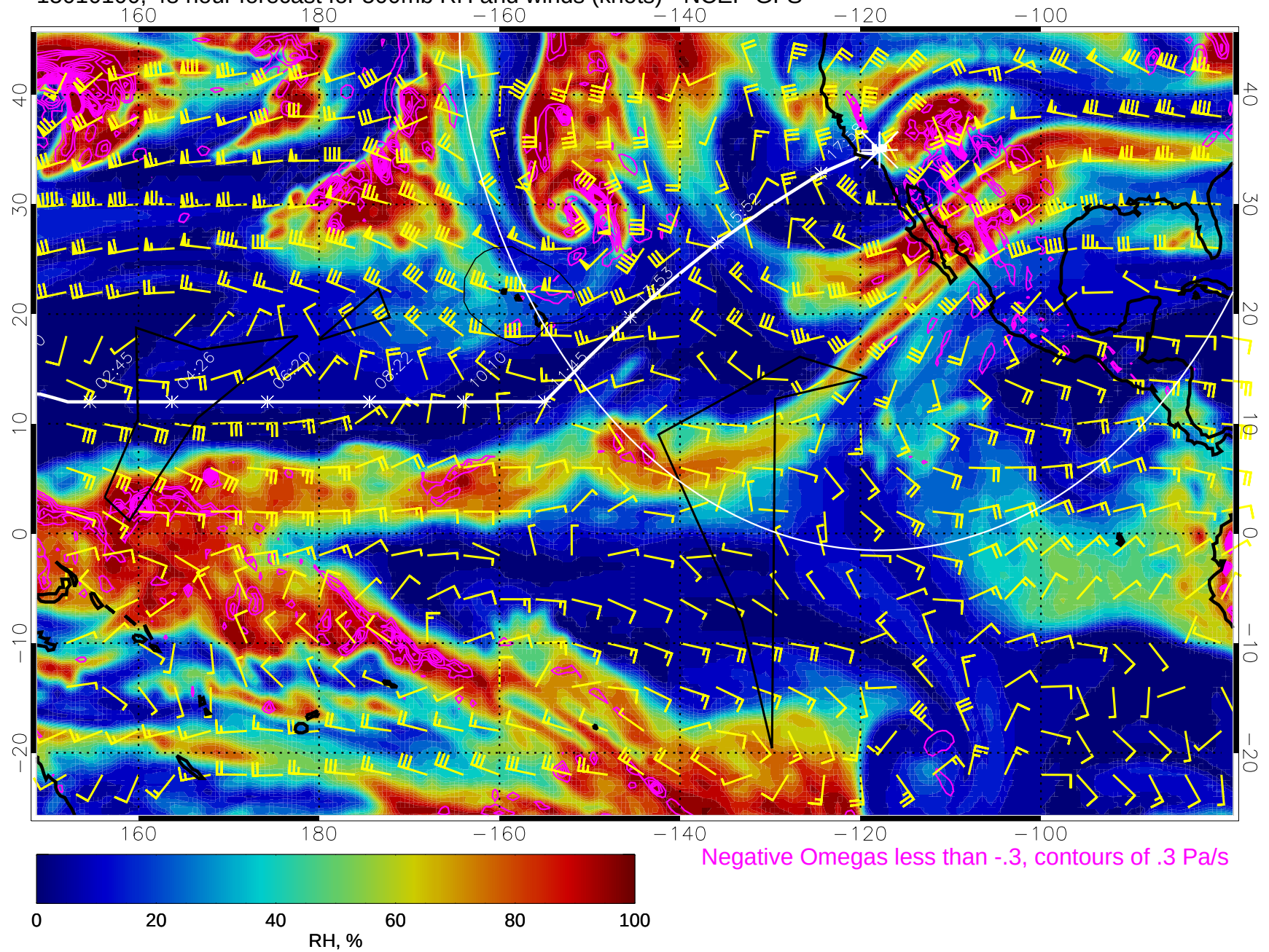
15010100, 48 hour forecast for 500mb RH and winds (knots) - NCEP GFS
