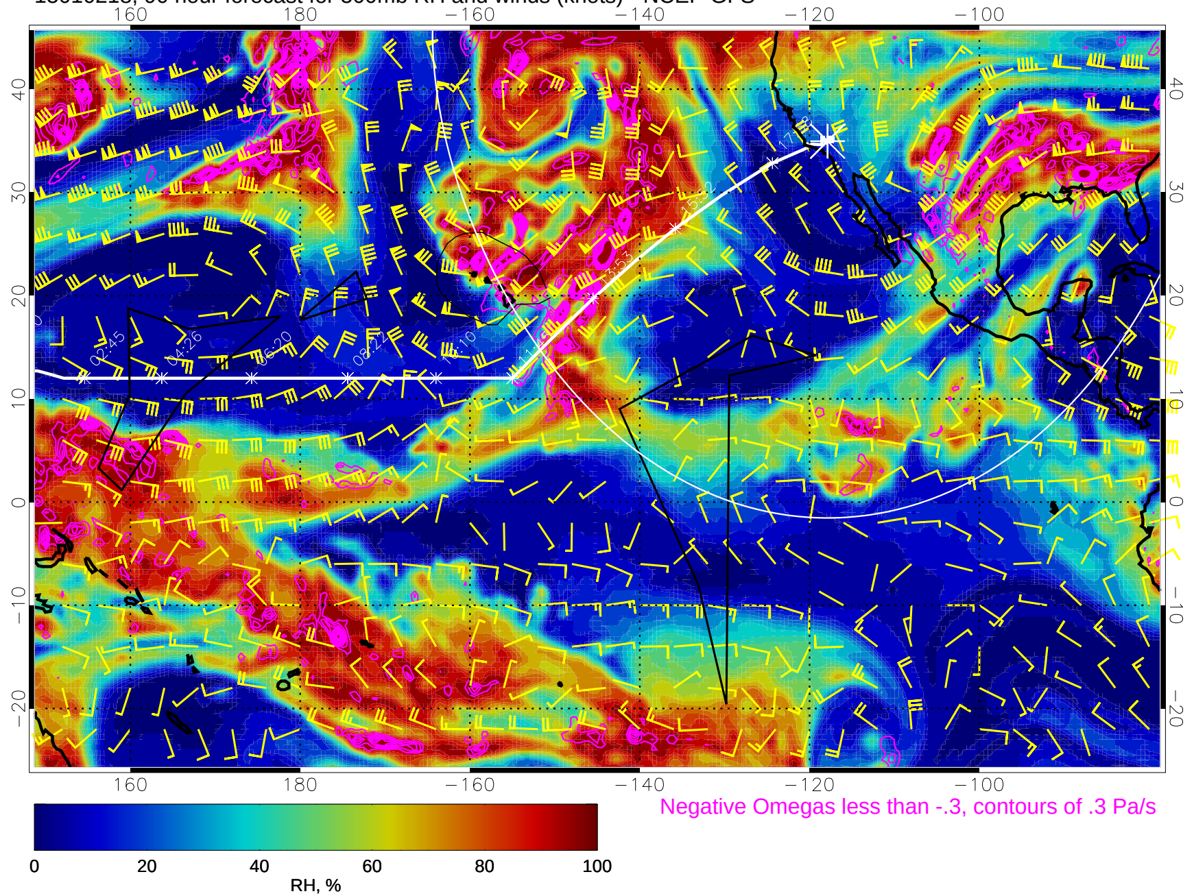
15010218, 90 hour forecast for 500mb RH and winds (knots) - NCEP GFS
