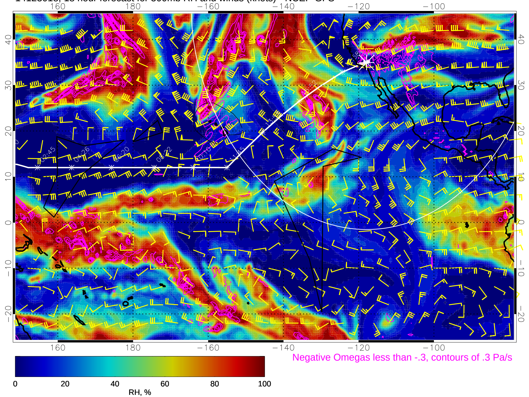
14123018, 18 hour forecast for 500mb RH and winds (knots) - NCEP GFS
