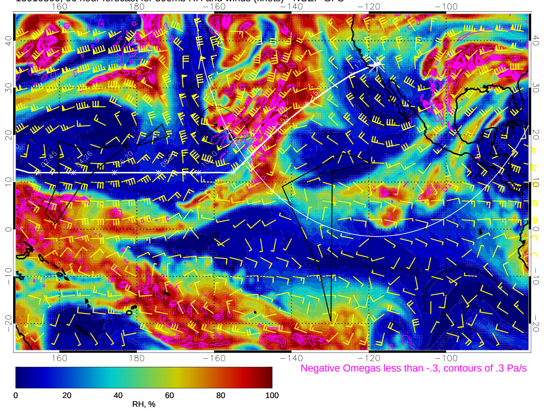
15010300, 96 hour forecast for 500mb RH and winds (knots) - NCEP GFS
