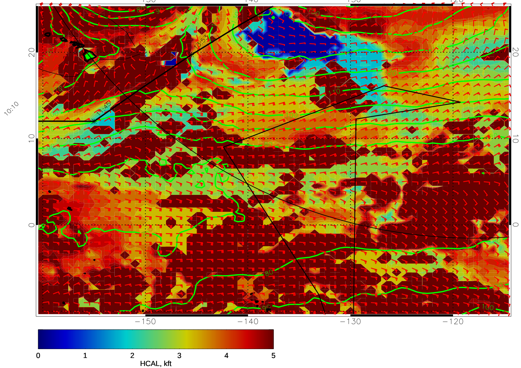
15010112, 60 hour forecast for HCAL, 1000mb Z, and winds (knots) -- NCEP GFS
