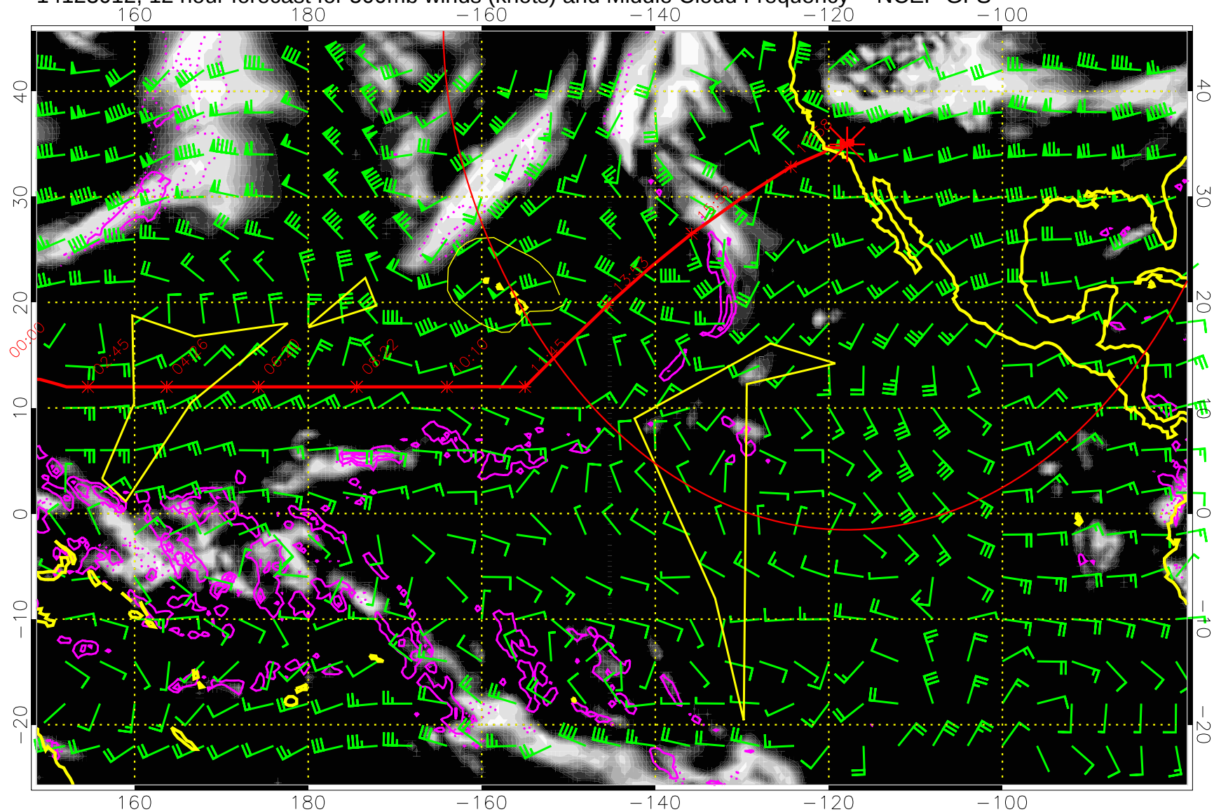
14123012, 12 hour forecast for 500mb winds (knots) and Middle Cloud Frequency -- NCEP GFS
