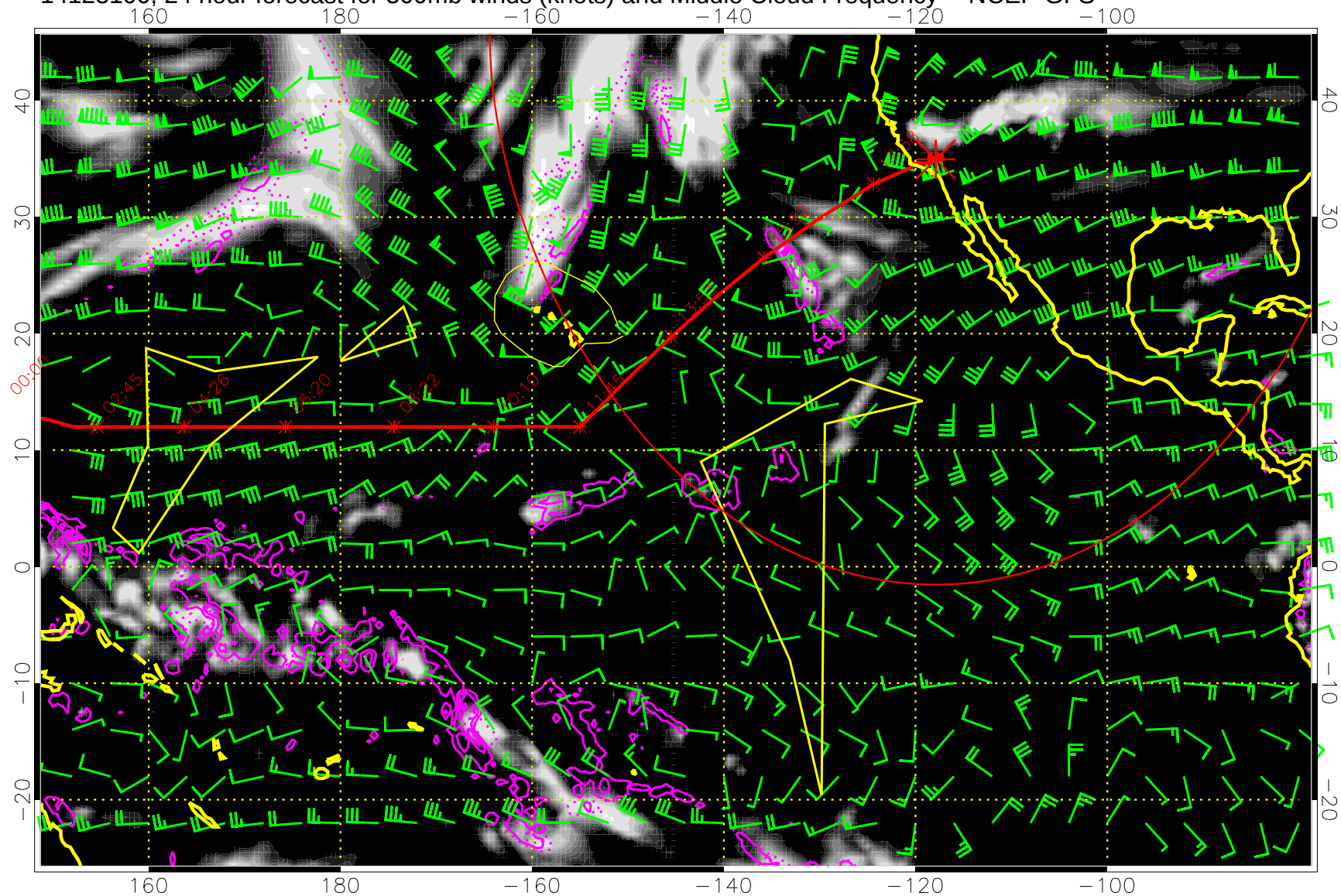
14123100, 24 hour forecast for 500mb winds (knots) and Middle Cloud Frequency -- NCEP GFS
