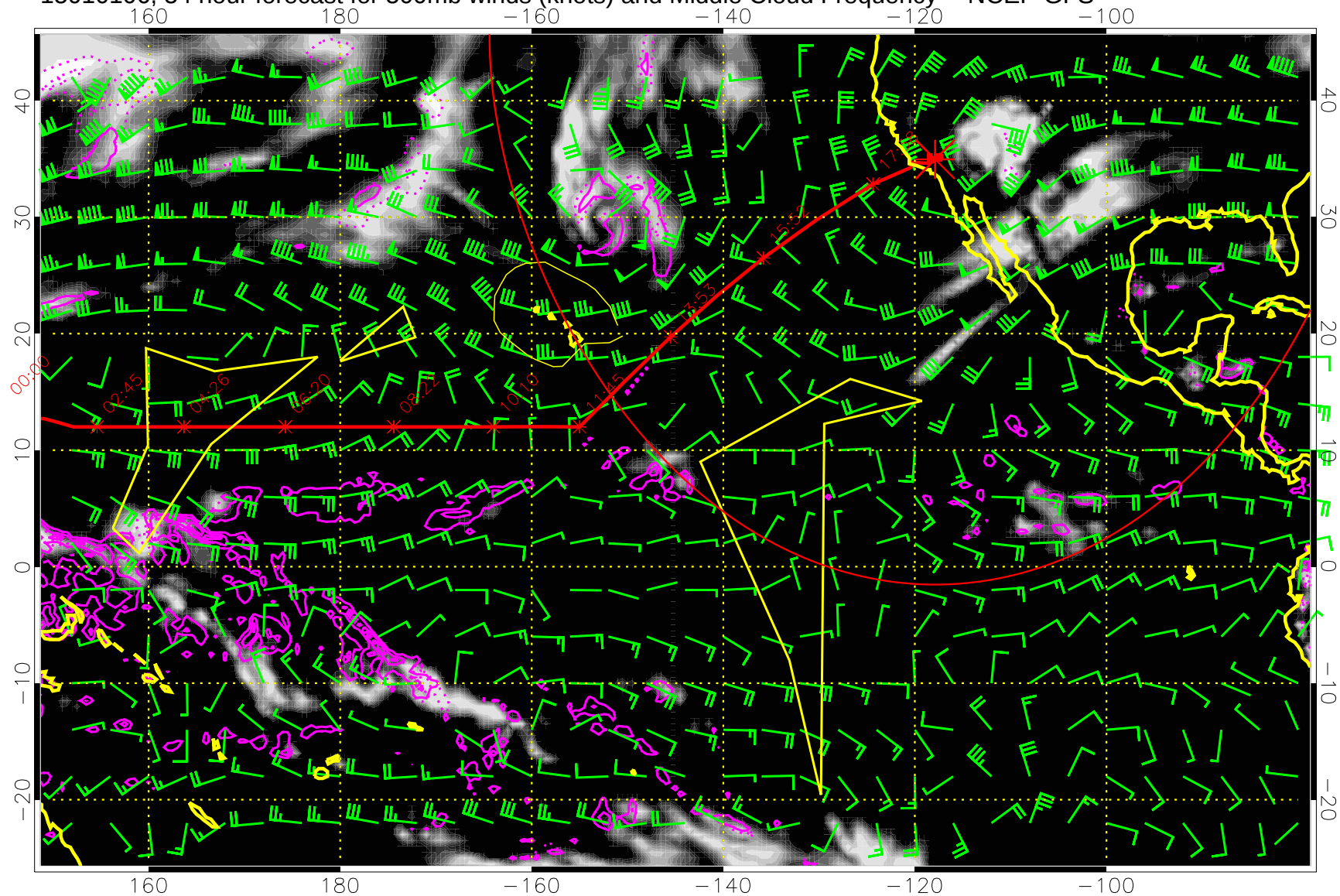
15010106, 54 hour forecast for 500mb winds (knots) and Middle Cloud Frequency -- NCEP GFS
