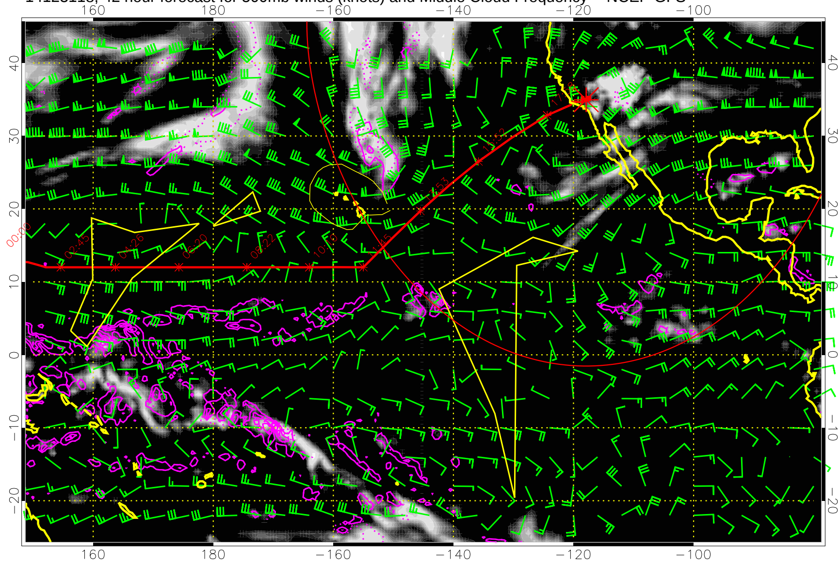
14123118, 42 hour forecast for 500mb winds (knots) and Middle Cloud Frequency -- NCEP GFS
