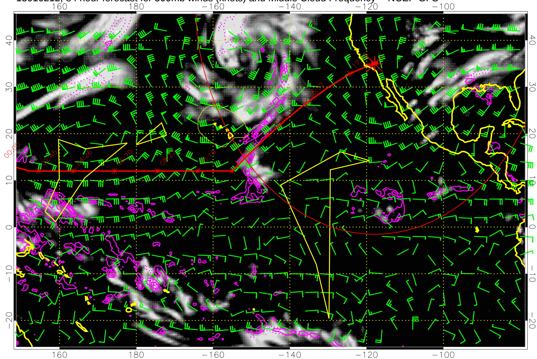
15010212, 84 hour forecast for 500mb winds (knots) and Middle Cloud Frequency -- NCEP GFS
