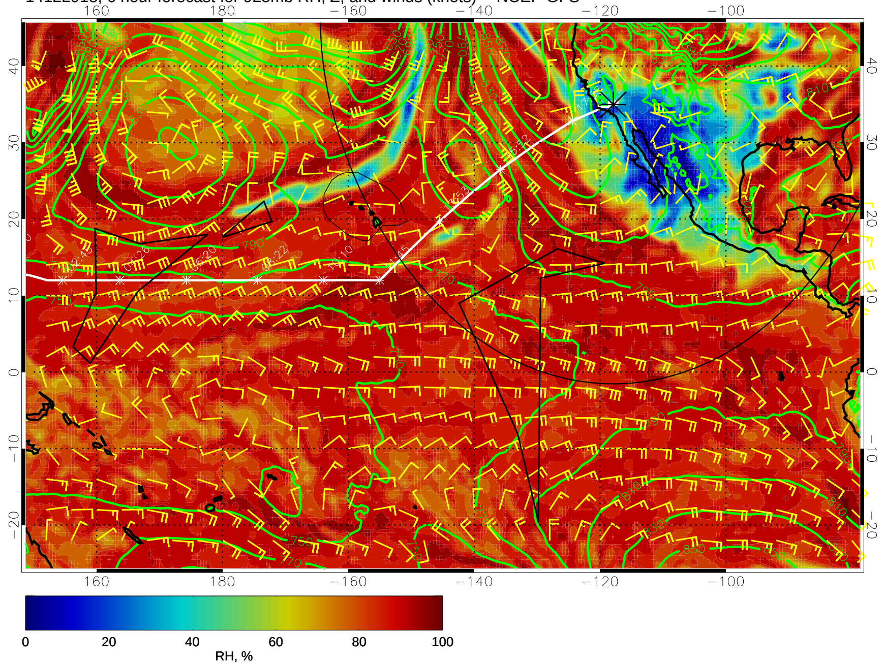
14122918, 6 hour forecast for 925mb RH, Z, and winds (knots) -- NCEP GFS
