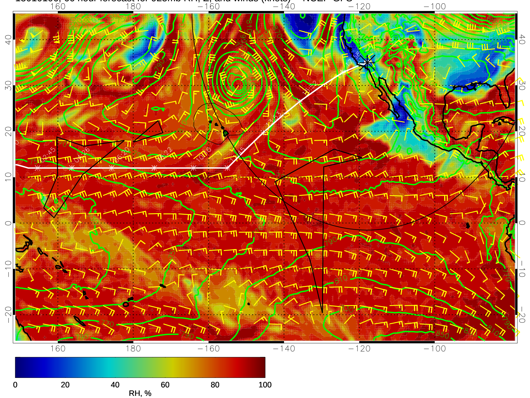
15010106, 66 hour forecast for 925mb RH, Z, and winds (knots) -- NCEP GFS
