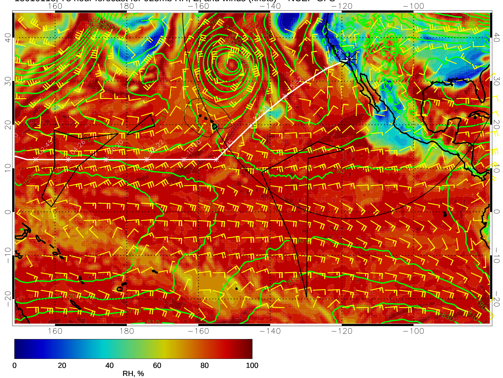
15010118, 78 hour forecast for 925mb RH, Z, and winds (knots) -- NCEP GFS
