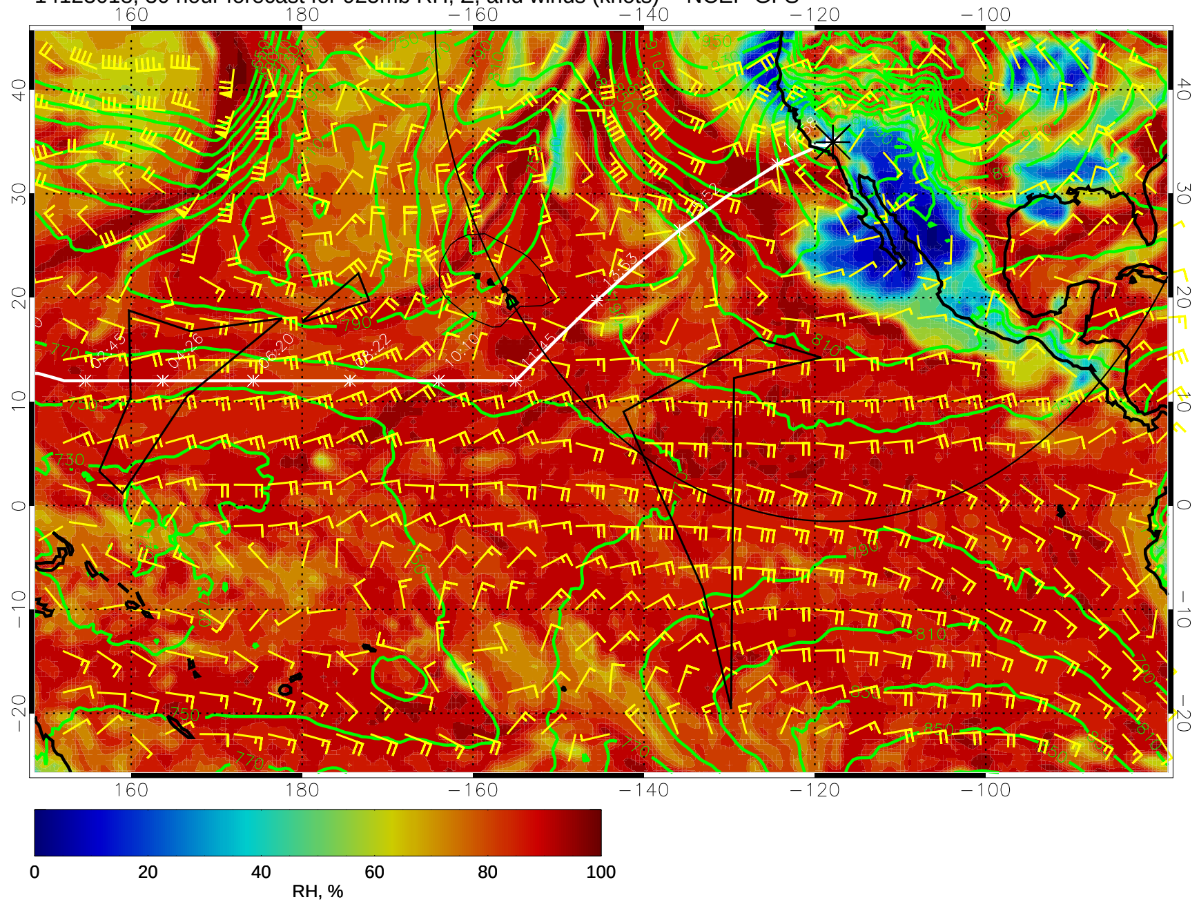
14123018, 30 hour forecast for 925mb RH, Z, and winds (knots) -- NCEP GFS
