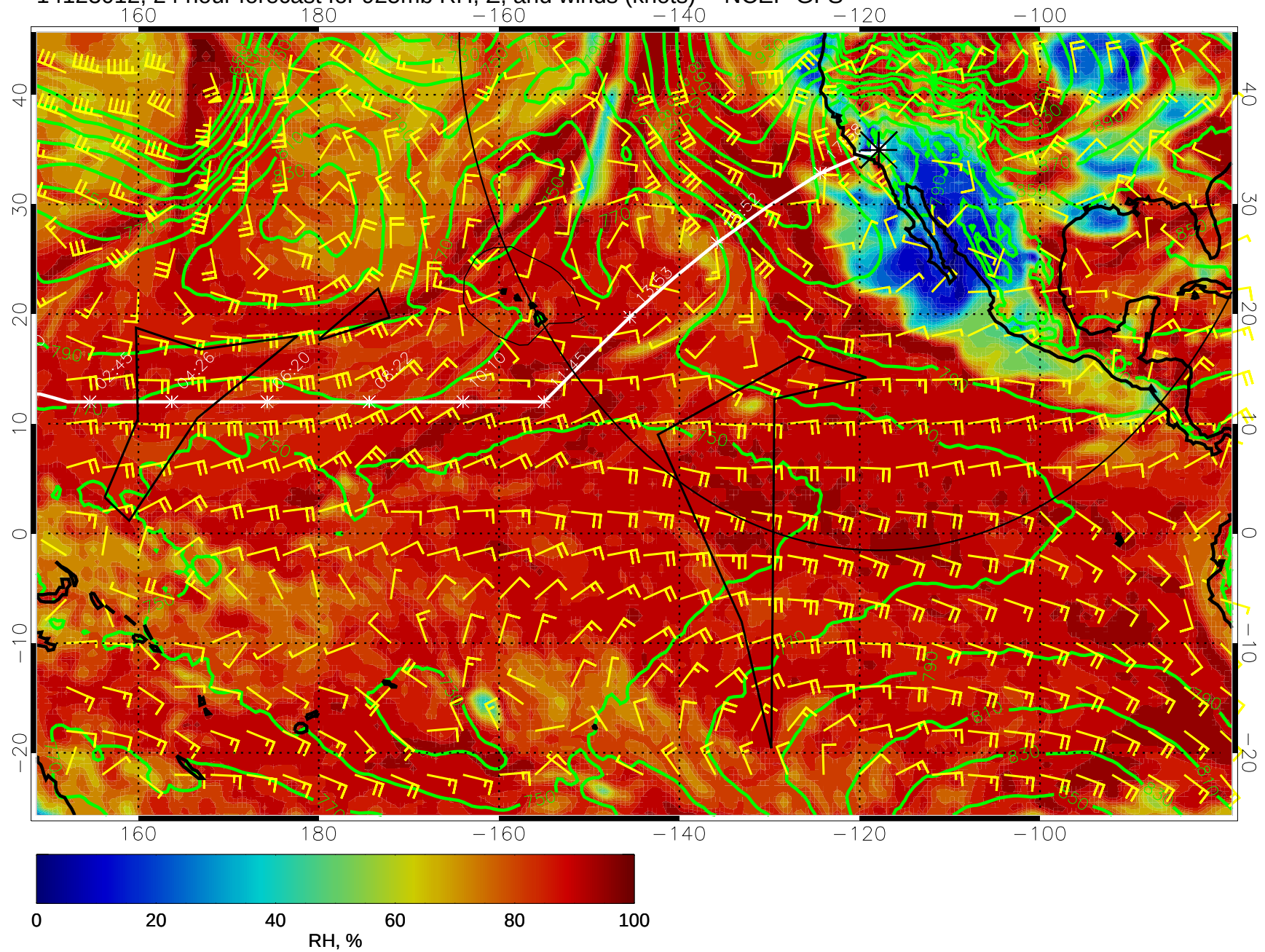
14123012, 24 hour forecast for 925mb RH, Z, and winds (knots) -- NCEP GFS
