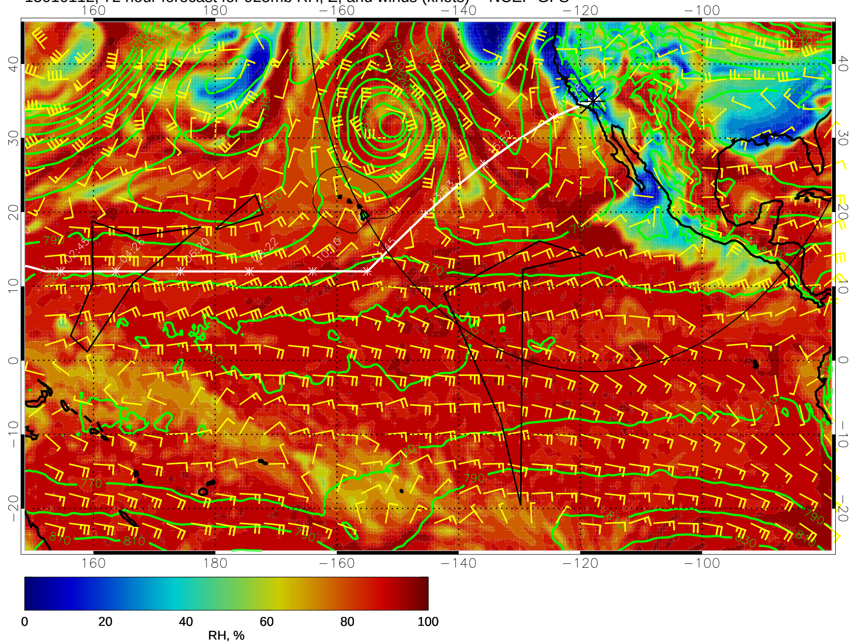
15010112, 72 hour forecast for 925mb RH, Z, and winds (knots) -- NCEP GFS
