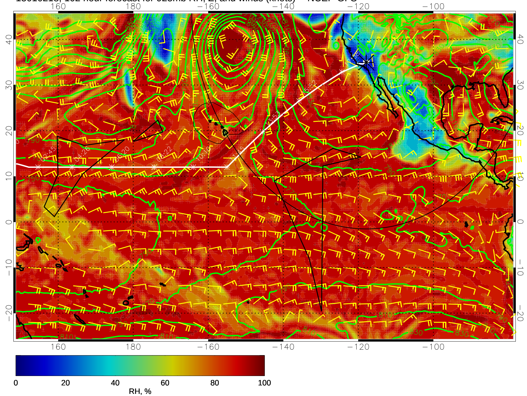
15010218, 102 hour forecast for 925mb RH, Z, and winds (knots) -- NCEP GFS
