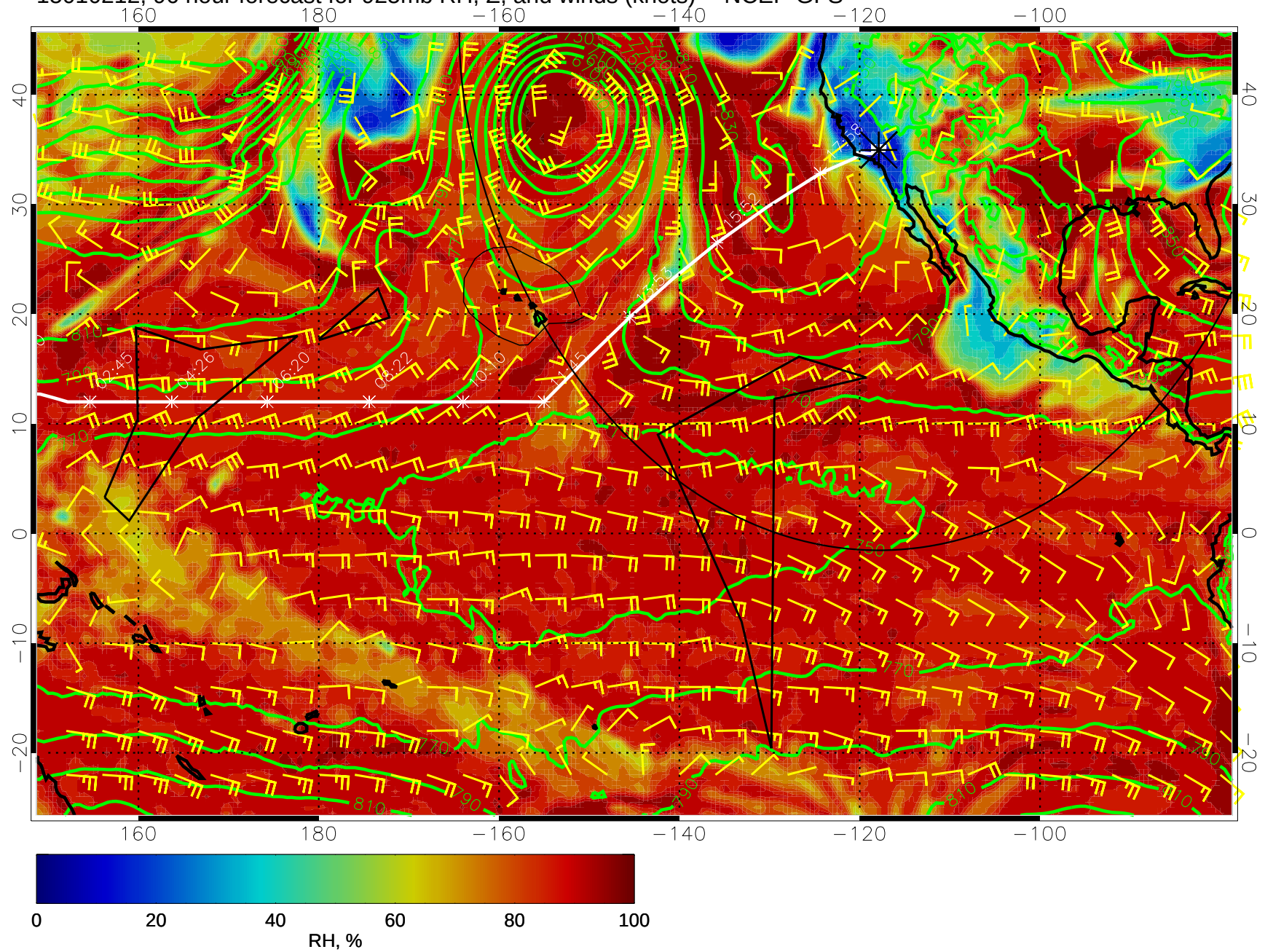
15010212, 96 hour forecast for 925mb RH, Z, and winds (knots) -- NCEP GFS
