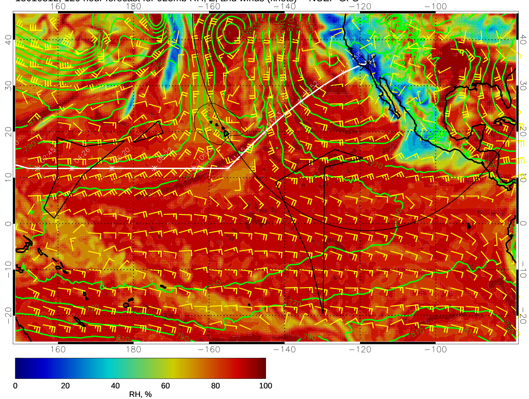
15010312, 120 hour forecast for 925mb RH, Z, and winds (knots) -- NCEP GFS
