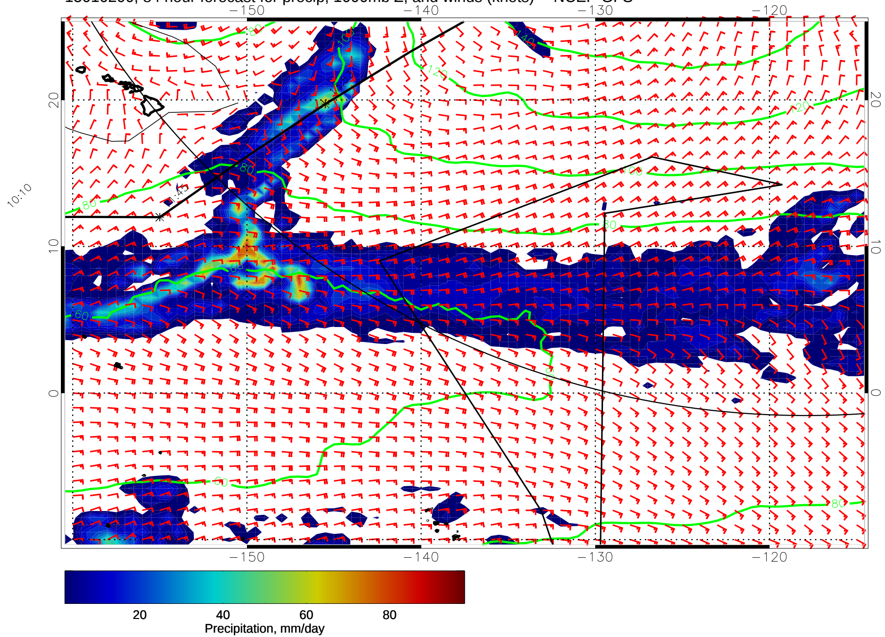
15010200, 84 hour forecast for precip, 1000mb Z, and winds (knots) -- NCEP GFS
