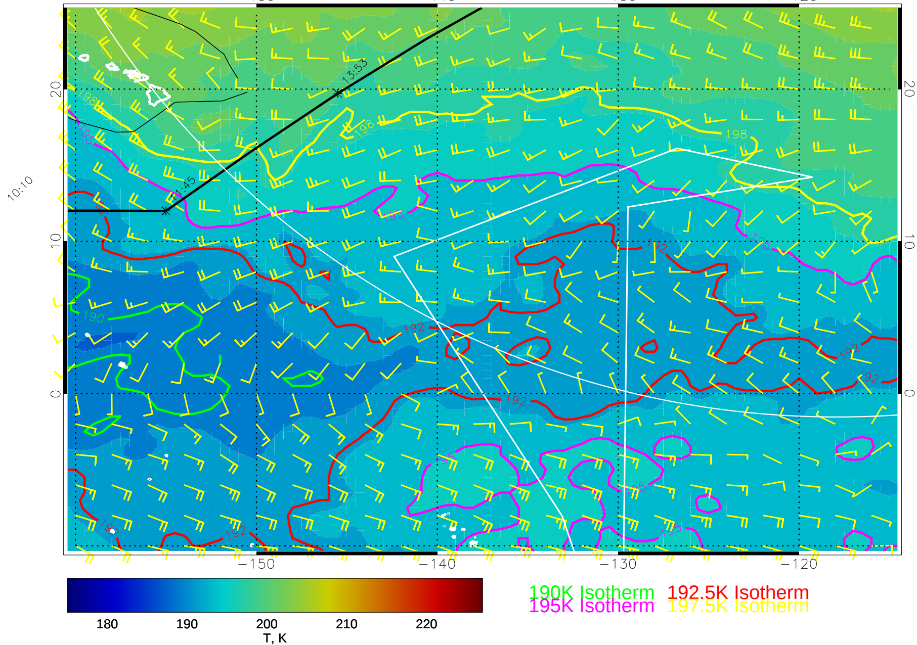
15010118, 78 hour forecast for 70mb T and winds (knots) -- NCEP GFS
