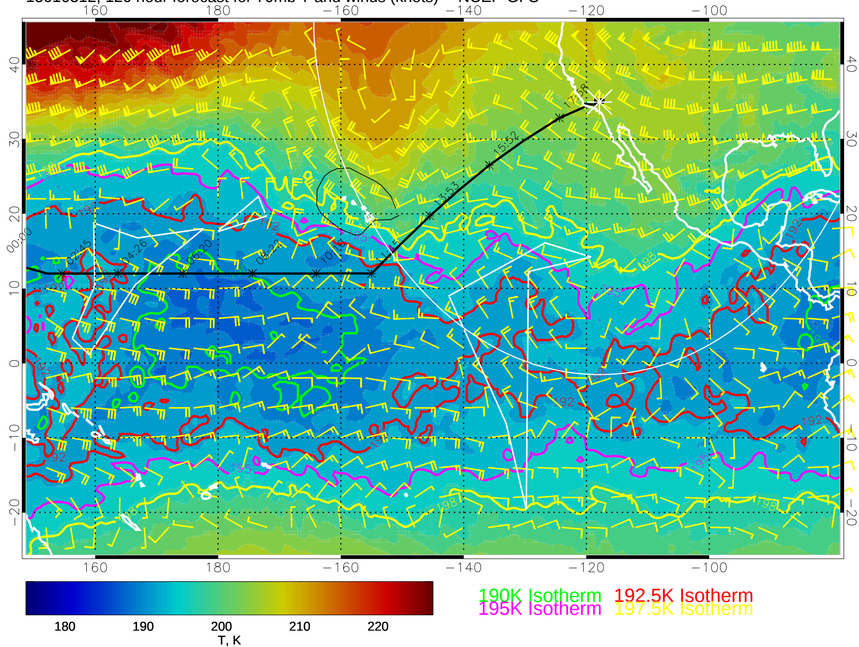
15010312, 120 hour forecast for 70mb T and winds (knots) -- NCEP GFS
