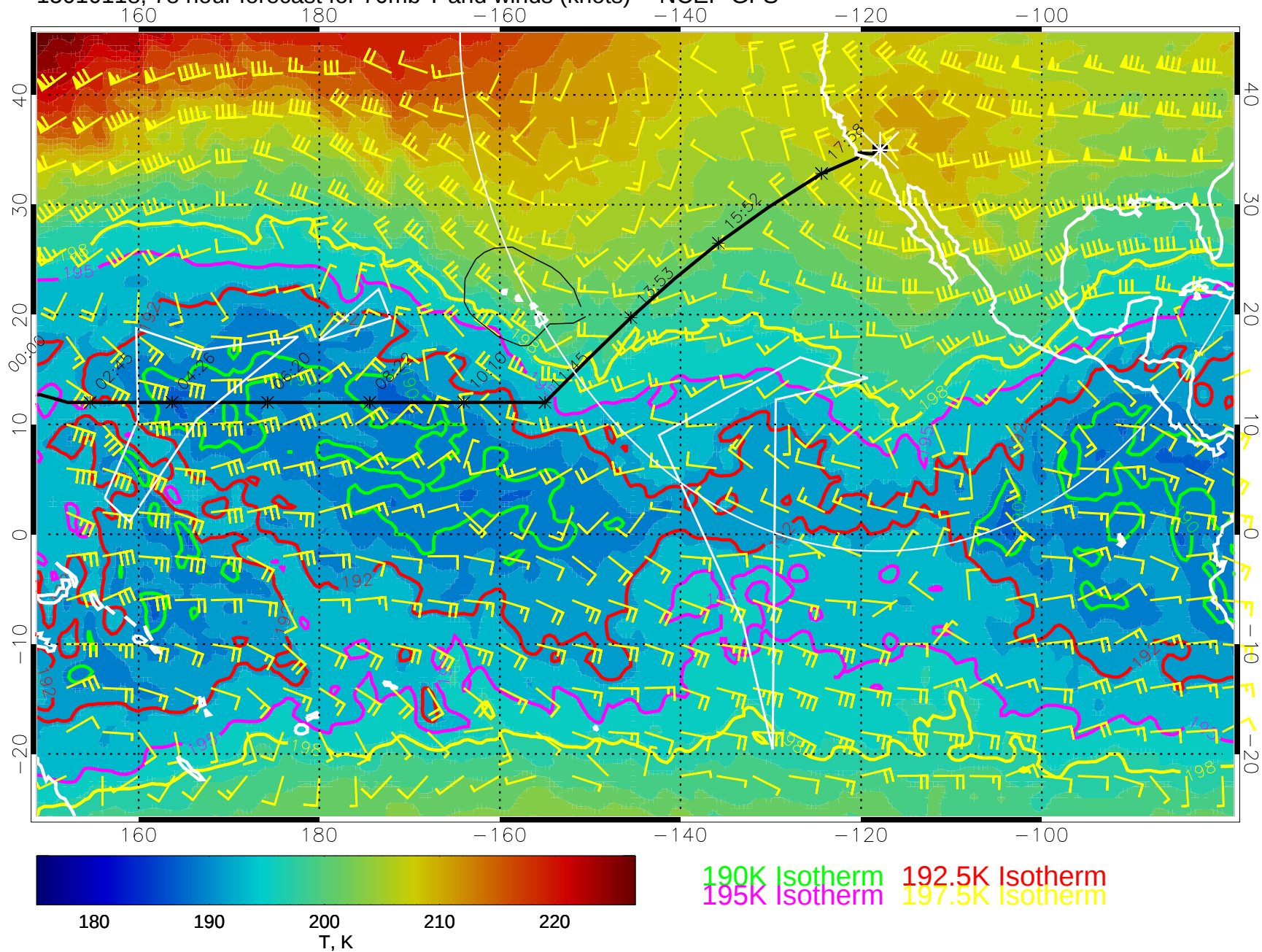
15010118, 78 hour forecast for 70mb T and winds (knots) -- NCEP GFS
