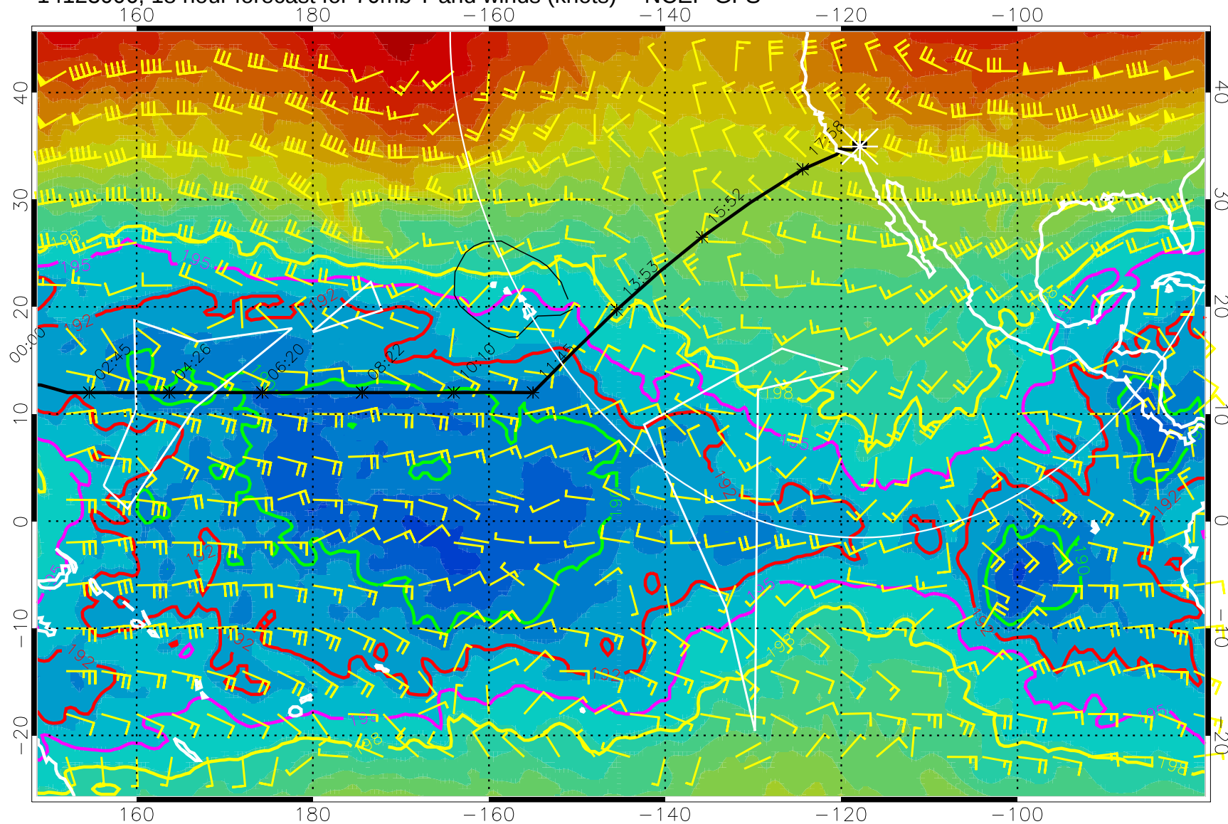
14123006, 18 hour forecast for 70mb T and winds (knots) -- NCEP GFS
