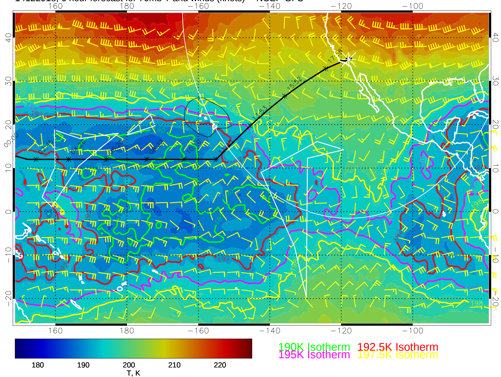
14122918, 6 hour forecast for 70mb T and winds (knots) -- NCEP GFS
