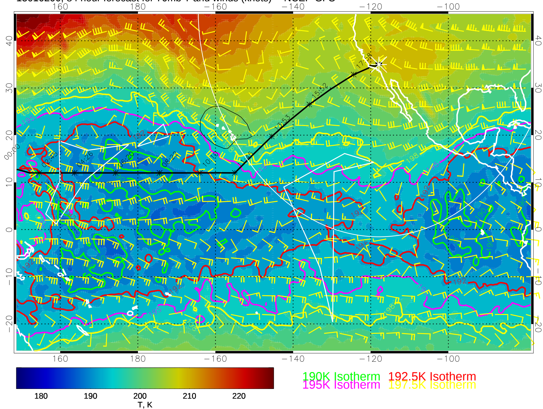
15010200, 84 hour forecast for 70mb T and winds (knots) -- NCEP GFS
