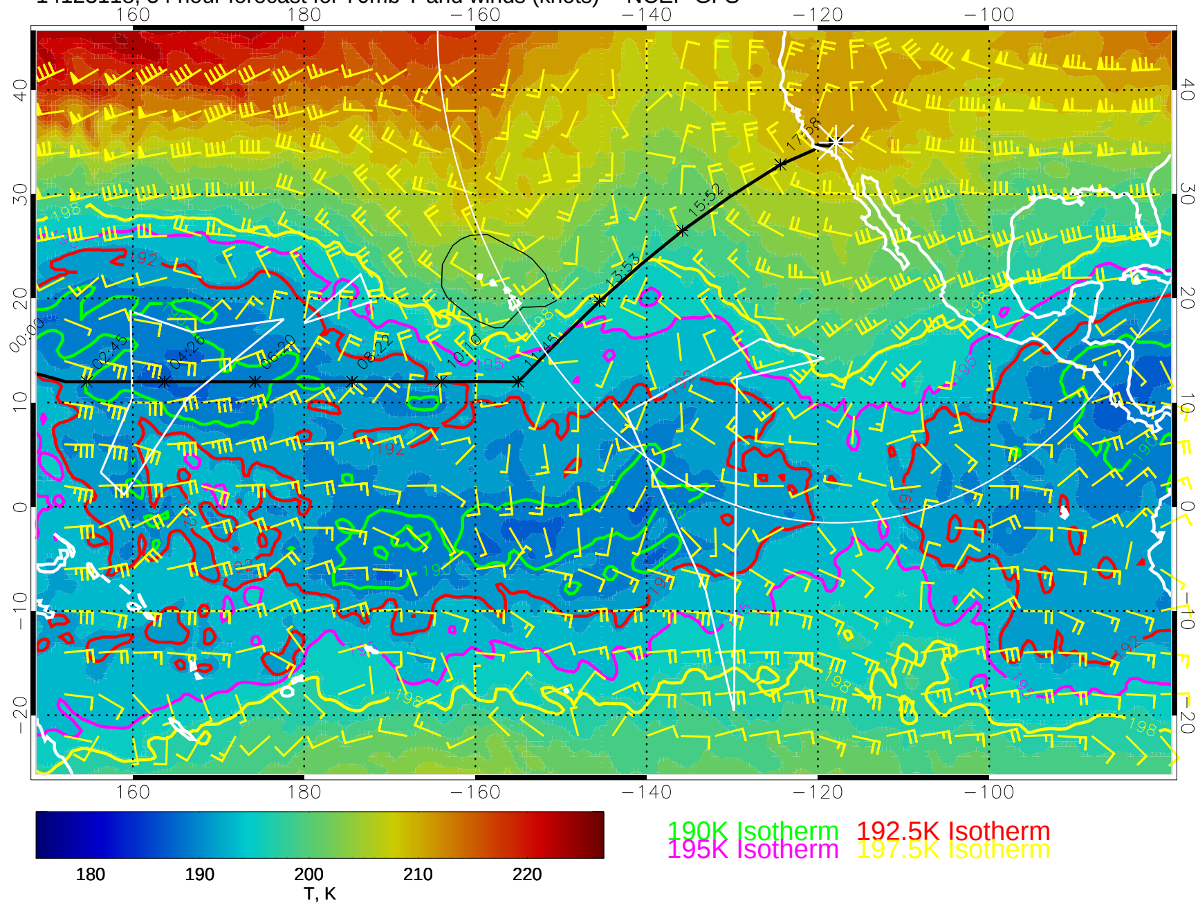
14123118, 54 hour forecast for 70mb T and winds (knots) -- NCEP GFS
