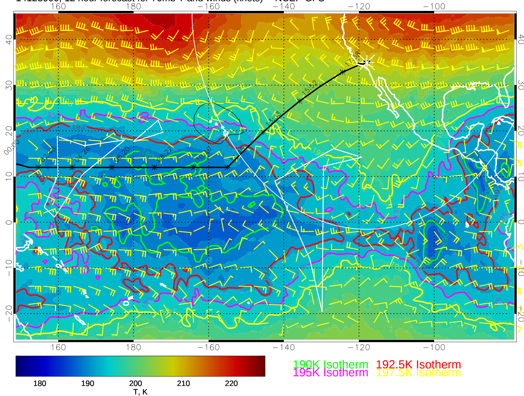
14123000, 12 hour forecast for 70mb T and winds (knots) -- NCEP GFS
