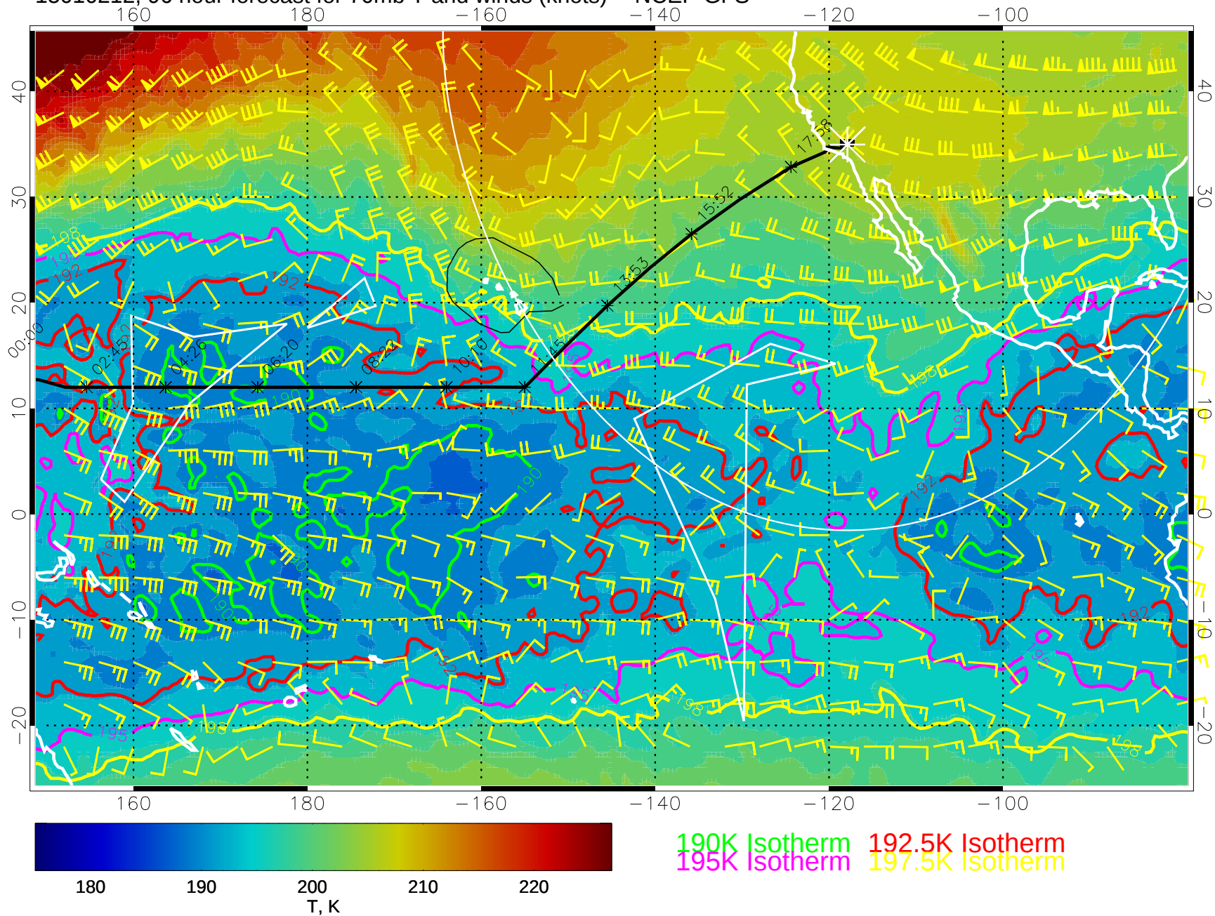
15010212, 96 hour forecast for 70mb T and winds (knots) -- NCEP GFS
