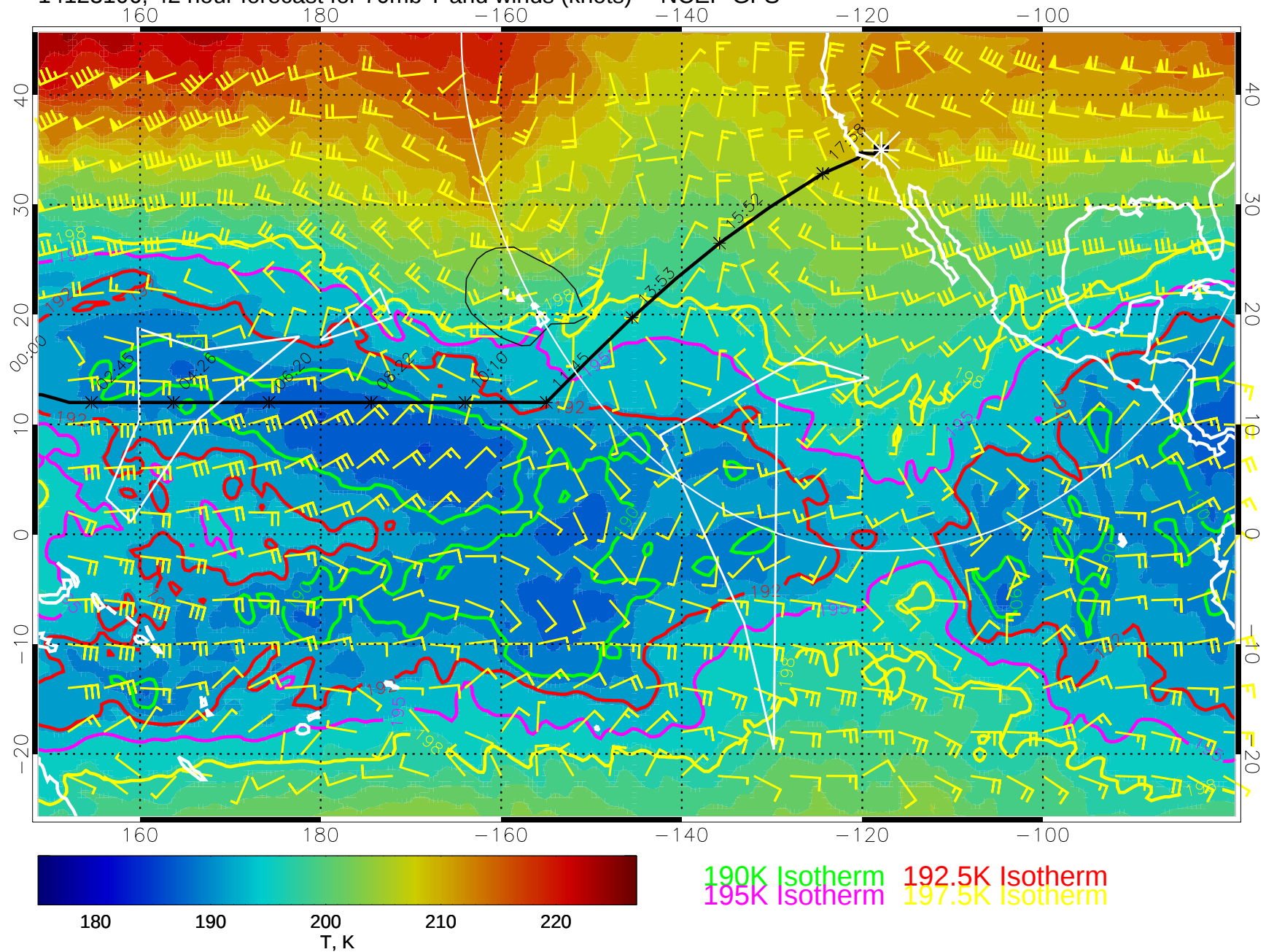
14123106, 42 hour forecast for 70mb T and winds (knots) -- NCEP GFS
