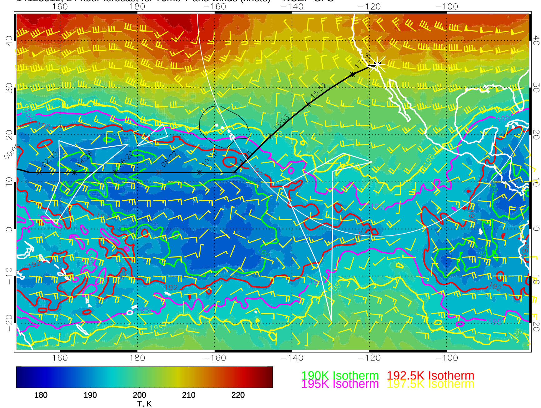
14123012, 24 hour forecast for 70mb T and winds (knots) -- NCEP GFS
