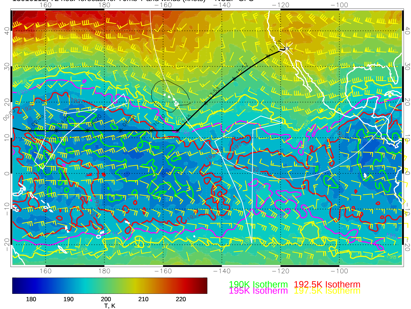
15010112, 72 hour forecast for 70mb T and winds (knots) -- NCEP GFS
