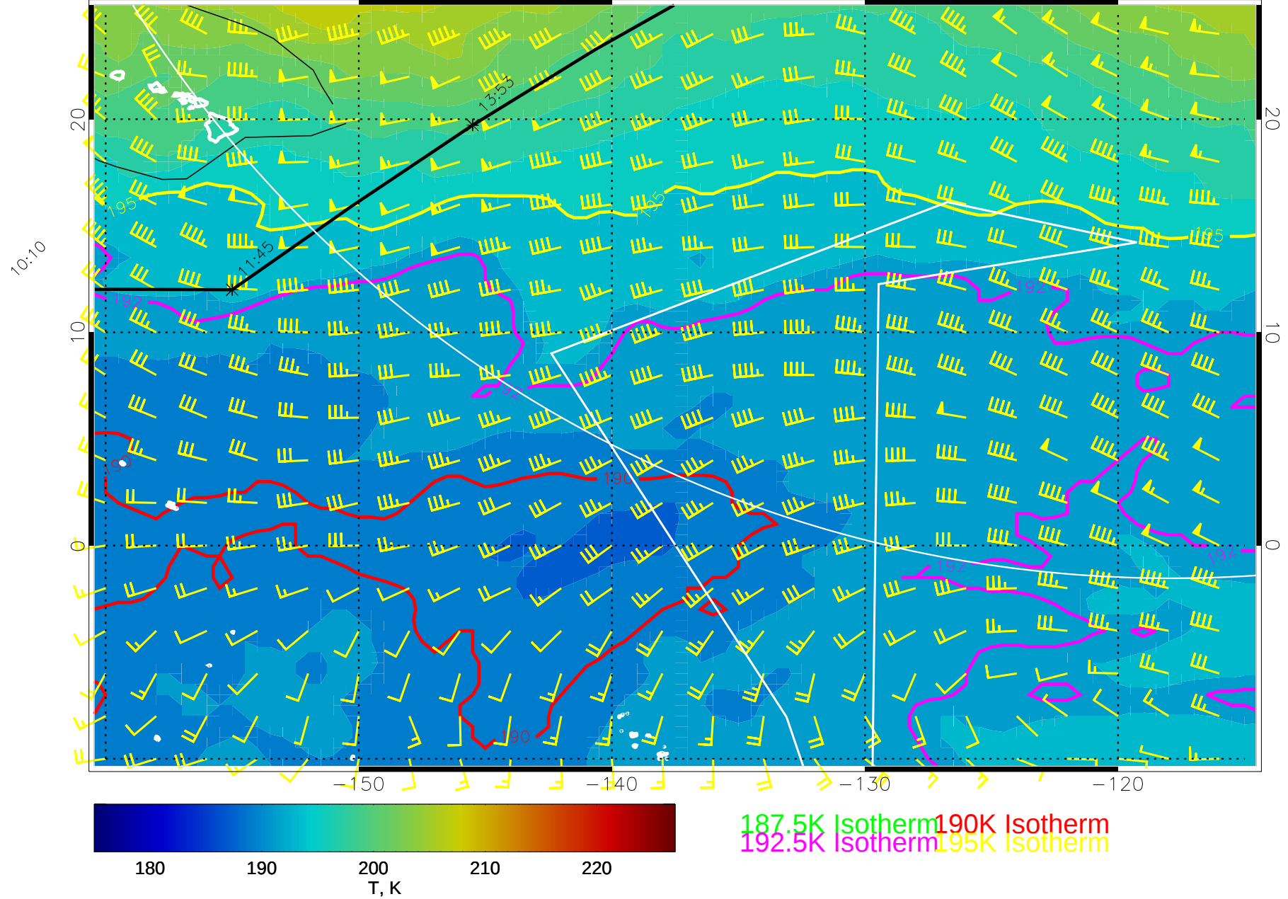
15010106, 66 hour forecast for 100mb T and winds (knots) -- NCEP GFS
