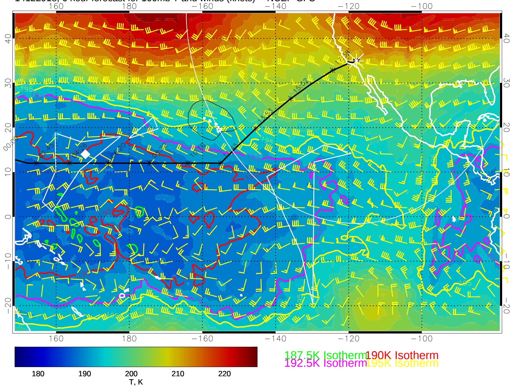
14122918, 6 hour forecast for 100mb T and winds (knots) -- NCEP GFS
