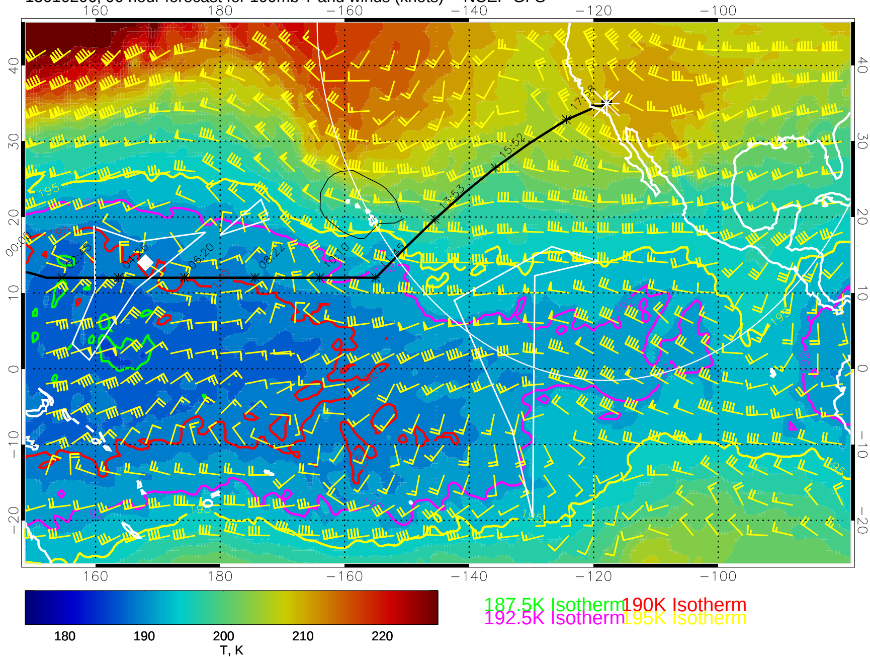
15010206, 90 hour forecast for 100mb T and winds (knots) -- NCEP GFS
