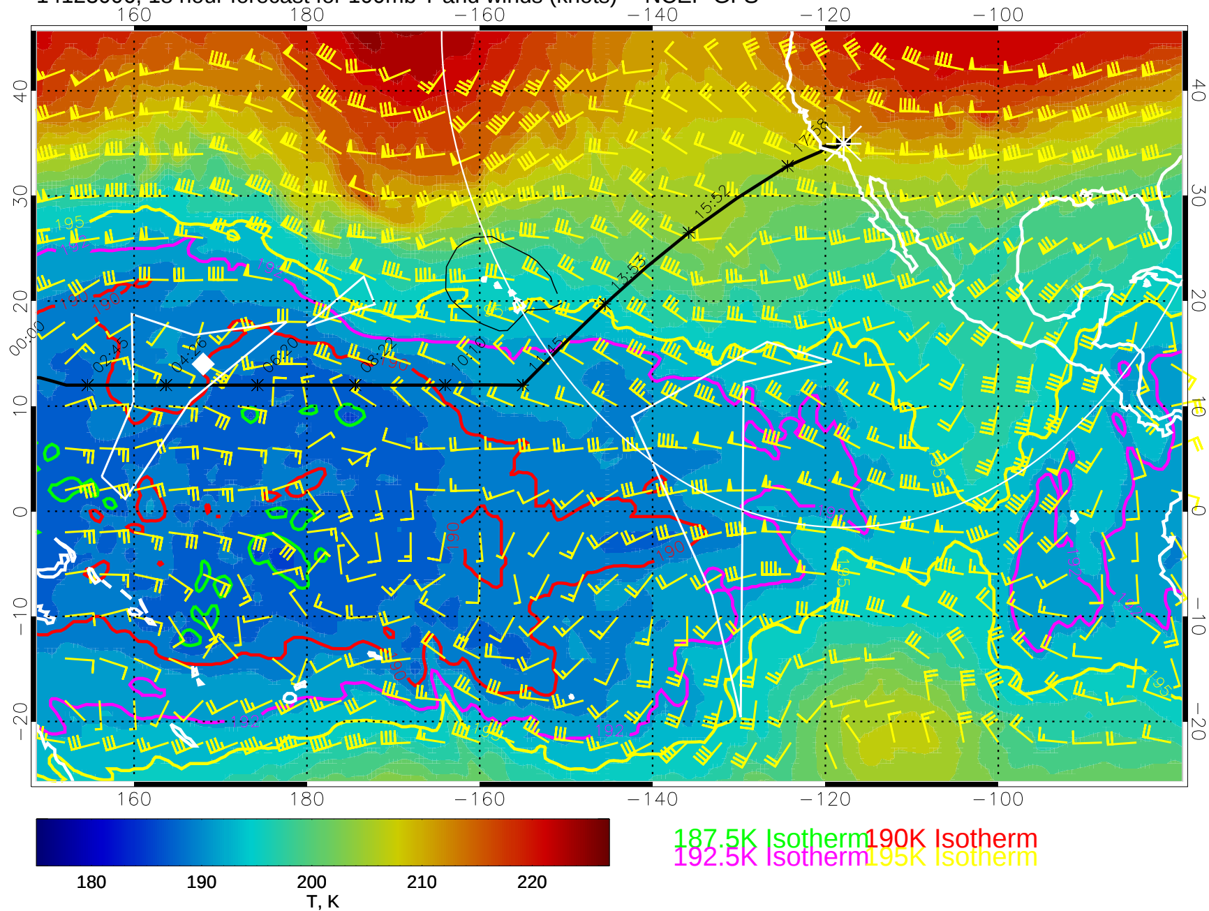
14123006, 18 hour forecast for 100mb T and winds (knots) -- NCEP GFS
