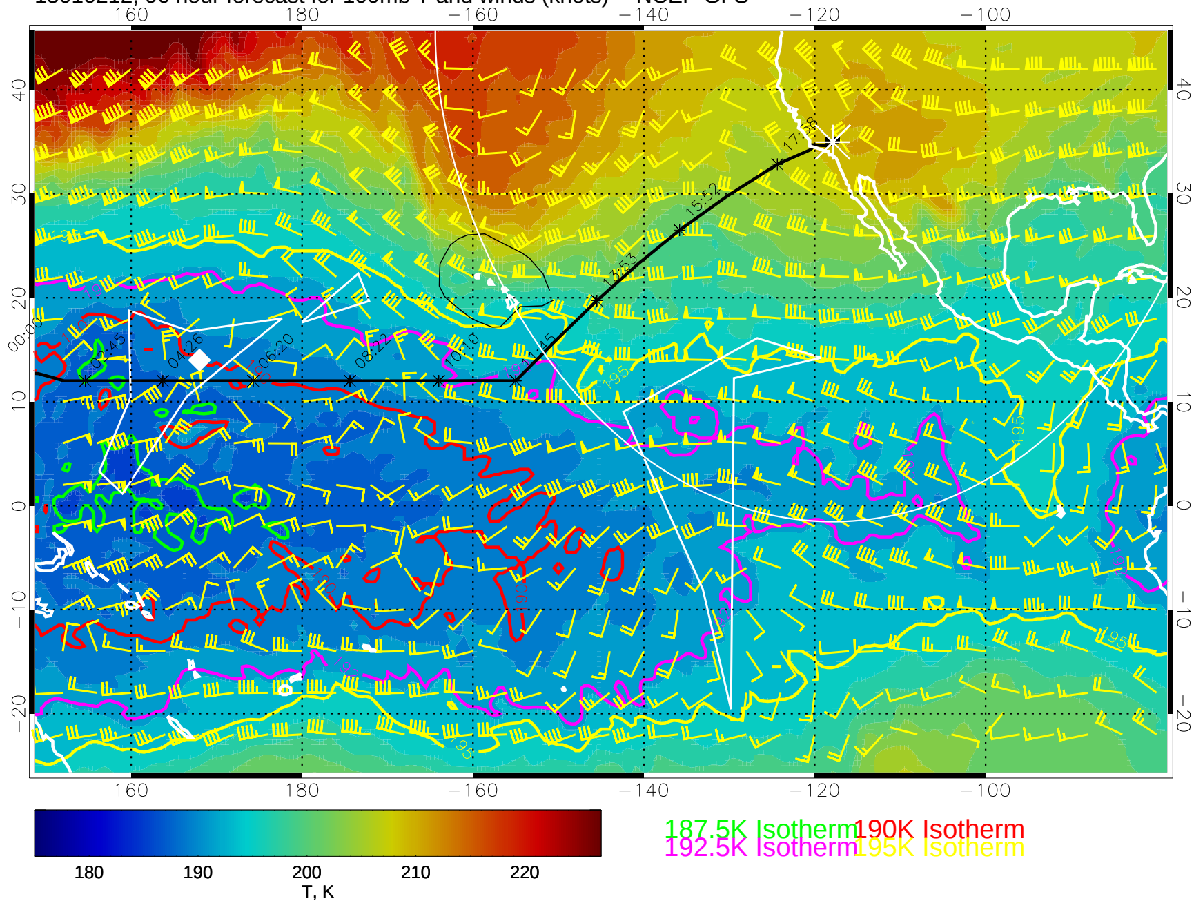
15010212, 96 hour forecast for 100mb T and winds (knots) -- NCEP GFS
