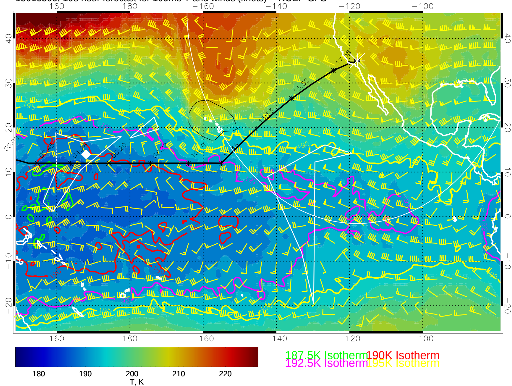
15010300, 108 hour forecast for 100mb T and winds (knots) -- NCEP GFS
