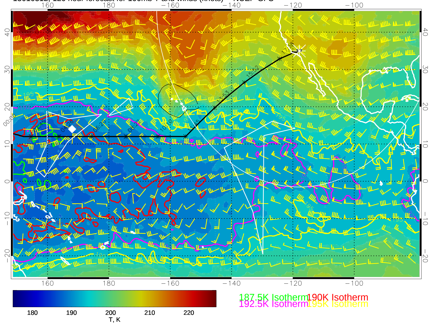
15010312, 120 hour forecast for 100mb T and winds (knots) -- NCEP GFS
