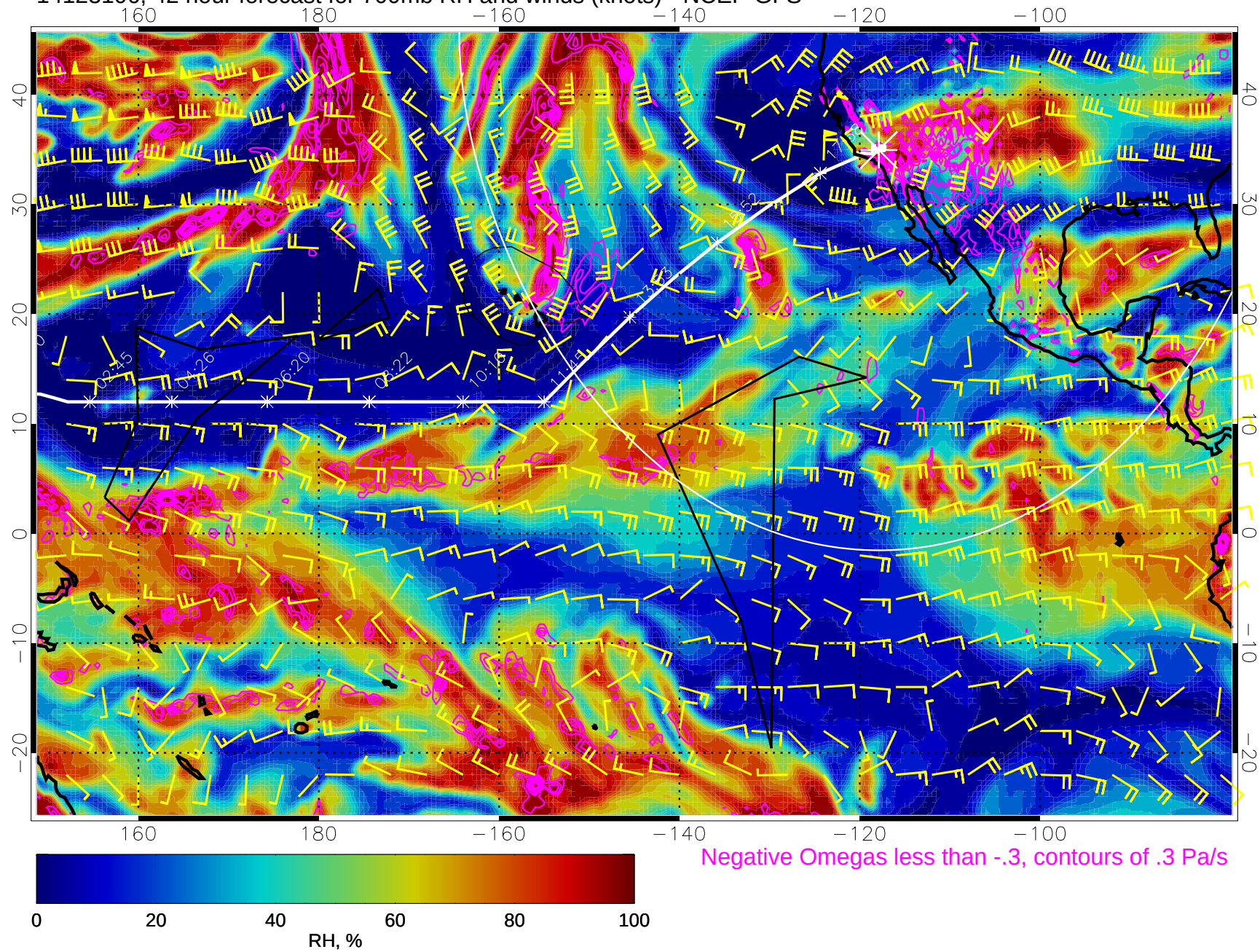
14123106, 42 hour forecast for 700mb RH and winds (knots) - NCEP GFS
