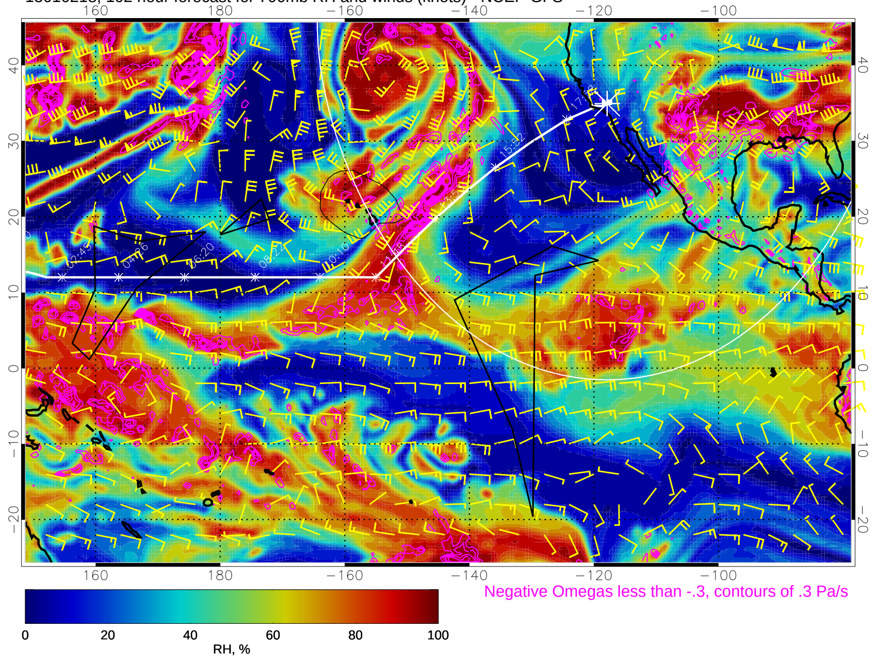
15010218, 102 hour forecast for 700mb RH and winds (knots) - NCEP GFS
