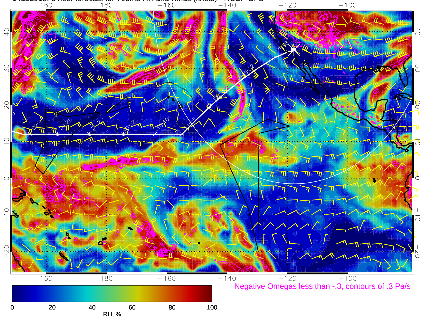
14122918, 6 hour forecast for 700mb RH and winds (knots) - NCEP GFS
