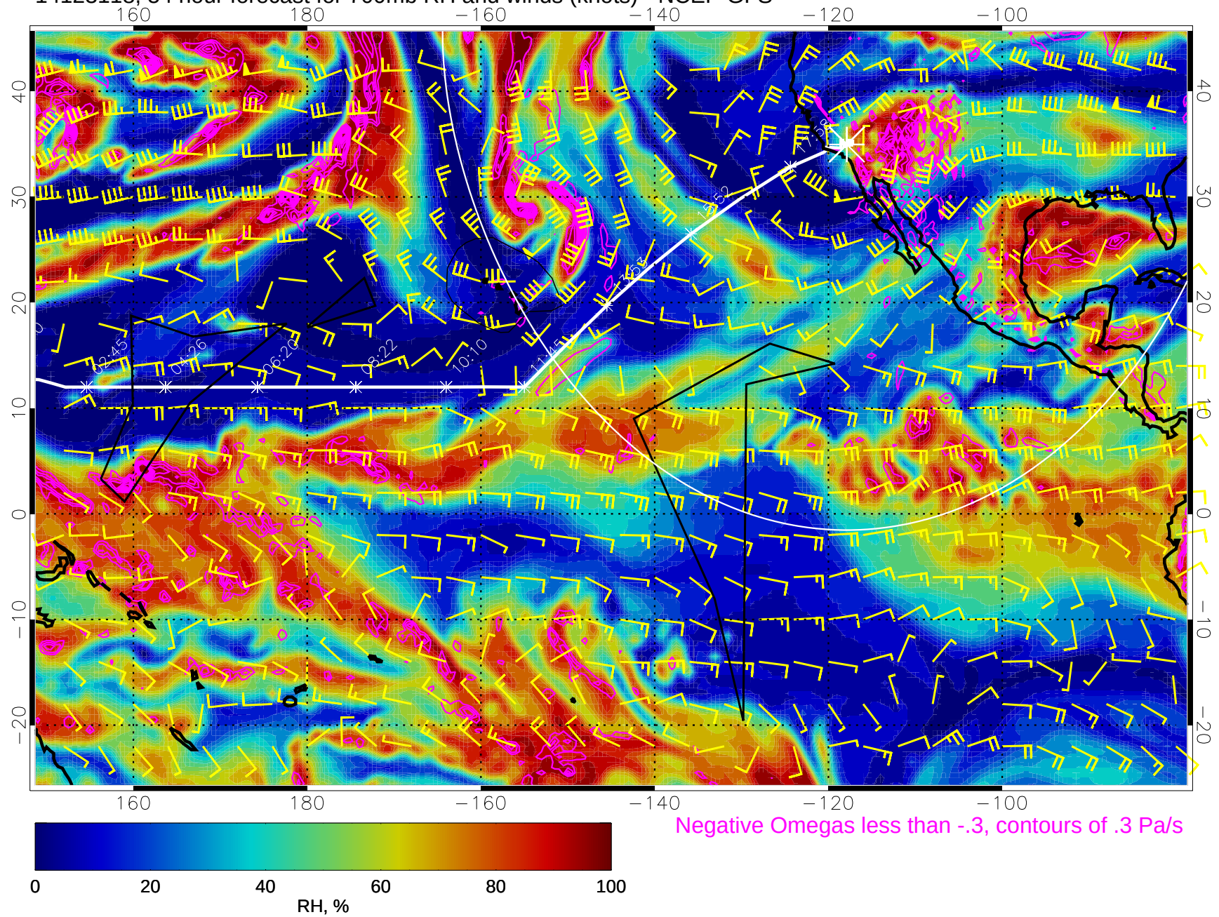
14123118, 54 hour forecast for 700mb RH and winds (knots) - NCEP GFS
