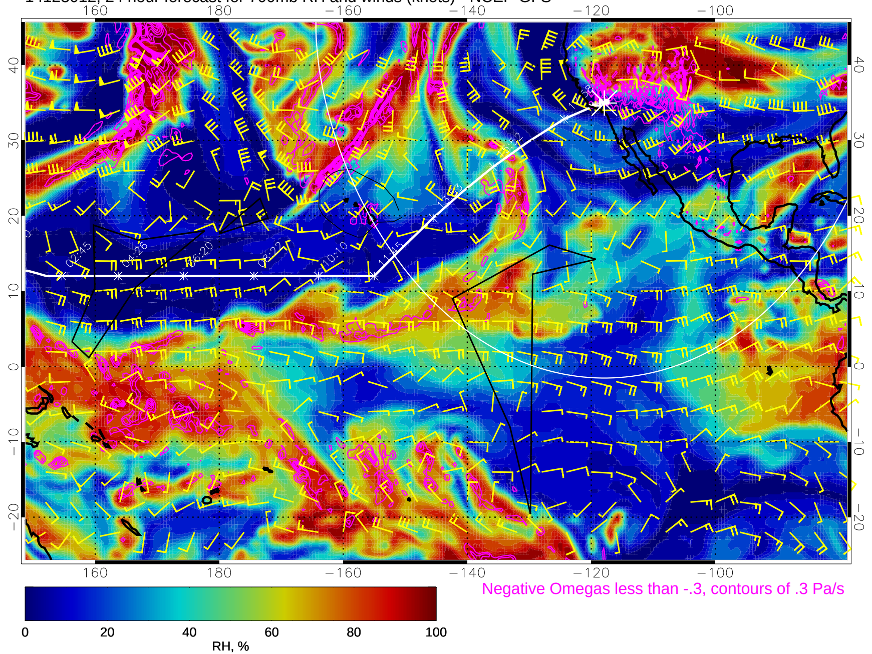
14123012, 24 hour forecast for 700mb RH and winds (knots) - NCEP GFS
