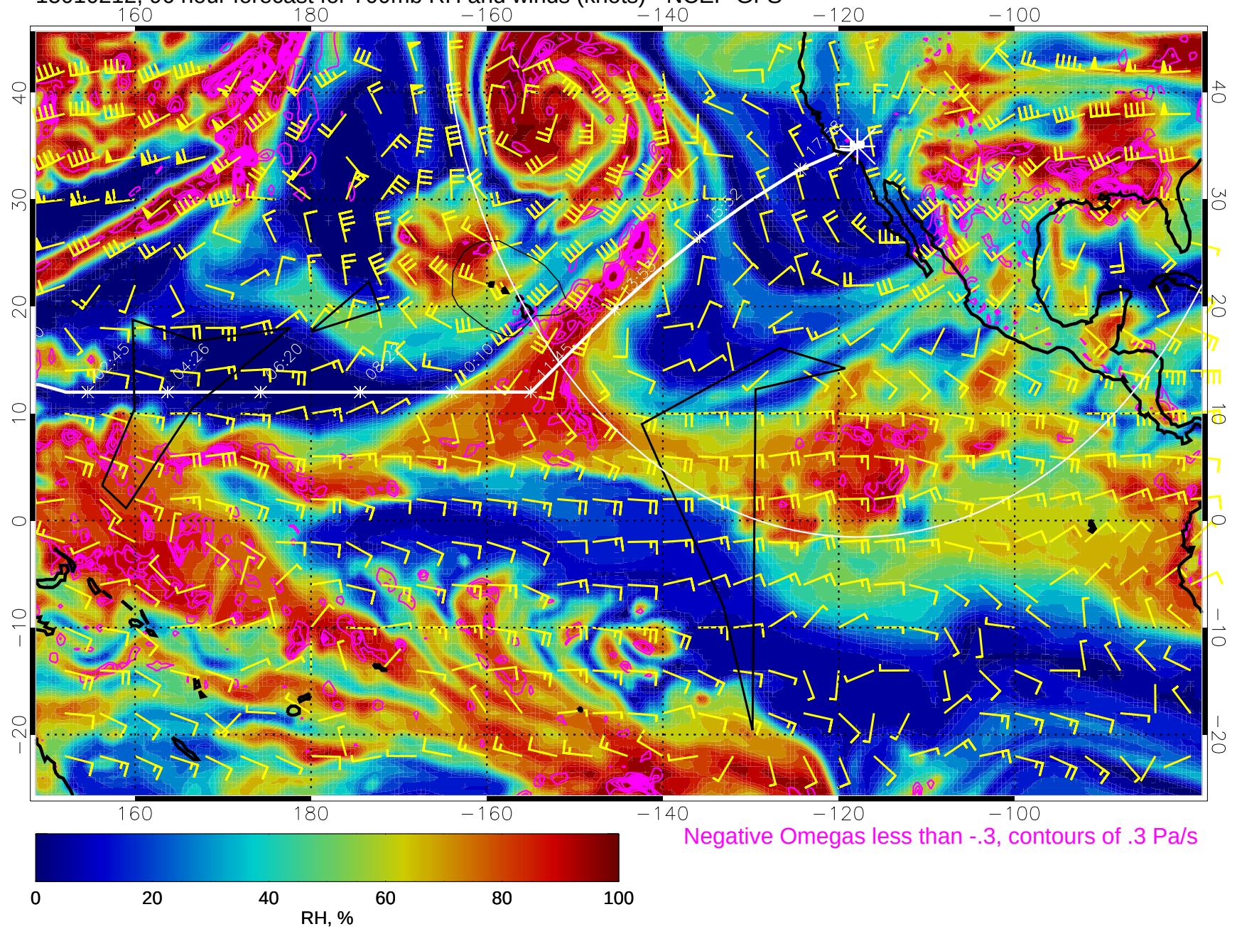
15010212, 96 hour forecast for 700mb RH and winds (knots) - NCEP GFS
