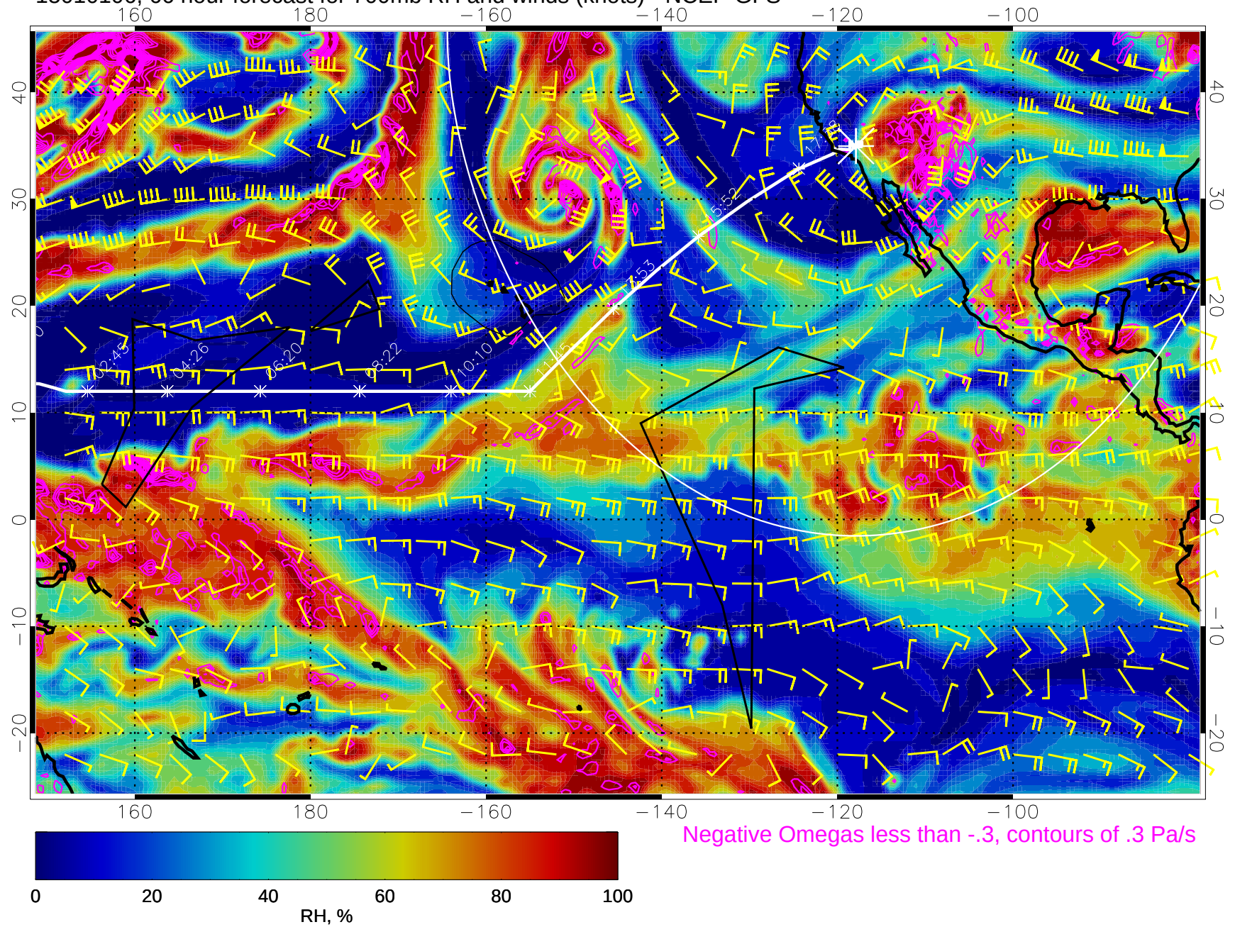
15010106, 66 hour forecast for 700mb RH and winds (knots) - NCEP GFS
