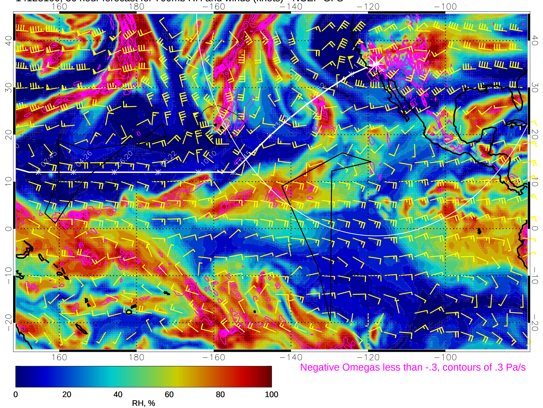
14123100, 36 hour forecast for 700mb RH and winds (knots) - NCEP GFS
