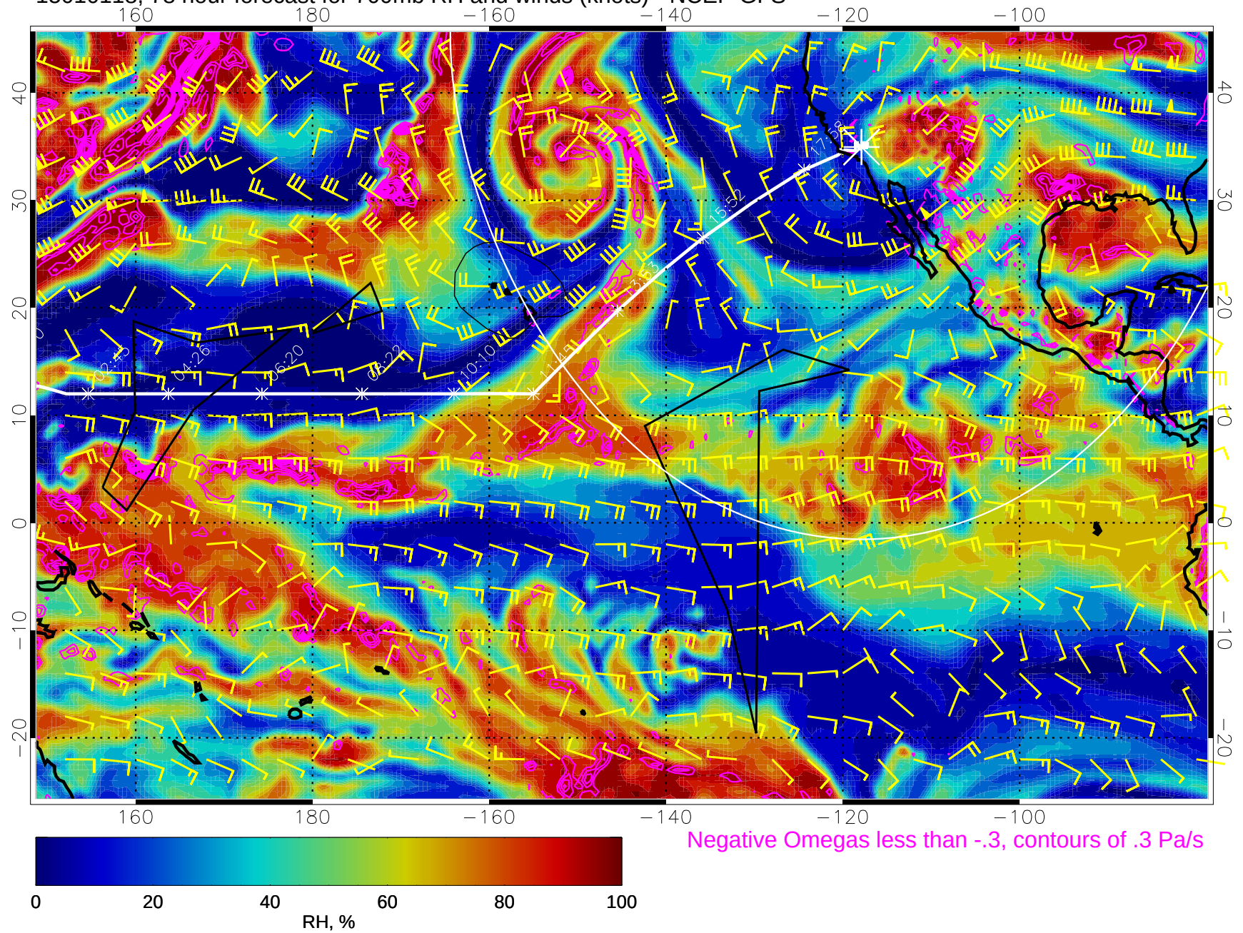
15010118, 78 hour forecast for 700mb RH and winds (knots) - NCEP GFS
