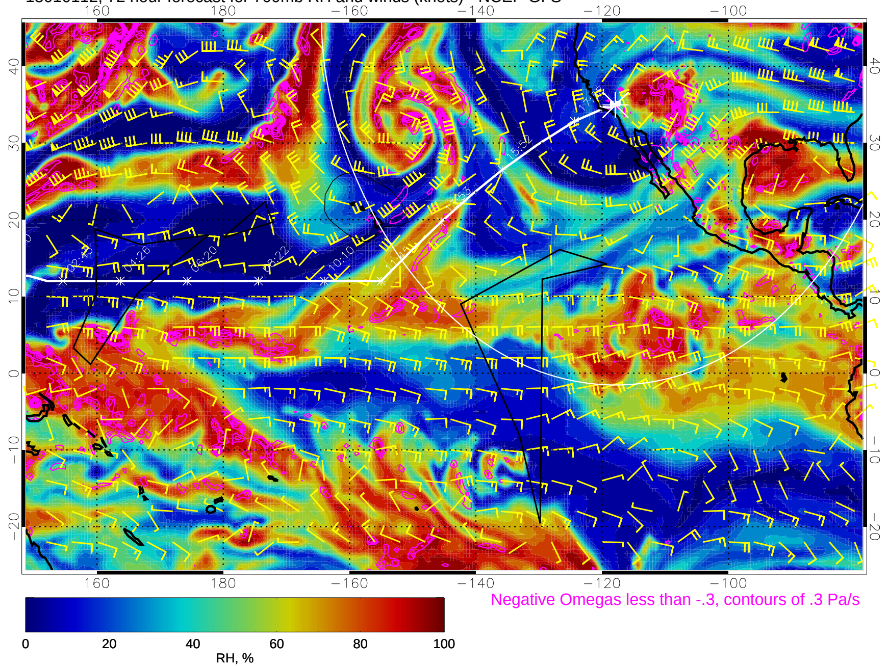
15010112, 72 hour forecast for 700mb RH and winds (knots) - NCEP GFS
