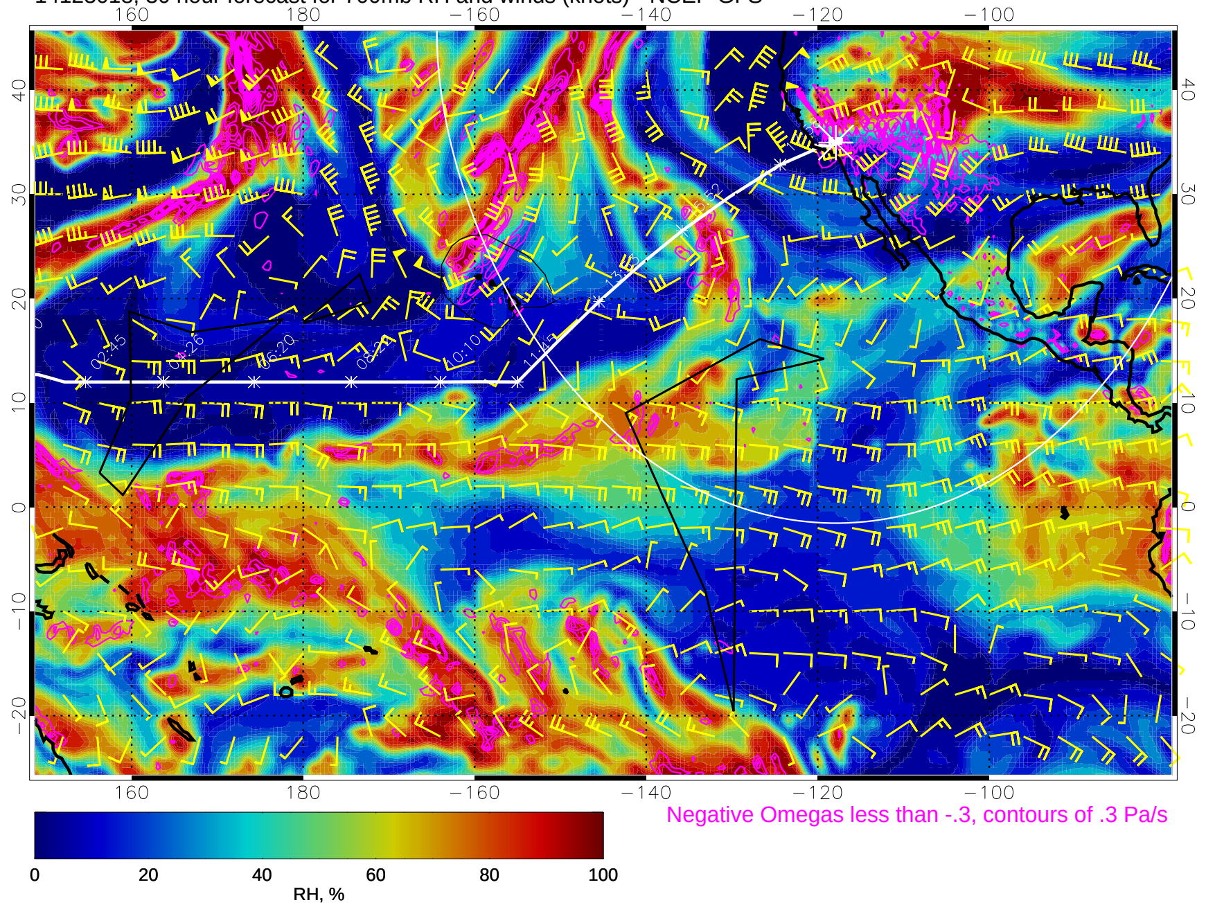
14123018, 30 hour forecast for 700mb RH and winds (knots) - NCEP GFS
