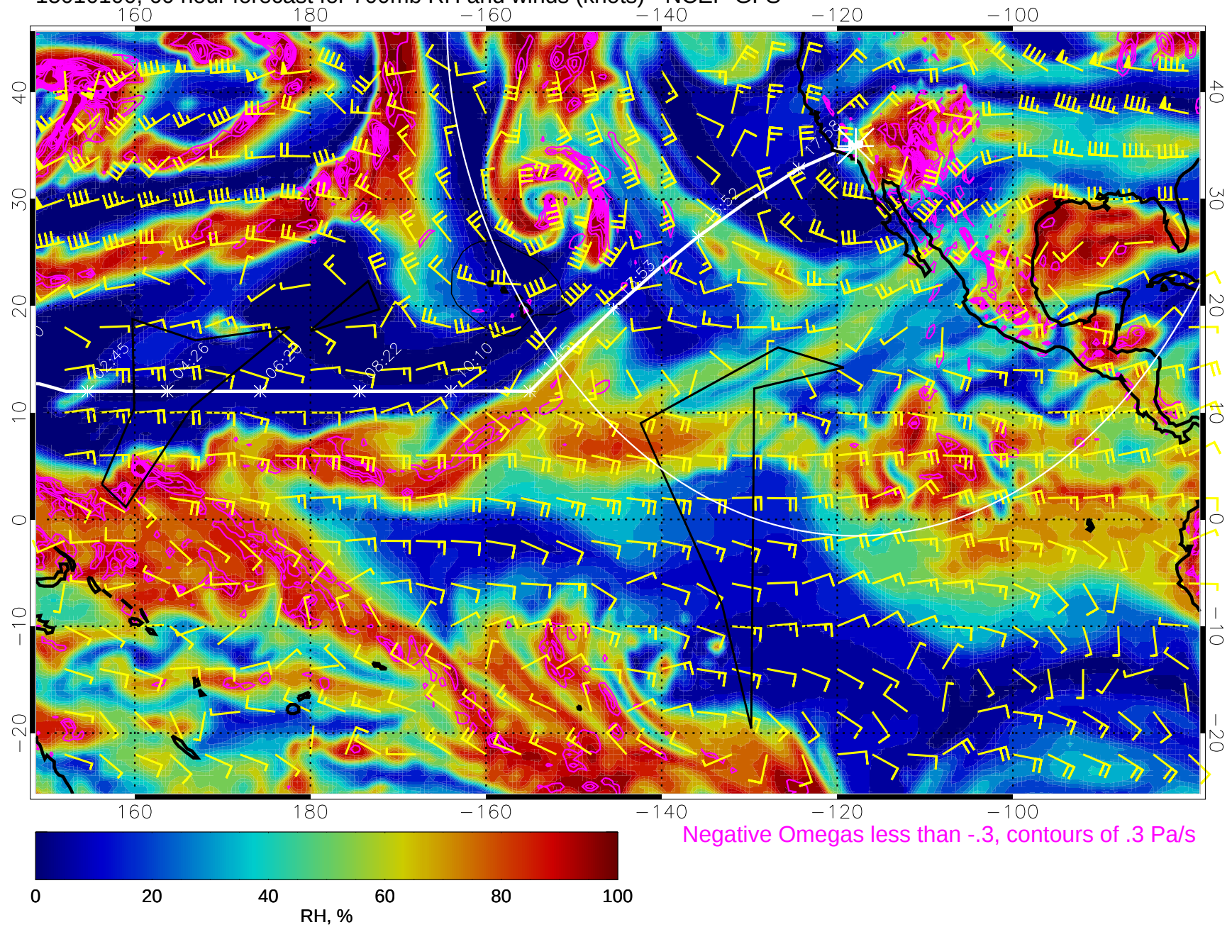
15010100, 60 hour forecast for 700mb RH and winds (knots) - NCEP GFS
