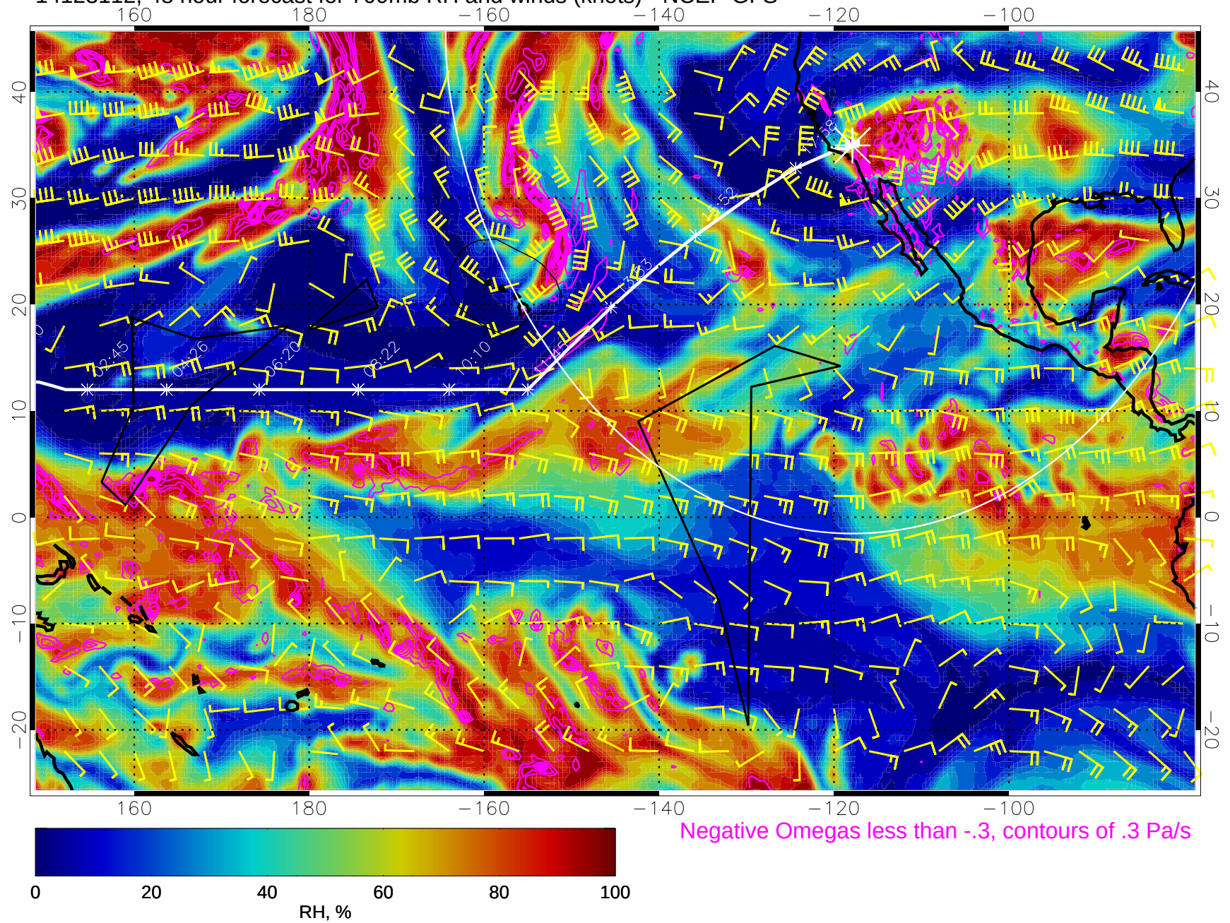
14123112, 48 hour forecast for 700mb RH and winds (knots) - NCEP GFS
