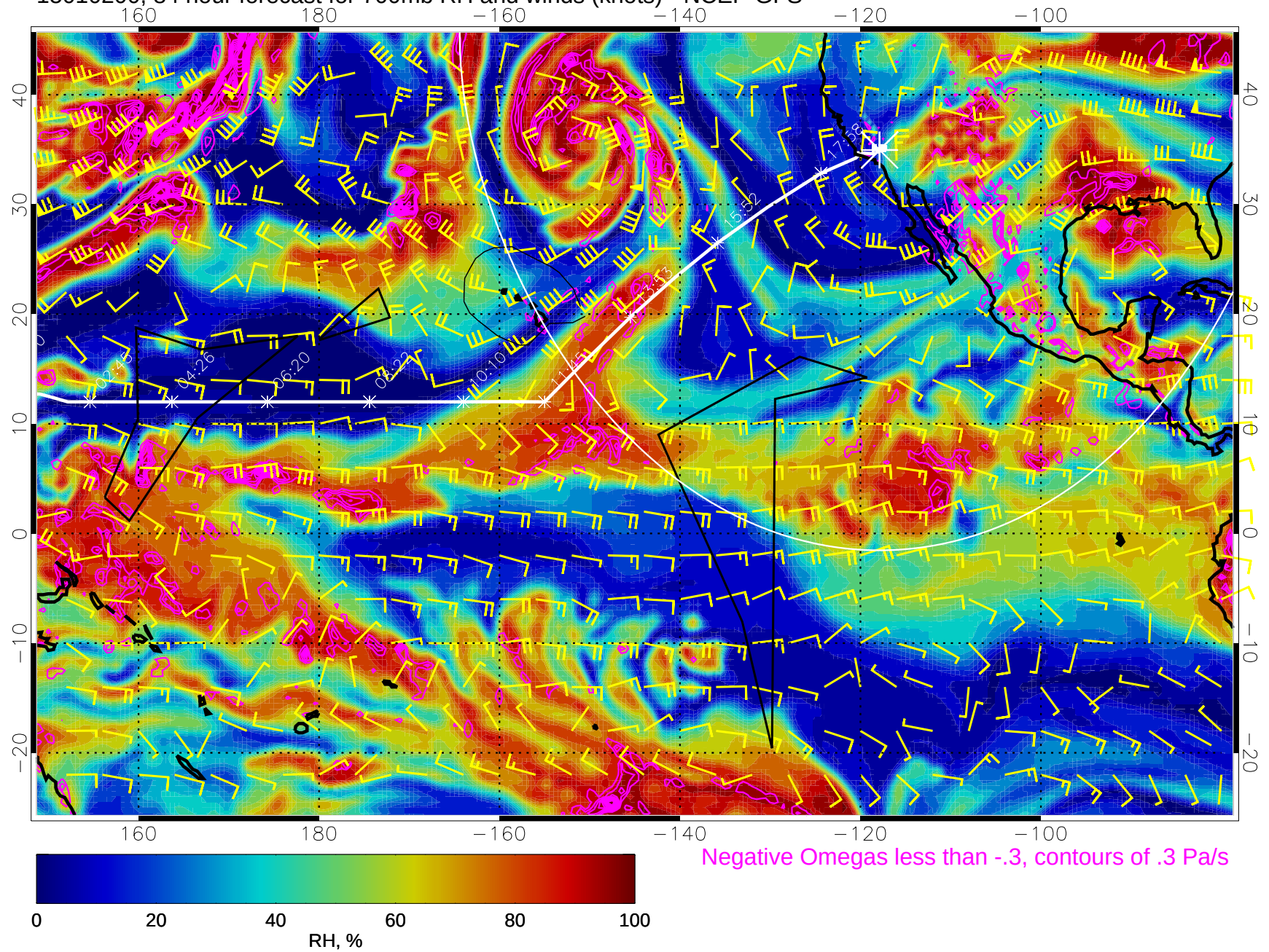
15010200, 84 hour forecast for 700mb RH and winds (knots) - NCEP GFS
