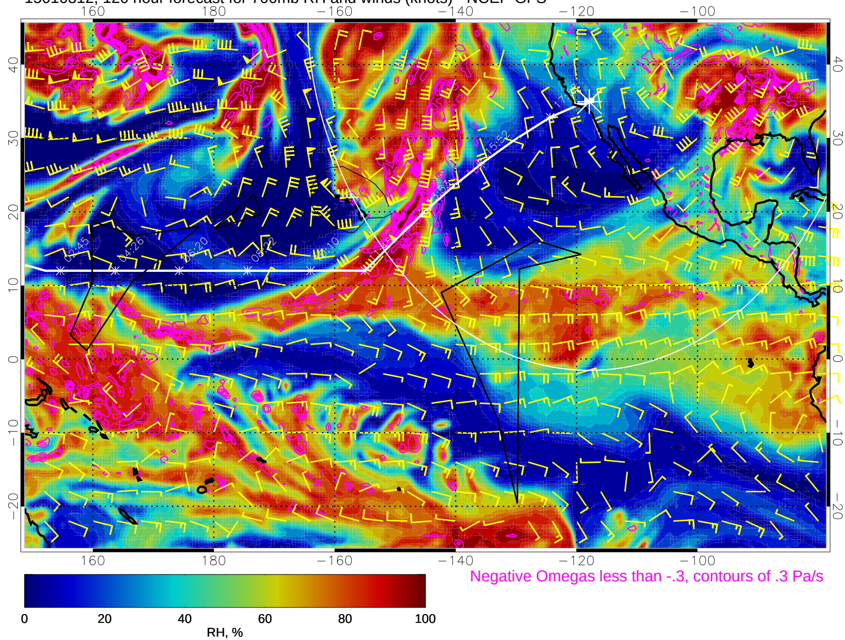
15010312, 120 hour forecast for 700mb RH and winds (knots) - NCEP GFS
