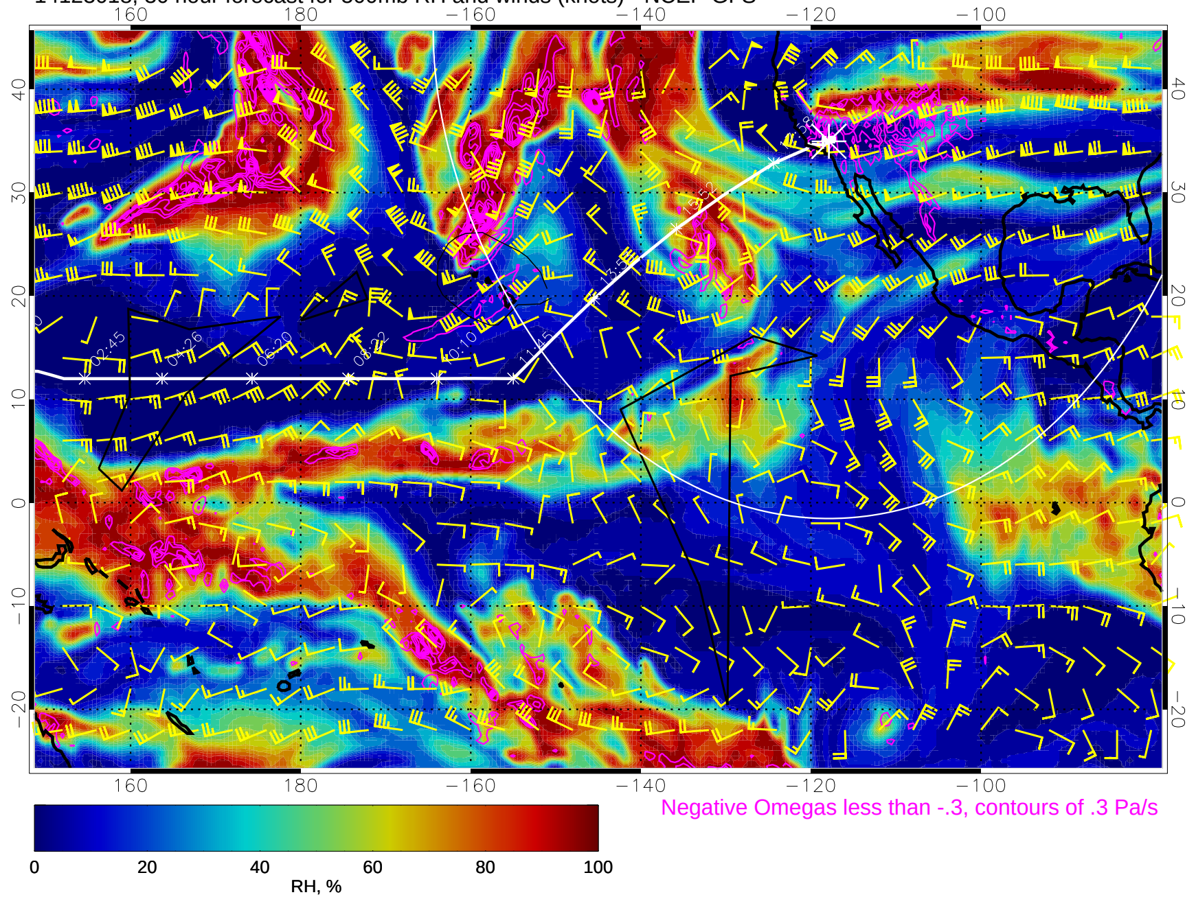
14123018, 30 hour forecast for 500mb RH and winds (knots) - NCEP GFS
