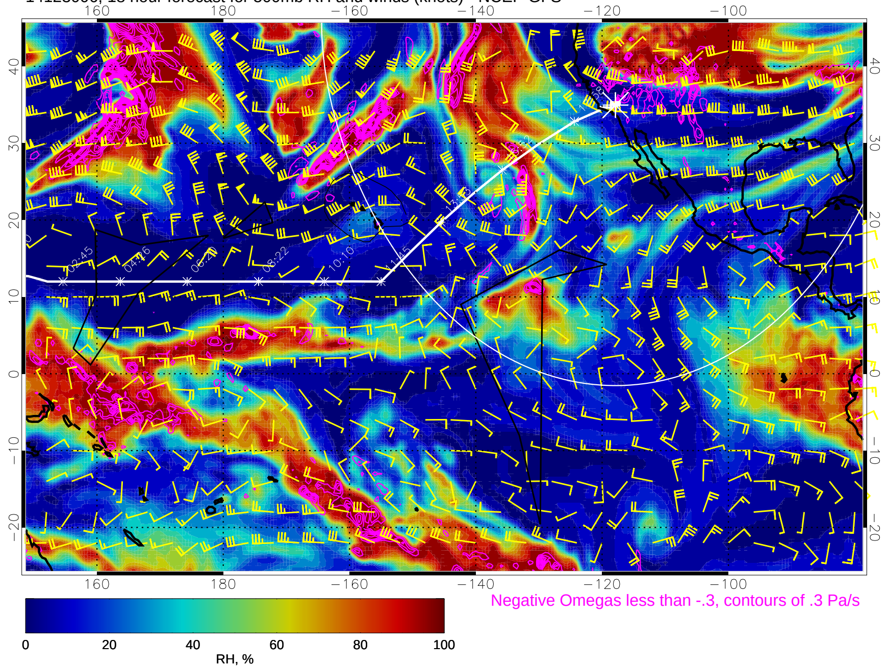
14123006, 18 hour forecast for 500mb RH and winds (knots) - NCEP GFS
