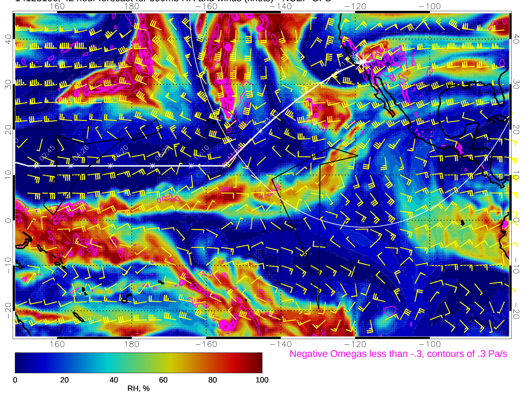
14123106, 42 hour forecast for 500mb RH and winds (knots) - NCEP GFS
