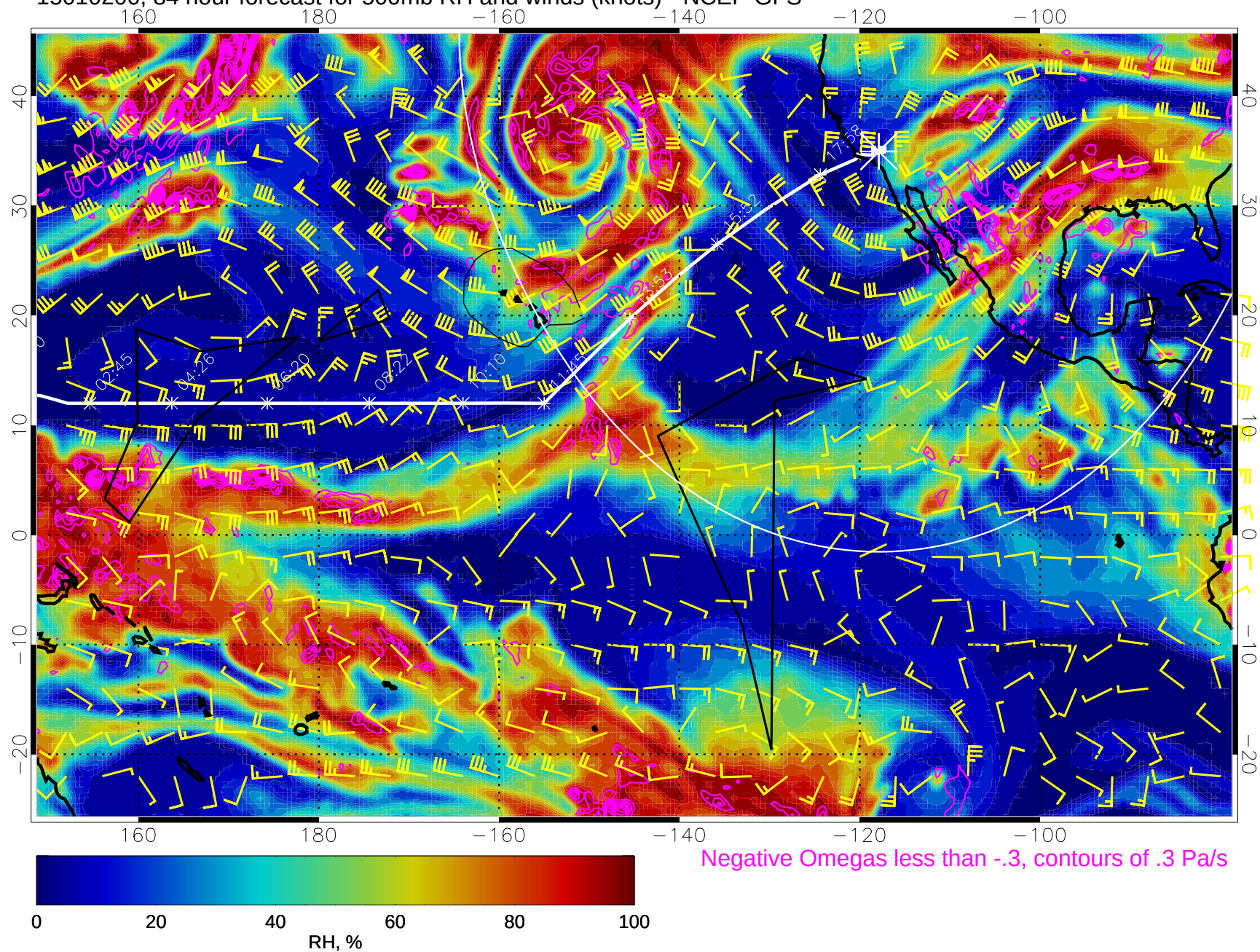
15010200, 84 hour forecast for 500mb RH and winds (knots) - NCEP GFS
