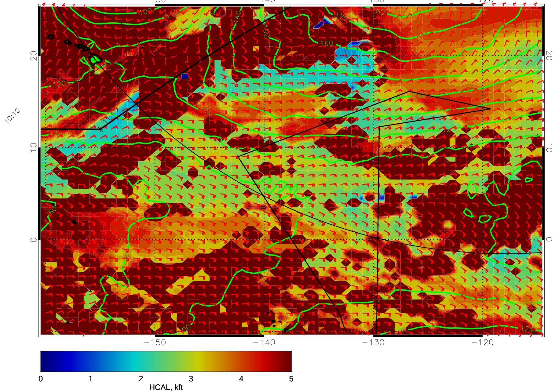
15010118, 78 hour forecast for HCAL, 1000mb Z, and winds (knots) -- NCEP GFS
