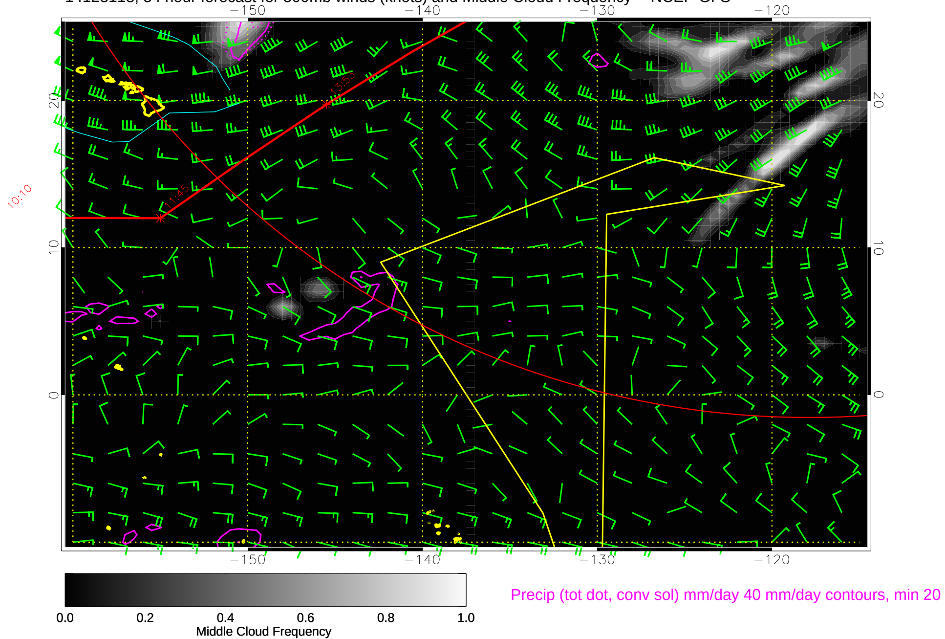
14123118, 54 hour forecast for 500mb winds (knots) and Middle Cloud Frequency -- NCEP GFS
