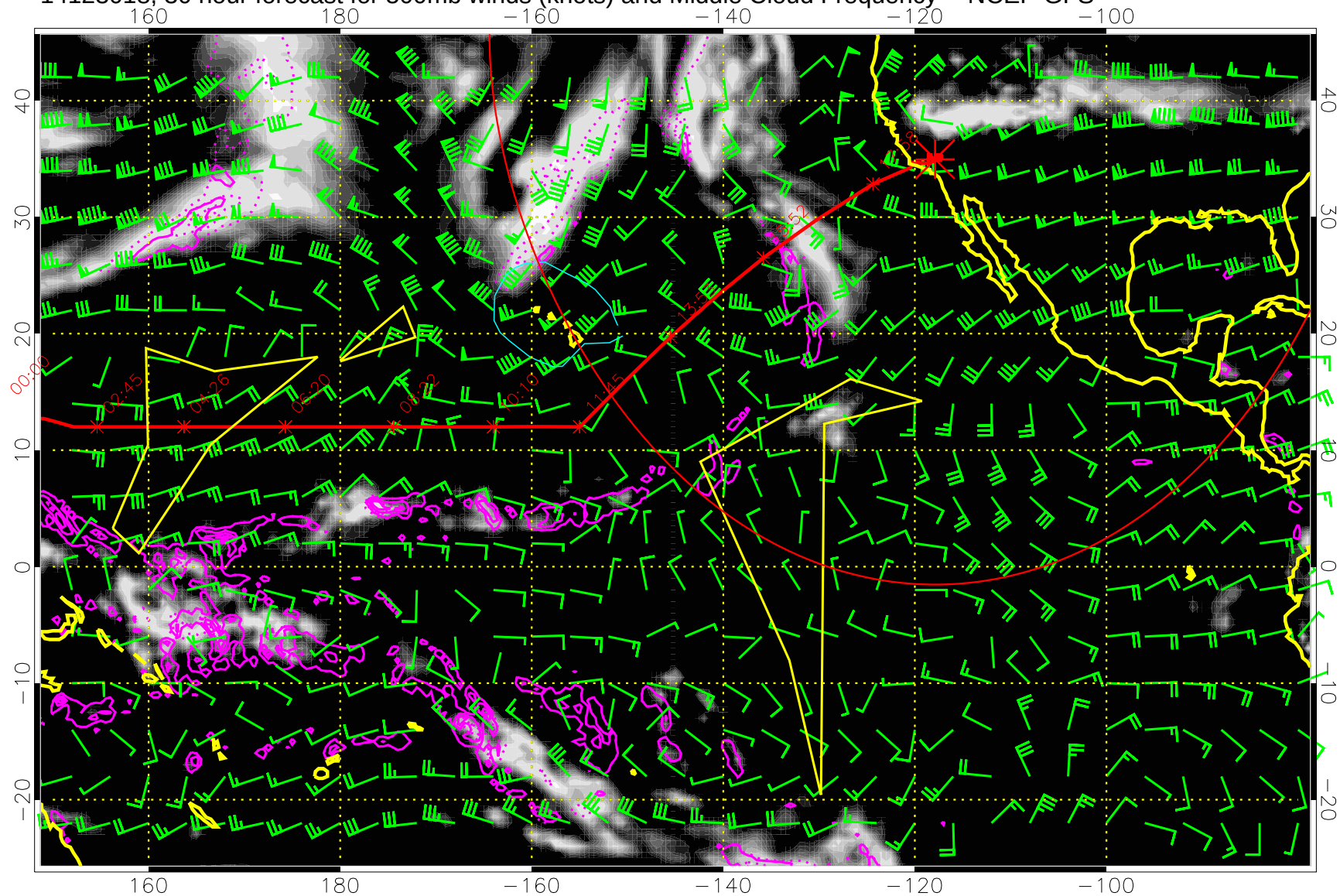
14123018, 30 hour forecast for 500mb winds (knots) and Middle Cloud Frequency -- NCEP GFS
