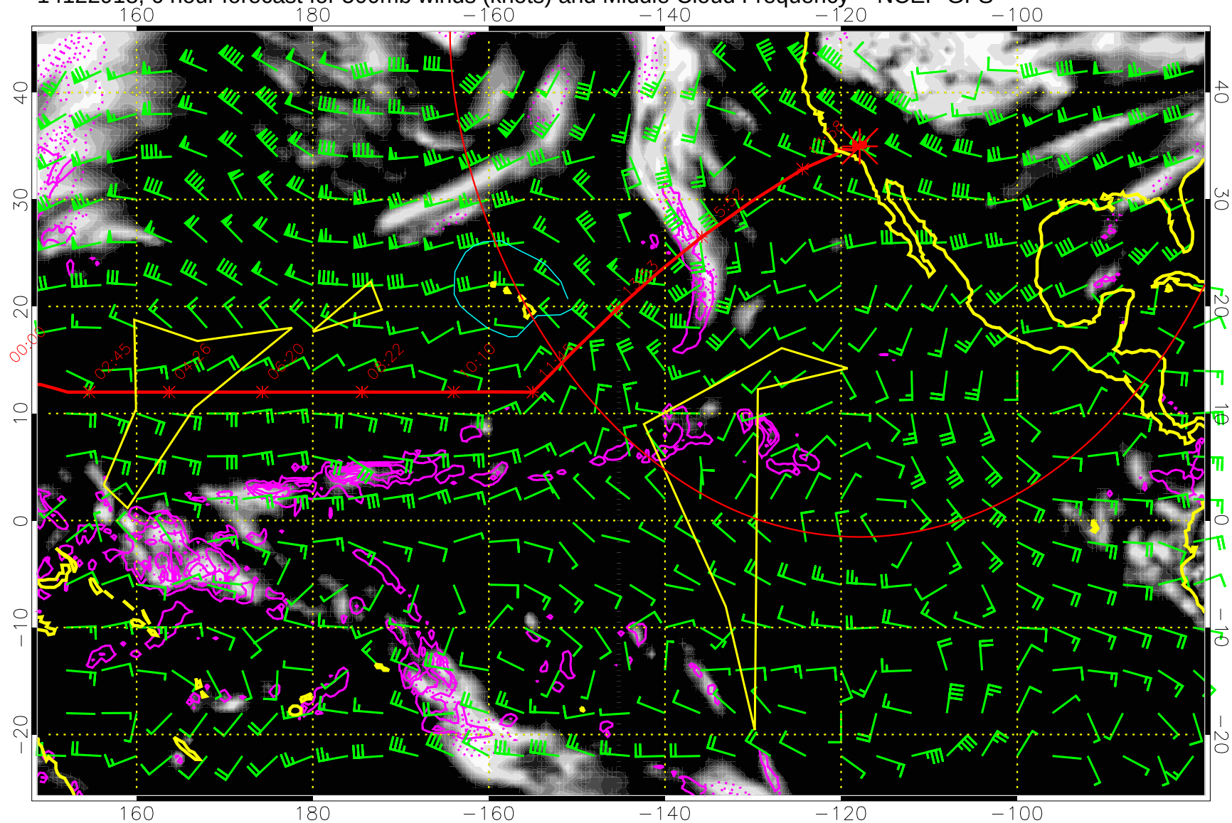
14122918, 6 hour forecast for 500mb winds (knots) and Middle Cloud Frequency -- NCEP GFS
