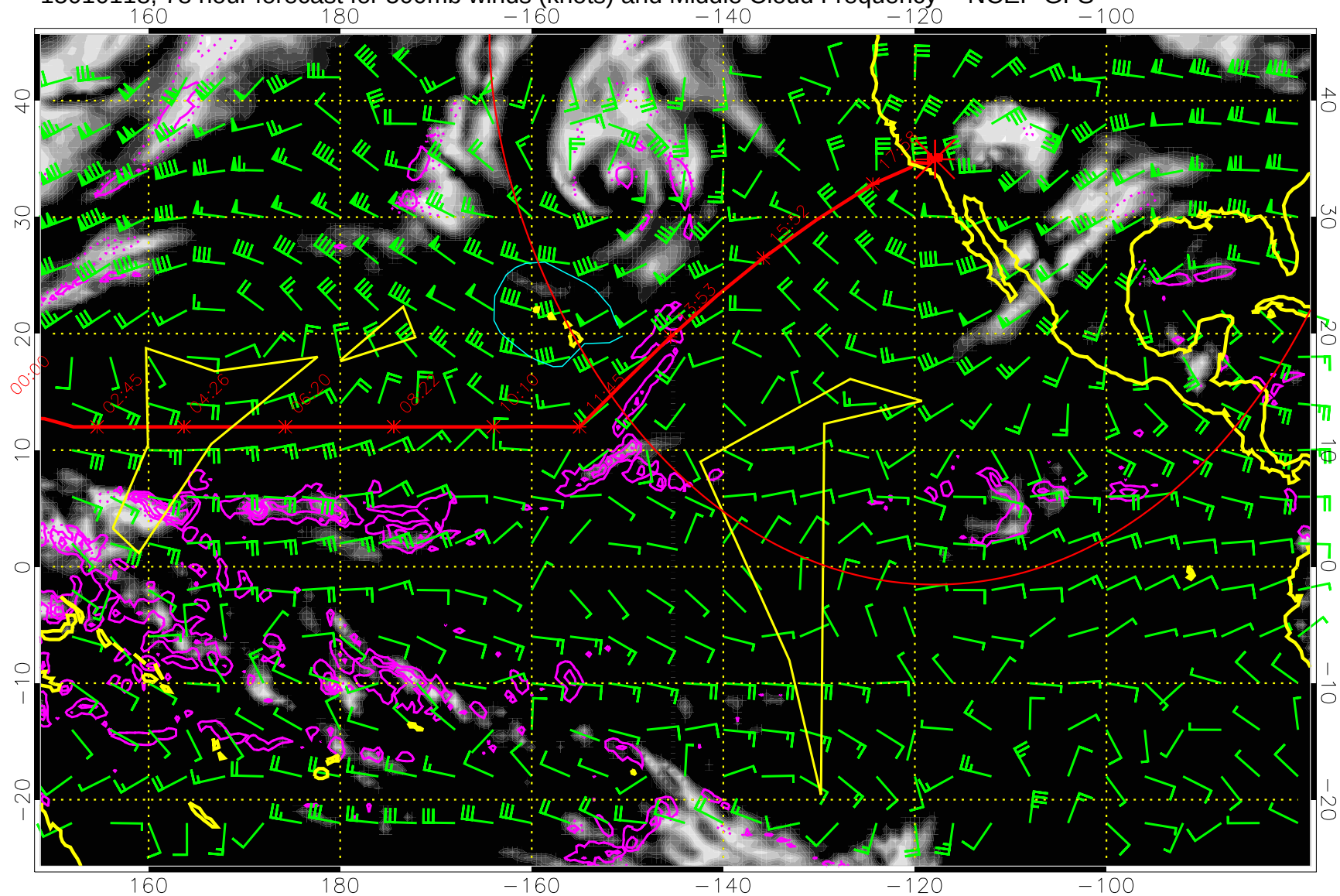
15010118, 78 hour forecast for 500mb winds (knots) and Middle Cloud Frequency -- NCEP GFS
