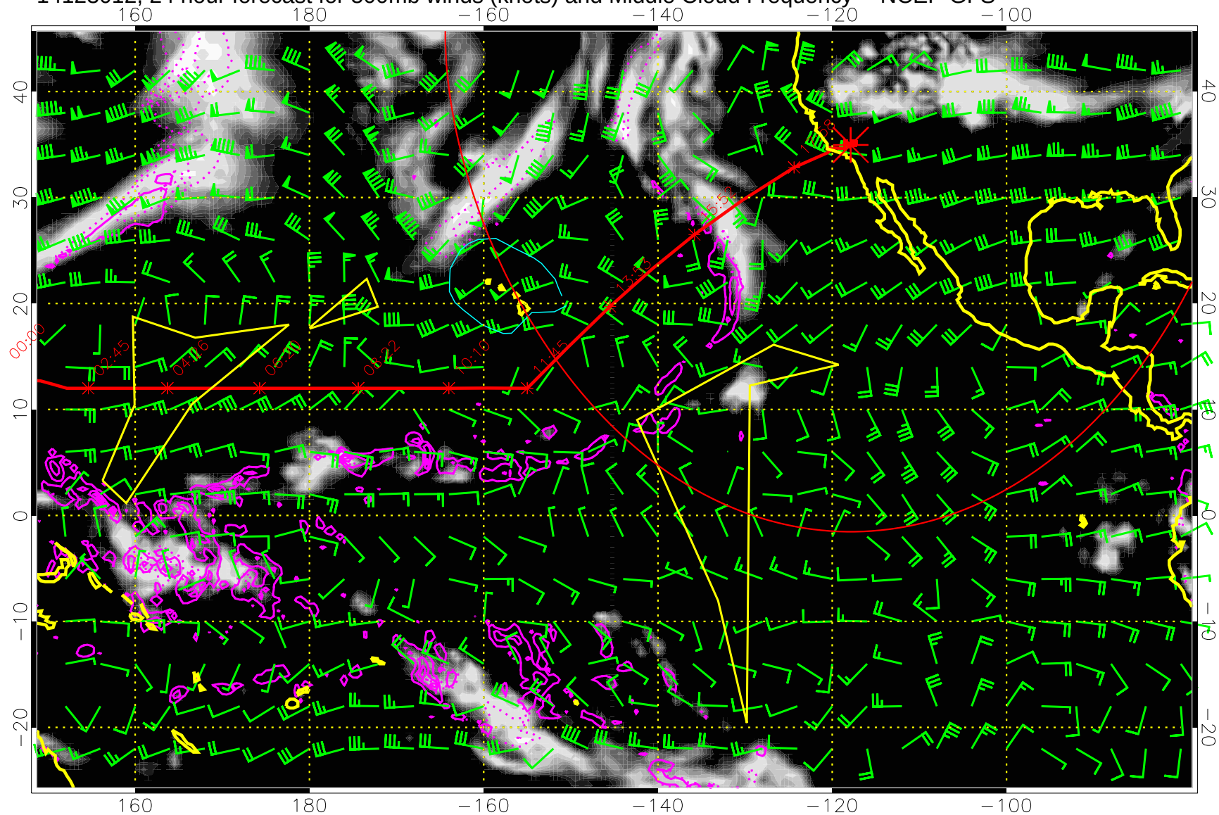
14123012, 24 hour forecast for 500mb winds (knots) and Middle Cloud Frequency -- NCEP GFS
