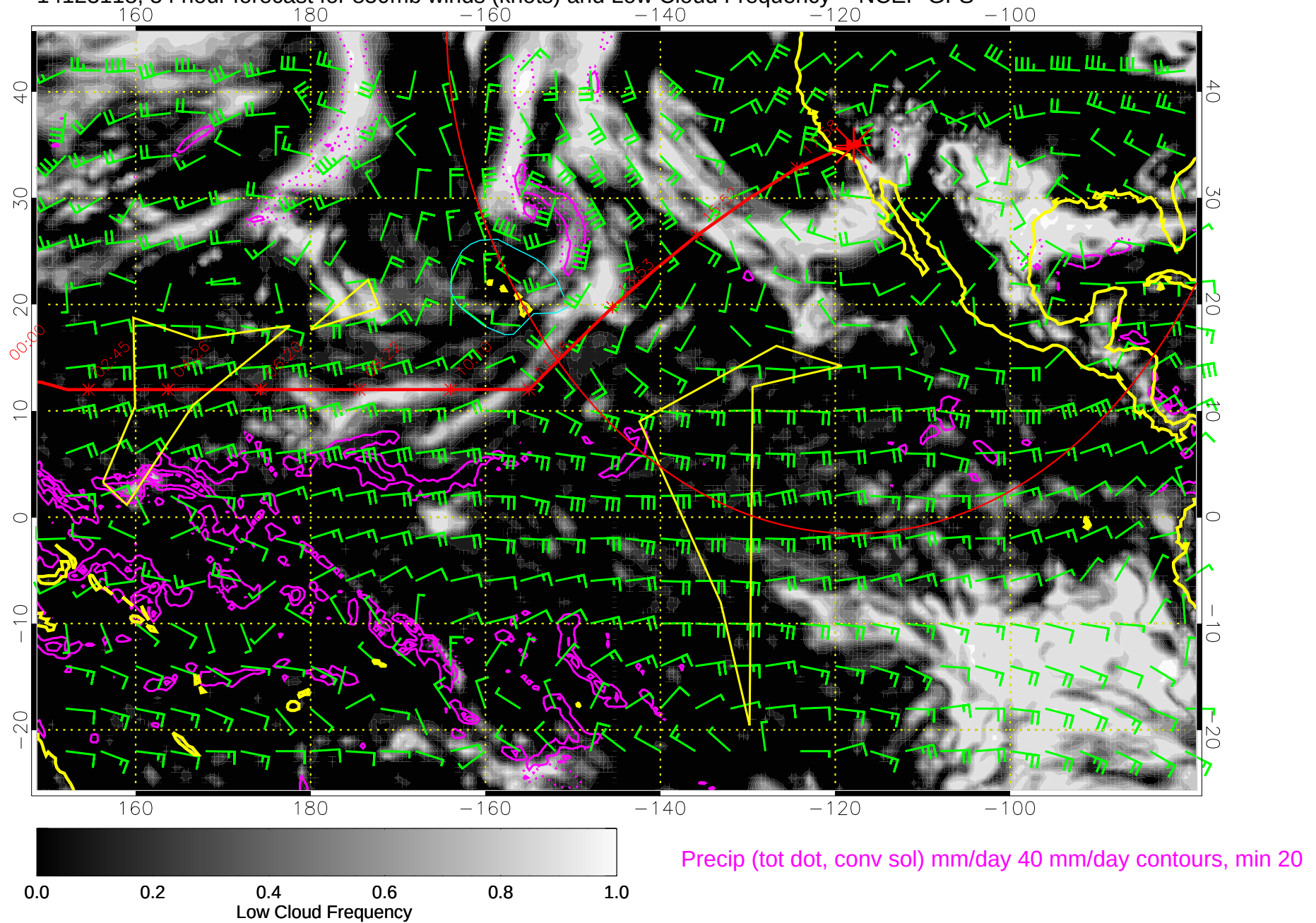
14123118, 54 hour forecast for 850mb winds (knots) and Low Cloud Frequency -- NCEP GFS
