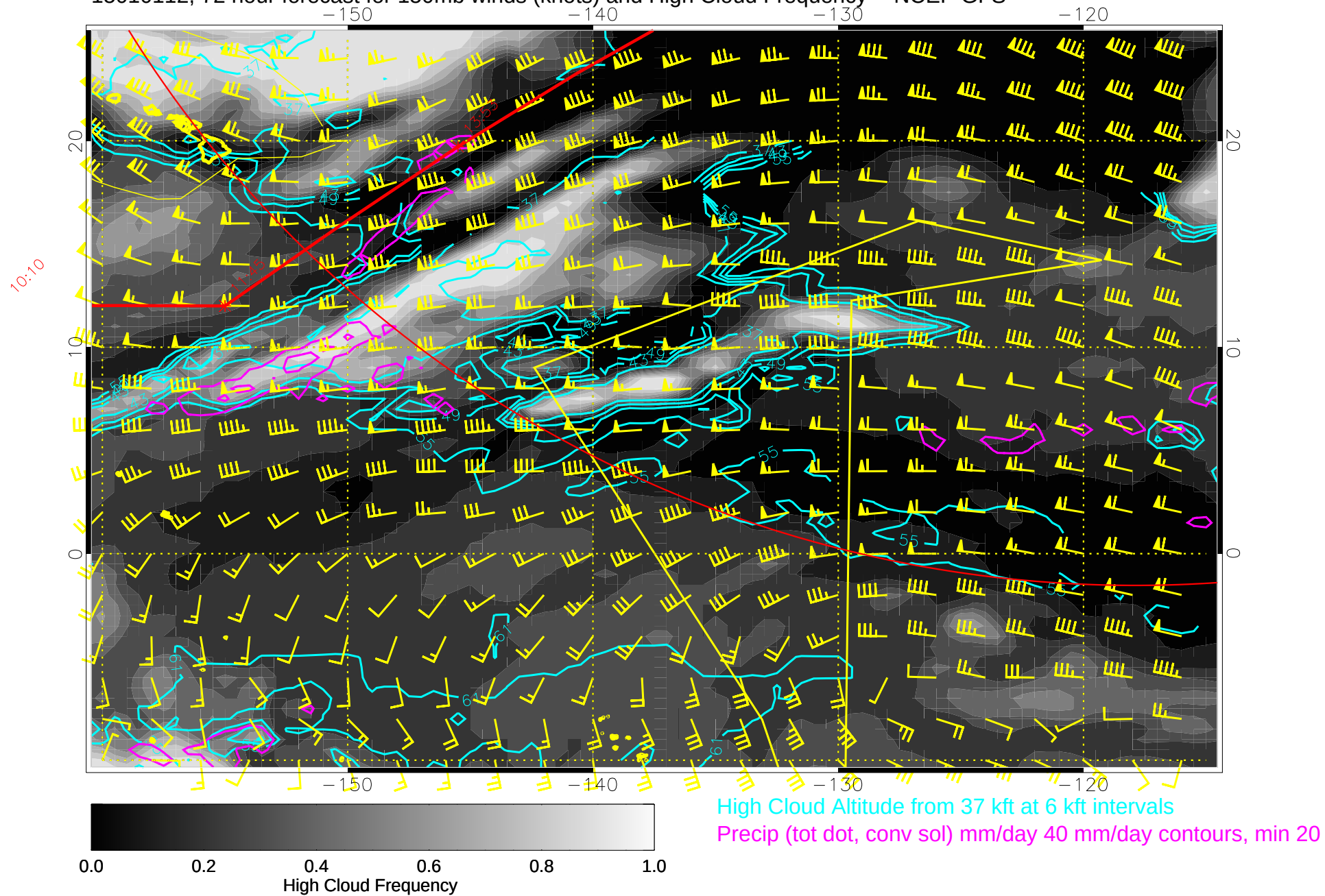
15010112, 72 hour forecast for 150mb winds (knots) and High Cloud Frequency -- NCEP GFS
