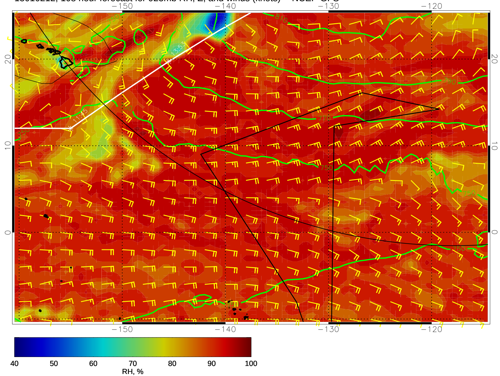
15010212, 108 hour forecast for 925mb RH, Z, and winds (knots) -- NCEP GFS
