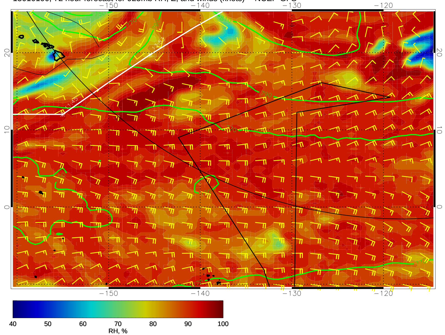
15010100, 72 hour forecast for 925mb RH, Z, and winds (knots) -- NCEP GFS
