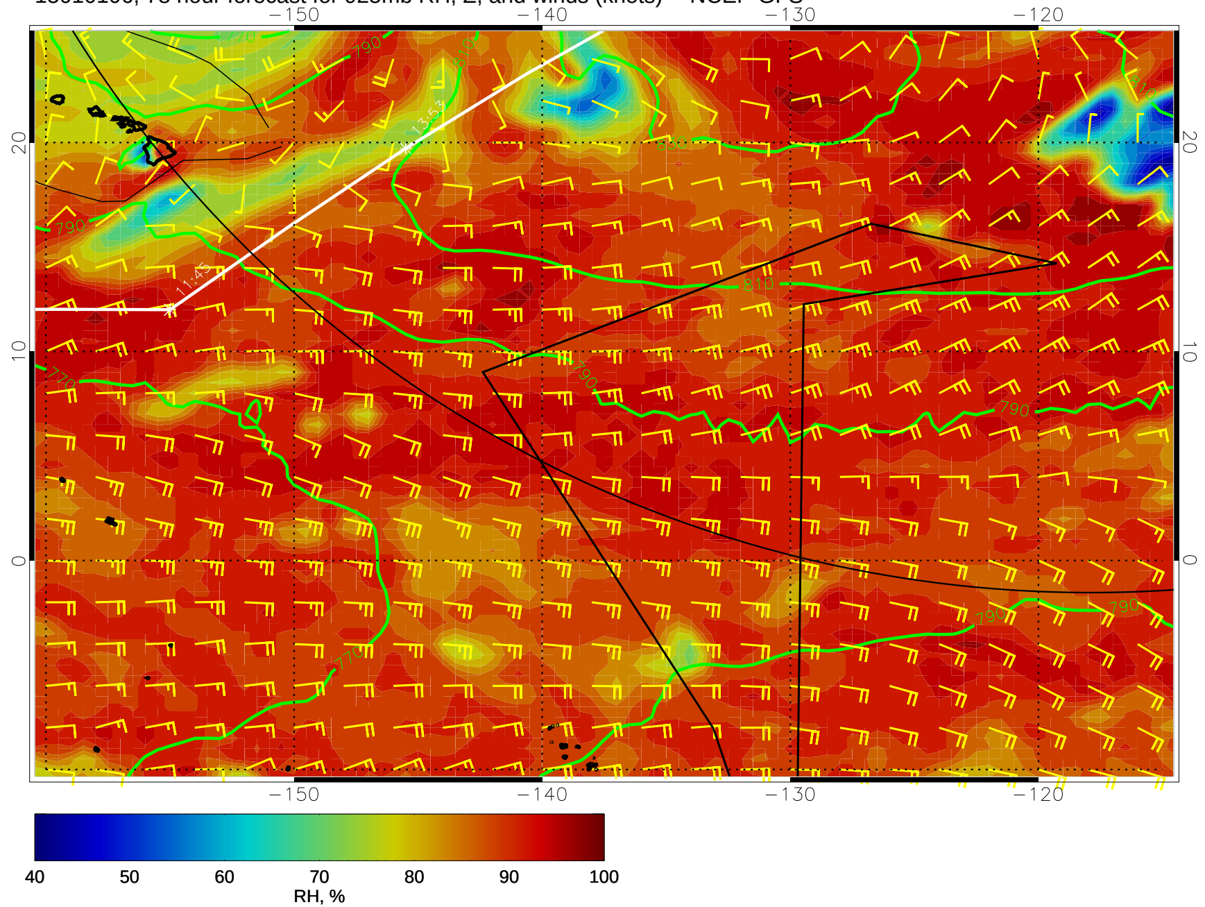
15010106, 78 hour forecast for 925mb RH, Z, and winds (knots) -- NCEP GFS
