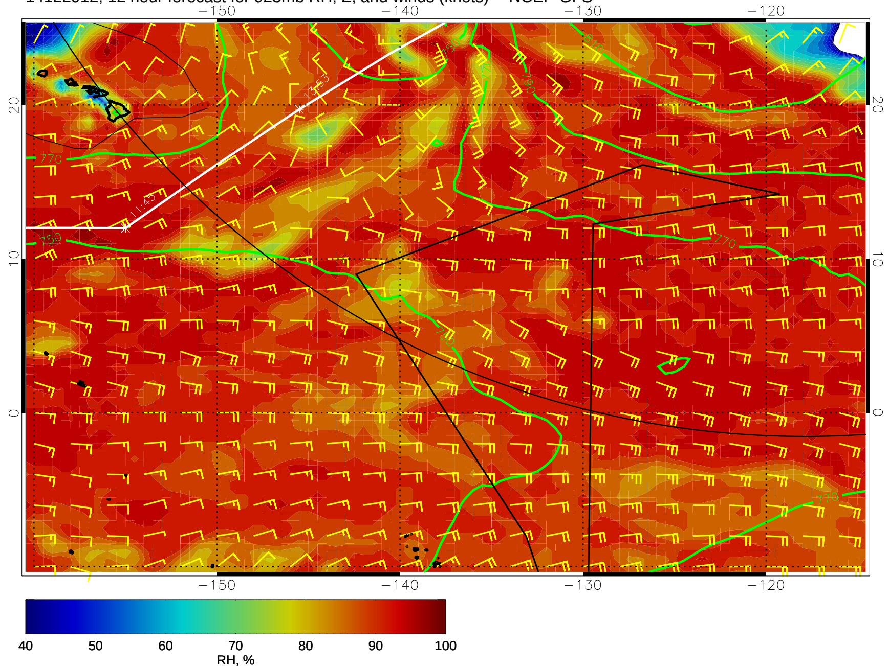
14122912, 12 hour forecast for 925mb RH, Z, and winds (knots) -- NCEP GFS
