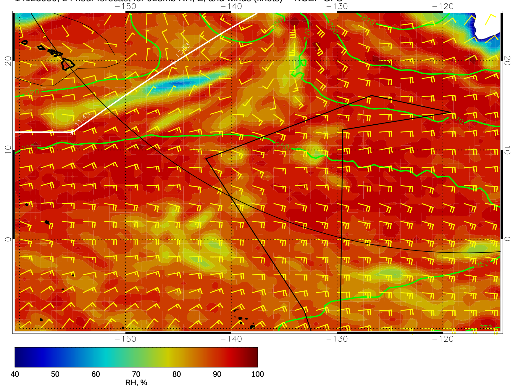
14123000, 24 hour forecast for 925mb RH, Z, and winds (knots) -- NCEP GFS
