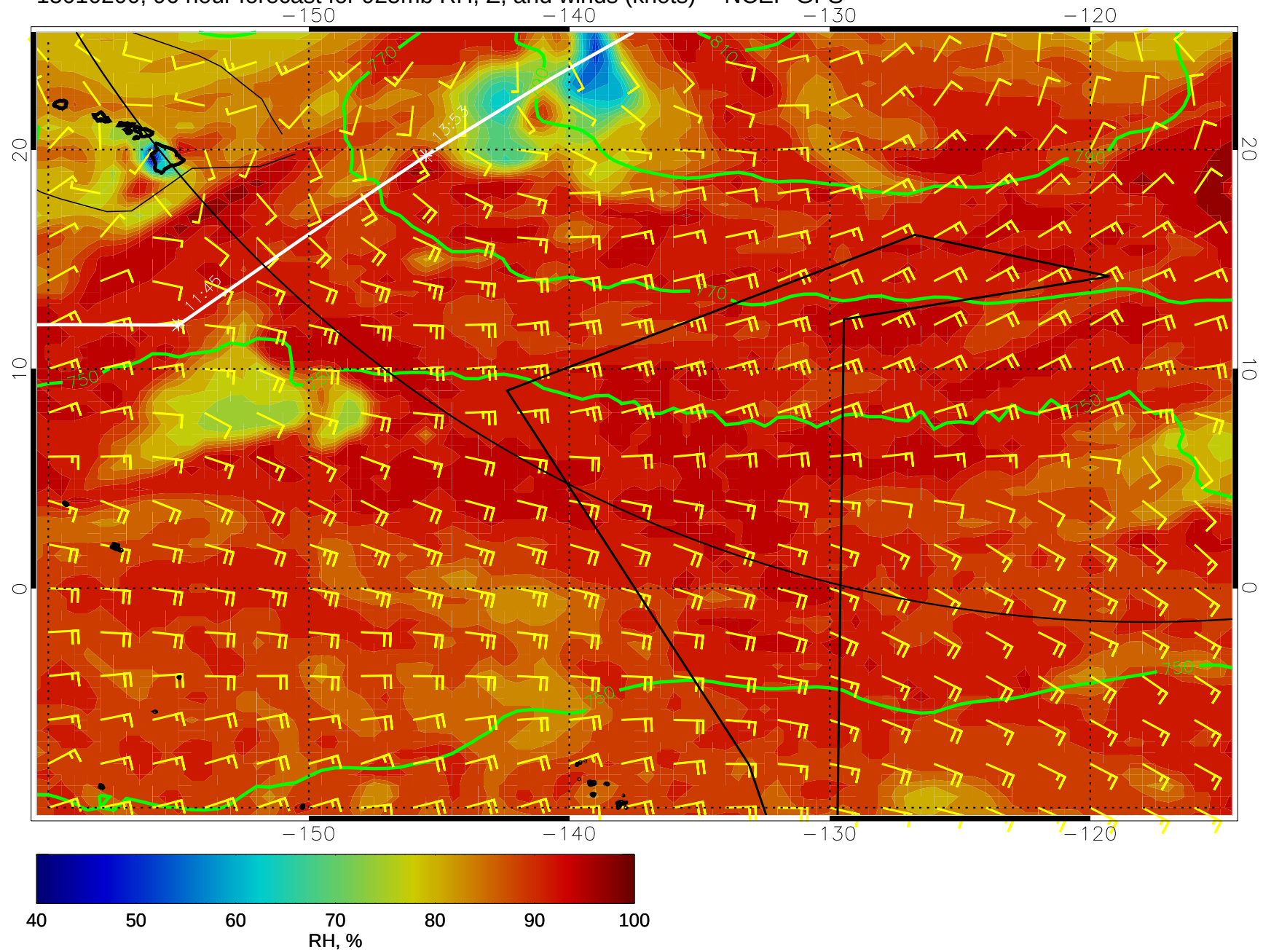
15010200, 96 hour forecast for 925mb RH, Z, and winds (knots) -- NCEP GFS
