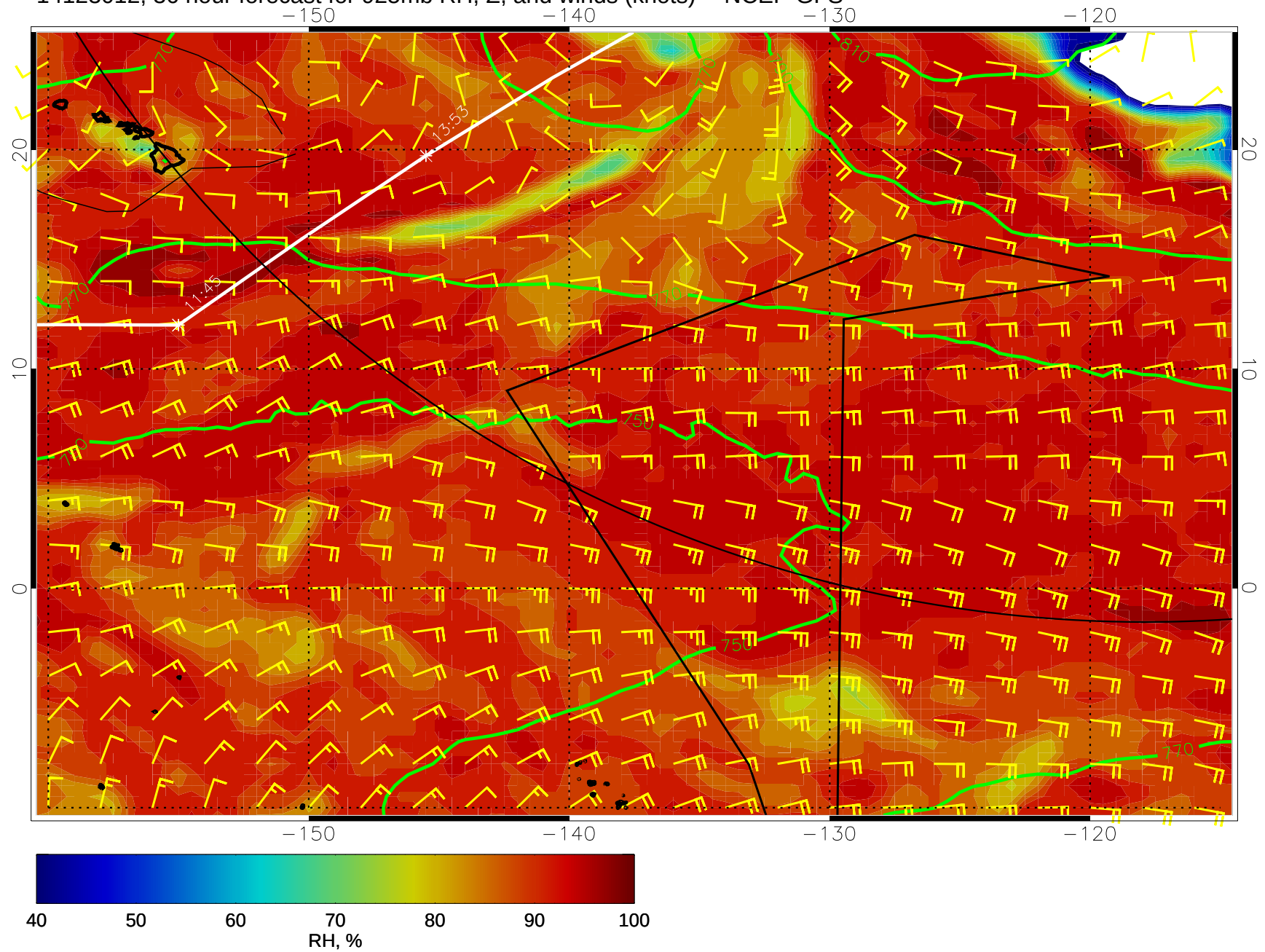
14123012, 36 hour forecast for 925mb RH, Z, and winds (knots) -- NCEP GFS
