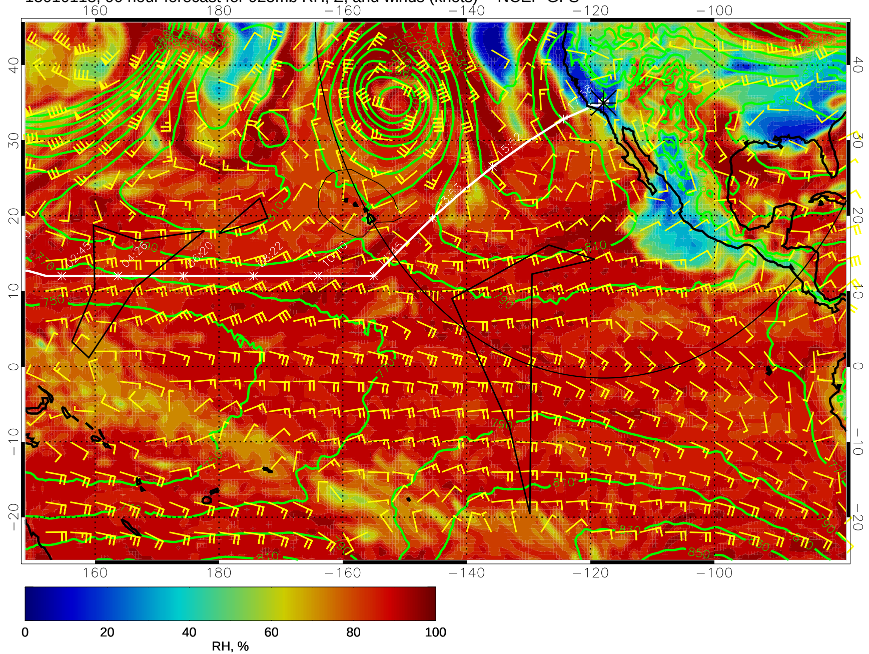
15010118, 90 hour forecast for 925mb RH, Z, and winds (knots) -- NCEP GFS
