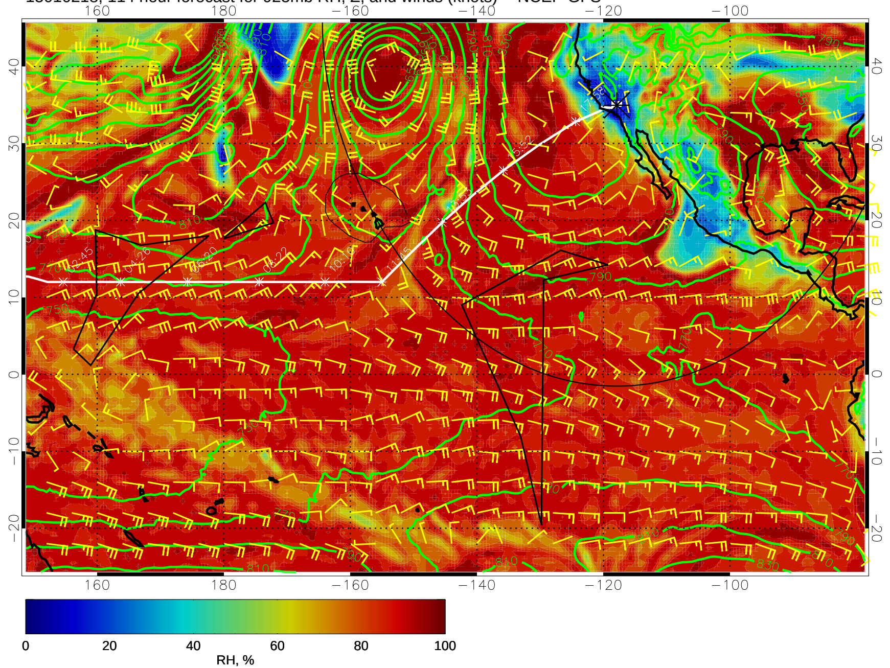
15010218, 114 hour forecast for 925mb RH, Z, and winds (knots) -- NCEP GFS
