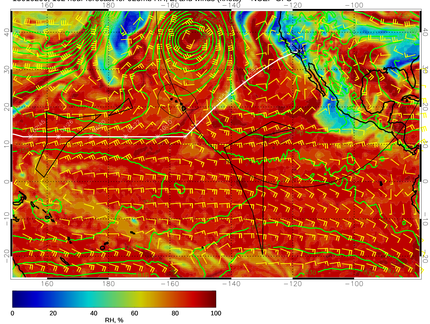
15010206, 102 hour forecast for 925mb RH, Z, and winds (knots) -- NCEP GFS
