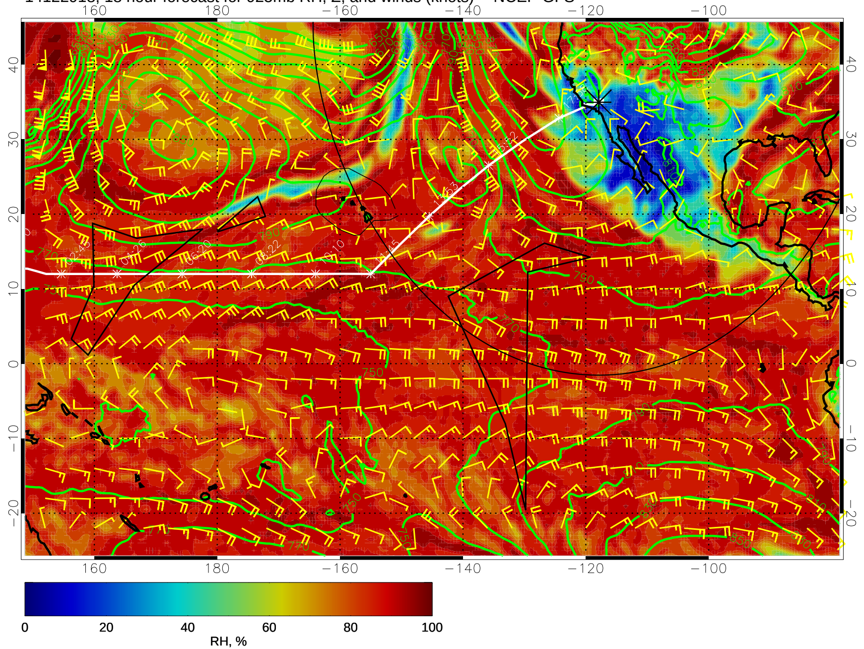
14122918, 18 hour forecast for 925mb RH, Z, and winds (knots) -- NCEP GFS
