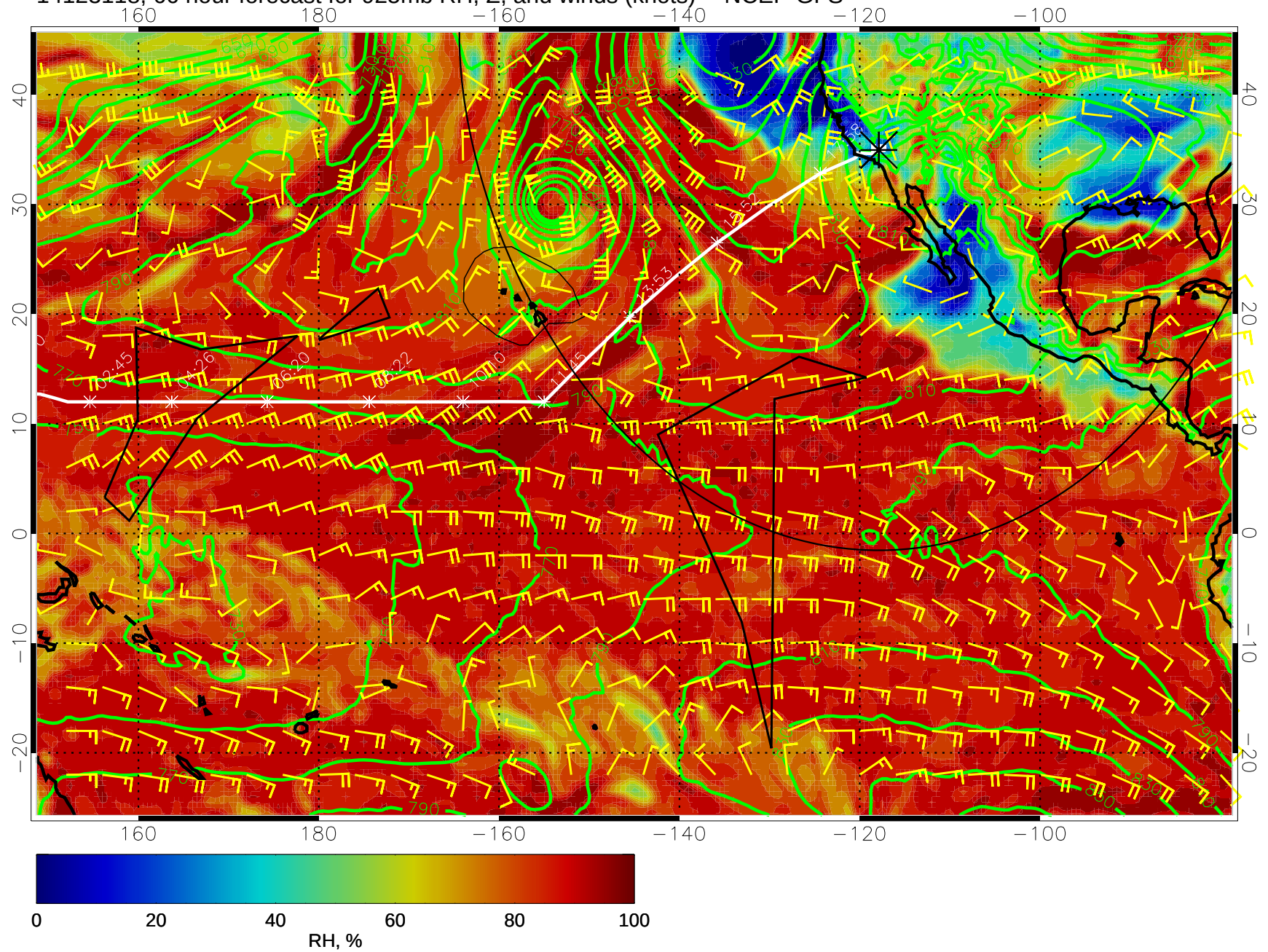
14123118, 66 hour forecast for 925mb RH, Z, and winds (knots) -- NCEP GFS
