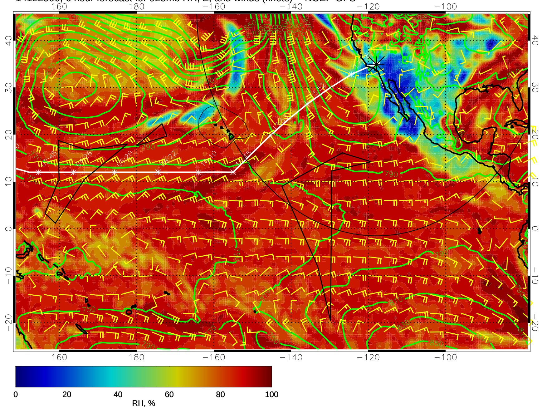
14122906, 6 hour forecast for 925mb RH, Z, and winds (knots) -- NCEP GFS
