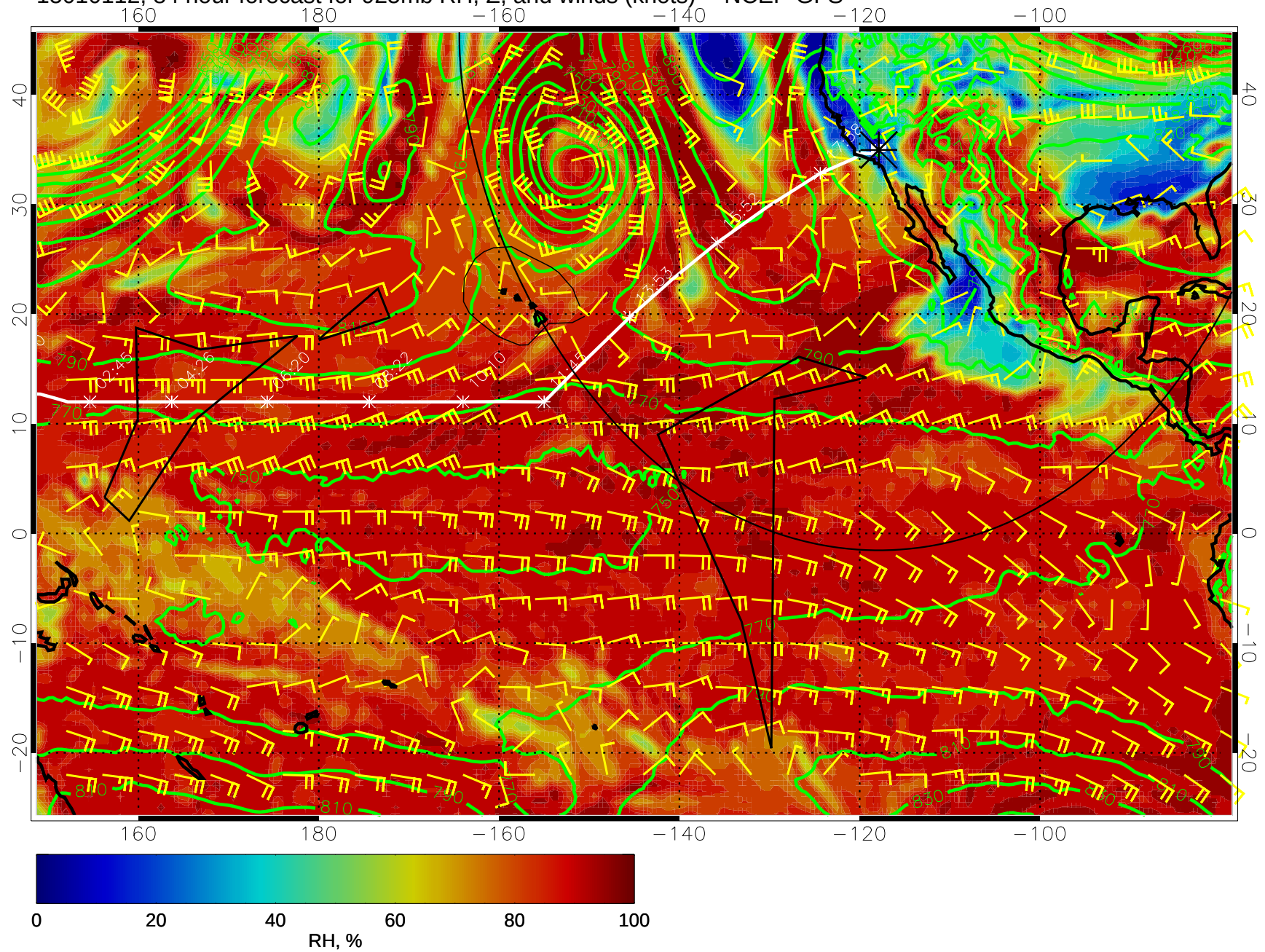
15010112, 84 hour forecast for 925mb RH, Z, and winds (knots) -- NCEP GFS
