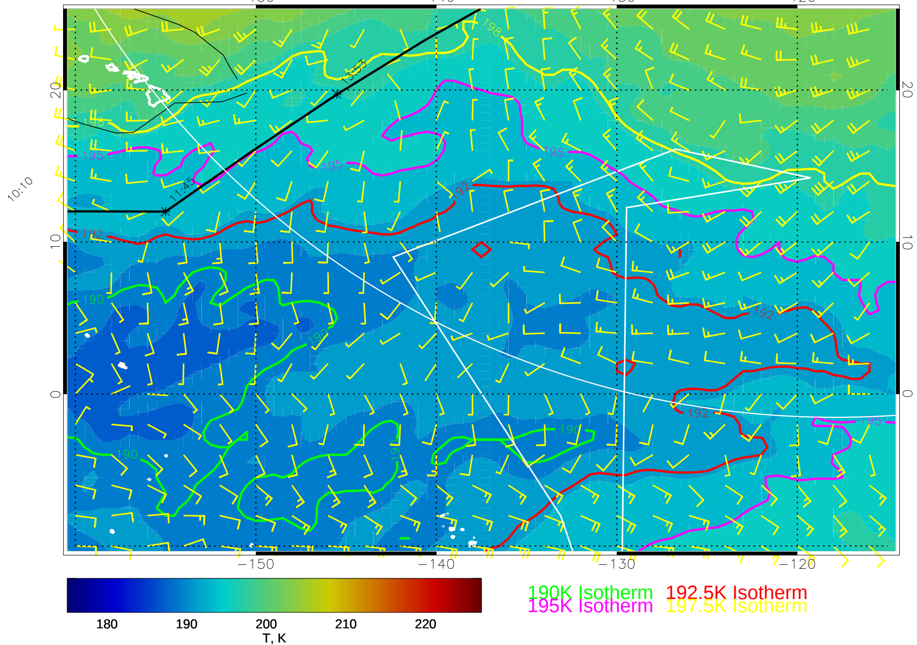
14123112, 60 hour forecast for 70mb T and winds (knots) -- NCEP GFS
