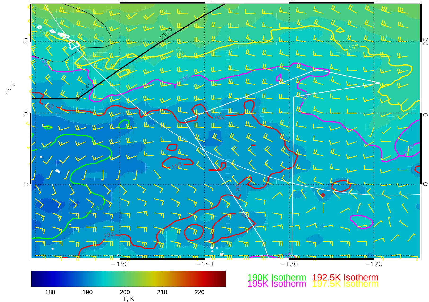
15010206, 102 hour forecast for 70mb T and winds (knots) -- NCEP GFS
