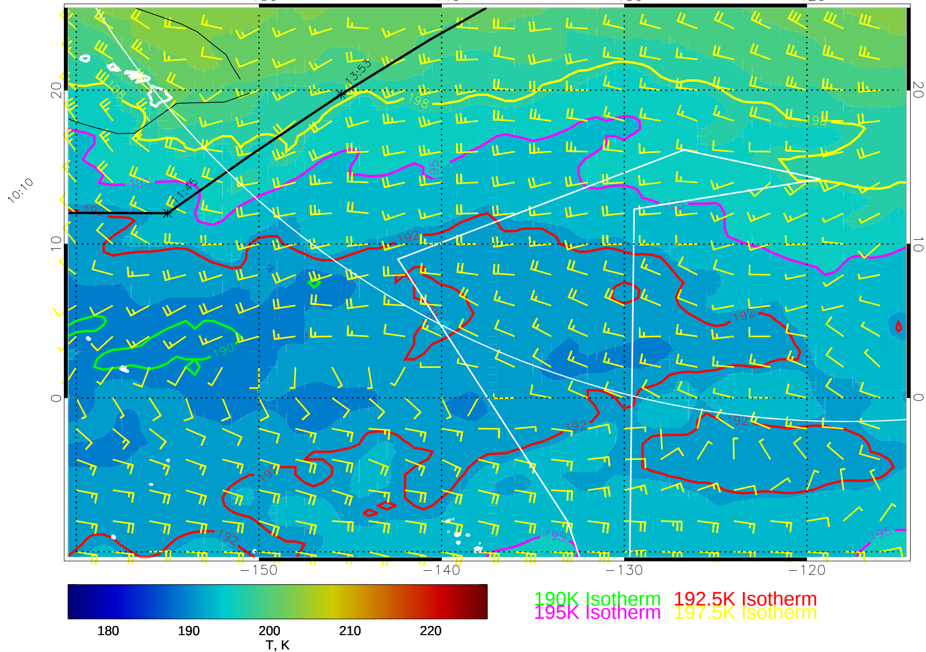
15010200, 96 hour forecast for 70mb T and winds (knots) -- NCEP GFS
