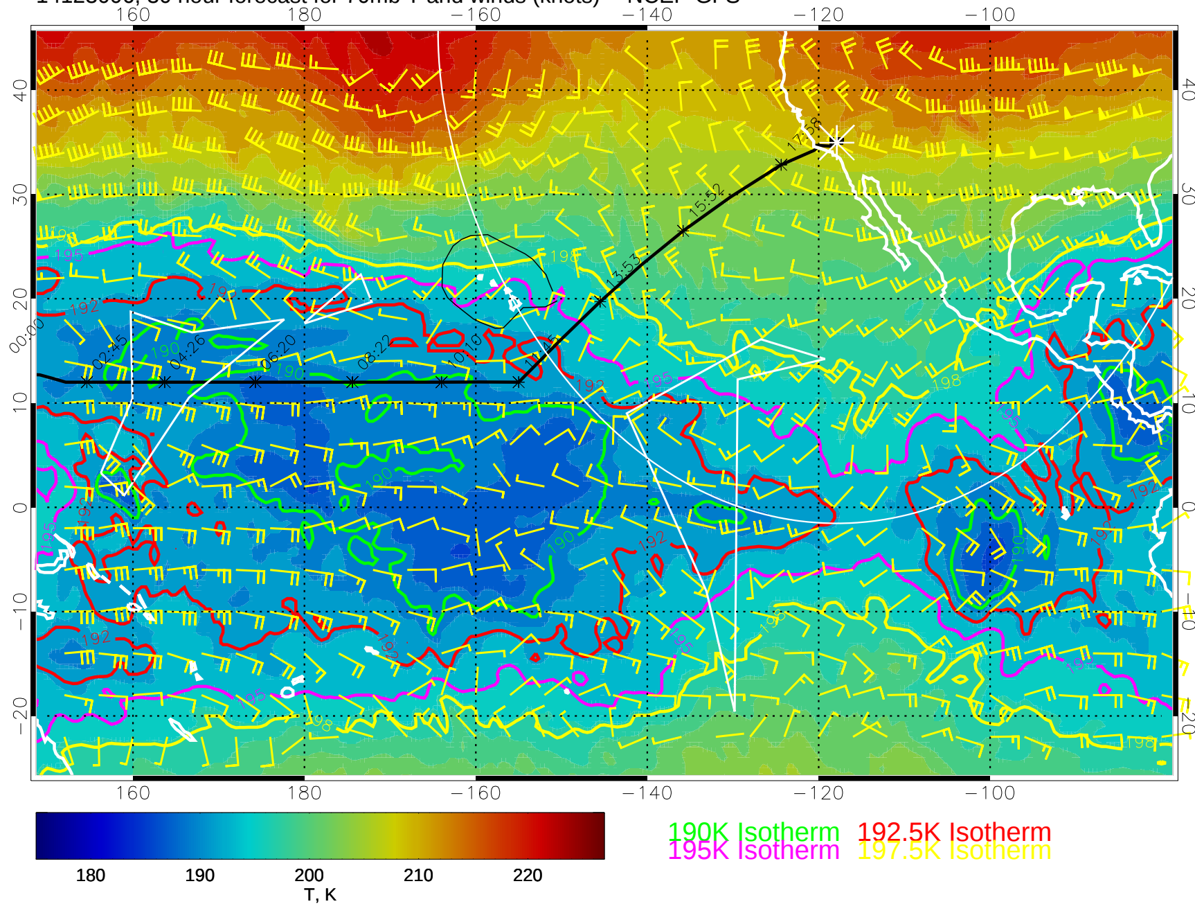
14123006, 30 hour forecast for 70mb T and winds (knots) -- NCEP GFS
