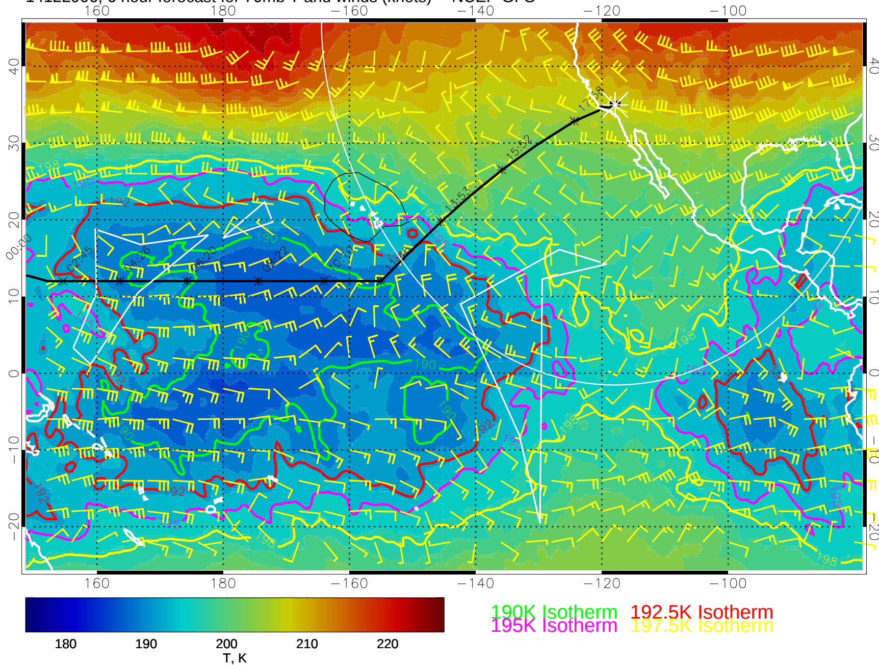
14122906, 6 hour forecast for 70mb T and winds (knots) -- NCEP GFS
