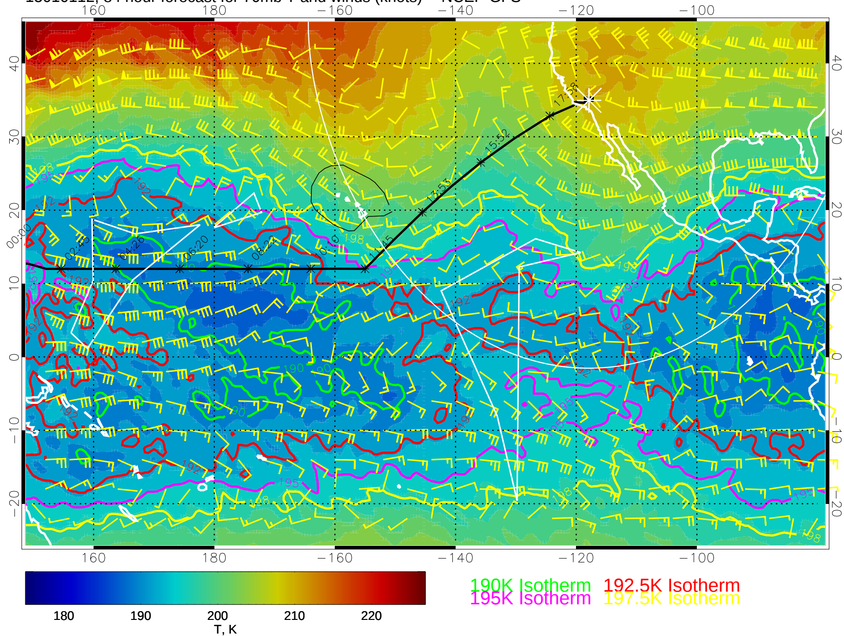
15010112, 84 hour forecast for 70mb T and winds (knots) -- NCEP GFS
