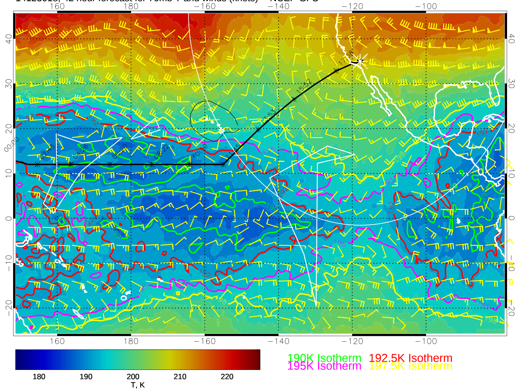
14123018, 42 hour forecast for 70mb T and winds (knots) -- NCEP GFS
