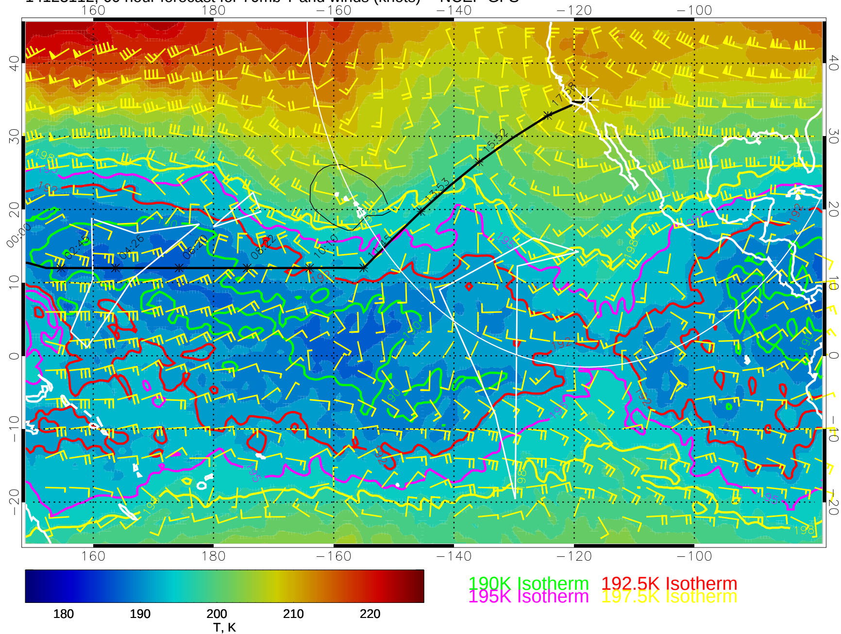
14123112, 60 hour forecast for 70mb T and winds (knots) -- NCEP GFS
