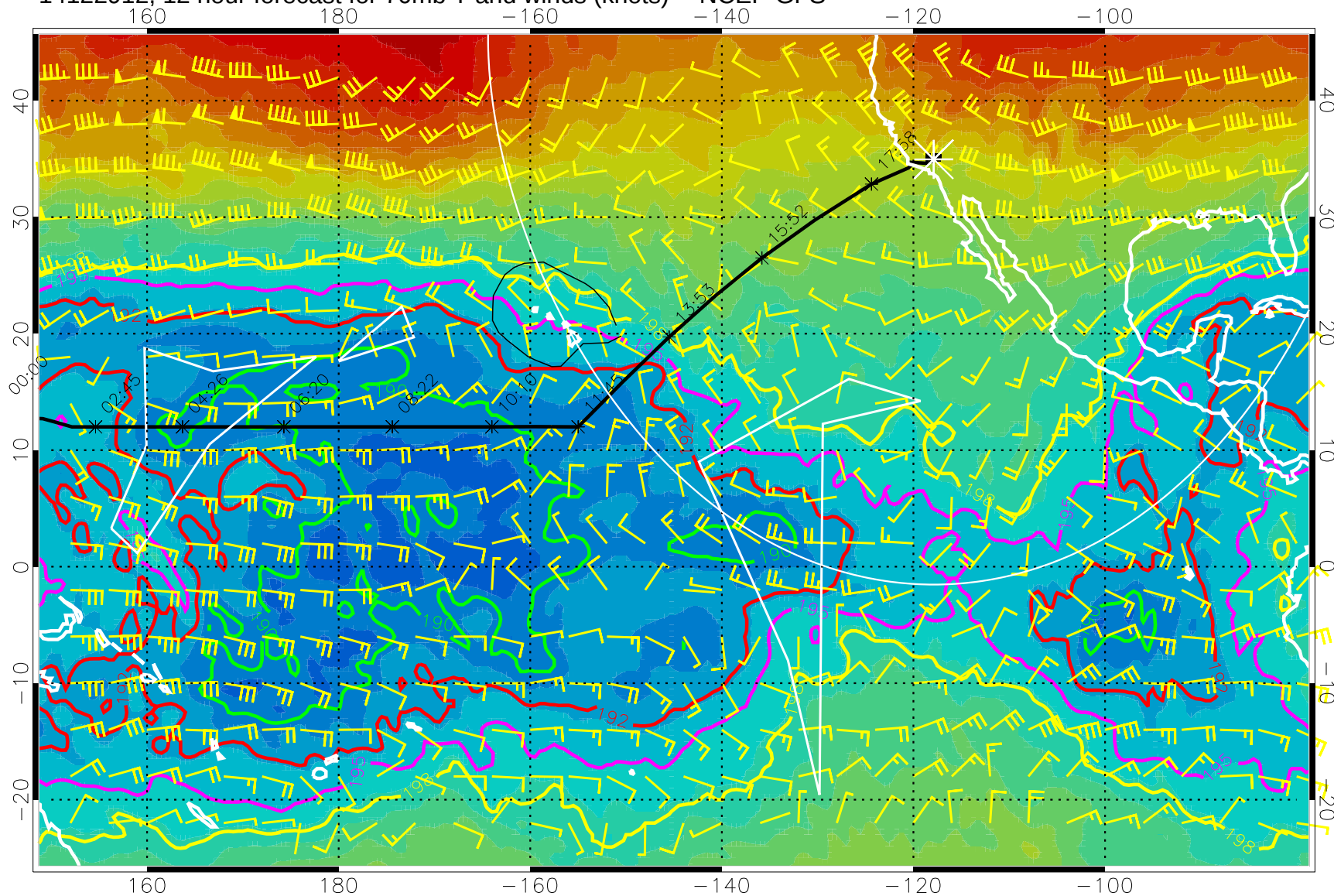
14122912, 12 hour forecast for 70mb T and winds (knots) -- NCEP GFS
