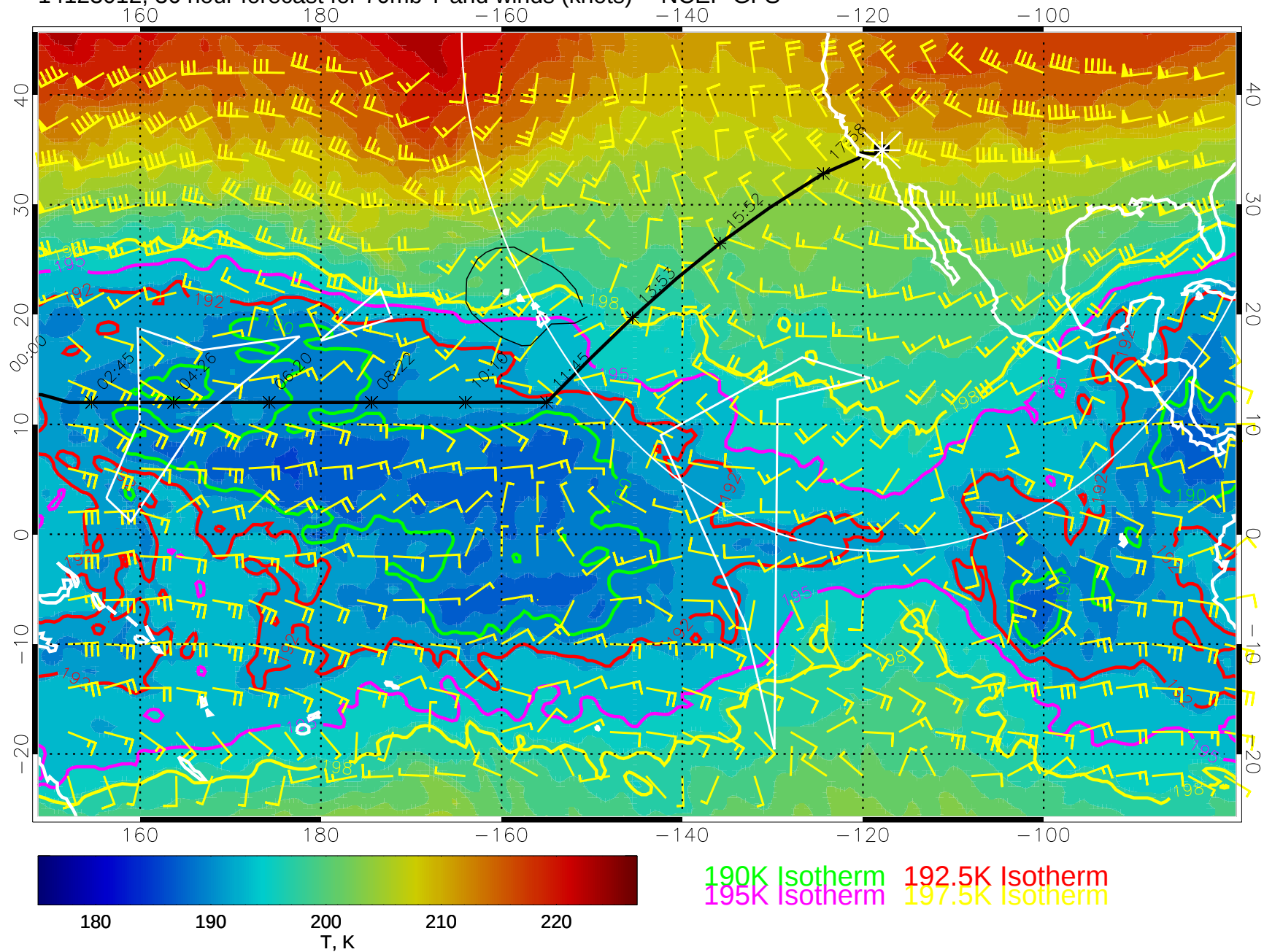
14123012, 36 hour forecast for 70mb T and winds (knots) -- NCEP GFS
