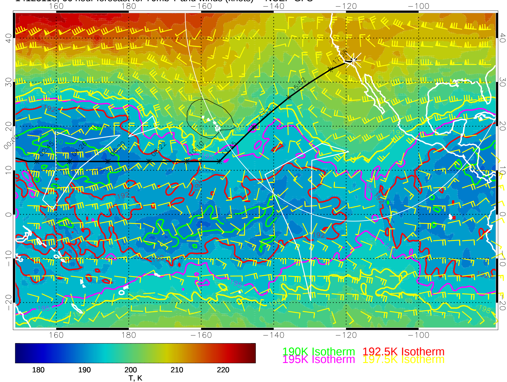
14123118, 66 hour forecast for 70mb T and winds (knots) -- NCEP GFS
