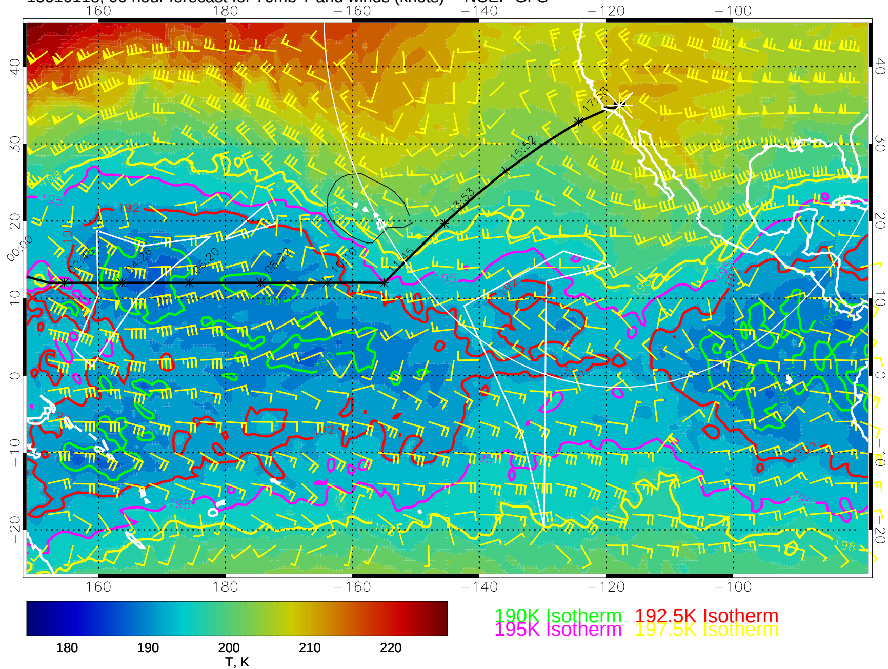
15010118, 90 hour forecast for 70mb T and winds (knots) -- NCEP GFS
