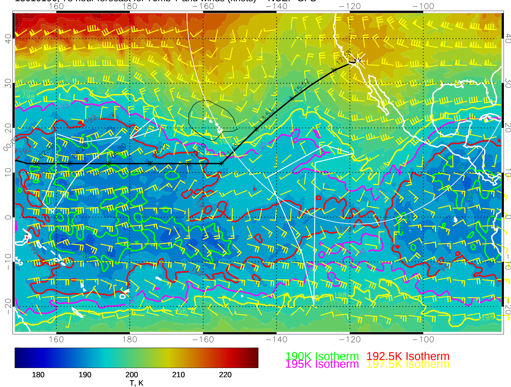
15010106, 78 hour forecast for 70mb T and winds (knots) -- NCEP GFS
