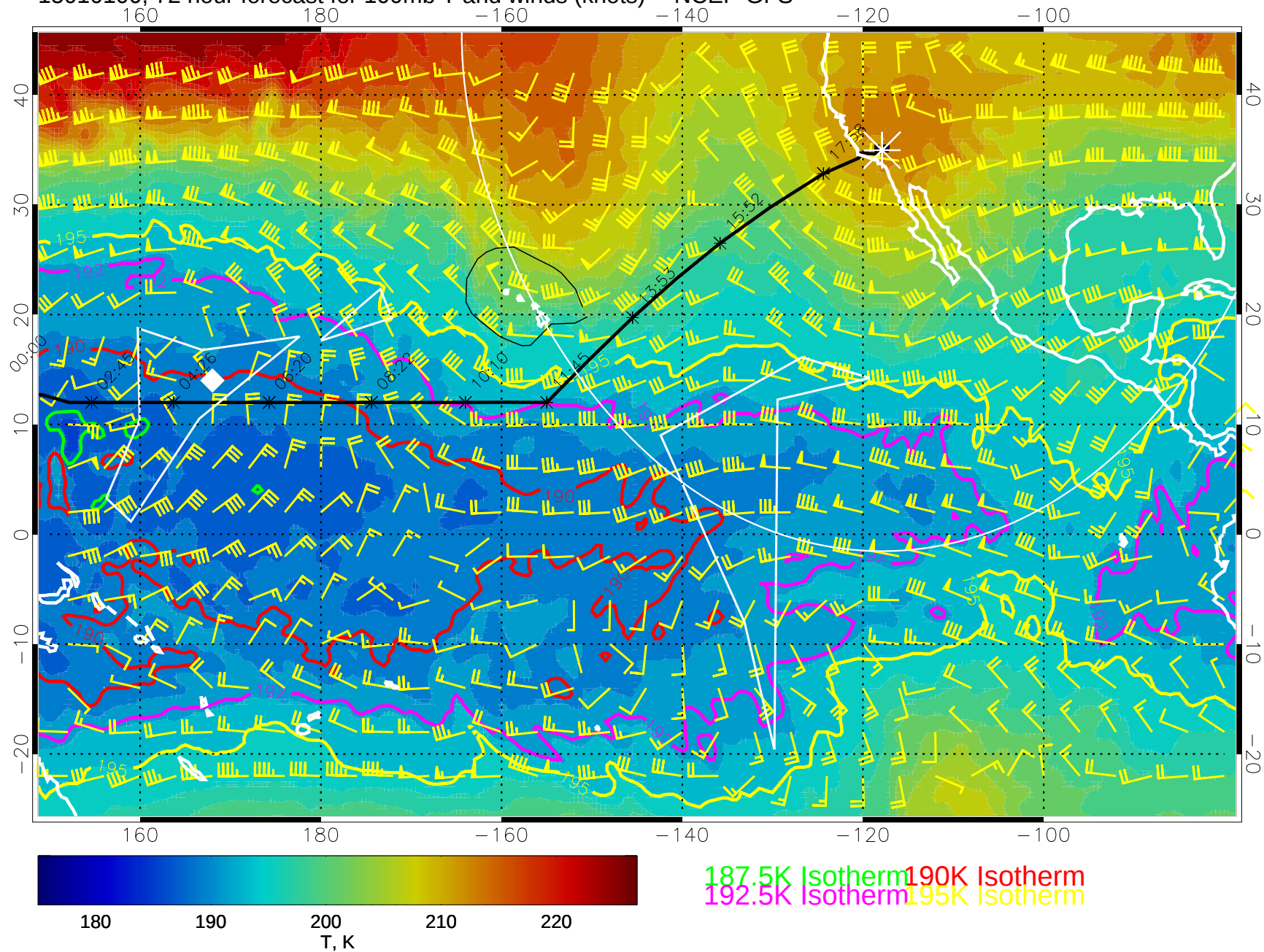
15010100, 72 hour forecast for 100mb T and winds (knots) -- NCEP GFS
