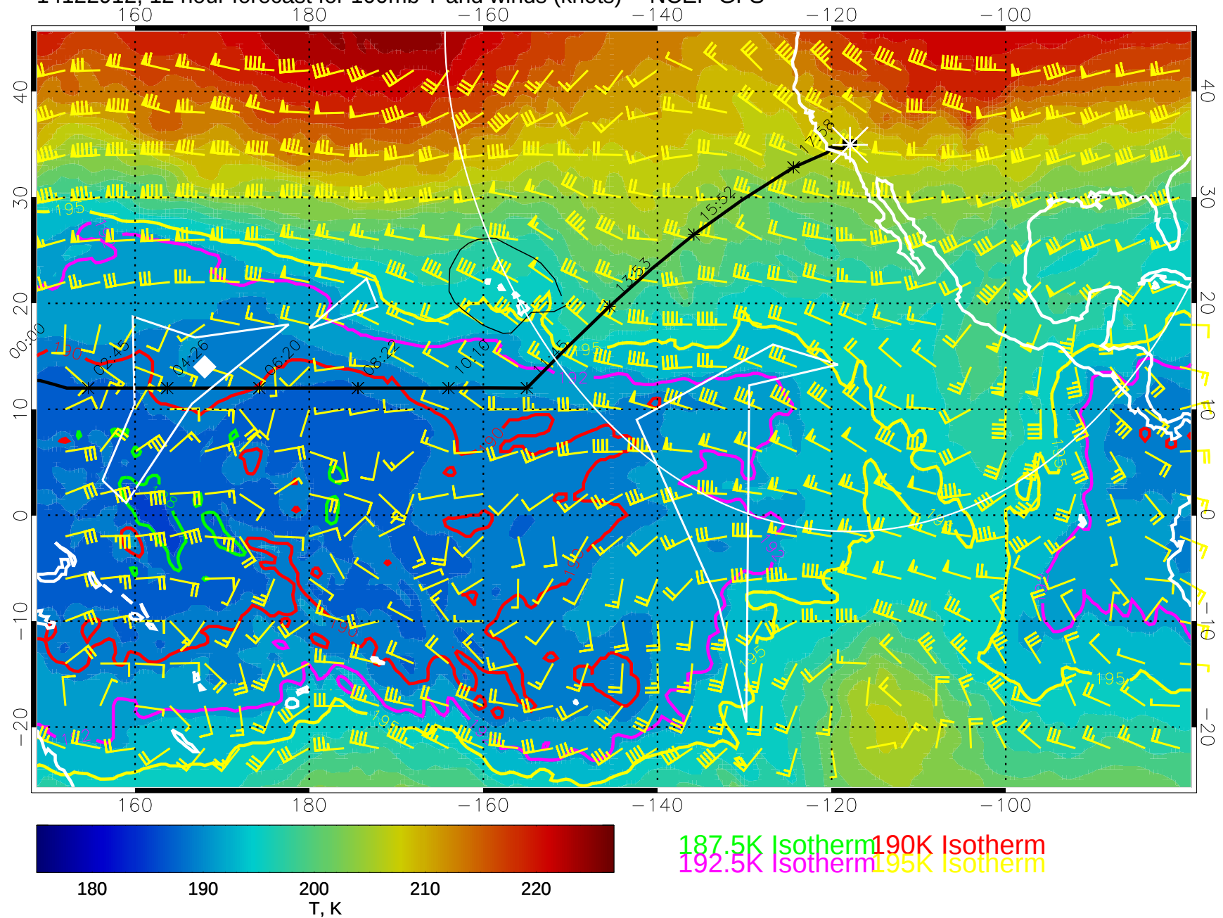
14122912, 12 hour forecast for 100mb T and winds (knots) -- NCEP GFS
