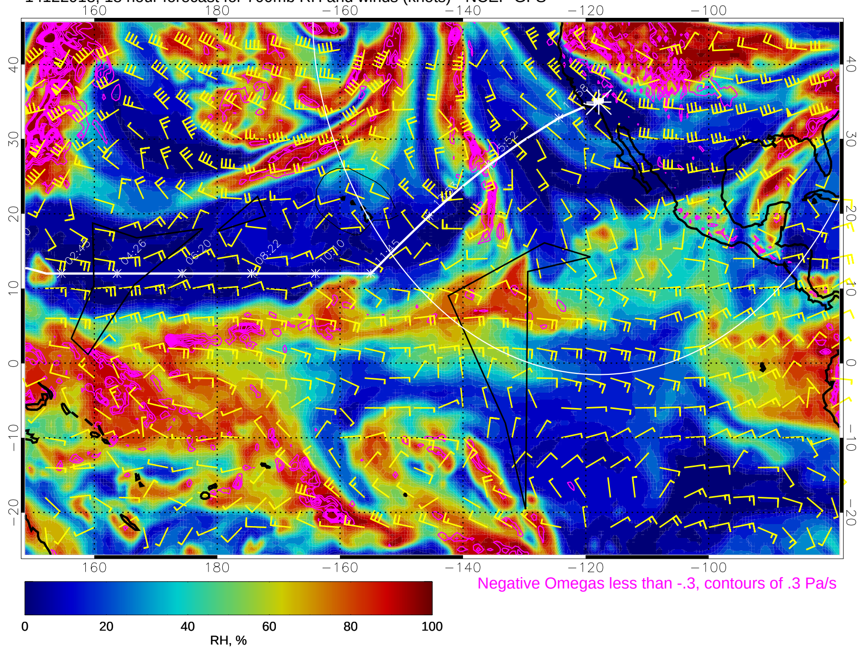
14122918, 18 hour forecast for 700mb RH and winds (knots) - NCEP GFS
