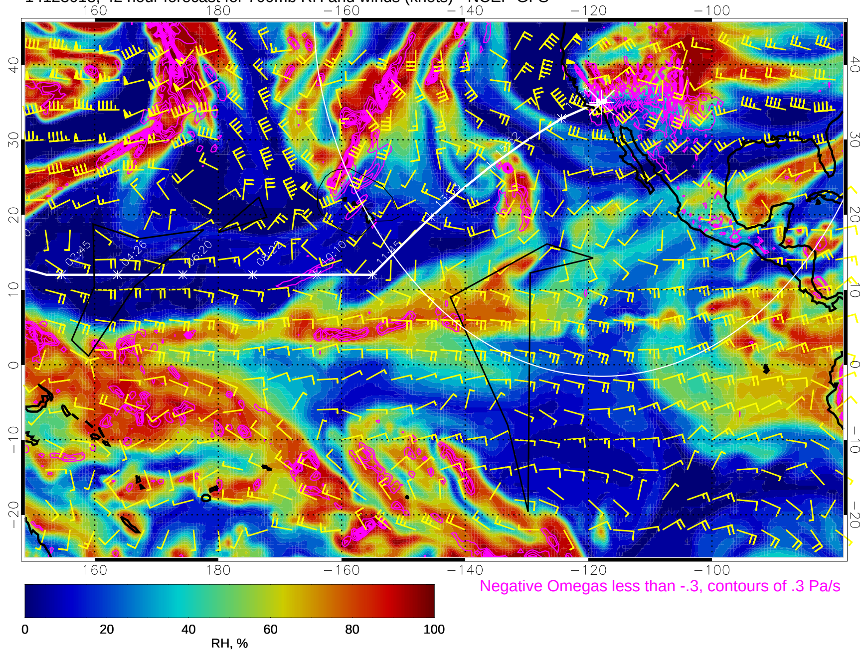
14123018, 42 hour forecast for 700mb RH and winds (knots) - NCEP GFS
