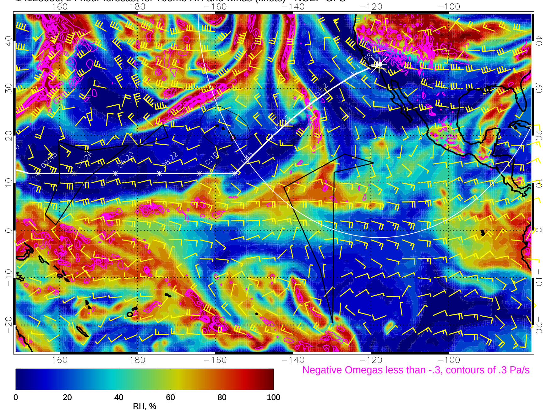
14123000, 24 hour forecast for 700mb RH and winds (knots) - NCEP GFS
