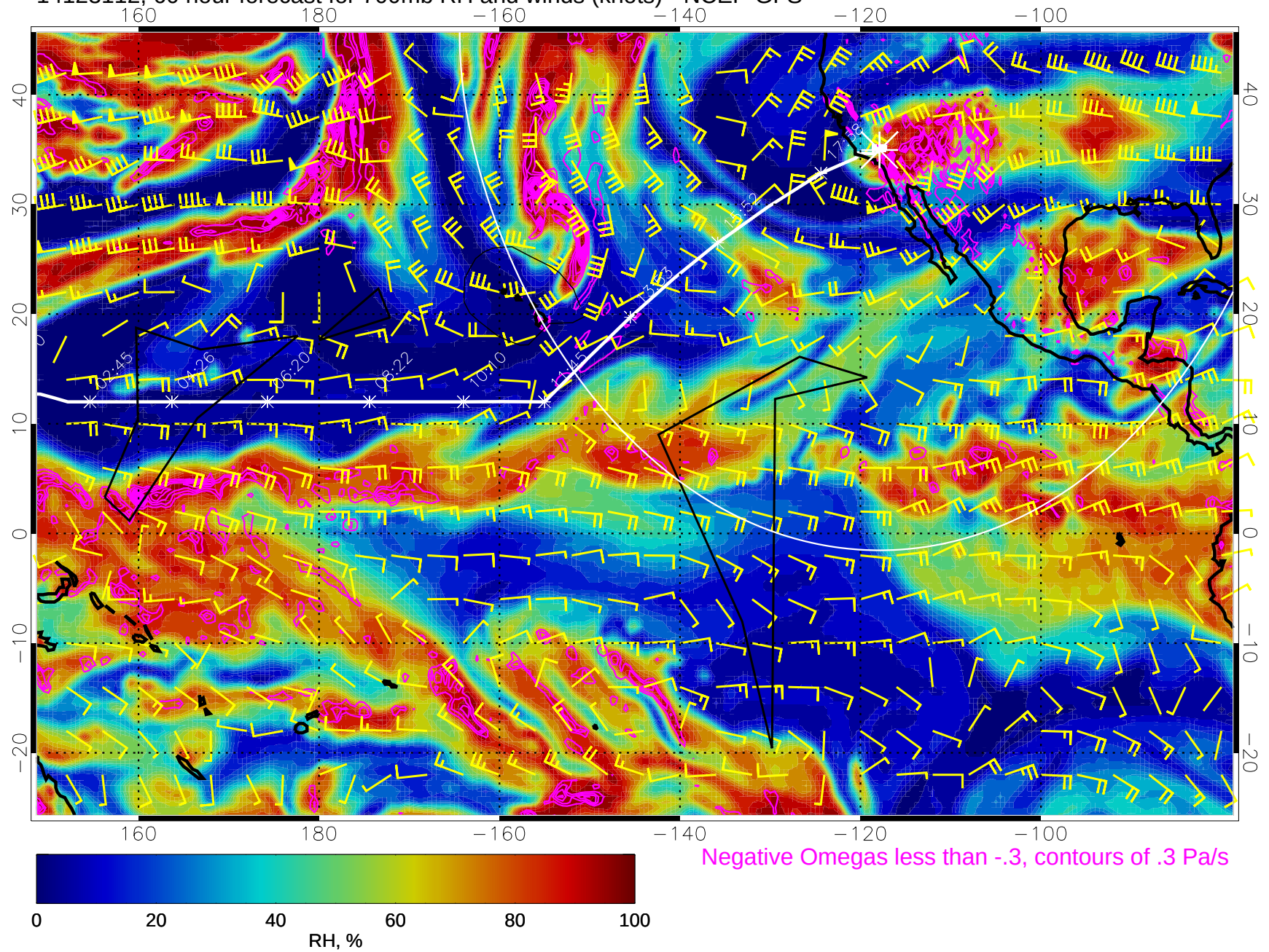
14123112, 60 hour forecast for 700mb RH and winds (knots) - NCEP GFS
