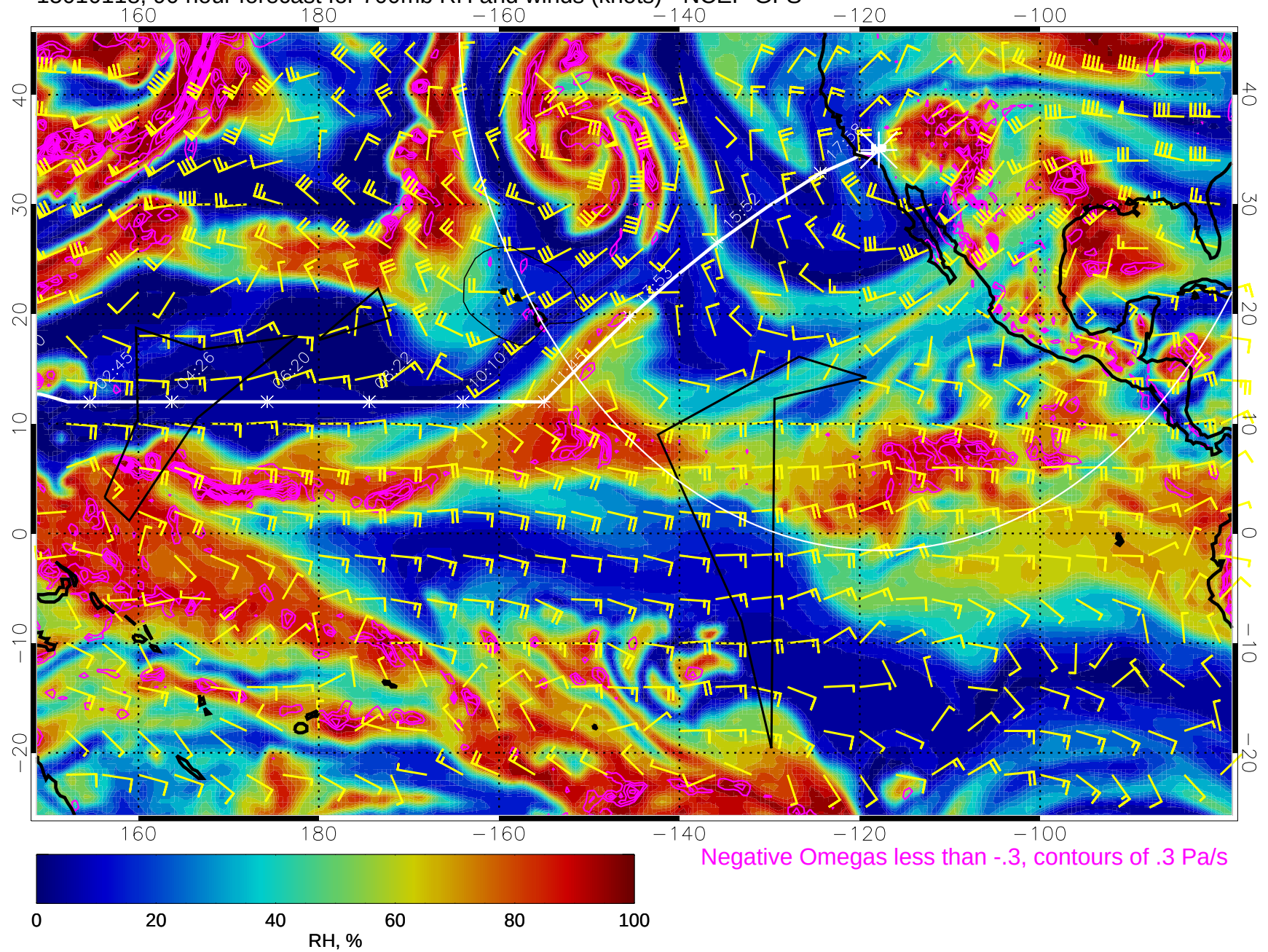
15010118, 90 hour forecast for 700mb RH and winds (knots) - NCEP GFS
