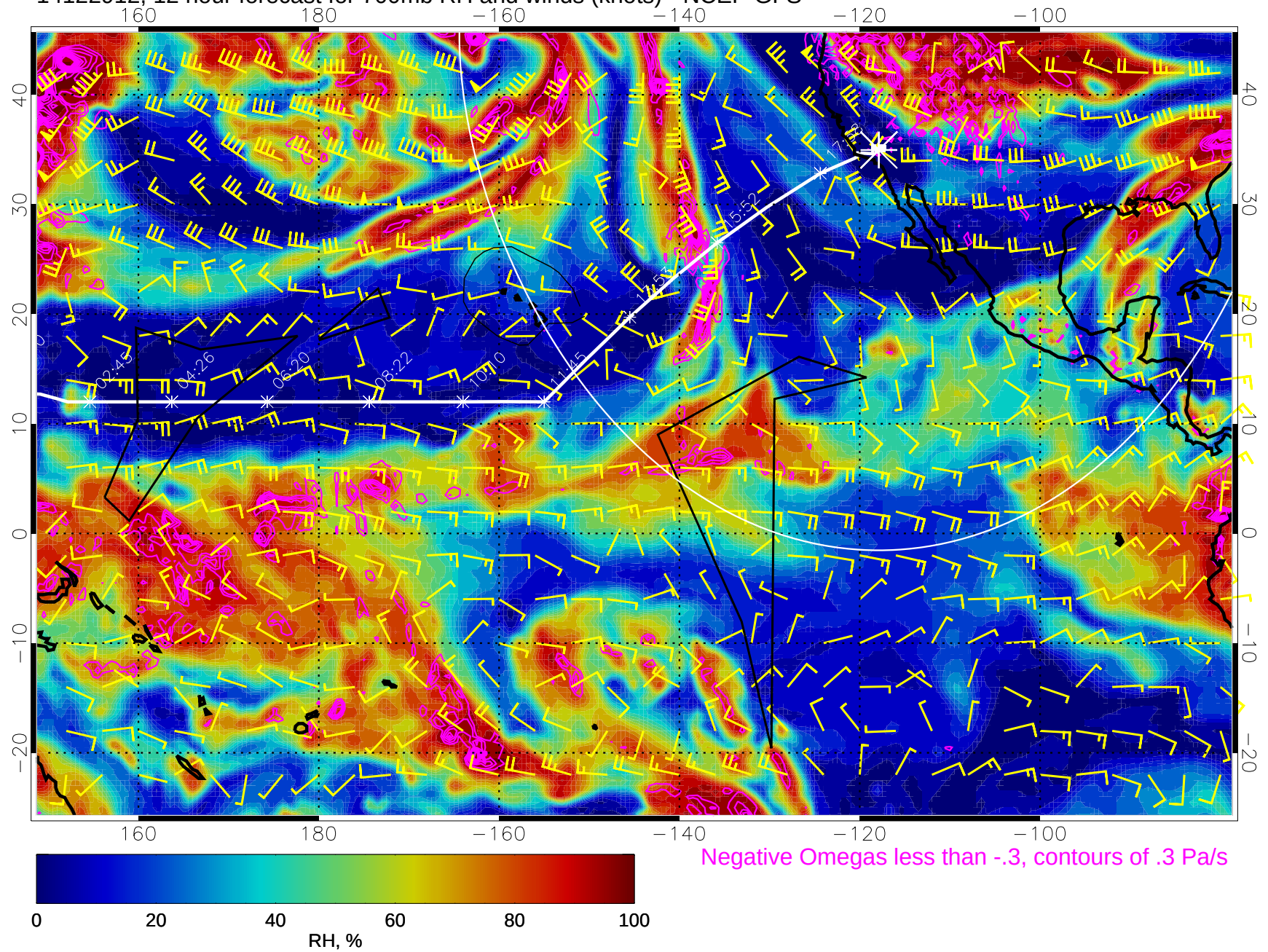
14122912, 12 hour forecast for 700mb RH and winds (knots) - NCEP GFS
