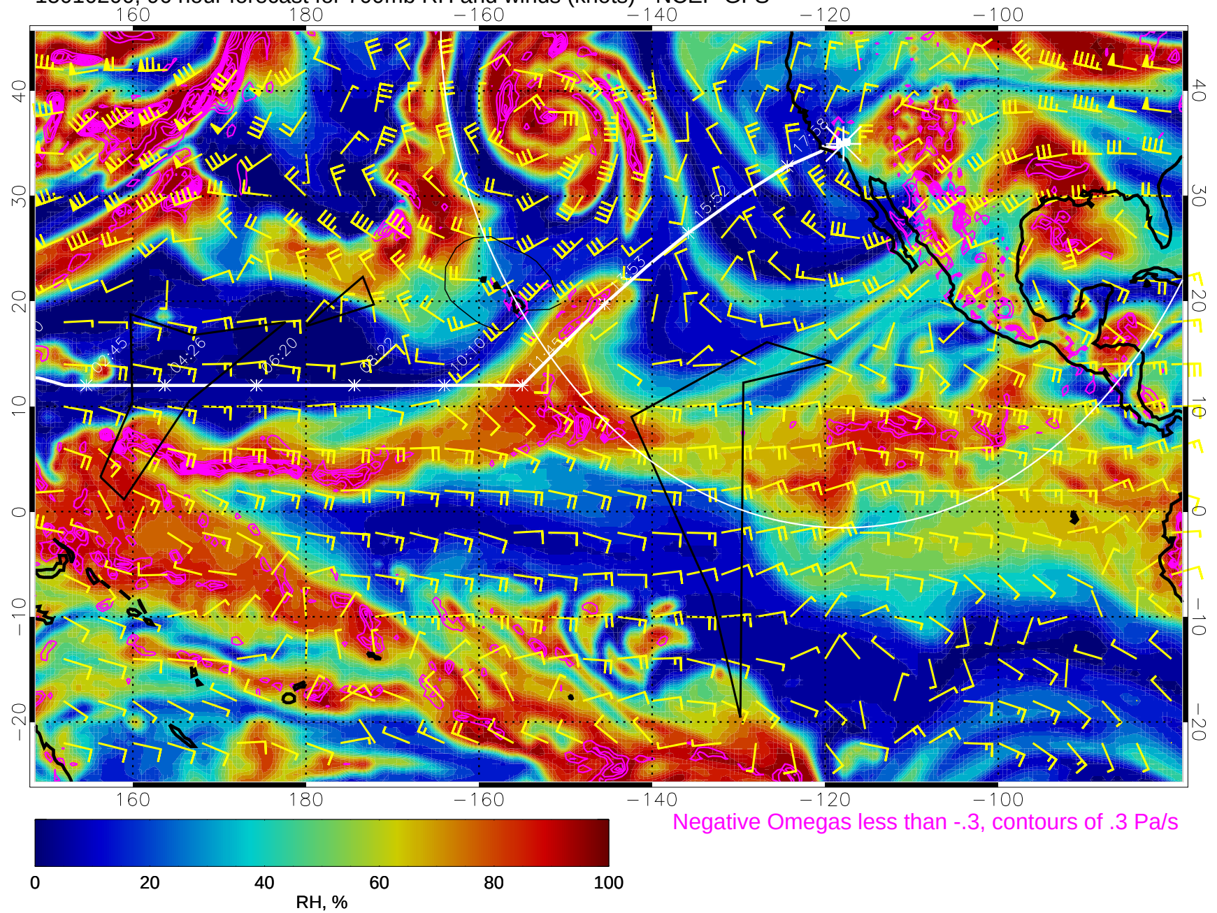
15010200, 96 hour forecast for 700mb RH and winds (knots) - NCEP GFS
