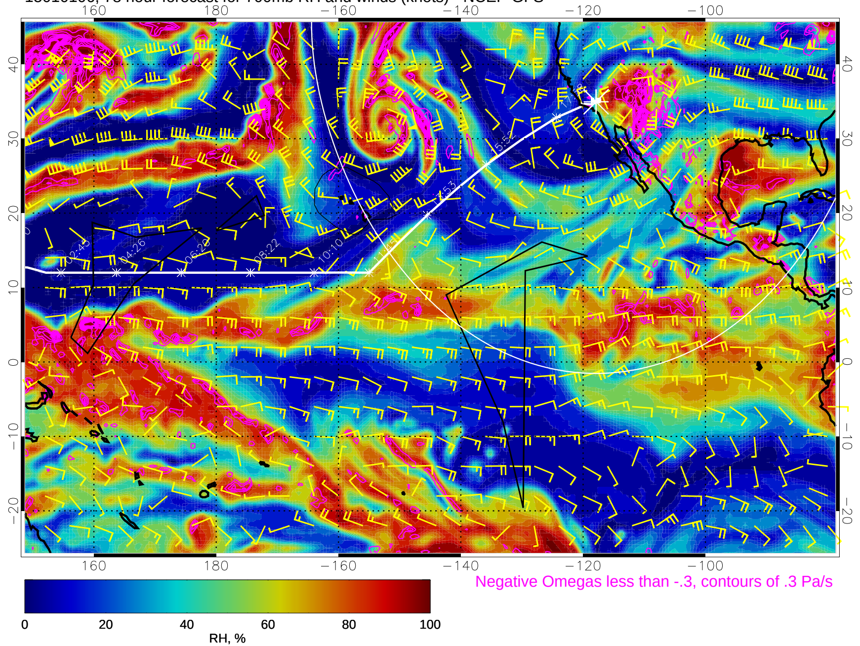
15010106, 78 hour forecast for 700mb RH and winds (knots) - NCEP GFS
