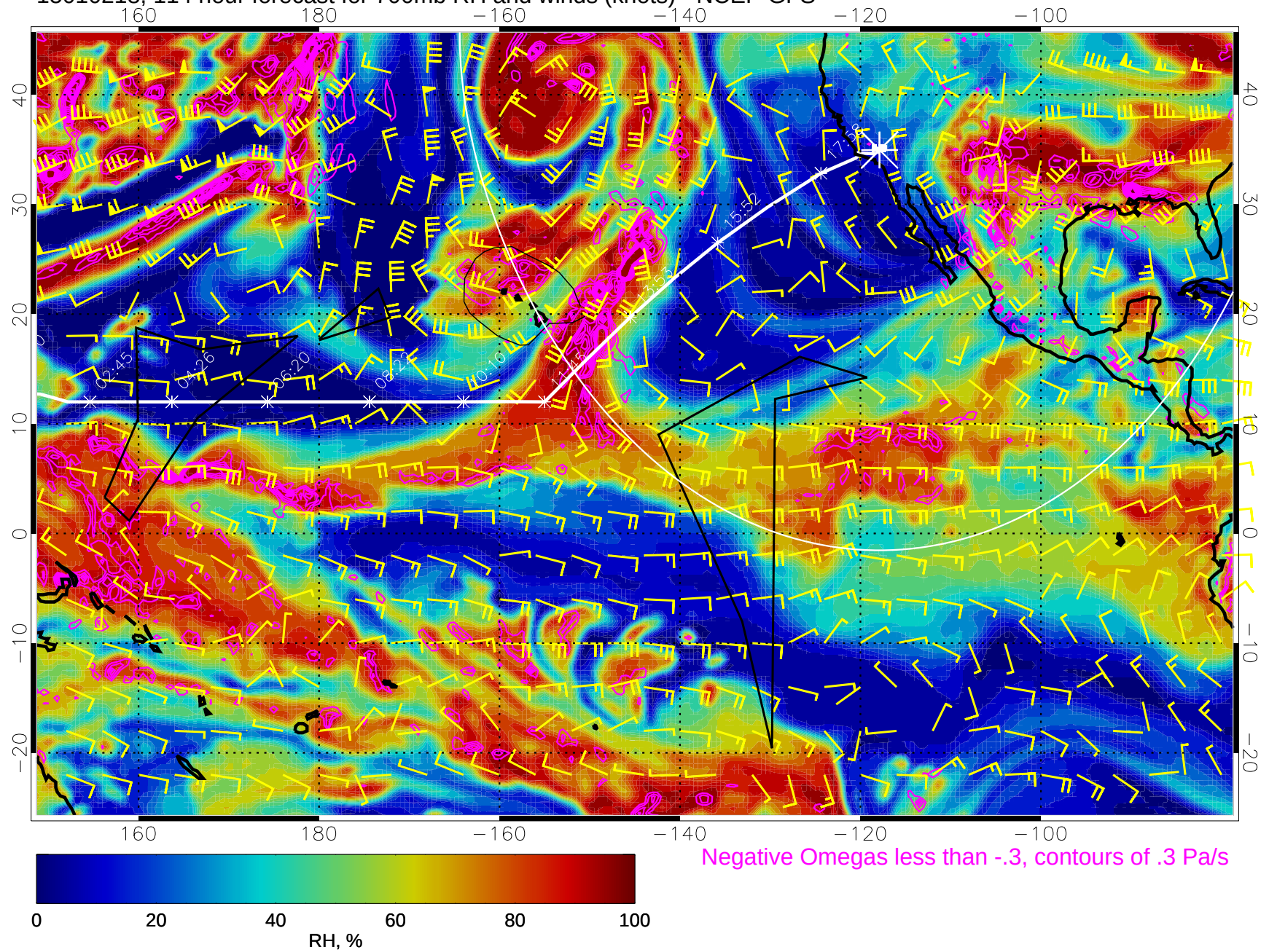
15010218, 114 hour forecast for 700mb RH and winds (knots) - NCEP GFS
