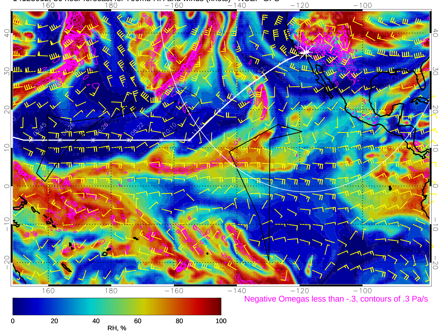
14123012, 36 hour forecast for 700mb RH and winds (knots) - NCEP GFS
