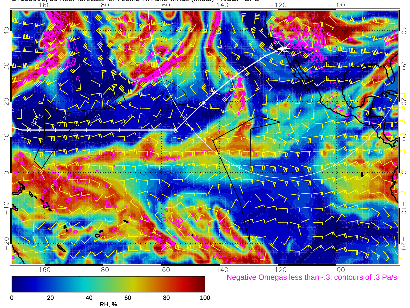
14123006, 30 hour forecast for 700mb RH and winds (knots) - NCEP GFS
