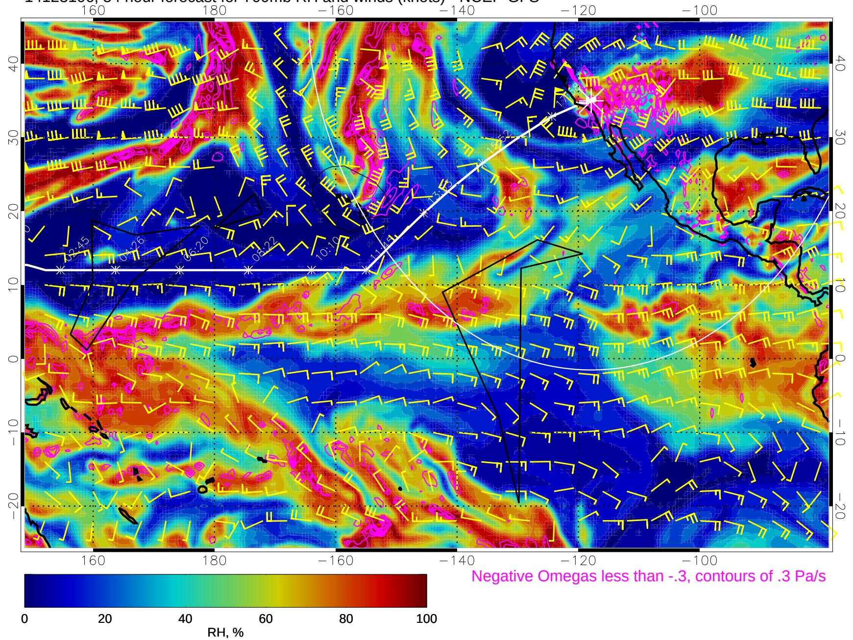
14123106, 54 hour forecast for 700mb RH and winds (knots) - NCEP GFS
