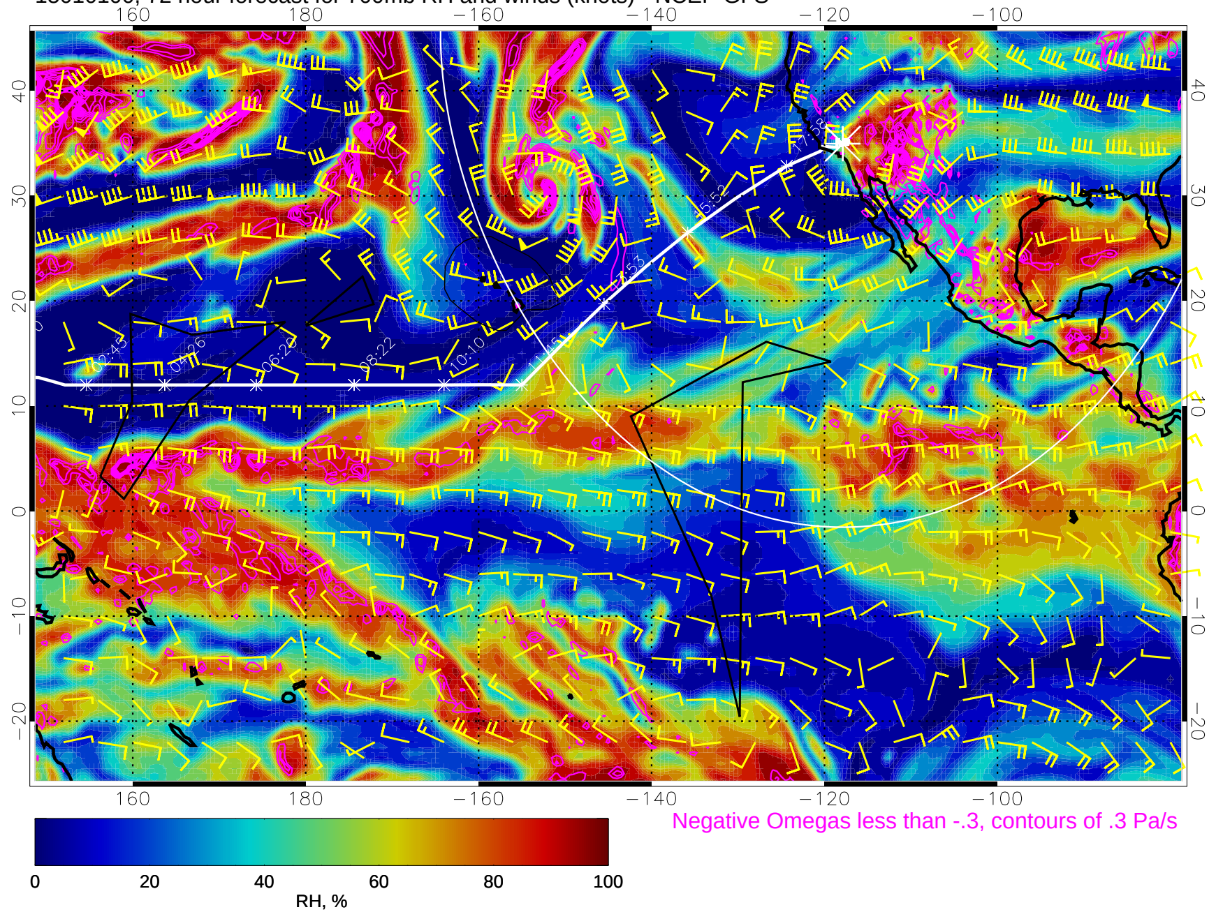
15010100, 72 hour forecast for 700mb RH and winds (knots) - NCEP GFS
