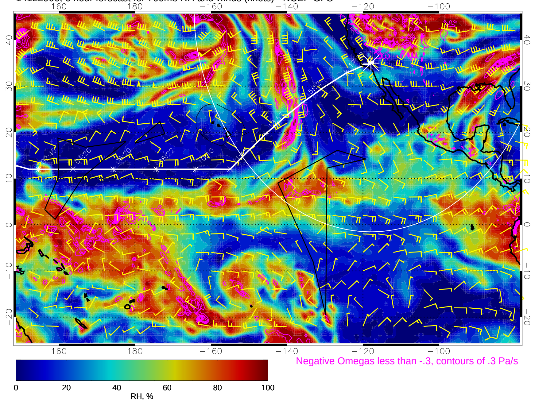
14122906, 6 hour forecast for 700mb RH and winds (knots) - NCEP GFS
