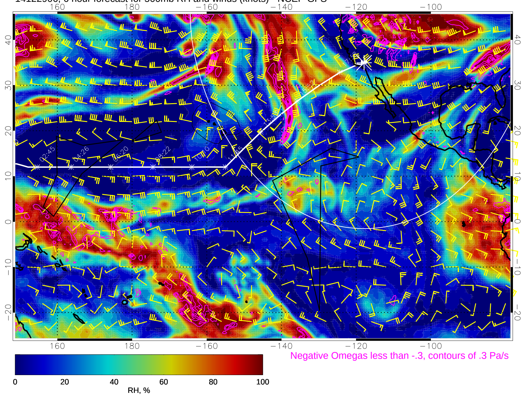
14122906, 6 hour forecast for 500mb RH and winds (knots) - NCEP GFS
