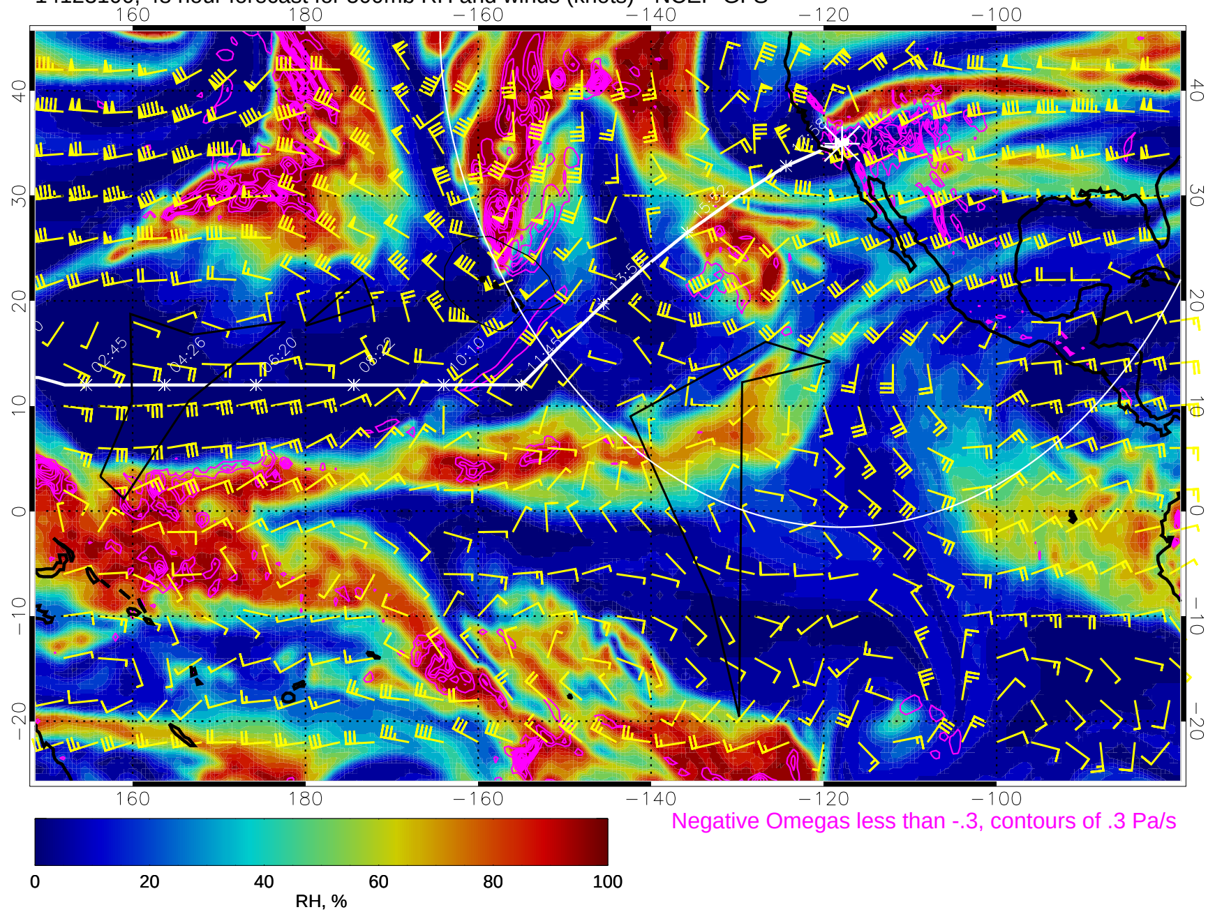
14123100, 48 hour forecast for 500mb RH and winds (knots) - NCEP GFS
