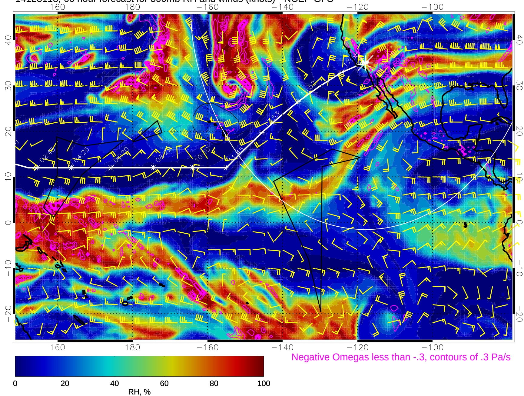
14123118, 66 hour forecast for 500mb RH and winds (knots) - NCEP GFS
