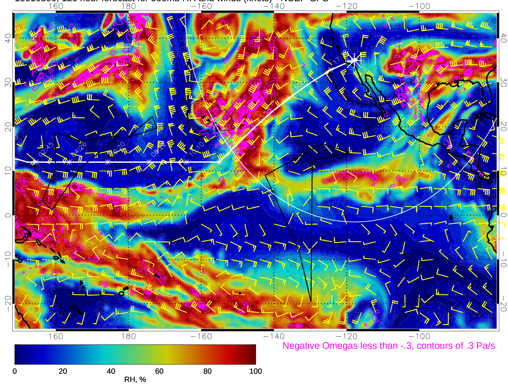
15010300, 120 hour forecast for 500mb RH and winds (knots) - NCEP GFS
