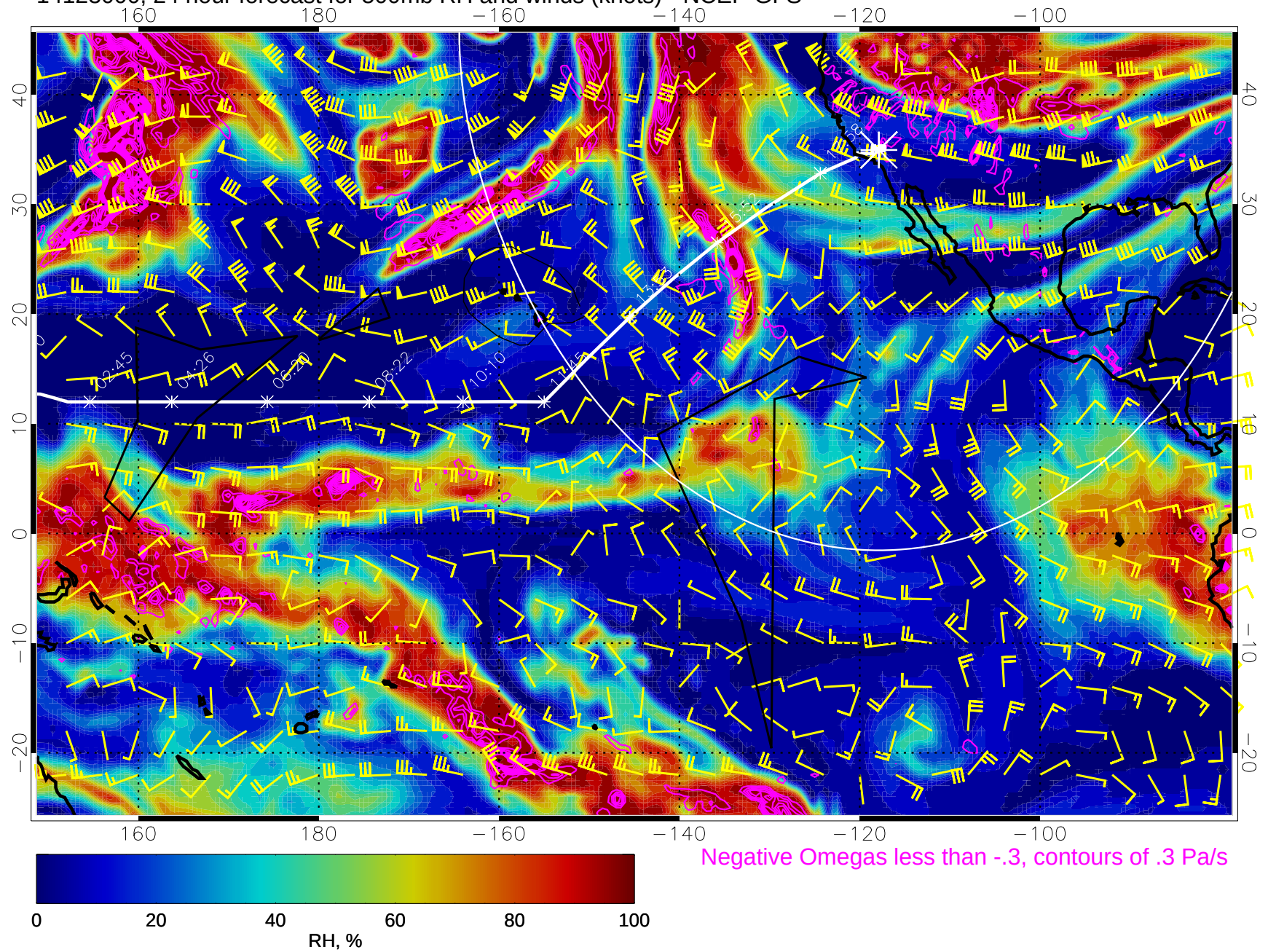
14123000, 24 hour forecast for 500mb RH and winds (knots) - NCEP GFS
