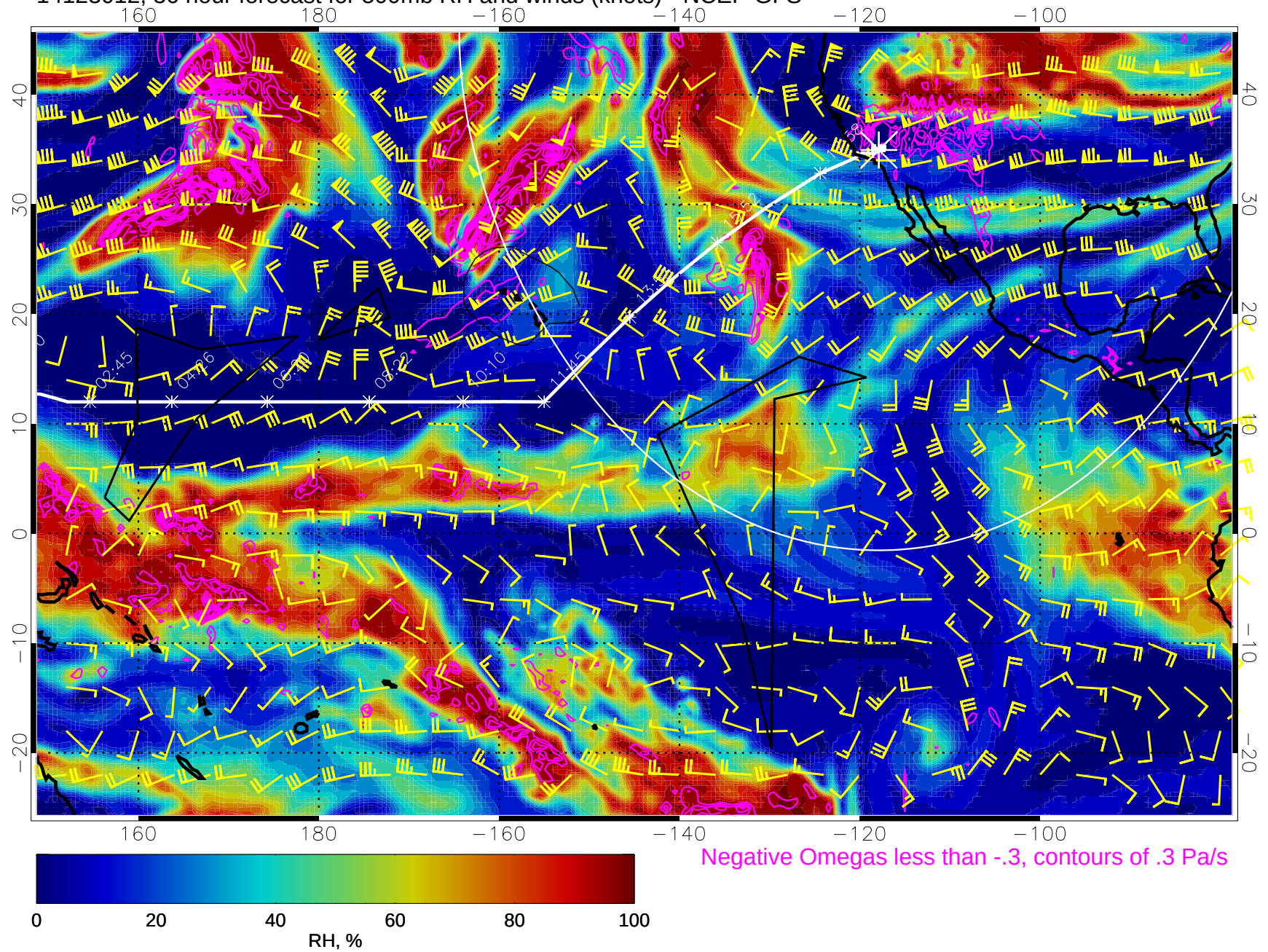
14123012, 36 hour forecast for 500mb RH and winds (knots) - NCEP GFS
