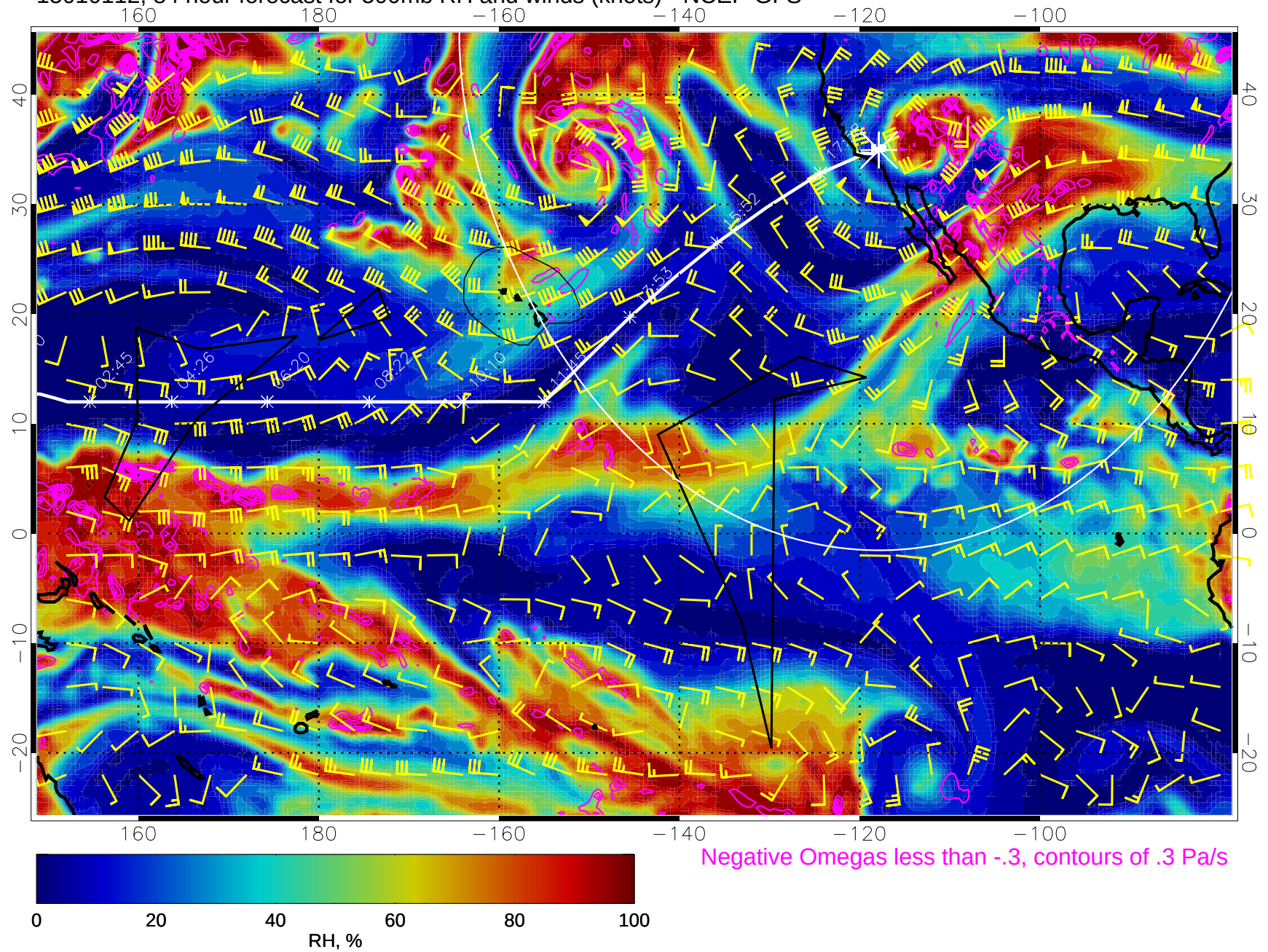
15010112, 84 hour forecast for 500mb RH and winds (knots) - NCEP GFS
