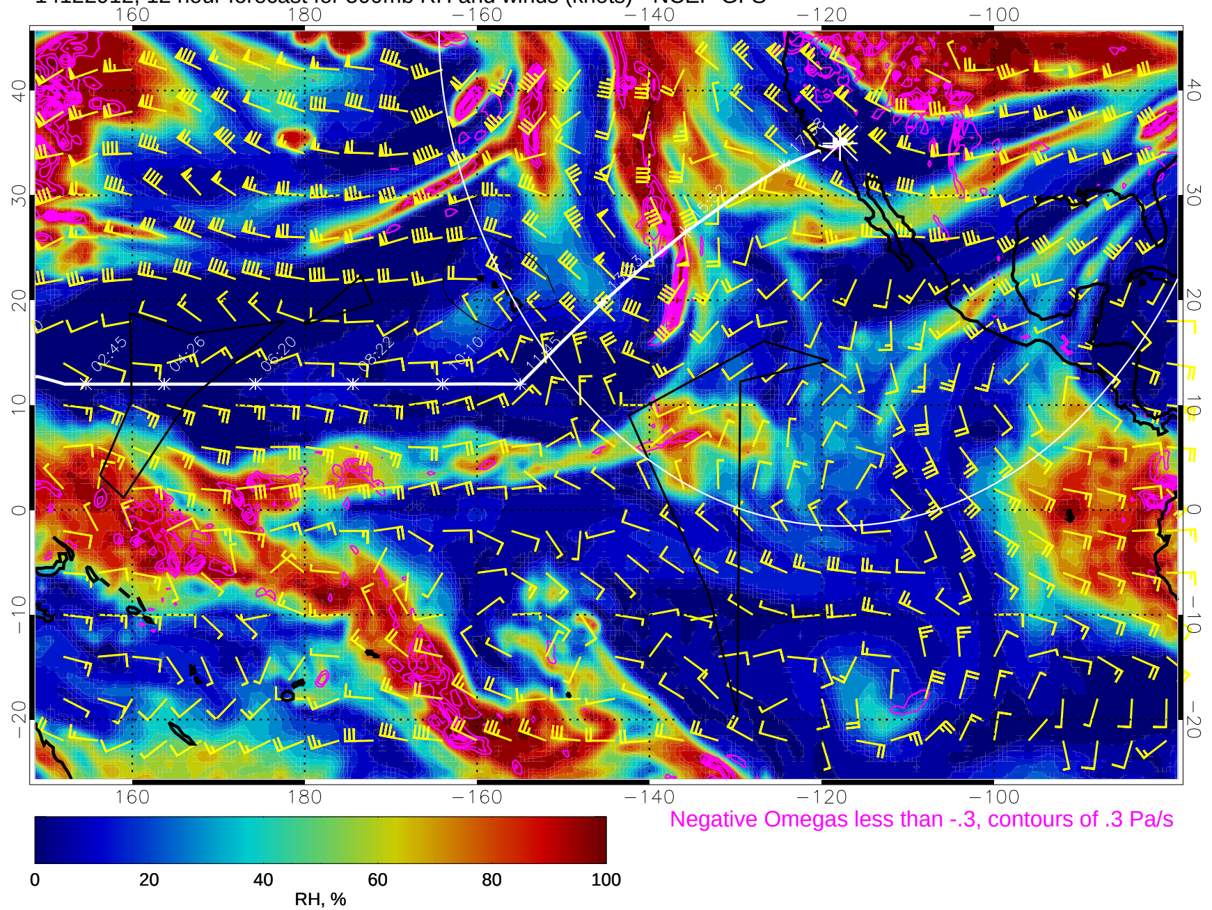
14122912, 12 hour forecast for 500mb RH and winds (knots) - NCEP GFS
