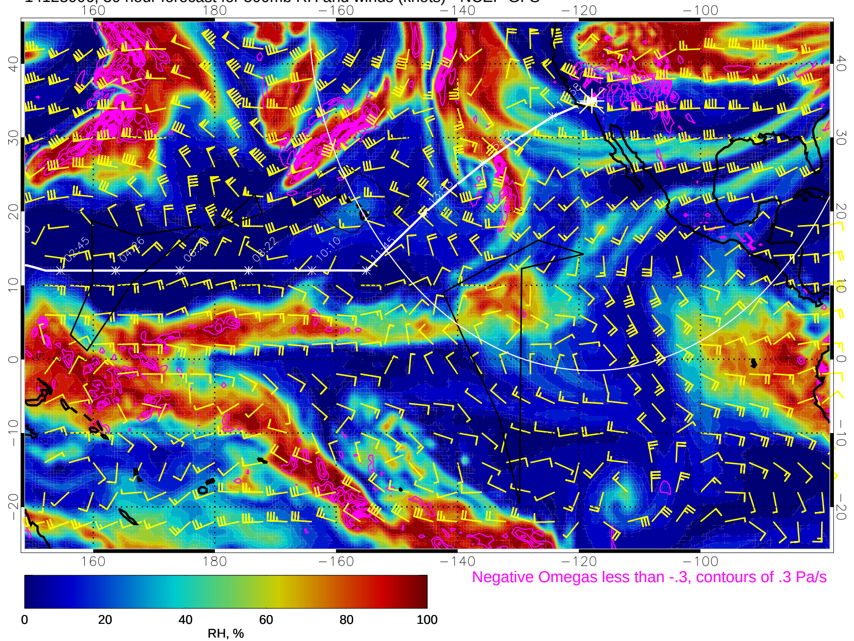
14123006, 30 hour forecast for 500mb RH and winds (knots) - NCEP GFS
