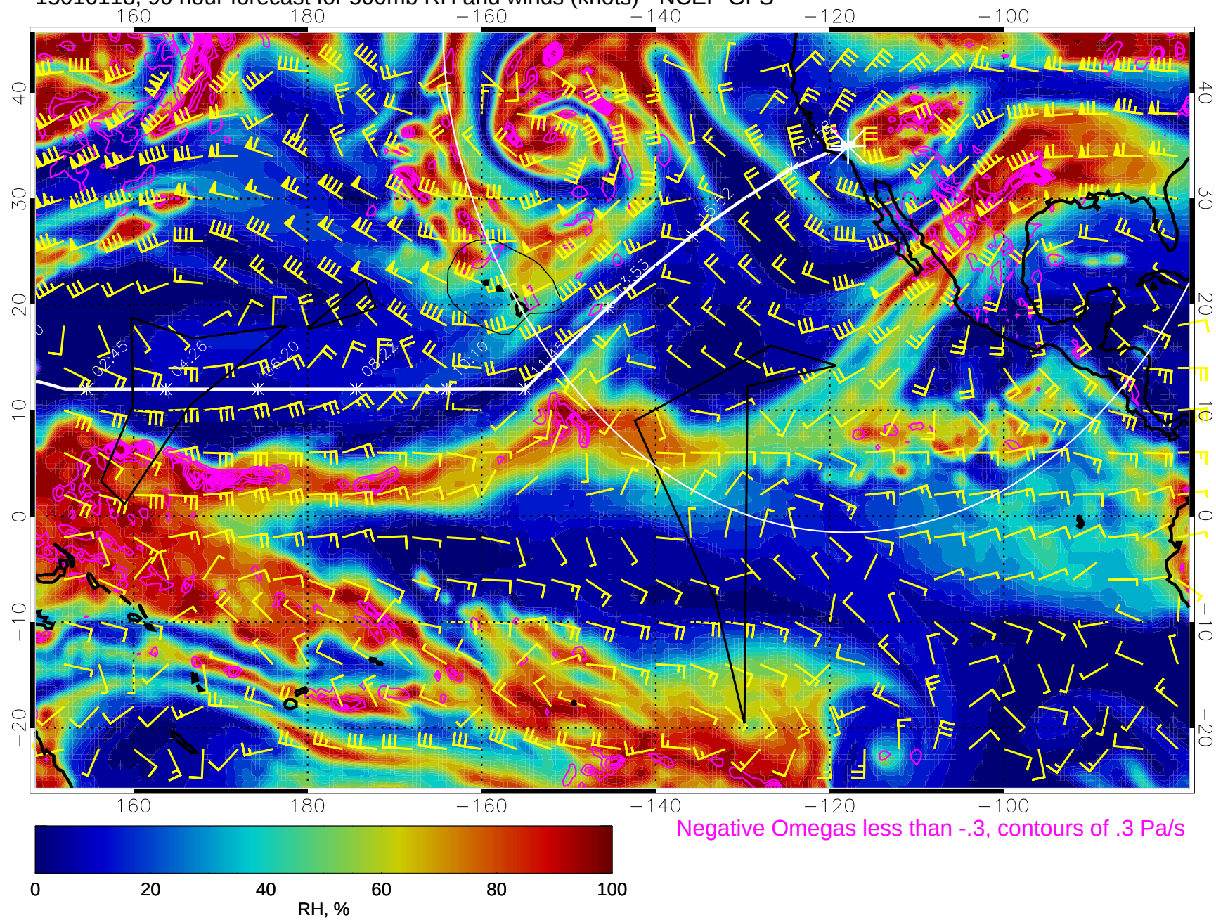
15010118, 90 hour forecast for 500mb RH and winds (knots) - NCEP GFS
