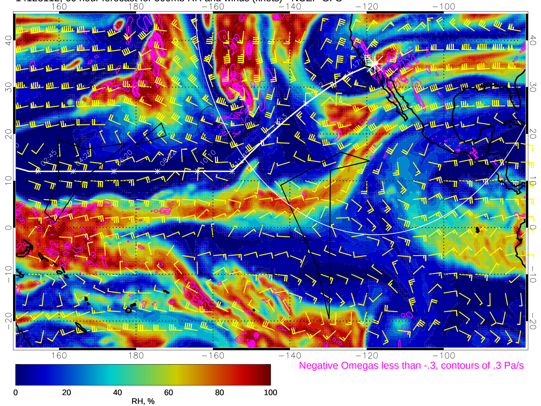
14123112, 60 hour forecast for 500mb RH and winds (knots) - NCEP GFS
