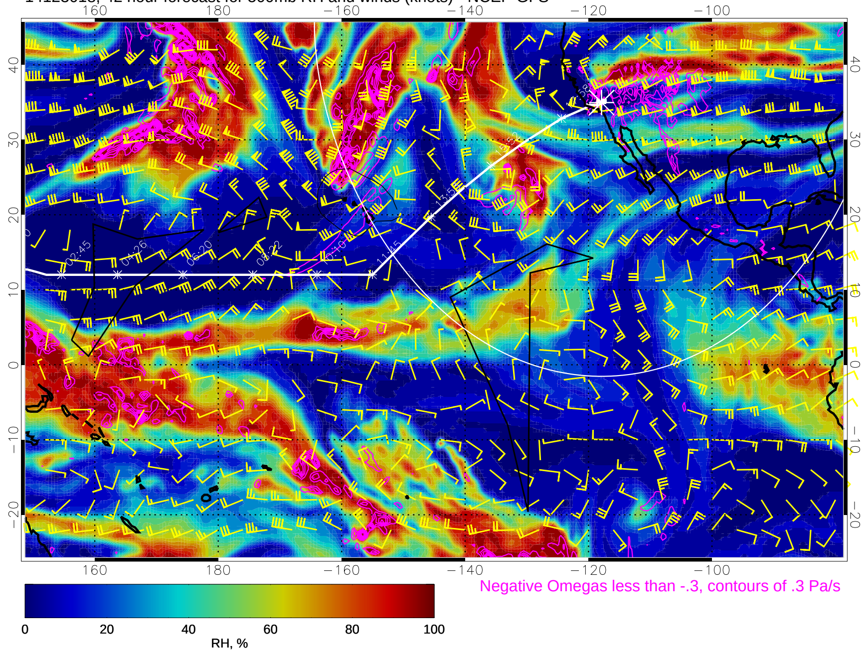
14123018, 42 hour forecast for 500mb RH and winds (knots) - NCEP GFS
