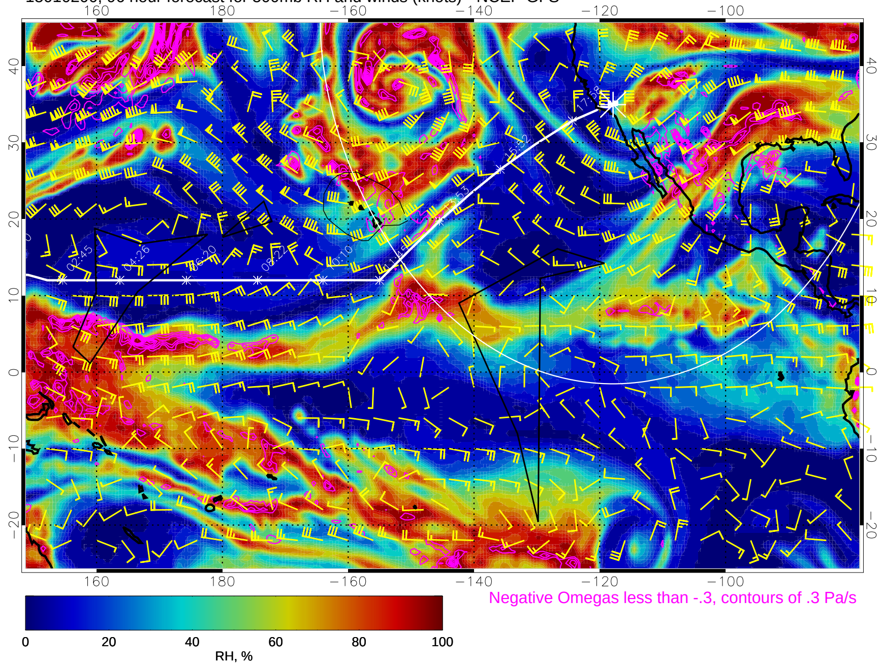
15010200, 96 hour forecast for 500mb RH and winds (knots) - NCEP GFS
