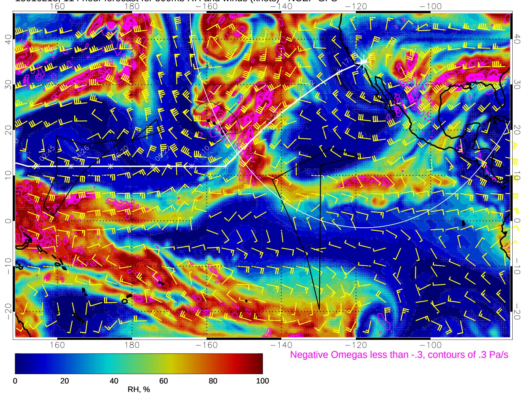
15010218, 114 hour forecast for 500mb RH and winds (knots) - NCEP GFS
