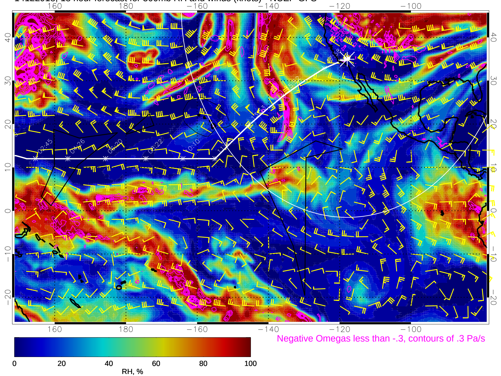
14122918, 18 hour forecast for 500mb RH and winds (knots) - NCEP GFS
