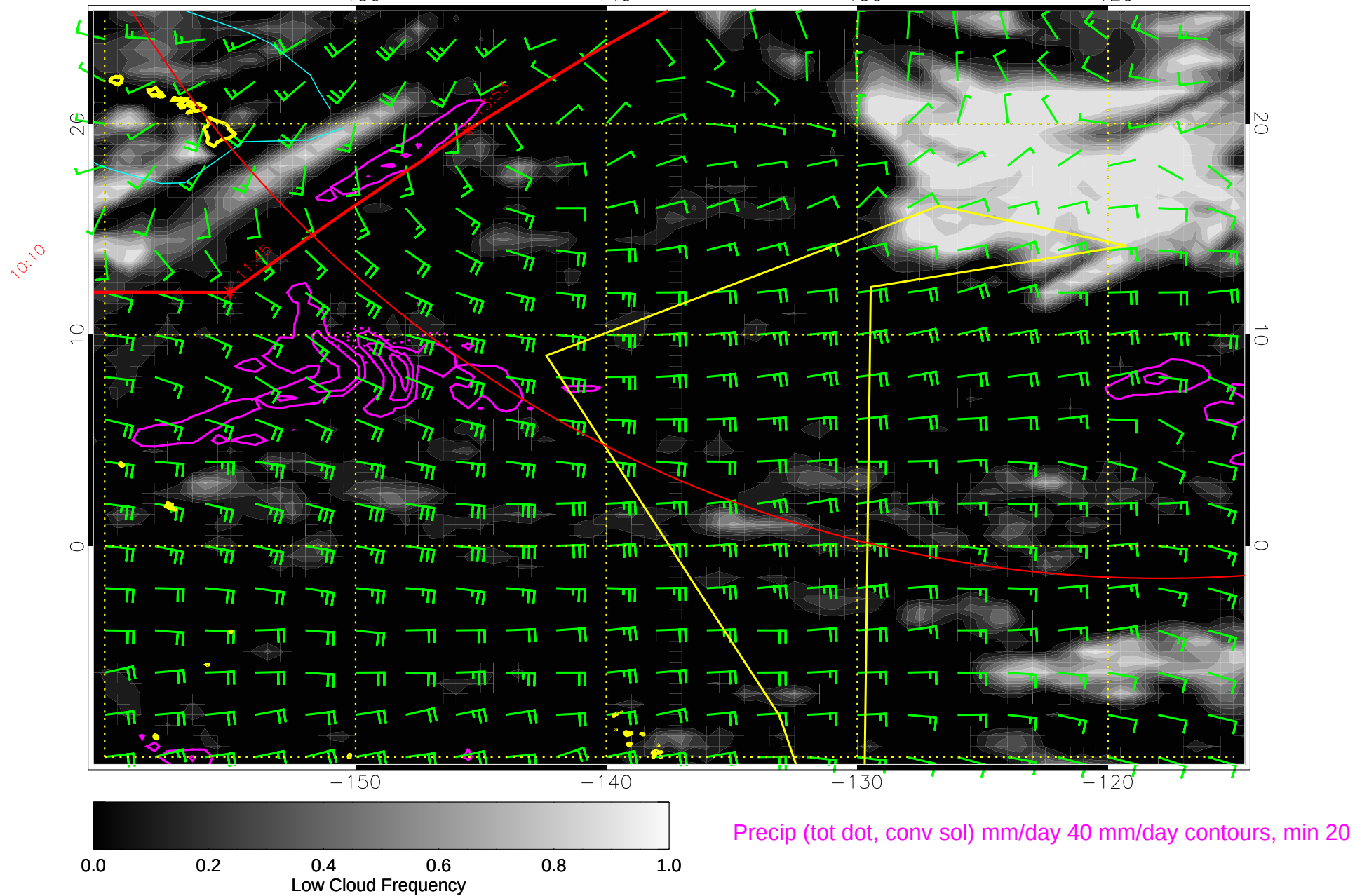
15010200, 96 hour forecast for 850mb winds (knots) and Low Cloud Frequency -- NCEP GFS
