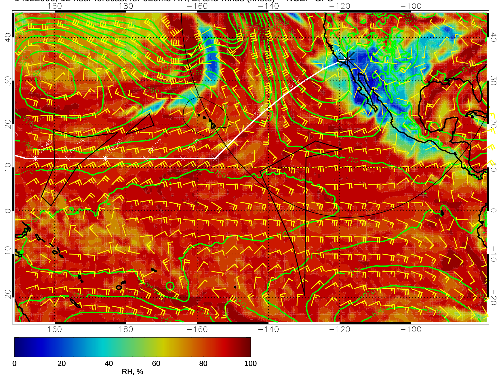
14122900, 12 hour forecast for 925mb RH, Z, and winds (knots) -- NCEP GFS
