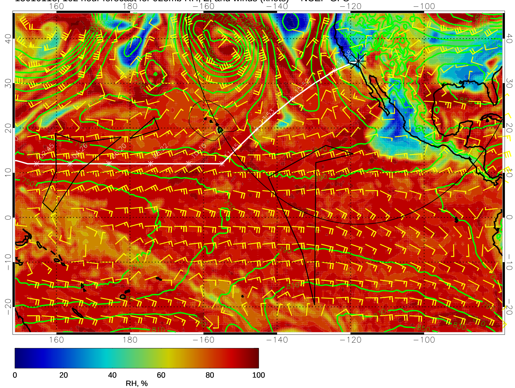
15010118, 102 hour forecast for 925mb RH, Z, and winds (knots) -- NCEP GFS
