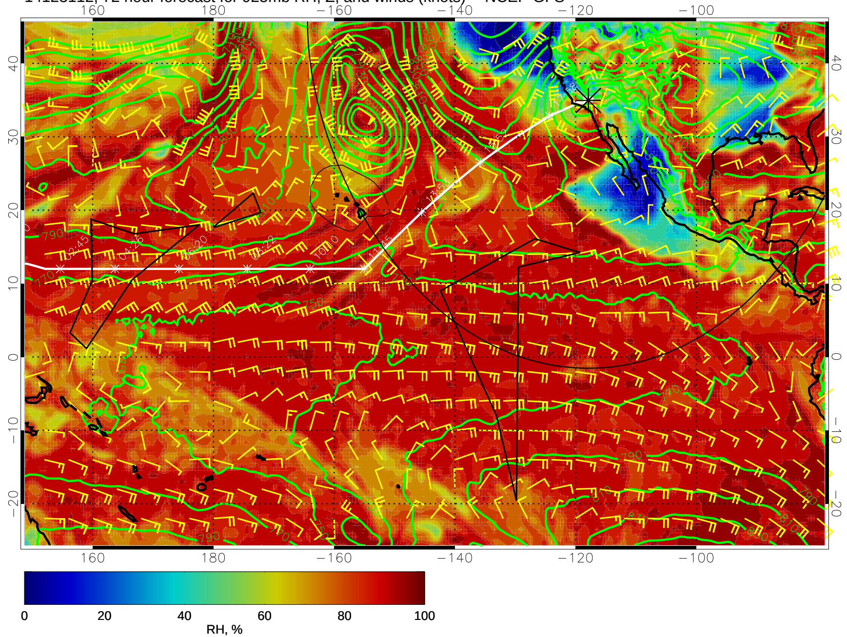
14123112, 72 hour forecast for 925mb RH, Z, and winds (knots) -- NCEP GFS
