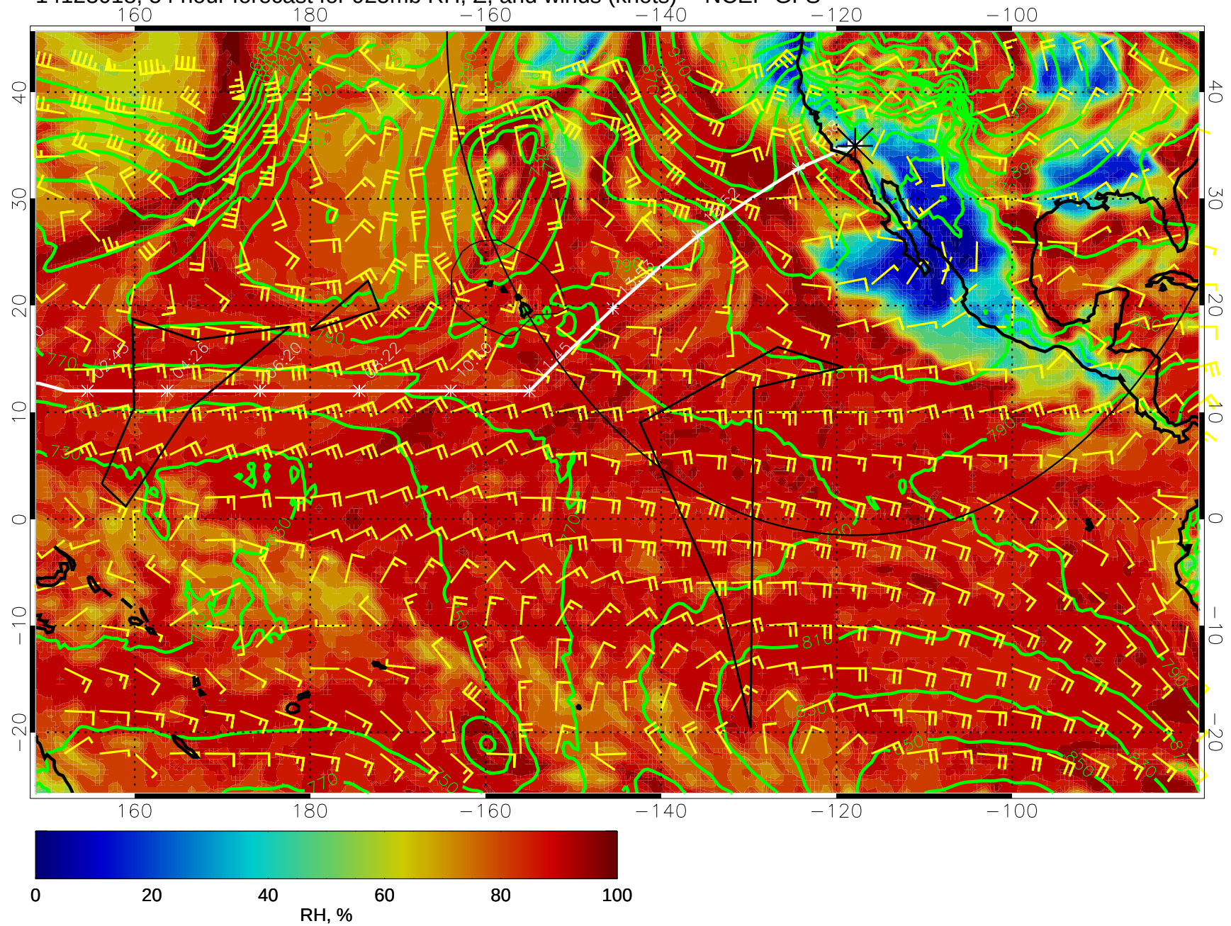
14123018, 54 hour forecast for 925mb RH, Z, and winds (knots) -- NCEP GFS
