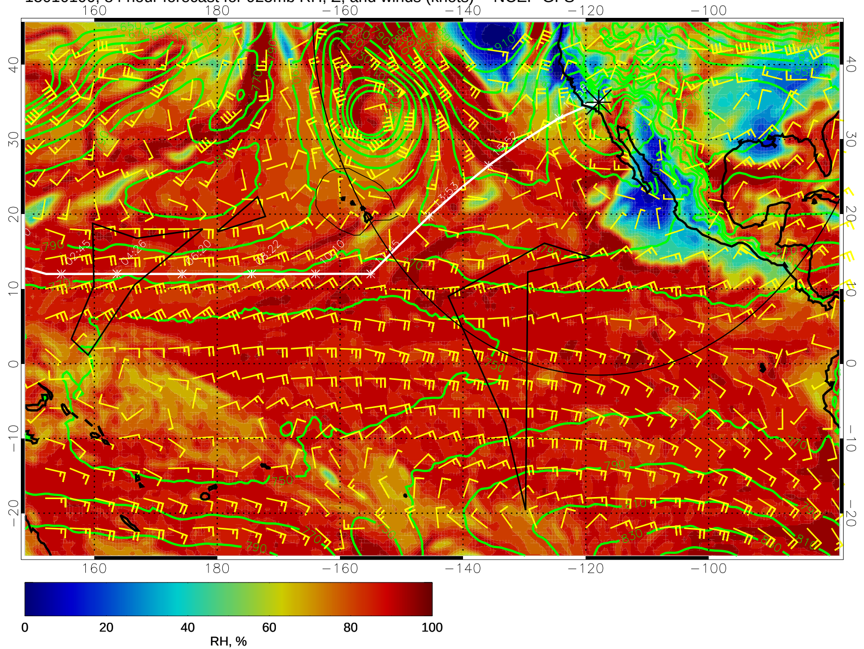
15010100, 84 hour forecast for 925mb RH, Z, and winds (knots) -- NCEP GFS
