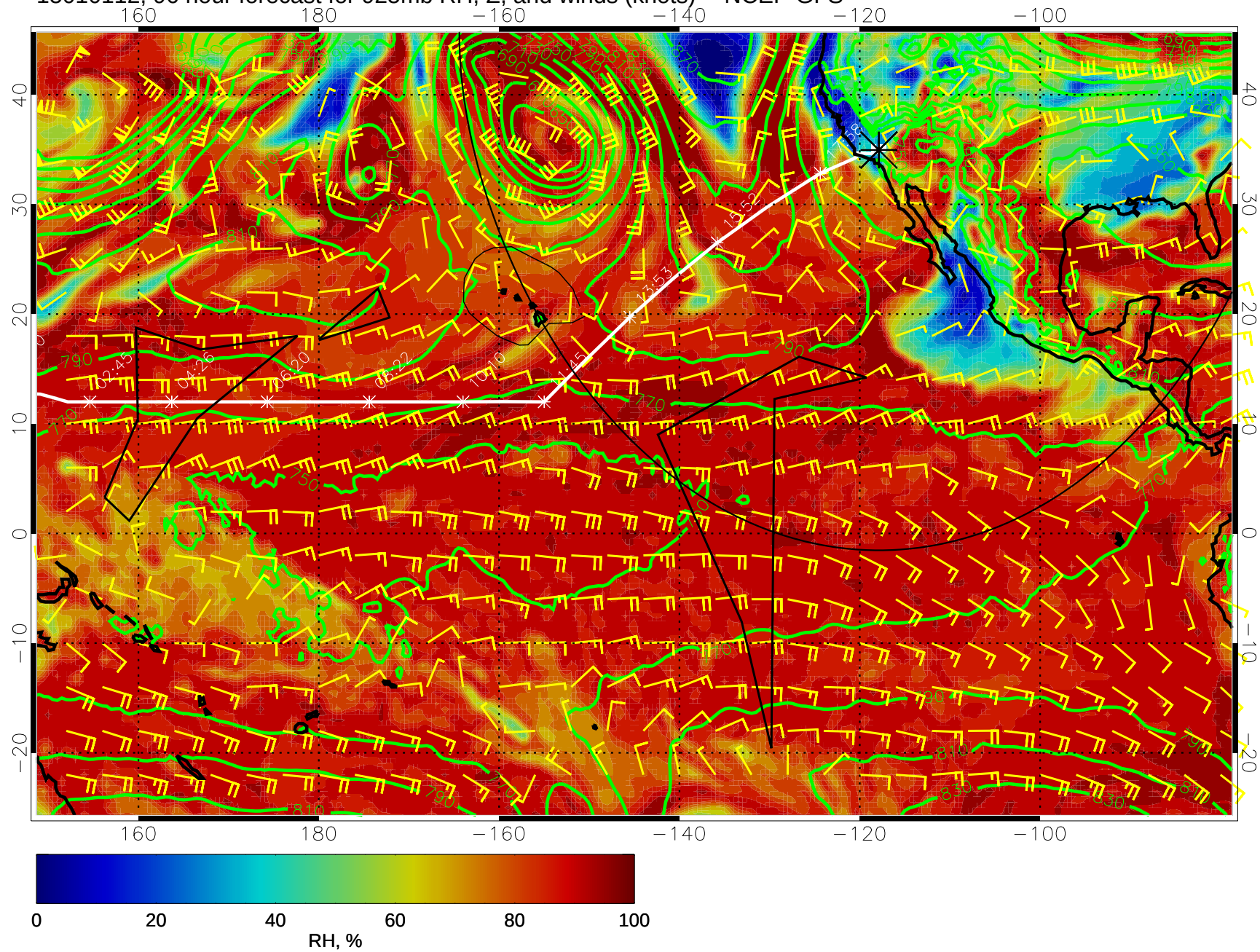
15010112, 96 hour forecast for 925mb RH, Z, and winds (knots) -- NCEP GFS
