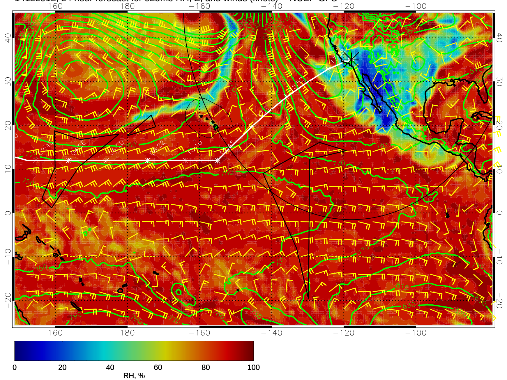
14122912, 24 hour forecast for 925mb RH, Z, and winds (knots) -- NCEP GFS
