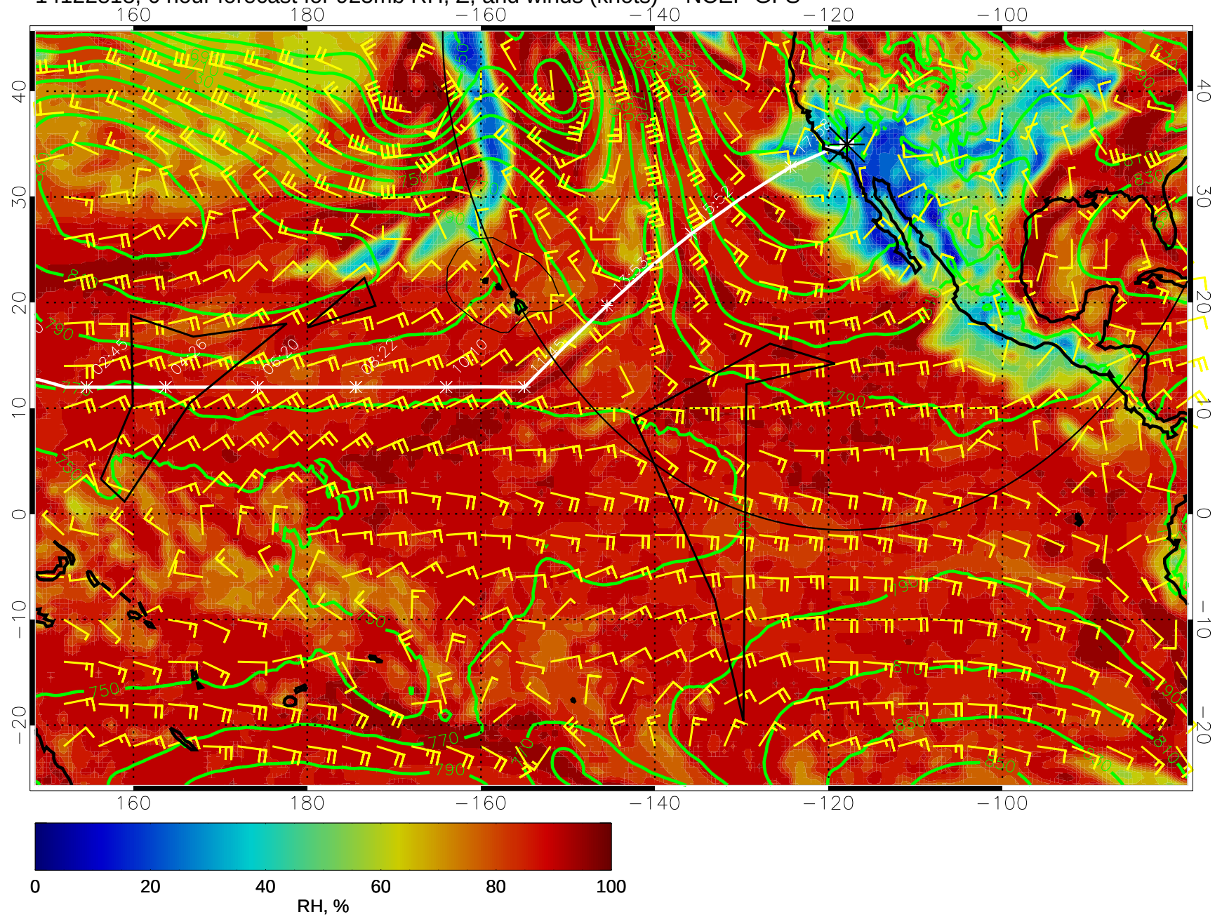
14122818, 6 hour forecast for 925mb RH, Z, and winds (knots) -- NCEP GFS
