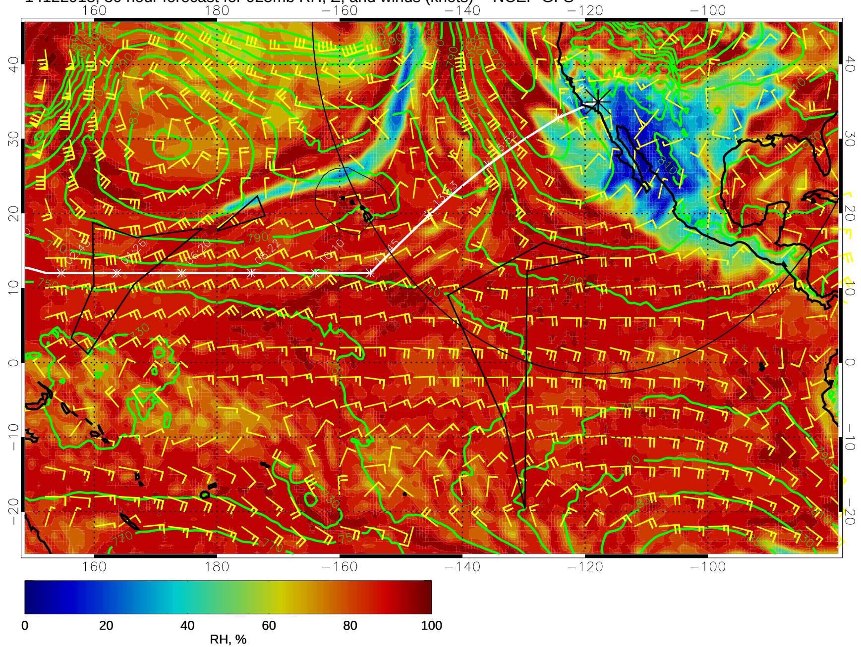
14122918, 30 hour forecast for 925mb RH, Z, and winds (knots) -- NCEP GFS
