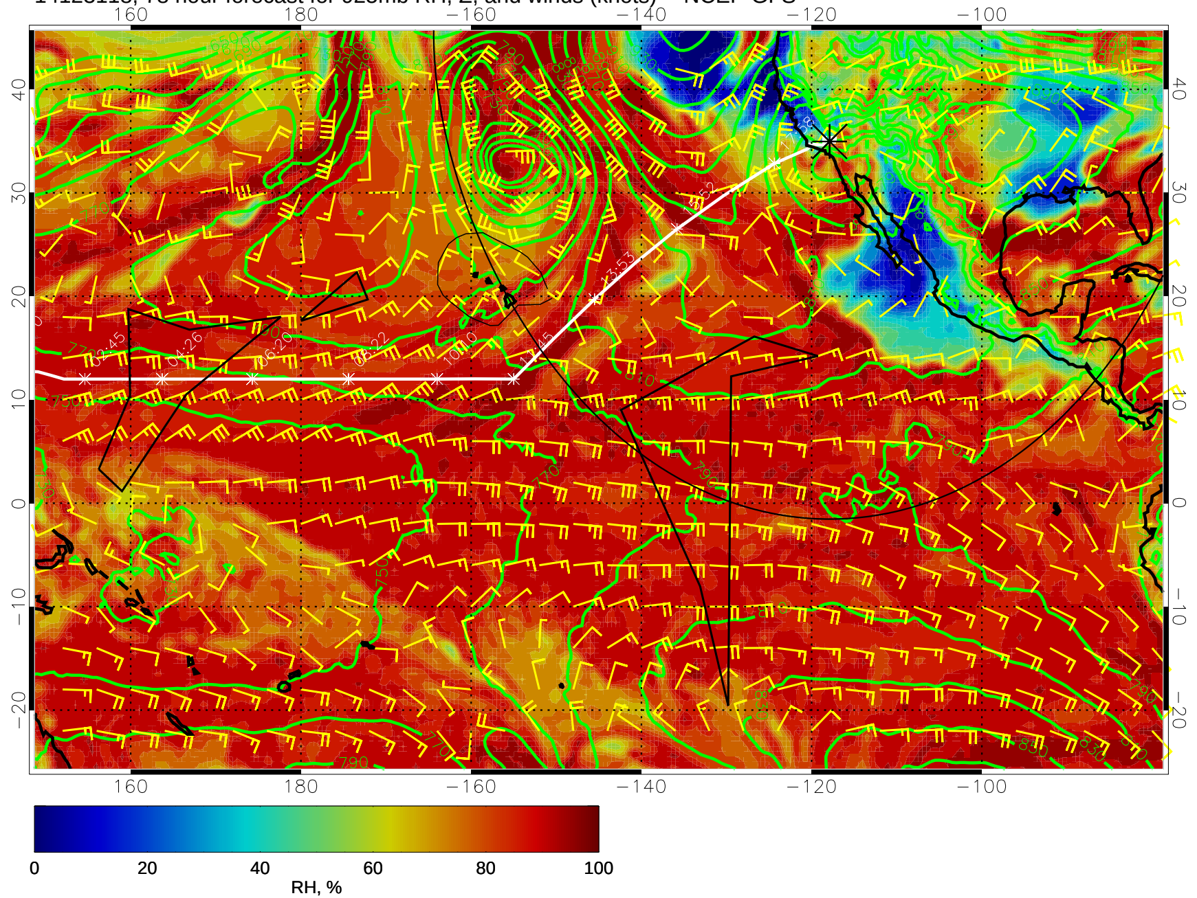
14123118, 78 hour forecast for 925mb RH, Z, and winds (knots) -- NCEP GFS
