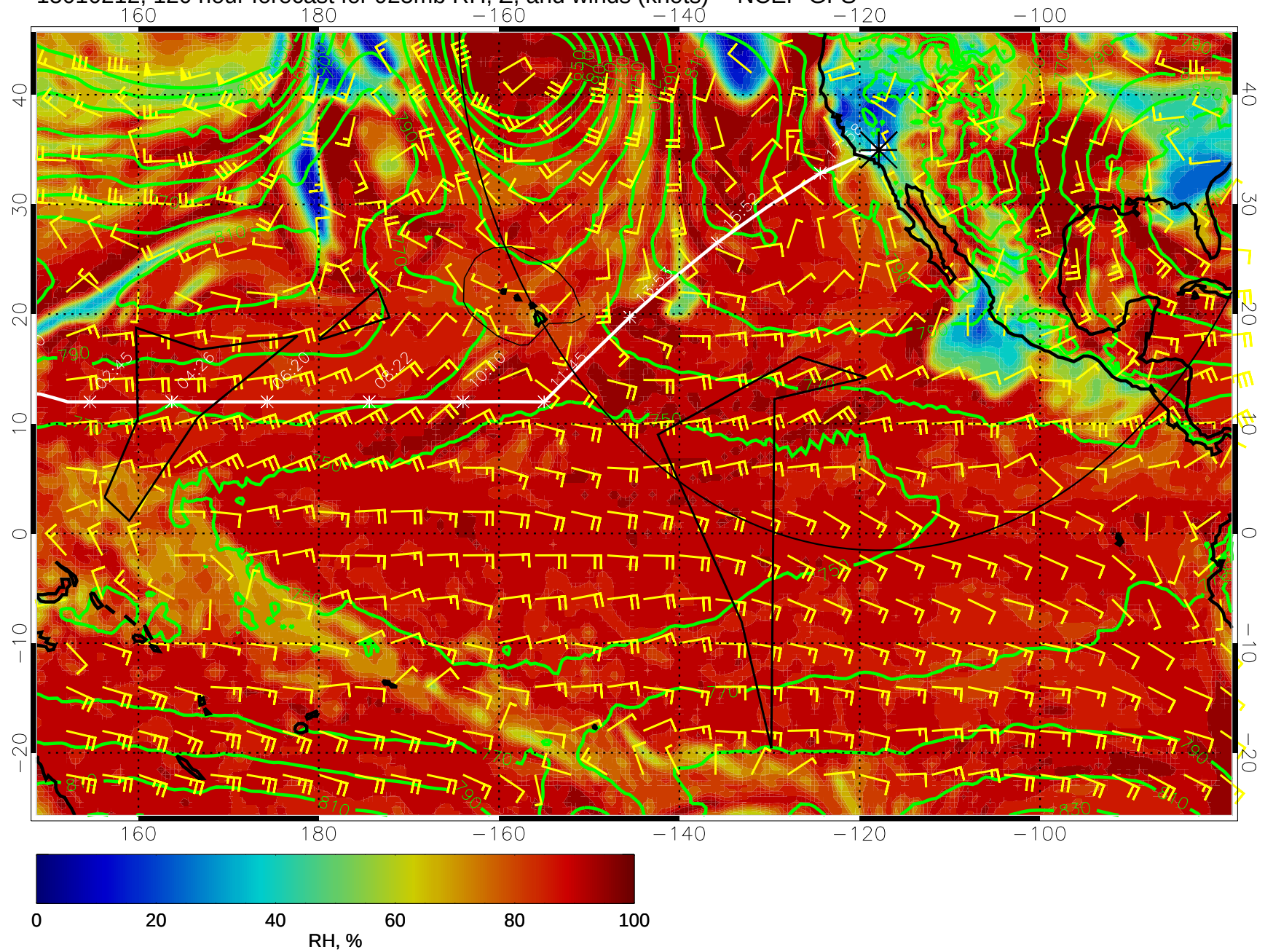
15010212, 120 hour forecast for 925mb RH, Z, and winds (knots) -- NCEP GFS
