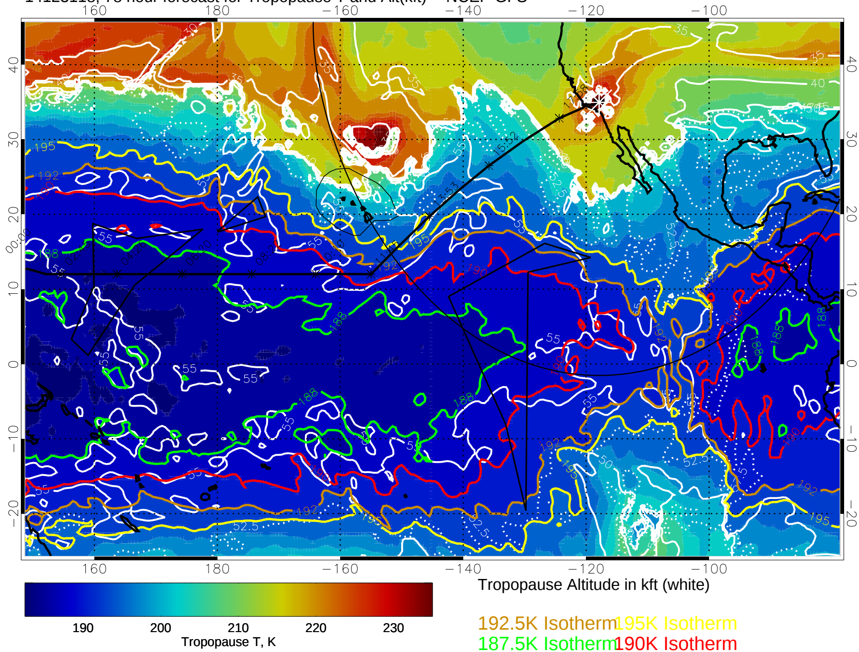
14123118, 78 hour forecast for Tropopause T and Alt(kft) -- NCEP GFS
