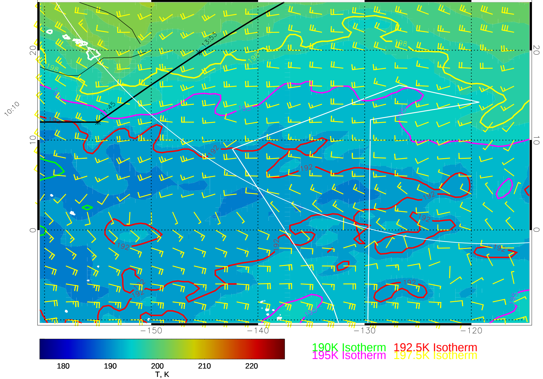
15010200, 108 hour forecast for 70mb T and winds (knots) -- NCEP GFS
