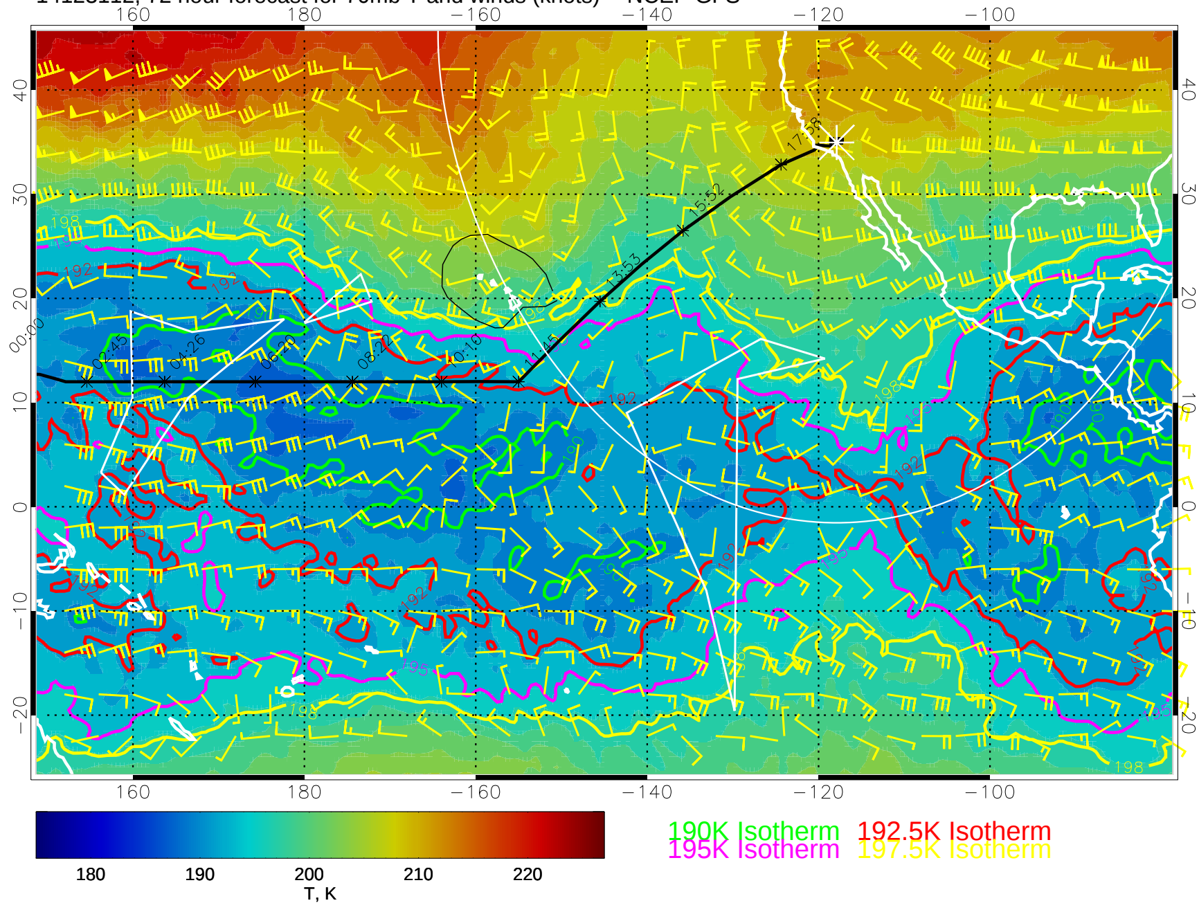
14123112, 72 hour forecast for 70mb T and winds (knots) -- NCEP GFS
