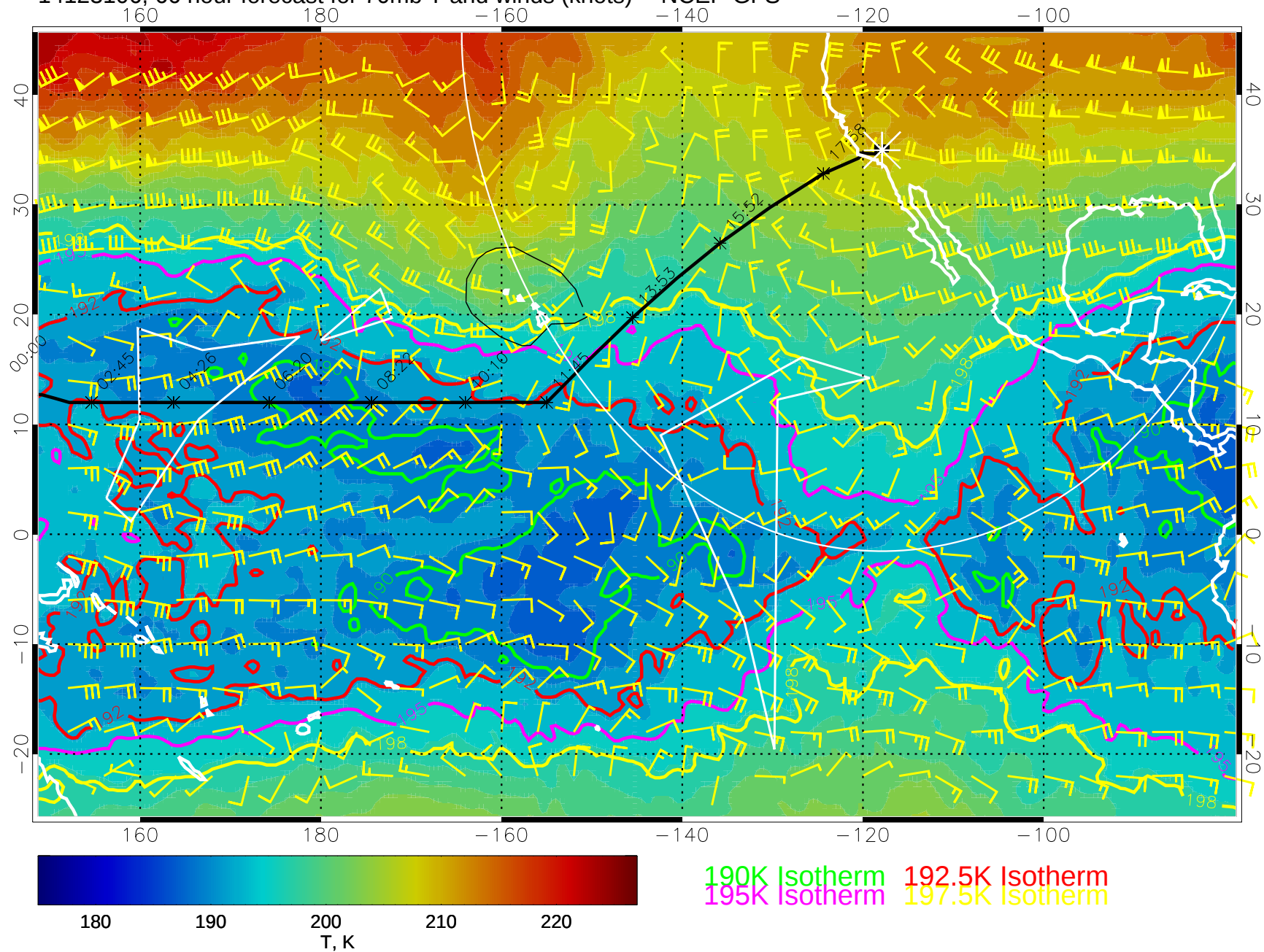
14123106, 66 hour forecast for 70mb T and winds (knots) -- NCEP GFS
