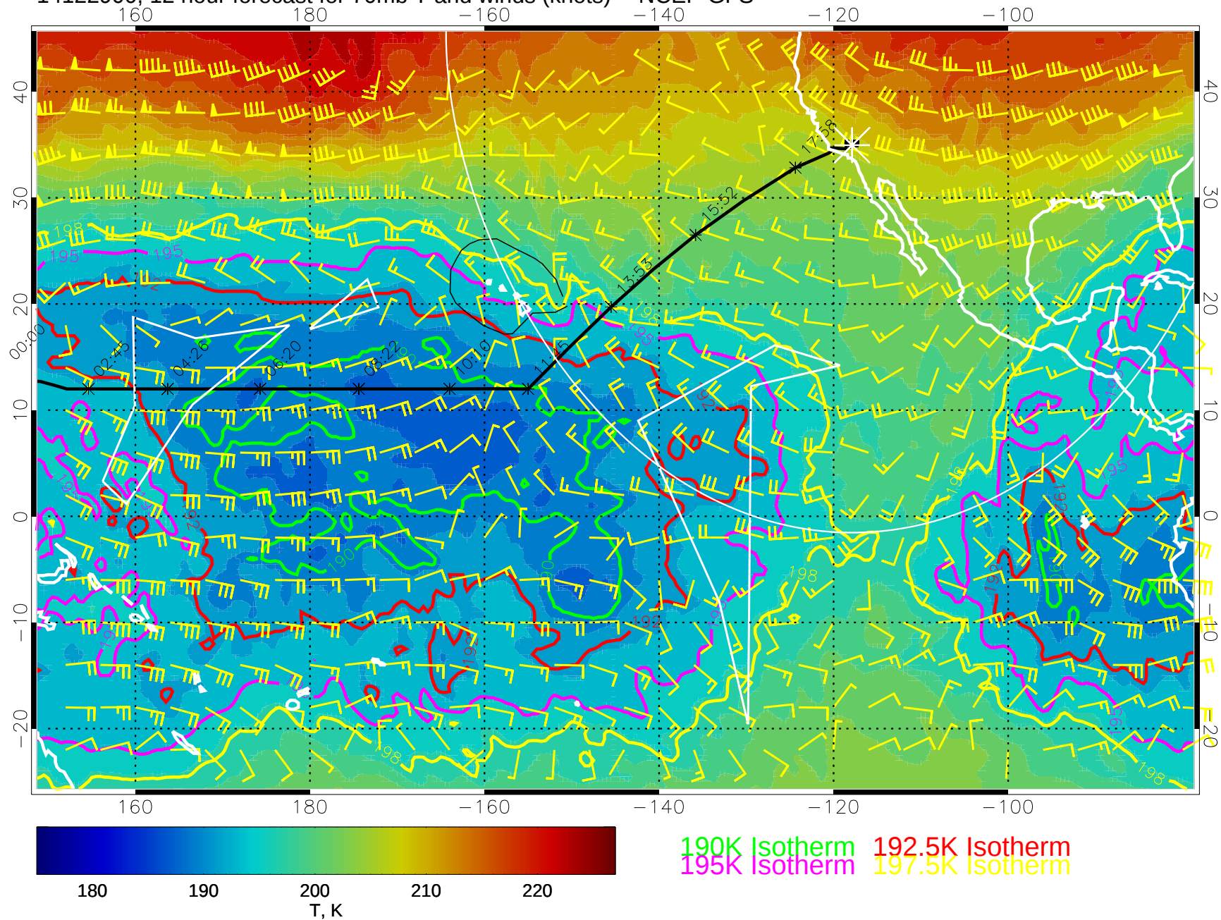
14122900, 12 hour forecast for 70mb T and winds (knots) -- NCEP GFS
