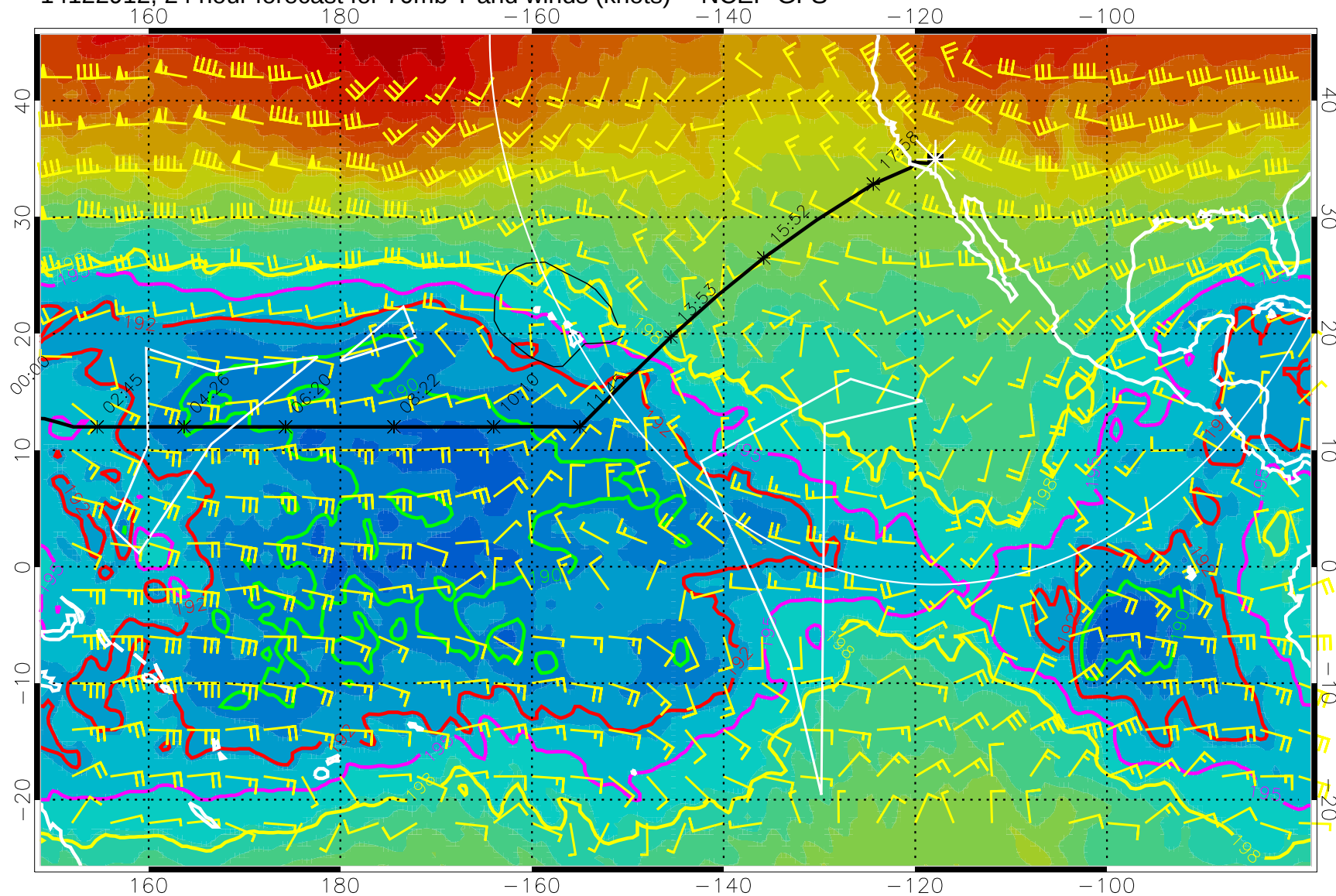
14122912, 24 hour forecast for 70mb T and winds (knots) -- NCEP GFS
