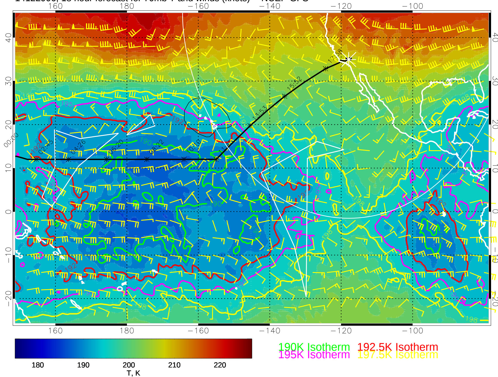
14122906, 18 hour forecast for 70mb T and winds (knots) -- NCEP GFS
