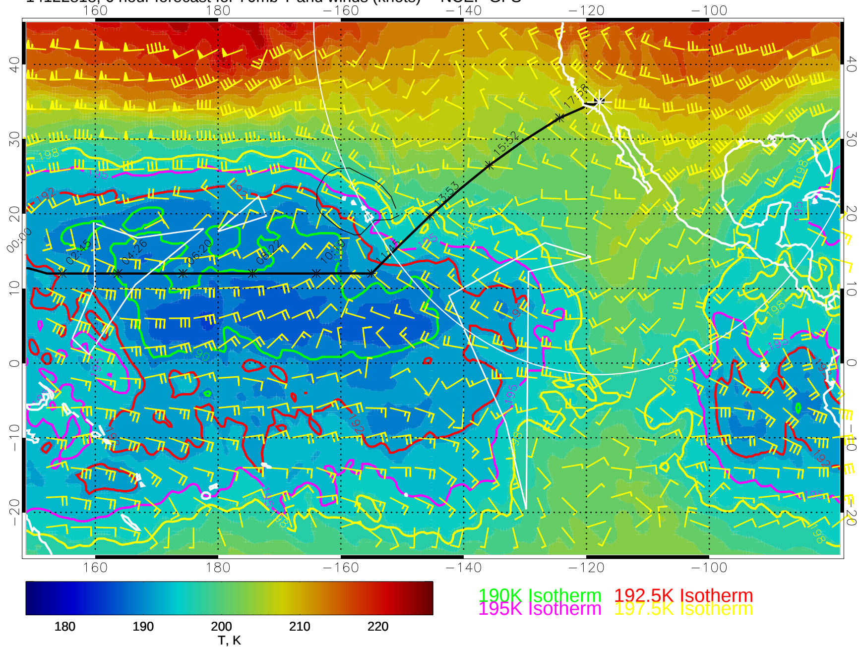
14122818, 6 hour forecast for 70mb T and winds (knots) -- NCEP GFS
