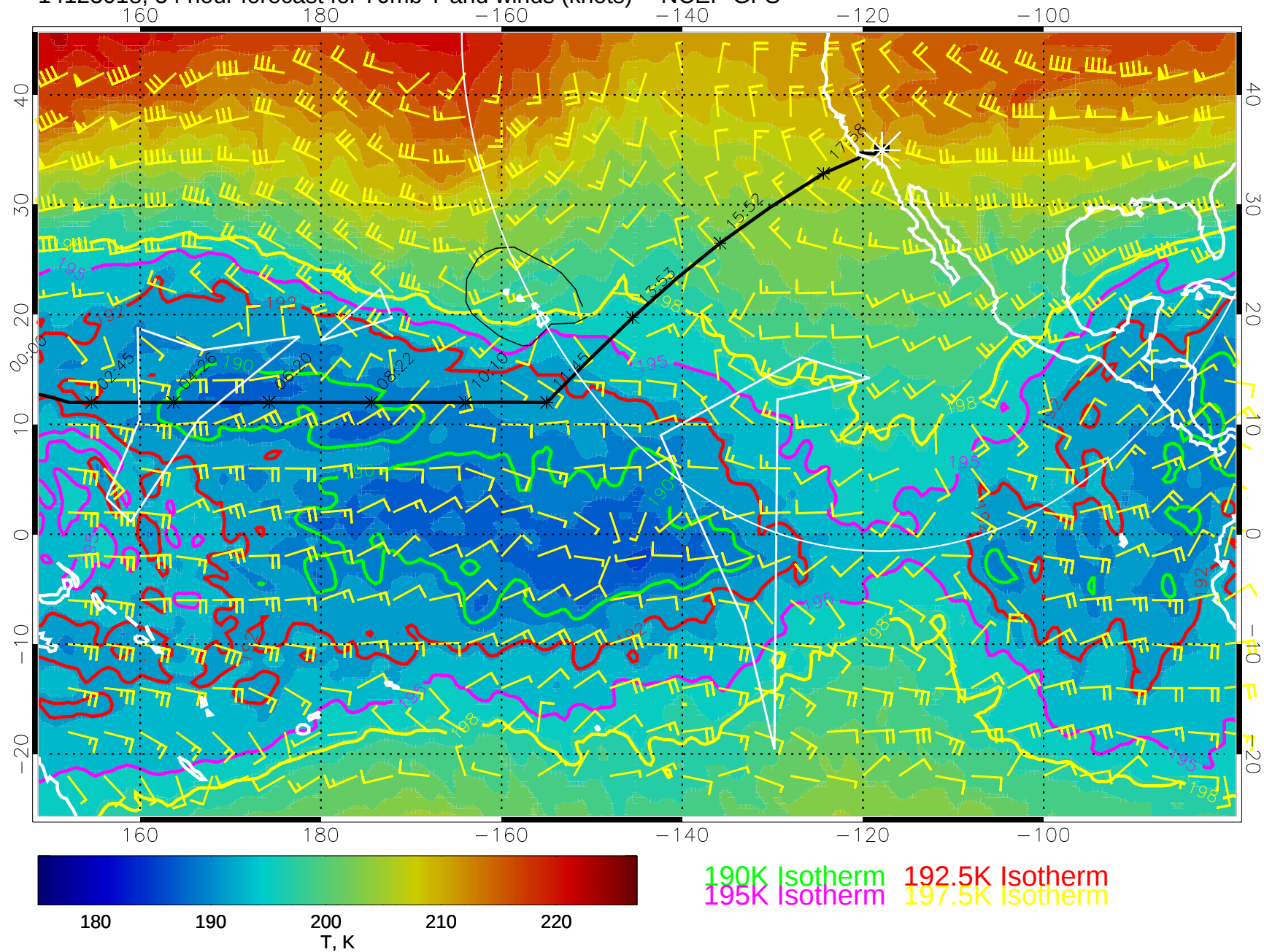
14123018, 54 hour forecast for 70mb T and winds (knots) -- NCEP GFS
