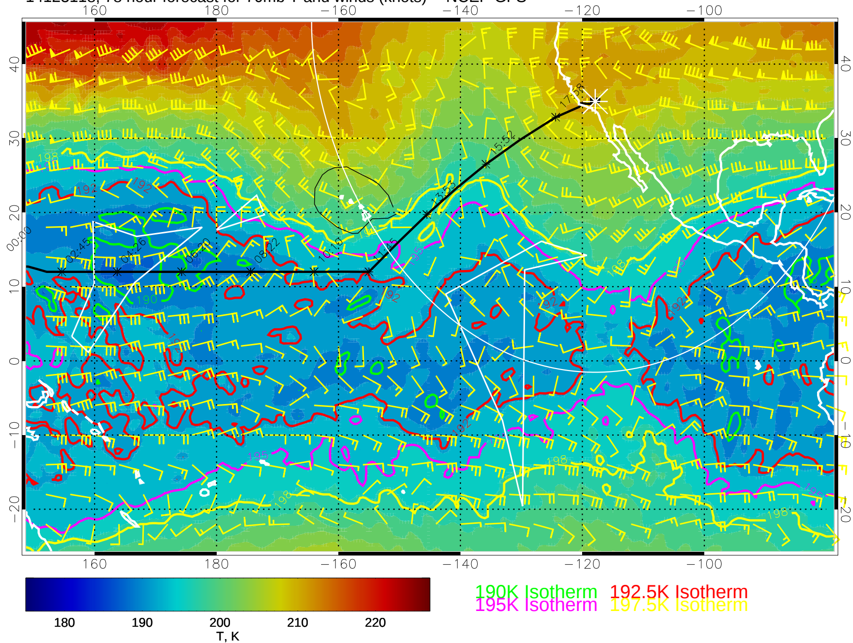
14123118, 78 hour forecast for 70mb T and winds (knots) -- NCEP GFS
