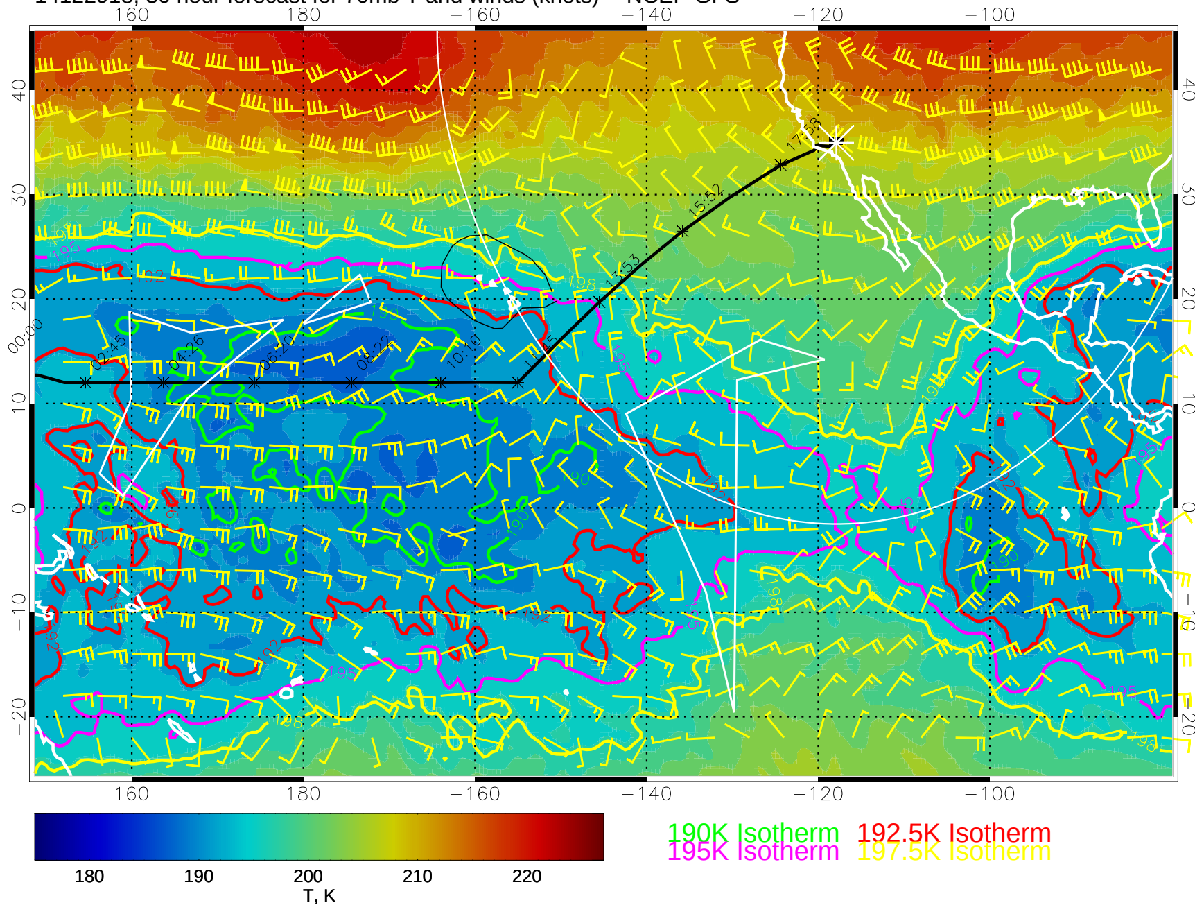
14122918, 30 hour forecast for 70mb T and winds (knots) -- NCEP GFS
