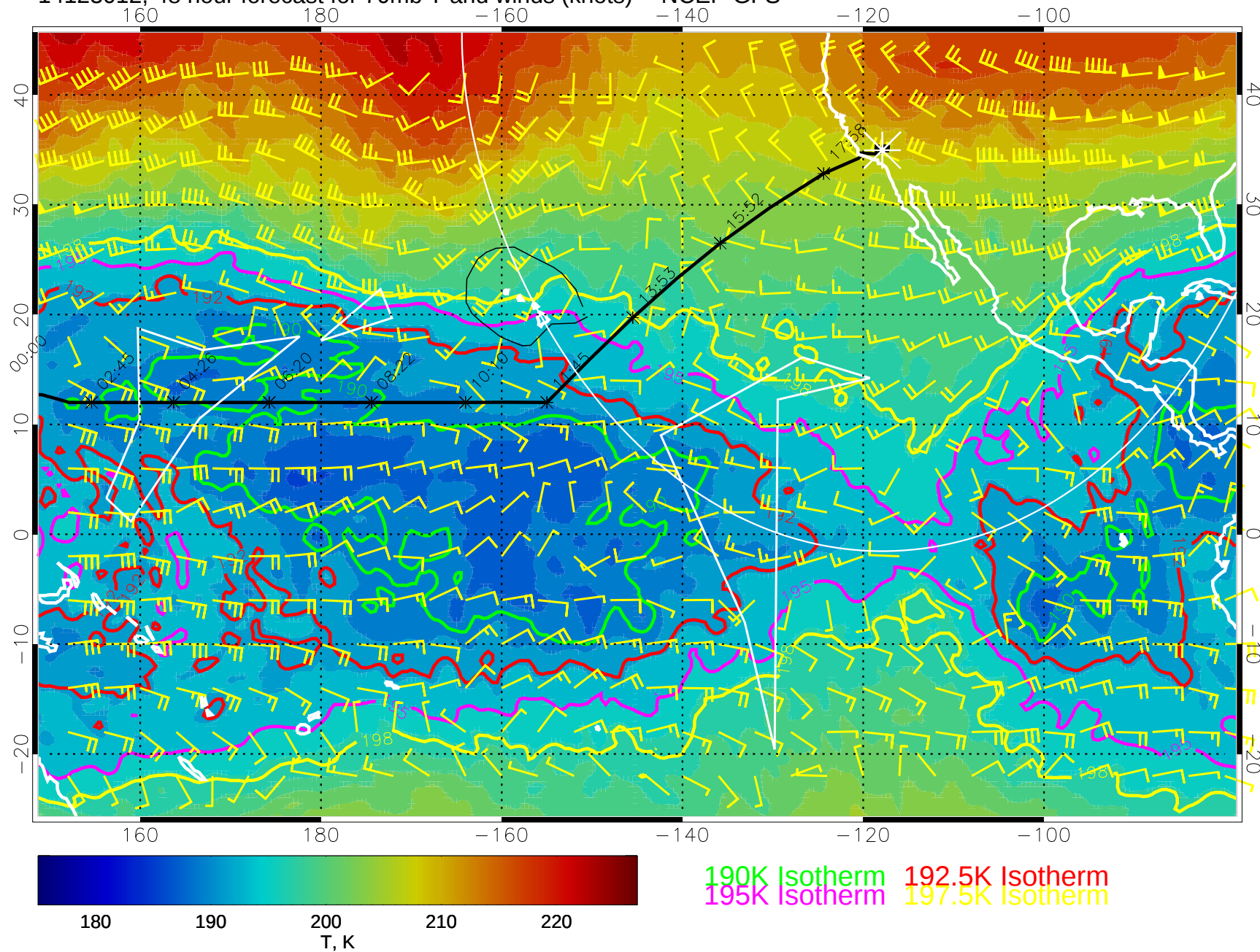
14123012, 48 hour forecast for 70mb T and winds (knots) -- NCEP GFS
