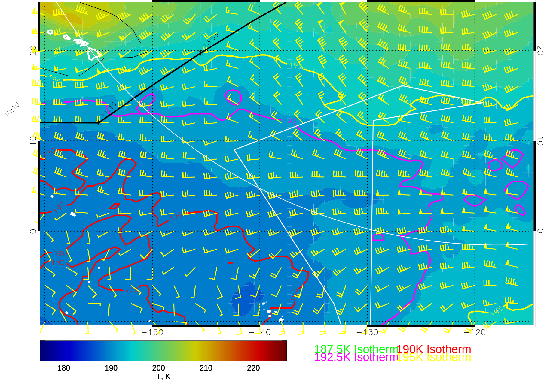
14123106, 66 hour forecast for 100mb T and winds (knots) -- NCEP GFS
