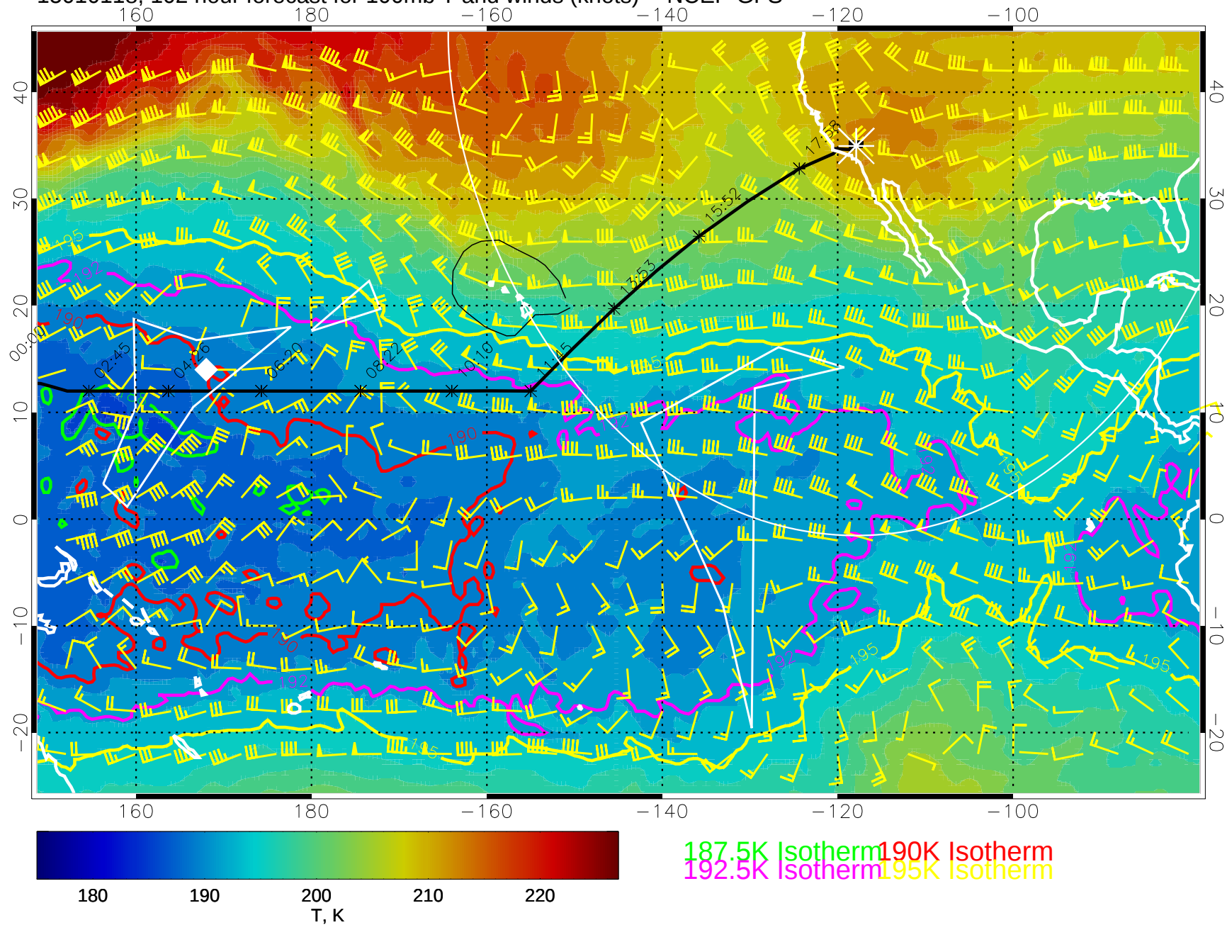
15010118, 102 hour forecast for 100mb T and winds (knots) -- NCEP GFS
