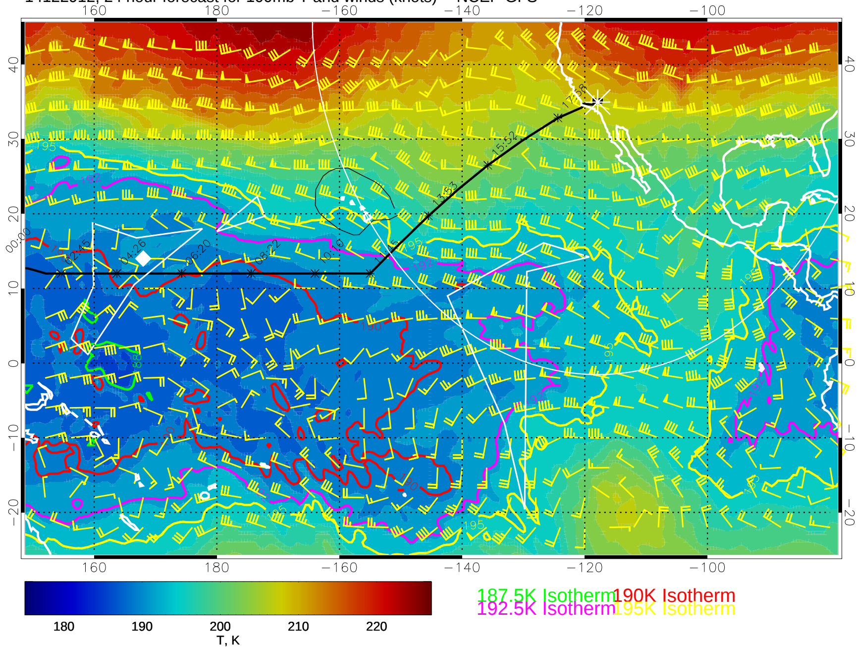
14122912, 24 hour forecast for 100mb T and winds (knots) -- NCEP GFS
