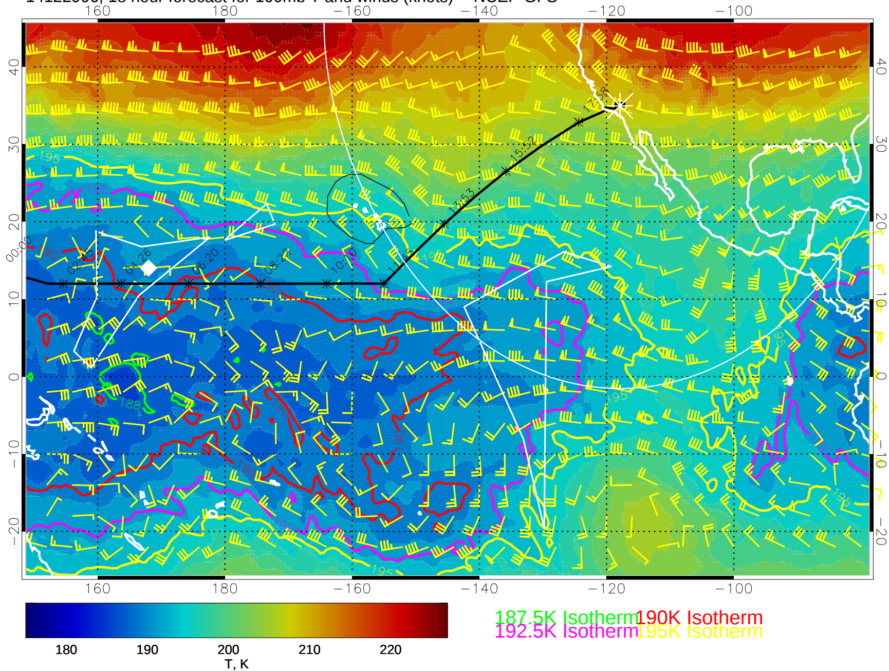
14122906, 18 hour forecast for 100mb T and winds (knots) -- NCEP GFS
