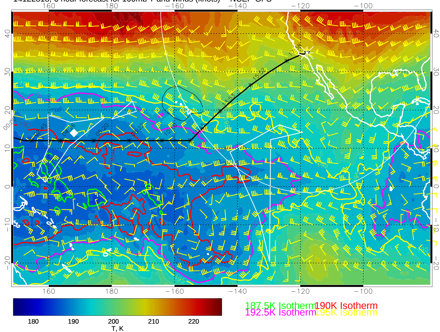
14122818, 6 hour forecast for 100mb T and winds (knots) -- NCEP GFS
