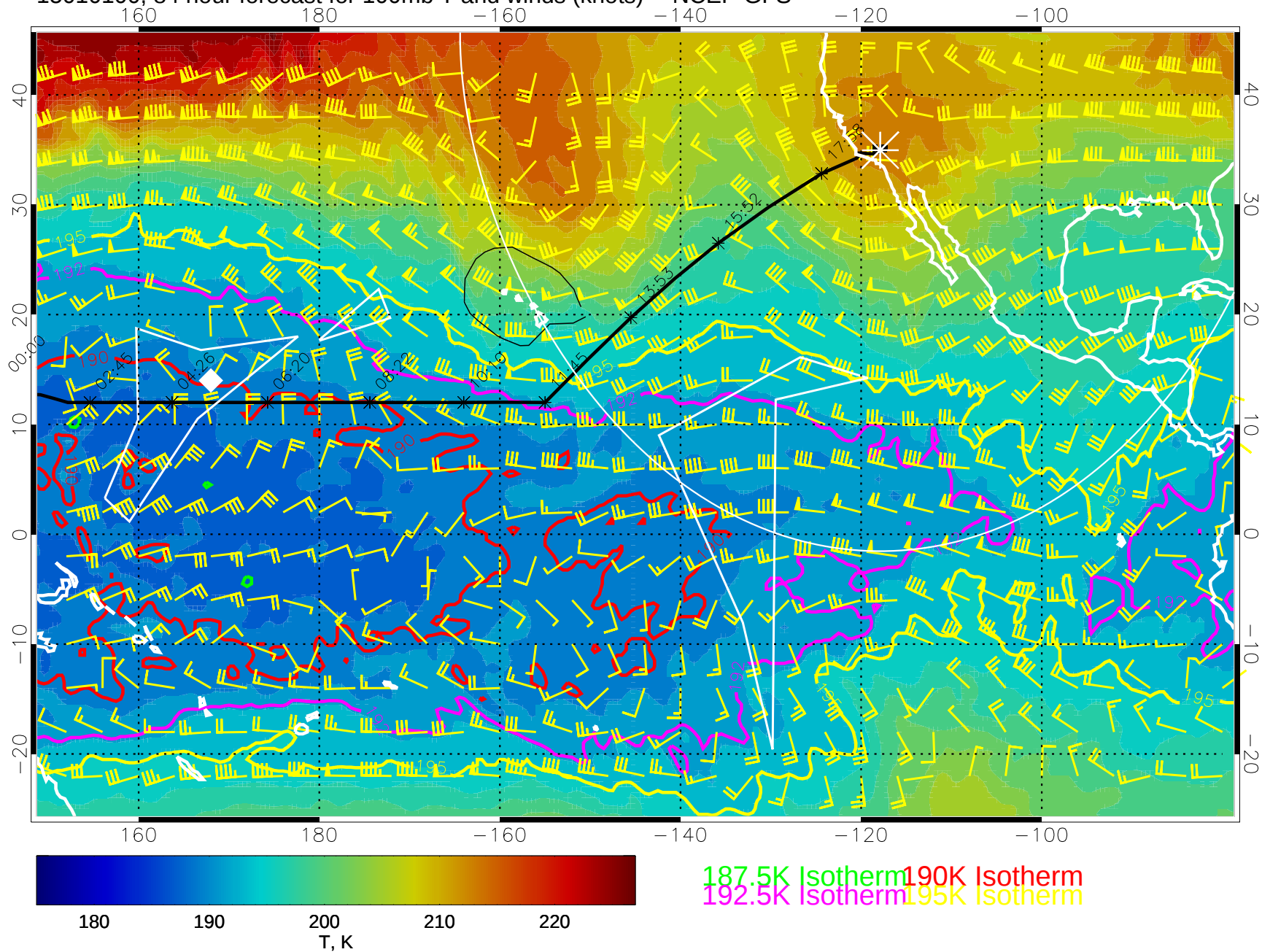
15010100, 84 hour forecast for 100mb T and winds (knots) -- NCEP GFS
