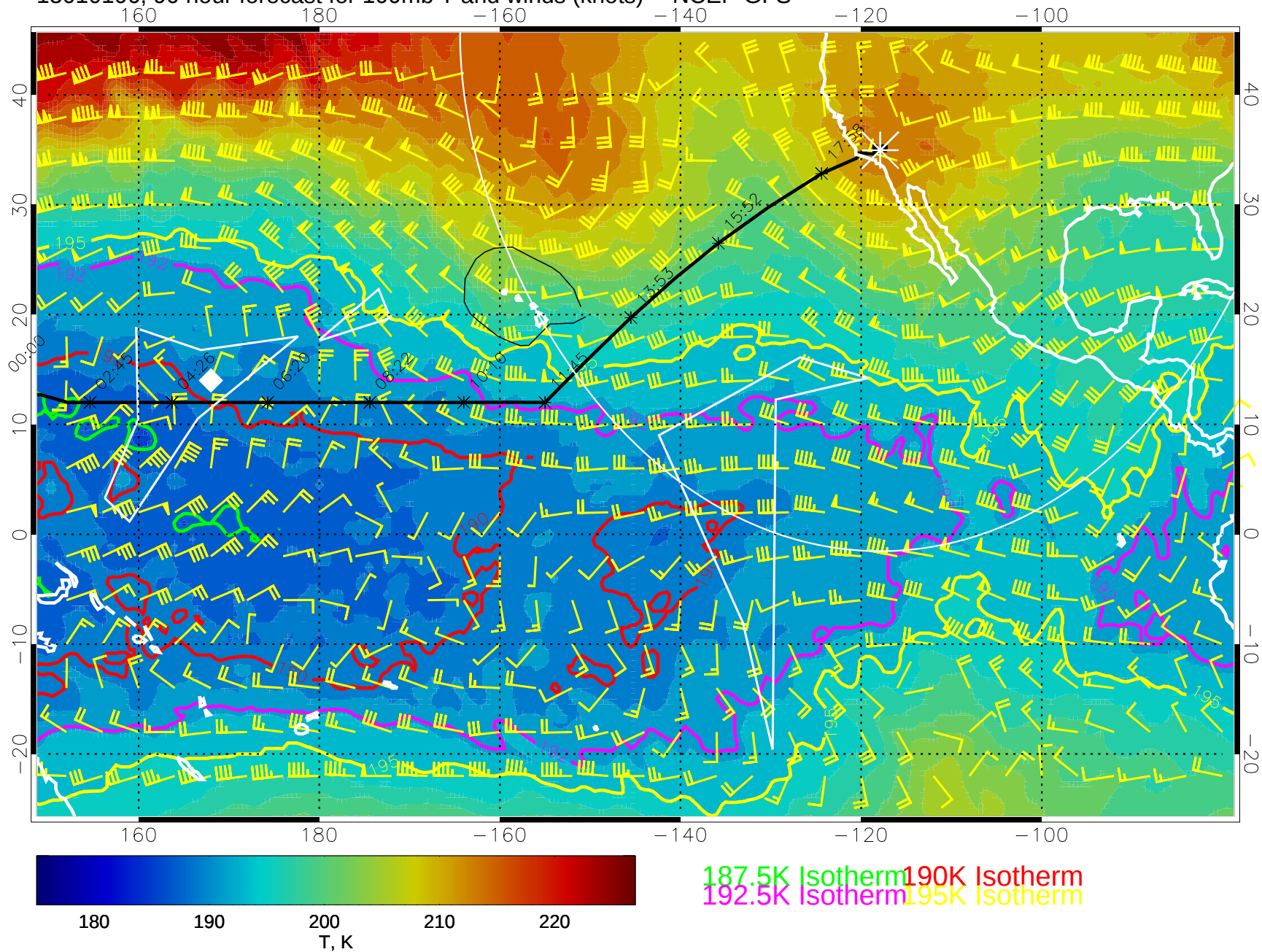
15010106, 90 hour forecast for 100mb T and winds (knots) -- NCEP GFS
