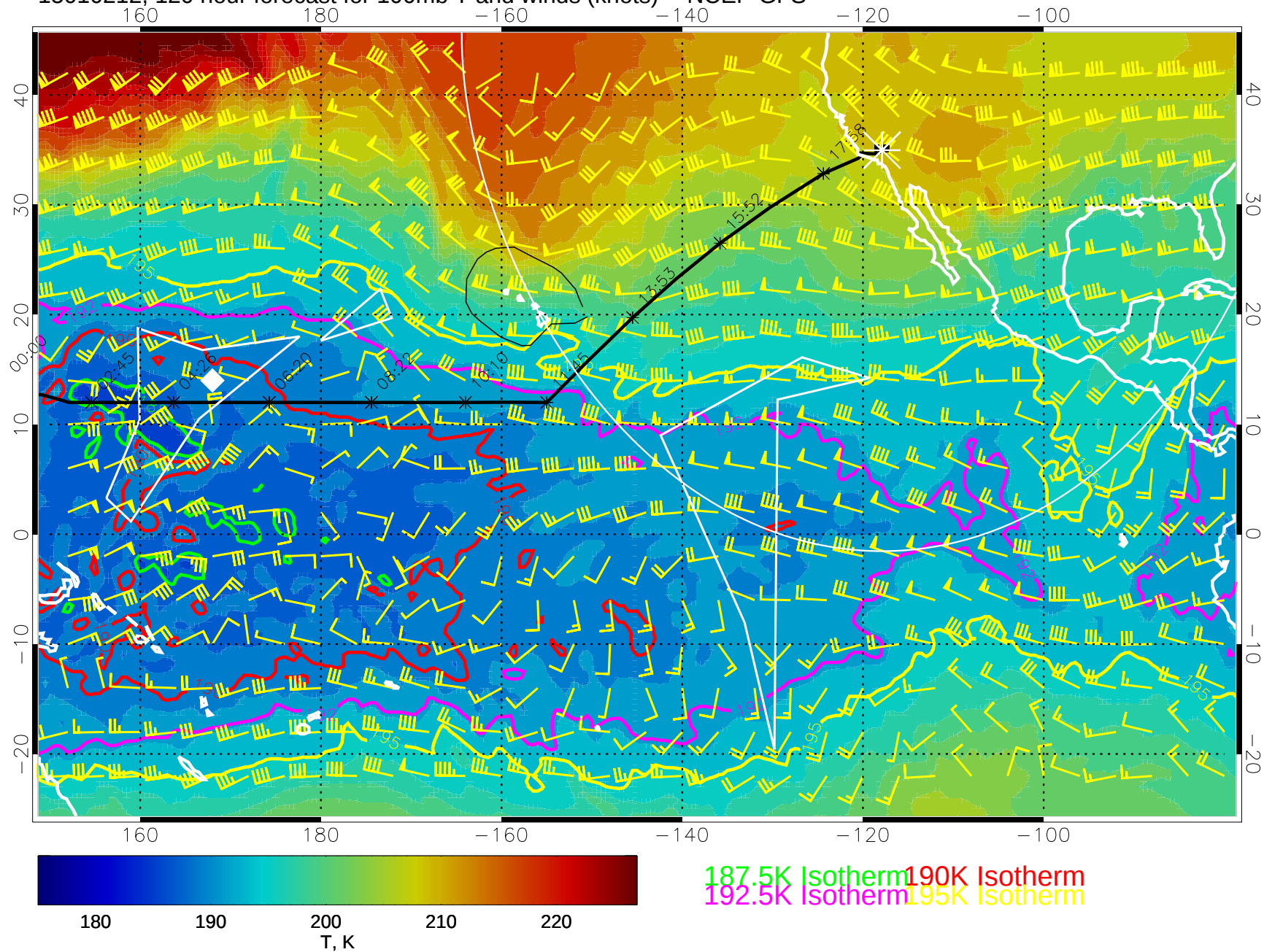
15010212, 120 hour forecast for 100mb T and winds (knots) -- NCEP GFS
